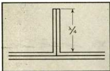
Fig. 4. A coaxial resonant cavity may be used as a stub support for a coaxial line.
