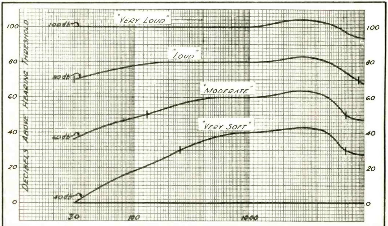
Fig. 3. Frequency response of normal ears at different loudness levels
