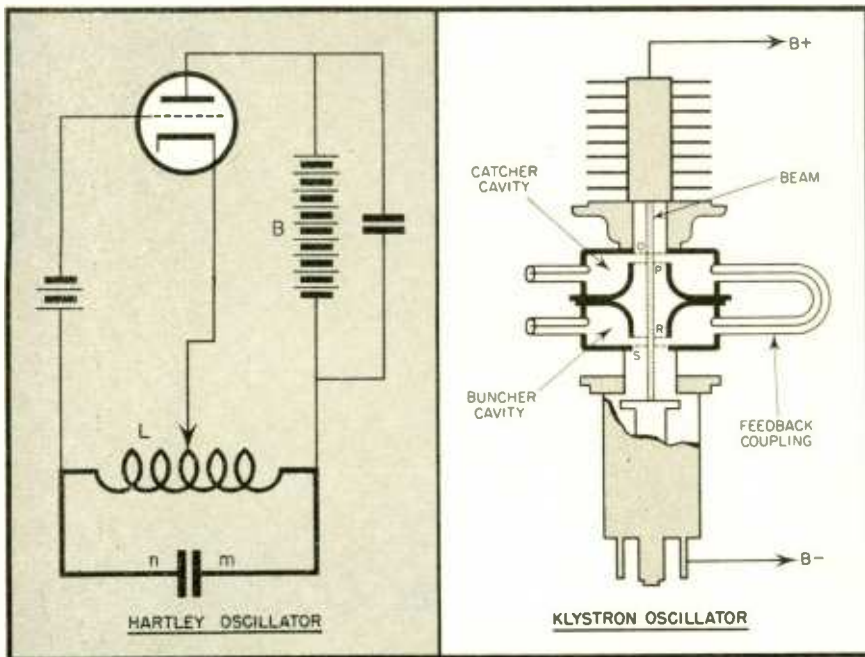
Fig. 1. Resonant cavities and resonant circuits in r-f oscillators. Cavities are more useful at higher frequencies than lumped-constant tank circuits, but are physically too large to be used at low radio frequencies
