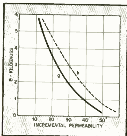
Fig. 2. Incremental permeability curves
