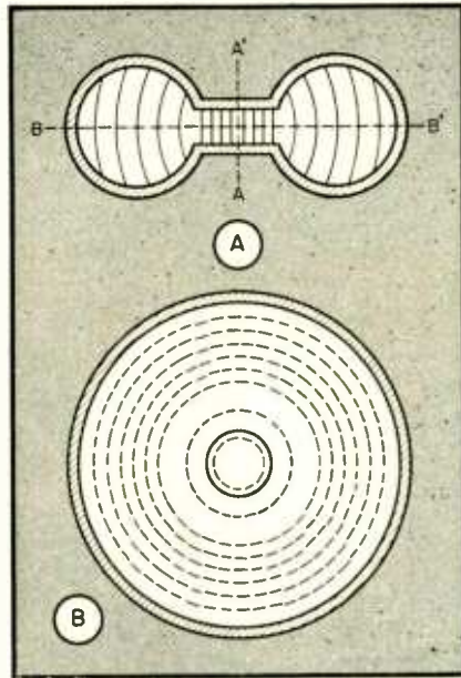
Fig. 7. Rhumbatron type of re-entrant cavity. (B) is a cross-section of the resonator cut along the line BB'
