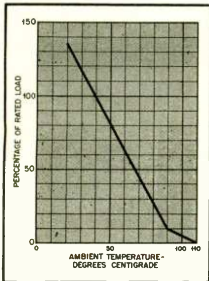
Fig. 6. Derating curve, composition potentiometers
