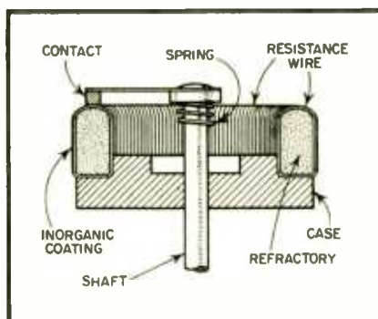
Fig. 1. Cross-section of power rheostat
