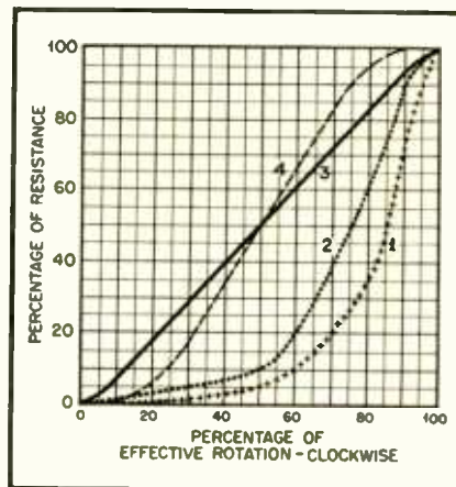
Fig. 7. Tapers for composition potentiometers
