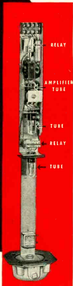
PHOTO-ELECTRIC DOOR CONTROL Above unit manufactured by General Electric Co., is a part of STANLEY "MAG:C DOOR" CONTROLS.
