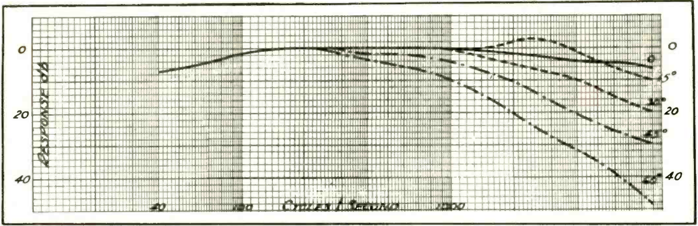
Fig. 2. Relative response with listener at various angles to loudspeaker
