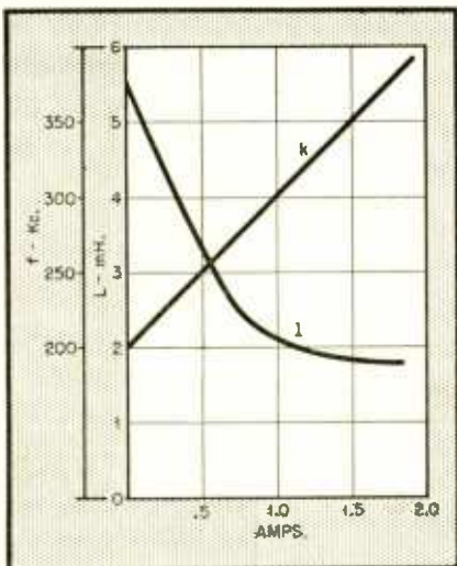
Fig. 4. Variation of inductance and frequency vs. d-c current
