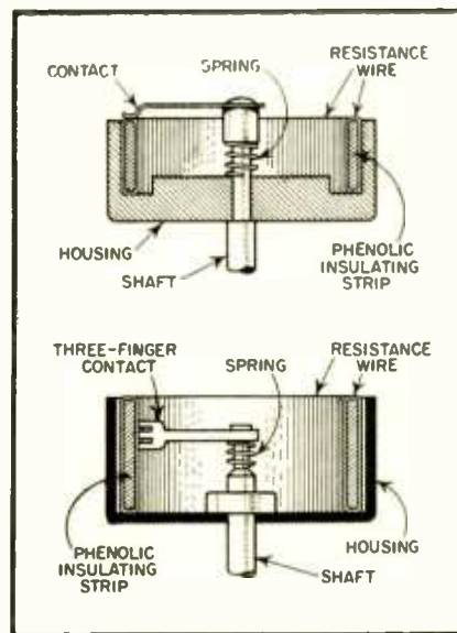
Fig. 4. Wire-wound potentiometer construction
