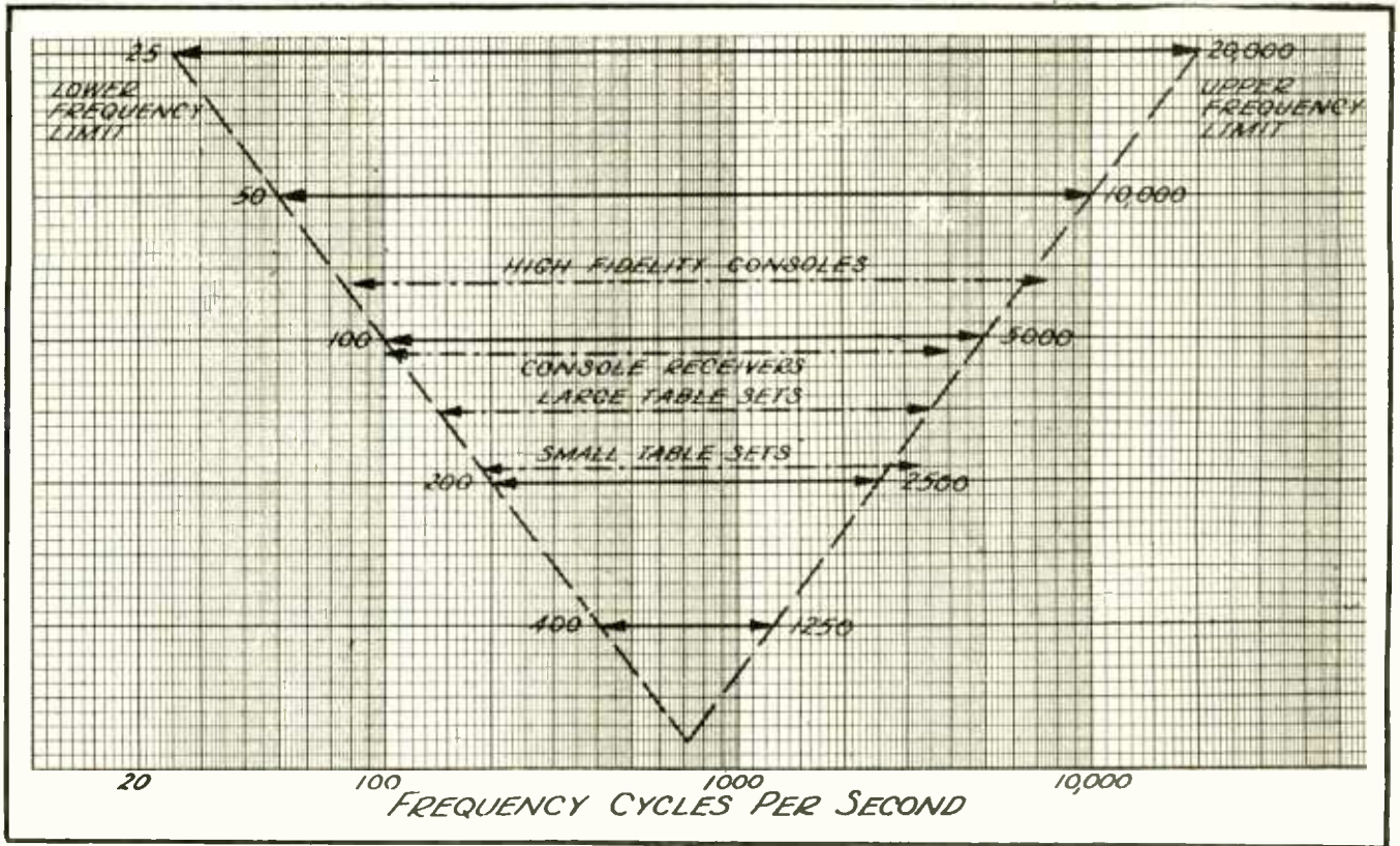
Fig. 1. Preferred lower and upper frequency limits. (Product equals 500,000)
