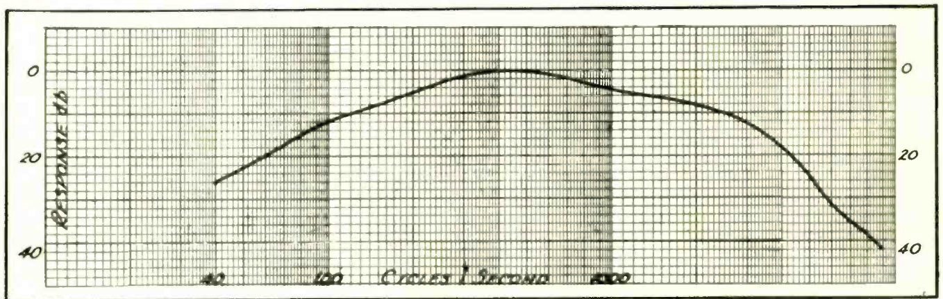
Fig. 4. Aural frequency response, young listener seated at 45° to loud-speaker, normal hearing, moderate loudness level
