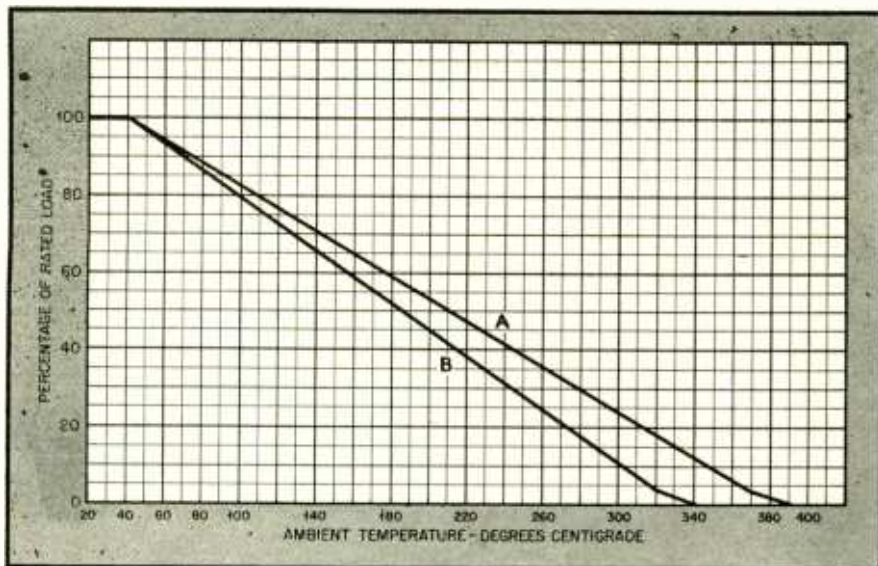
Fig. 2. Derating curve for power rheostats operated at elevated temperatures
