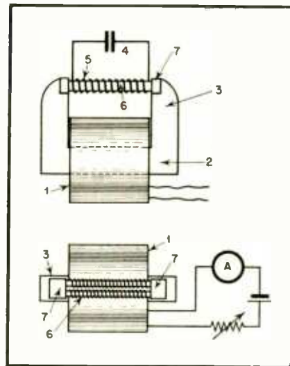
Fig. 3. Closed-type inductor design
