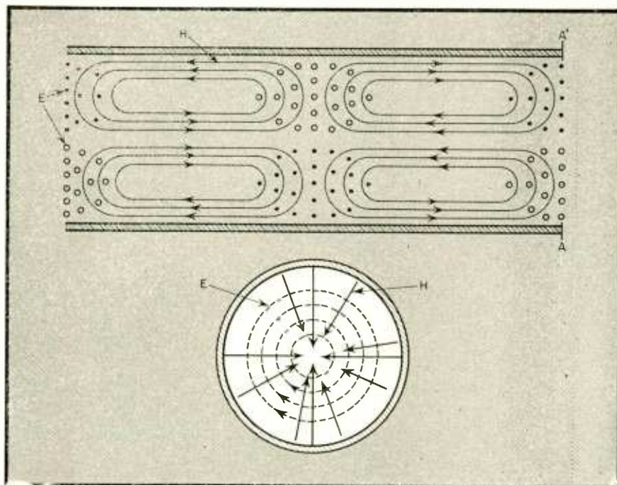
Fig. 6. The H_0 mode of a cylindrical wave guide. The section shown is a wavelength long and indicates a wave traveling to the left.
