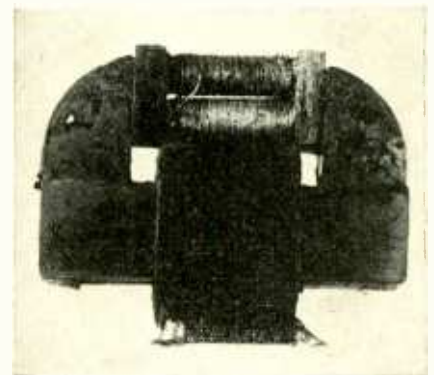
Fig. 6. Experimental inductor
