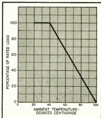
Fig. 3. Derating curve for low-temperature type, wire-wound potentiometer
