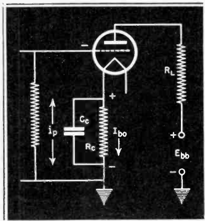
Fig. 5. Triode amplifier showing cathode-resistor method of obtaining grid bias.
