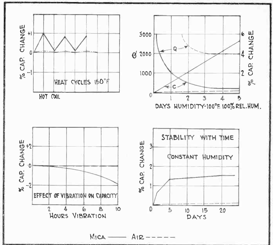
Fig. 6. Typical air vs. mica trimmer capacitor characteristics.
