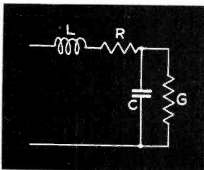
Fig. 7. Equivalent circuit of fixed capacitor.
