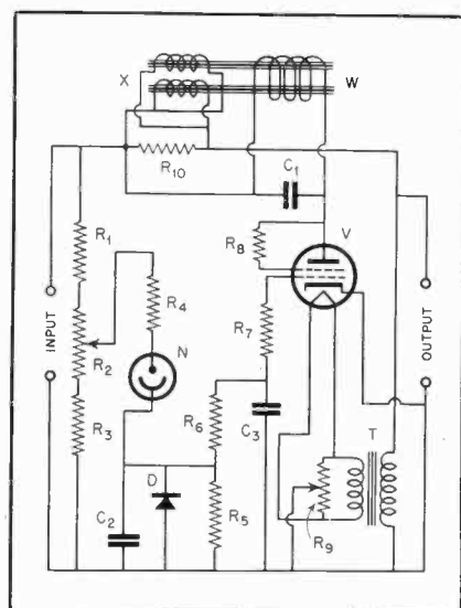
Fig. 1. Circuit of voltage stabilizer.
