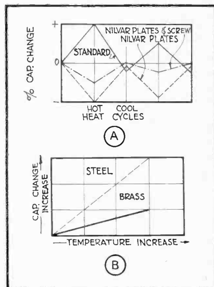
Fig. 5. Effects of temperature on compression-type trimmer capacitor.
