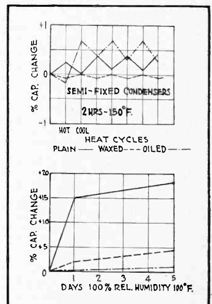
Fig. 9. Semi-fixed capacitor characteristics.
