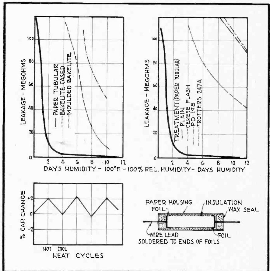
Fig. 13. Humidity characteristics of paper capacitors.
