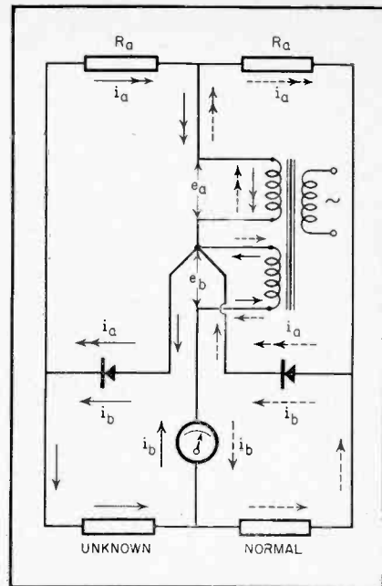
Fig. 2. Impedance bridge circuit.
