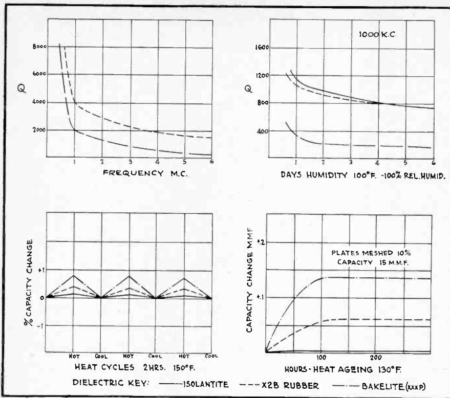
Fig. 12. Typical characteristics of a variable air capacitor.
