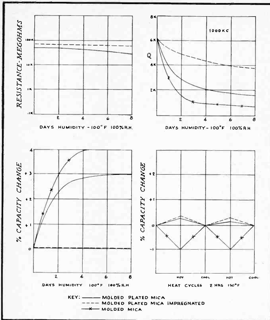
Fig. 8. Plated mica vs. mica film fixed capacitor characteristics.
