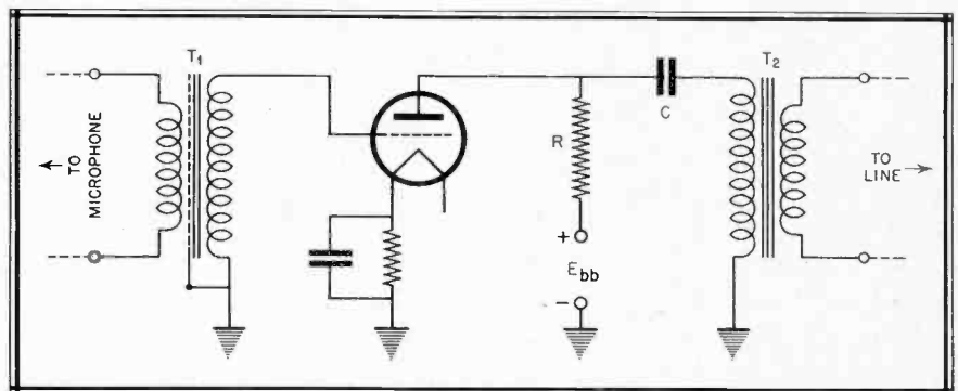
Fig. 2. Pre-amplifier with shunt-feed in the plate circuit.
