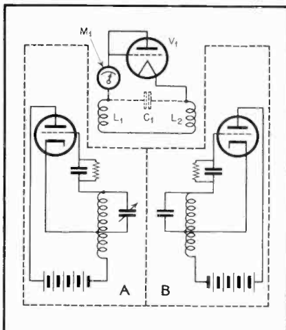
Fig. 1. Circuit of transducer.
