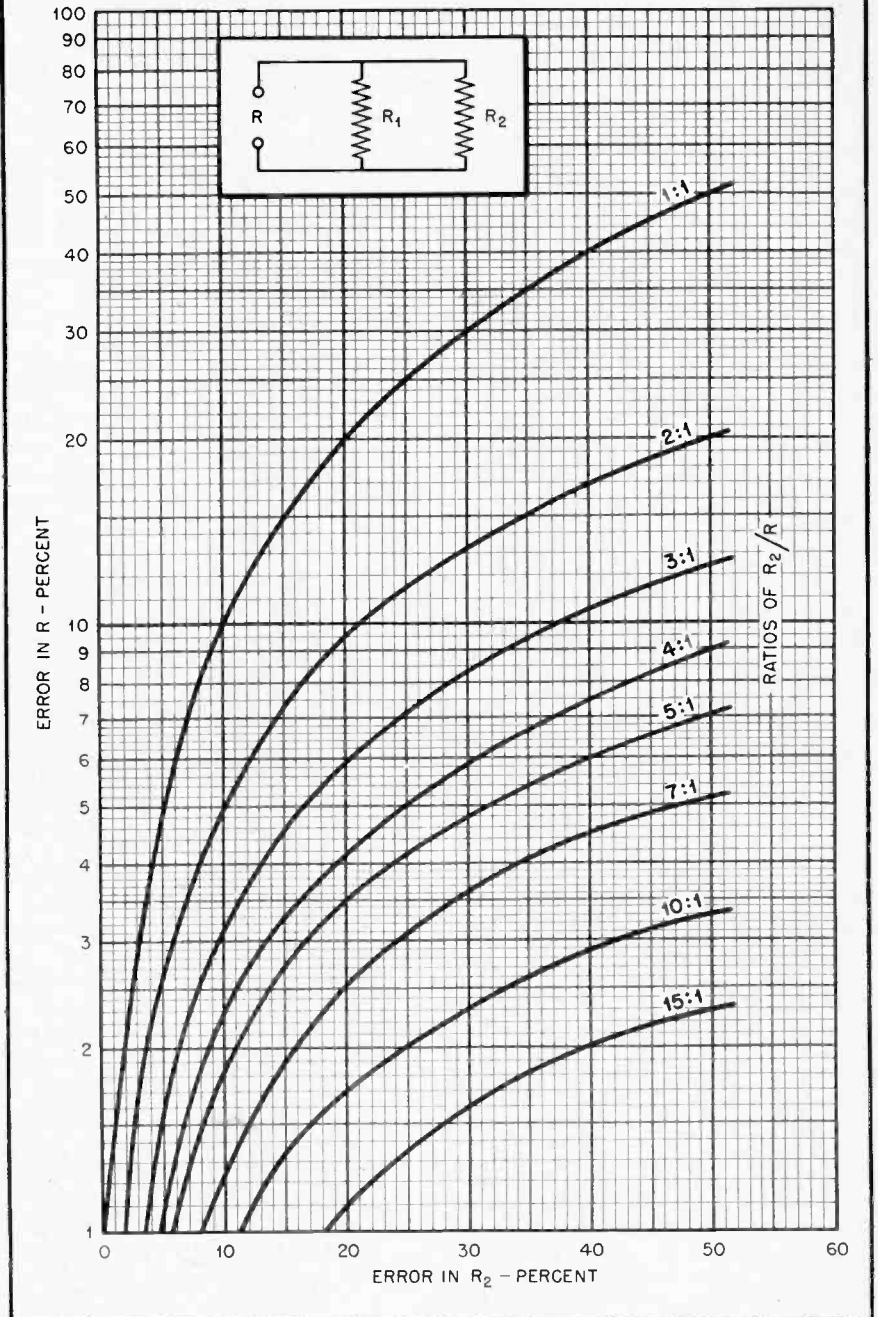
ERROR IN R Vs. ERROR IN R_2 FOR RATIOS OF R_2/R
