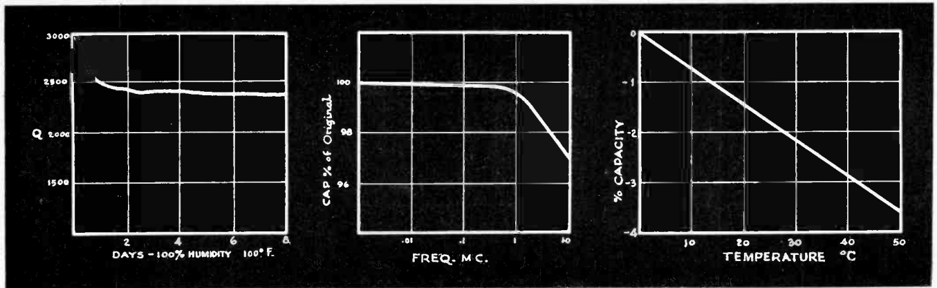
Fig. 10. Characteristic curves of Titanium Dioxide type of fixed capacitor.
