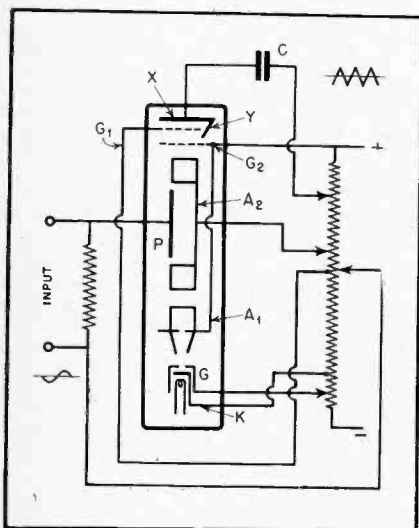
Fig. 1. Signal converter tube.
