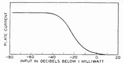
Fig. 1. Input-output characteristic.
