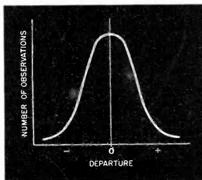
Fig. 1. Typical probability curve.
