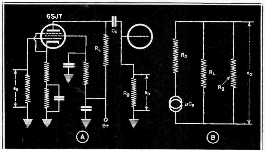
Fig. 1. Resistance-coupled wide-band amplifier and its equivalent circuit.
