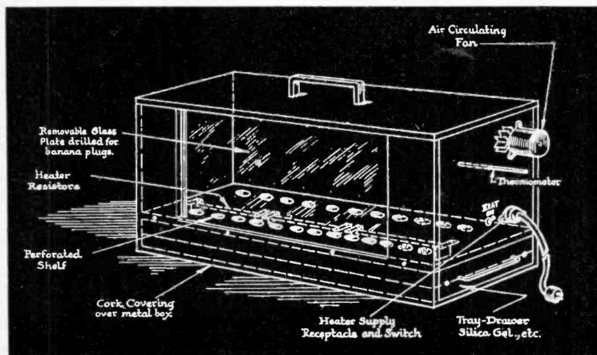
Fig. 3. Mechanical details of typical test chamber.
