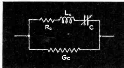
Fig. 11. Equivalent circuit of variable air capacitor.
