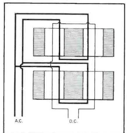
Fig. 2. Winding arrangement of choke.
