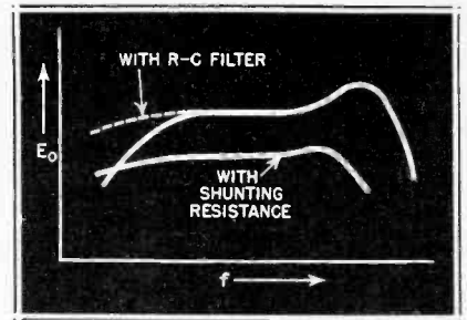
Fig. 3. Frequency response curves for transformer coupling.
