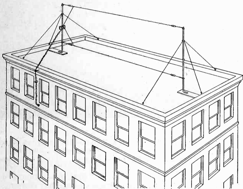
General Motors Antenna Installation No. G.M. 101 . . . a type particularly well adapted for apartments or city dwellings where many electrical disturbances must be considered.
