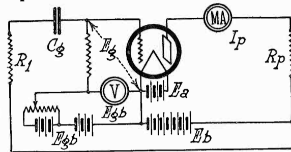
Fig. 3. Circuit of Typical Resistance Coupled Amplifier.
