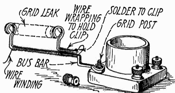
Combined Grid Condenser and Leak.
