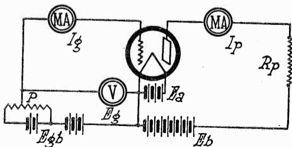
Fig. 1. Circuit Arrangement for Securing Curves in Fig. 2.
