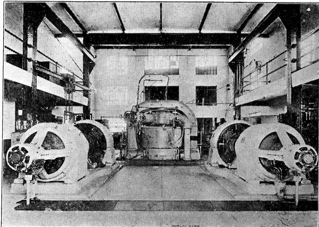
500 Watt Arc Transmitter at Pearl Harbor, T. H.
