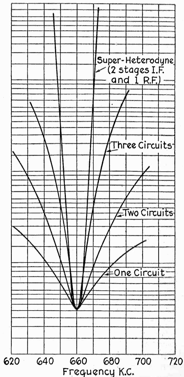
Relative Selectivity of Receivers.
