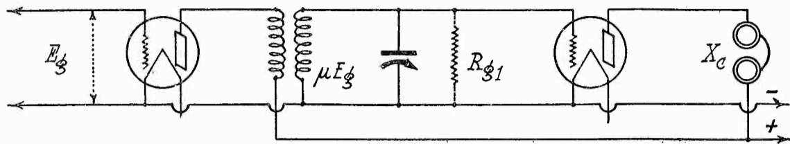
Fig. 3. Effect of Change in Load Resistance.
