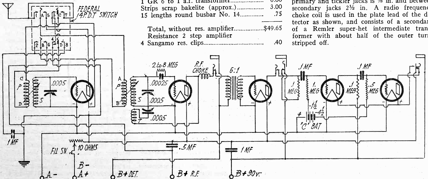
Circuit Diagram for Receiver "A La Brasspounder."
