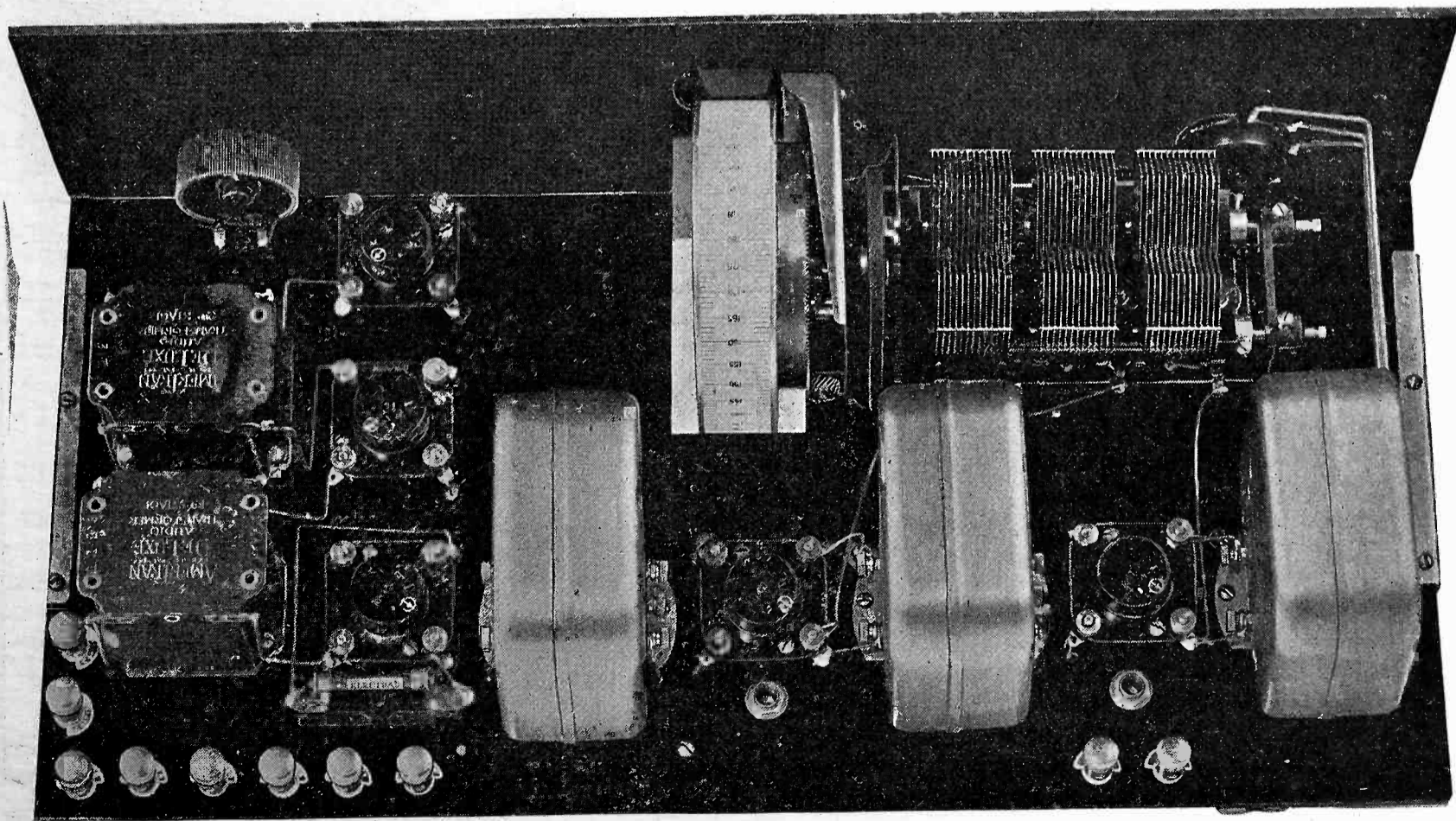
Rear View of Quadrphase.
