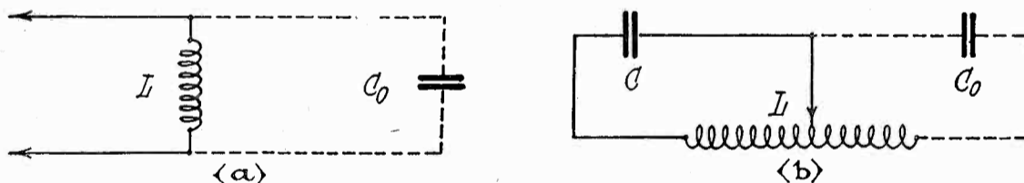
Fig. 2. Effect of Distributed Capacity.
