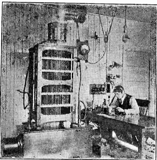
7½ K. W. Transmitter and Receiving Equipment at the Massie Wireless Station, San Francisco, 1907-1909.
