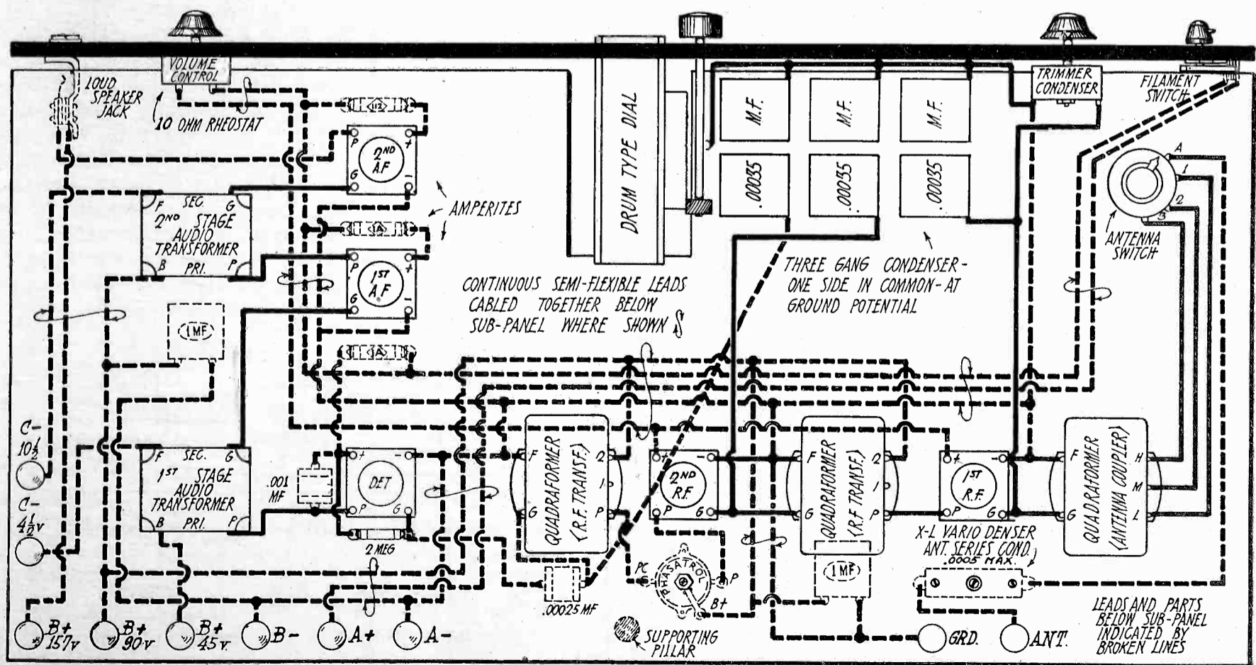
Fig. 3. Pictorial Wiring Diagram.
