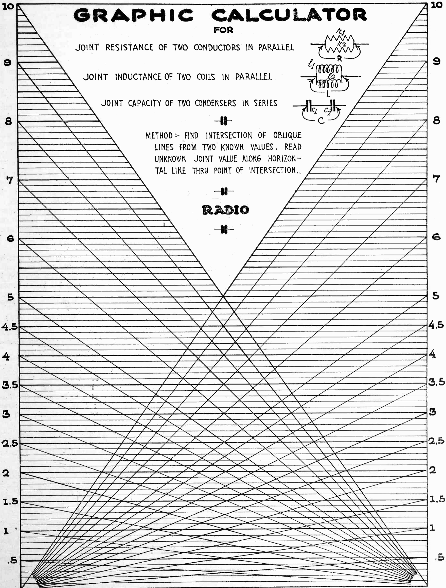
Handy Chart for Figuring Parallel Resistances and Inductances and Series Capacities.
