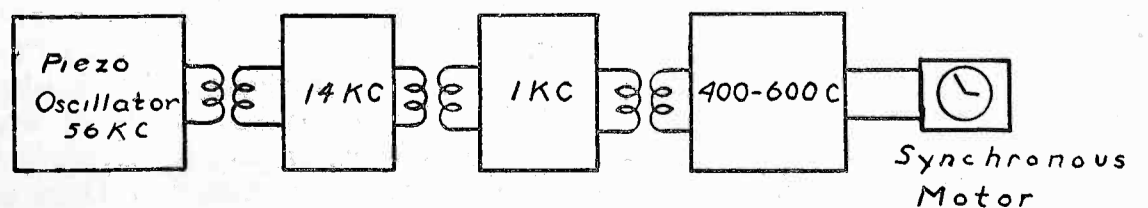
Fig. 4. Method Used in Calibrating Quartz Crystal.
