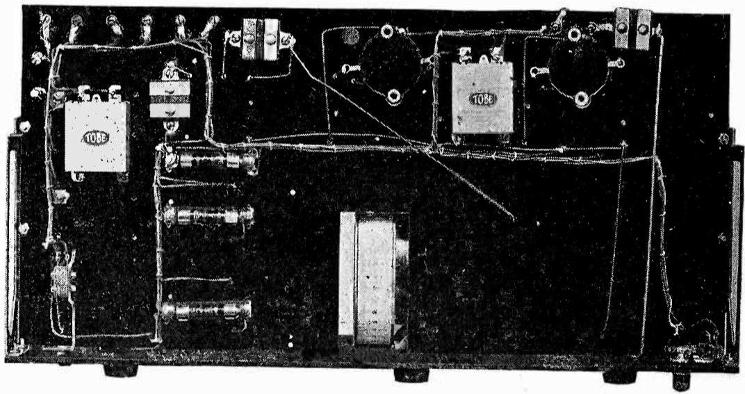
Lower Side of Sub-Panel.
