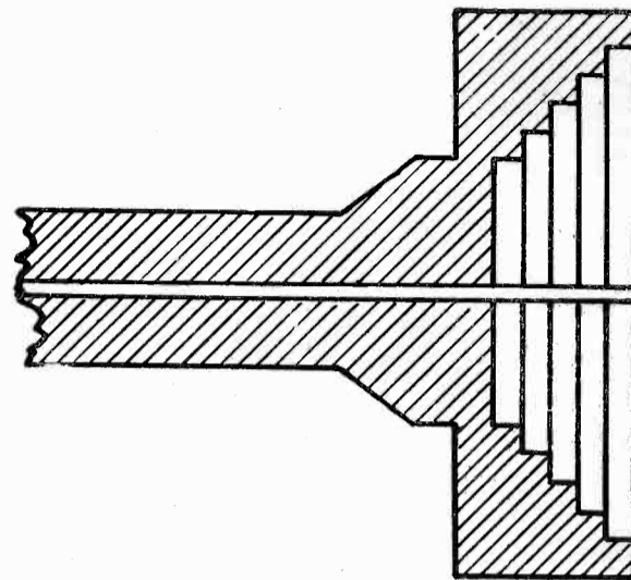
Fig. 2. Step Chuck.
