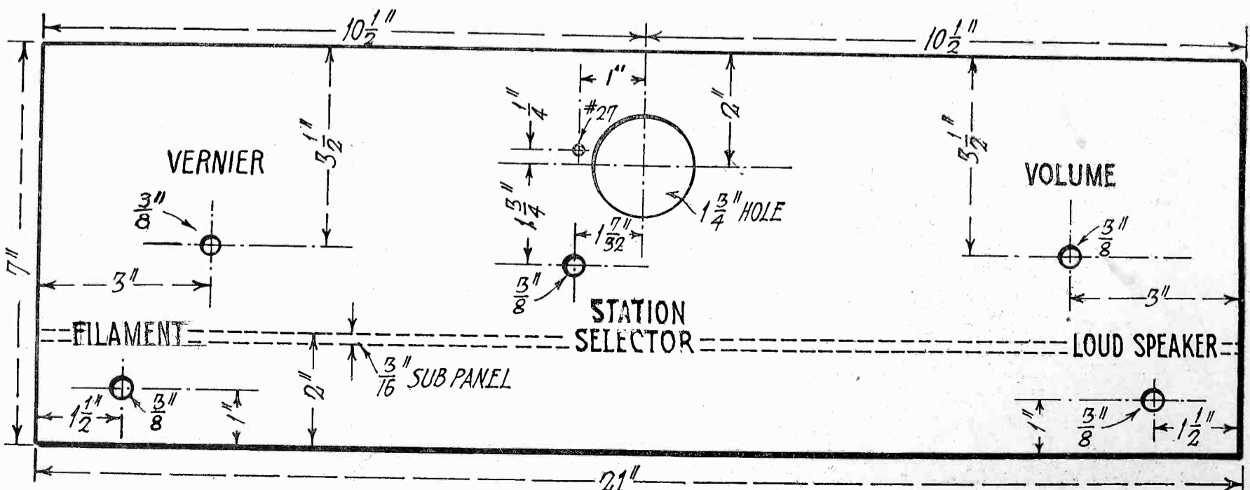
Fig. 2. Panel Layout.
