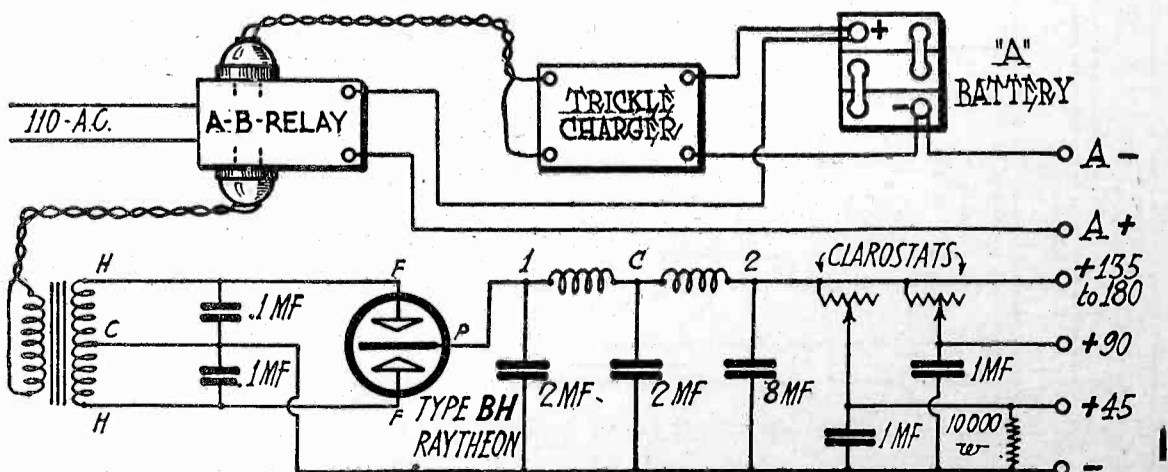
Fig. 6. Circuit Diagram of Power Plant.
