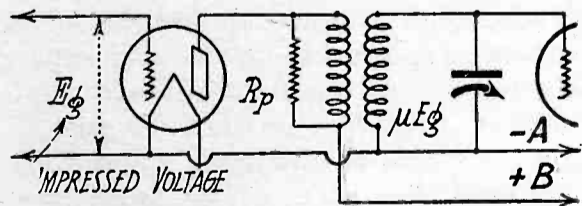
Fig. 1. Effect of Plate Resistance.
