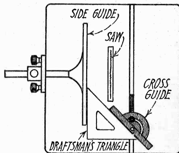
Fig. 3. Setting Saw-Table Cross-Guide.
