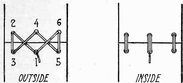
Fig. 6. Lacing Belt with Rawhide or Wire.
