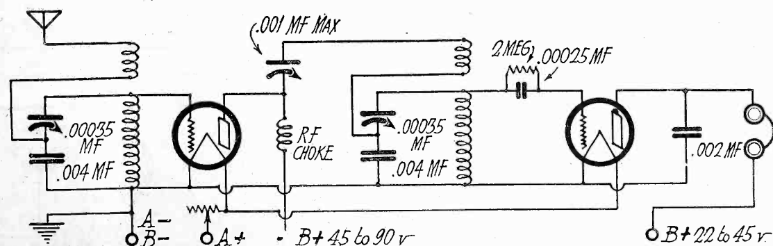
Fig. 1. Loftin and White Circuit.
