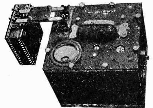
Fig. 5. Wavemeter Used as Secondary Standard.
