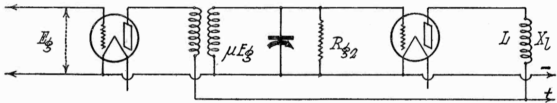
Fig. 4. Effect of Change in Plate Impedance.
