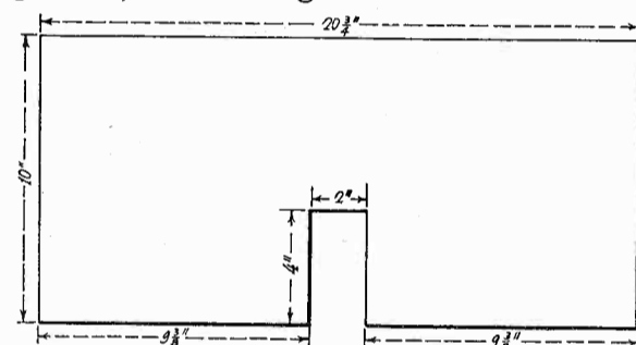
Fig. 4. Subpanel Dimensions.
