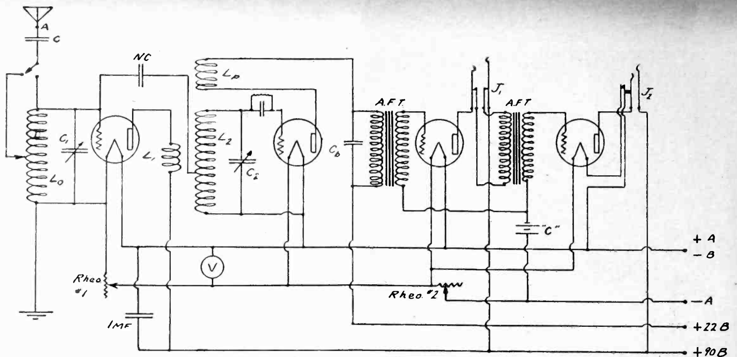
Fig. 2. Circuit Diagram for One Stage R. F., Detector and Two Stages A. F.
