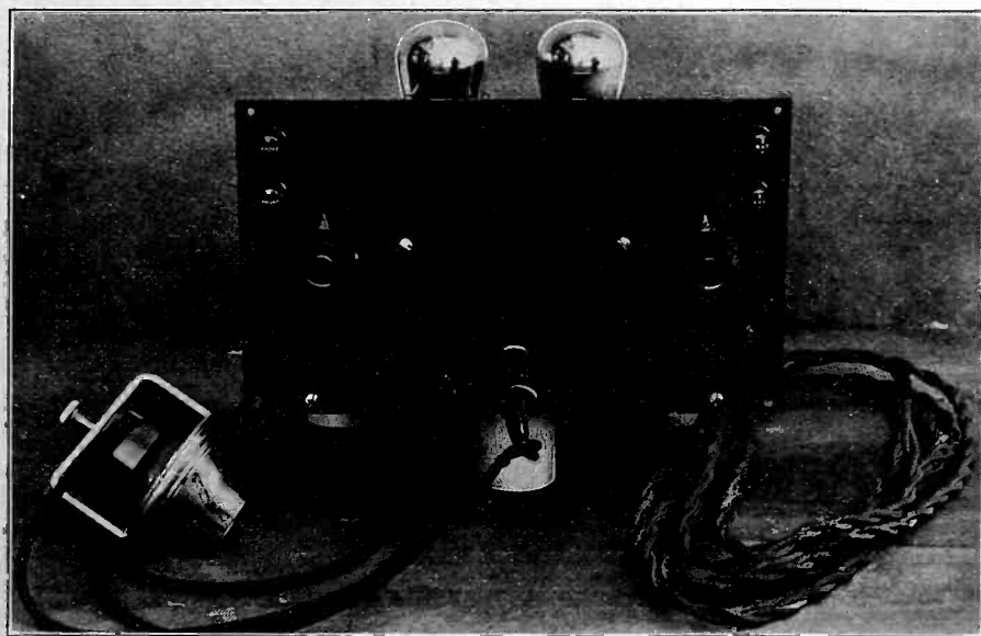
Fig. 1. Front panel view of the "A"-Batteryless two-stage audio amplifier. The amplifier tubes are arranged to project through the top of the cabinet.
