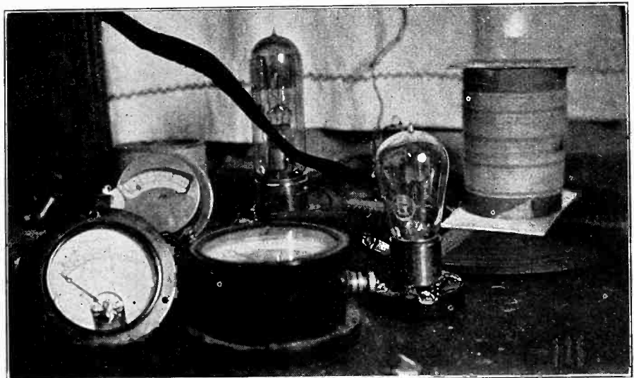
Set-Up for Moduloscope Observations
