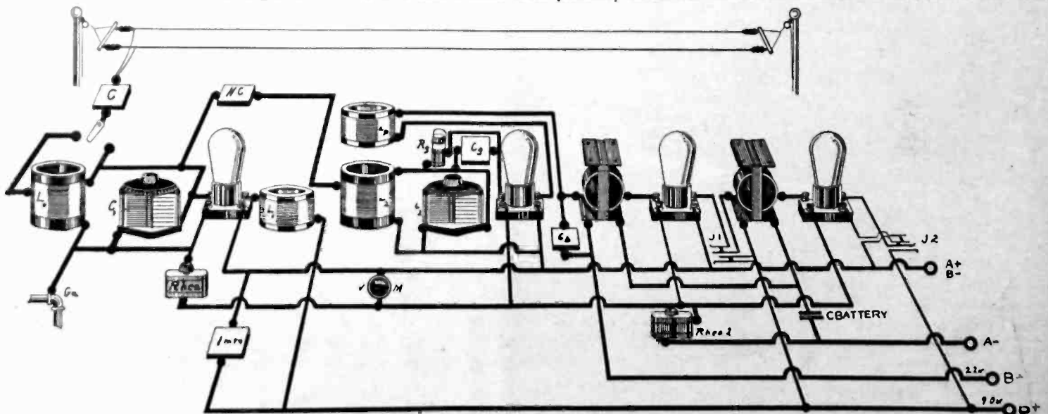
Fig. 3. Pictorial Layout of Parts. ( L_1 , L_2 and L_p should be combined in one regenaformer)
