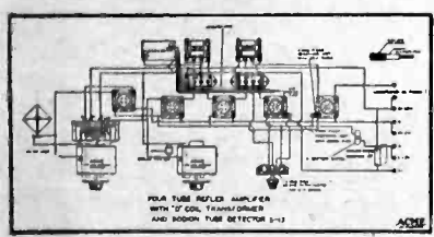
Wiring diagram new Model "S" Acmeflex Kitset
