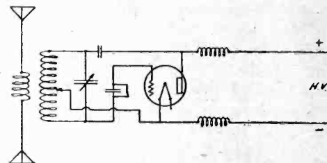
Fig. 4. Coupled Hartley Circuit
