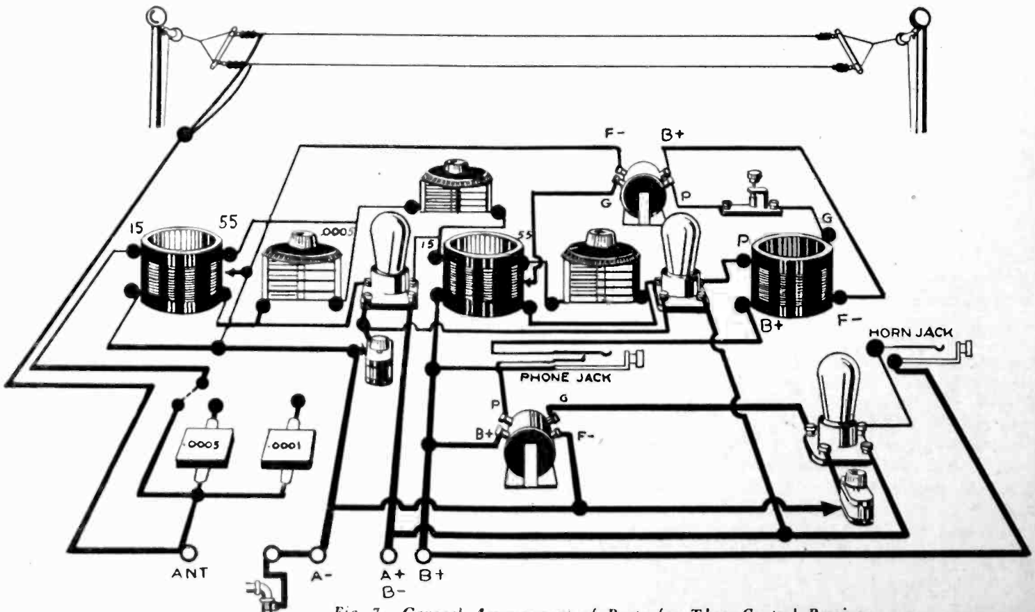
Fig. 7. General Arrangement of Parts for Three-Control Receiver
