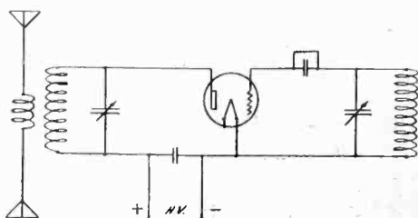
Fig. 3. Coupled Reversed Feed-back Circuit
