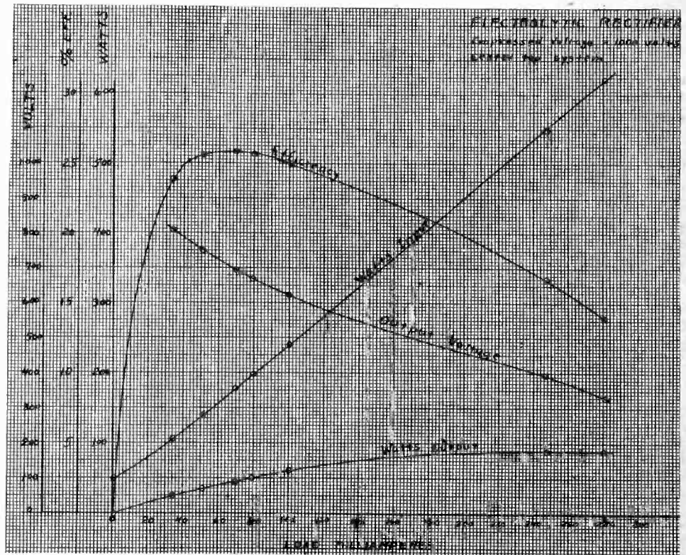
Curves of Electrolytic Rectifier, Center Tap System, with 1000 Volts
