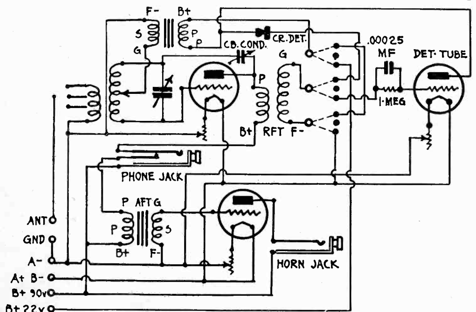
Fig. 4. Circuit Using Either Crystal or Tube Detector
