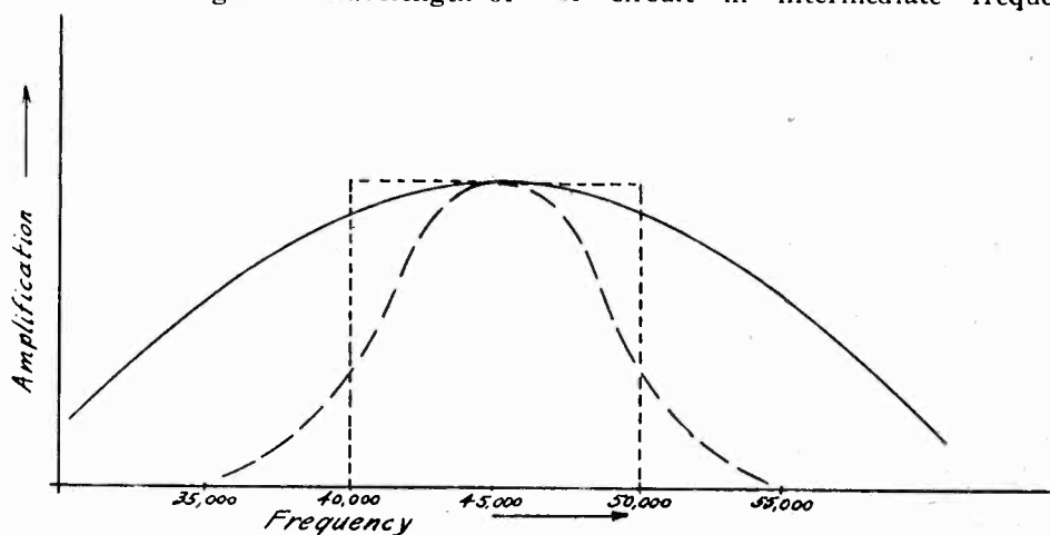
Fig. 2. Frequency-Amplification Characteristics of Three Different Intermediate Frequency Amplifiers ..... Theoretical Ideal Amplifier. - - - - Tuned Circuit Amplifier. ——— Transformer Coupled Amplifier.
