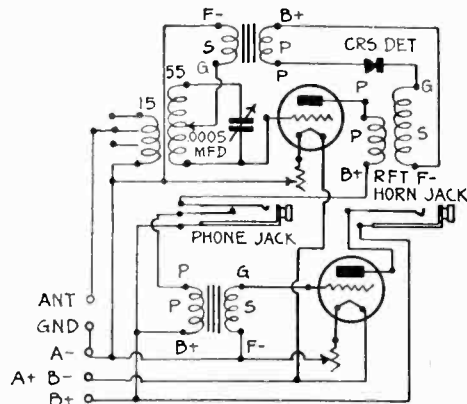
Fig. 1. Single Control Reflex with One Stage of R. F.
