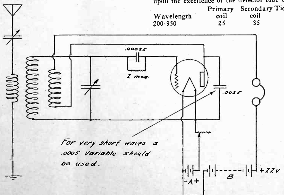
Fig. 2. Circuit Diagram of 3-coil All-wave Receiver
