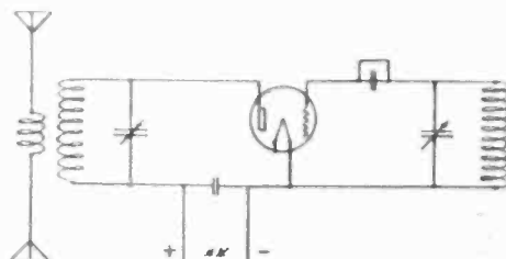
Fig. 3. Coupled Reversed Feed-back Circuit
