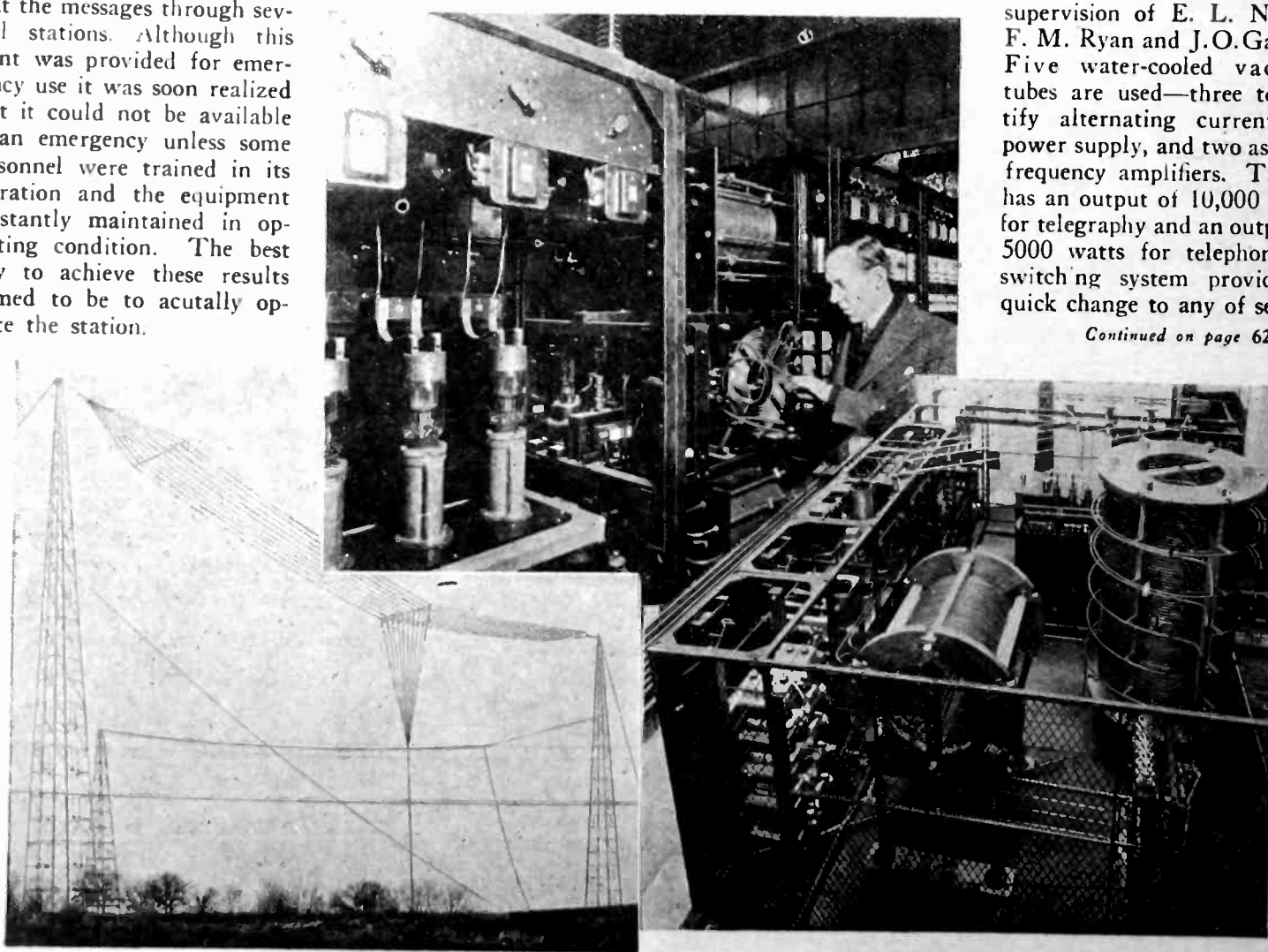
Fort Leavenworth Radio Station, showing antenna system and views of transmitting equipment.
