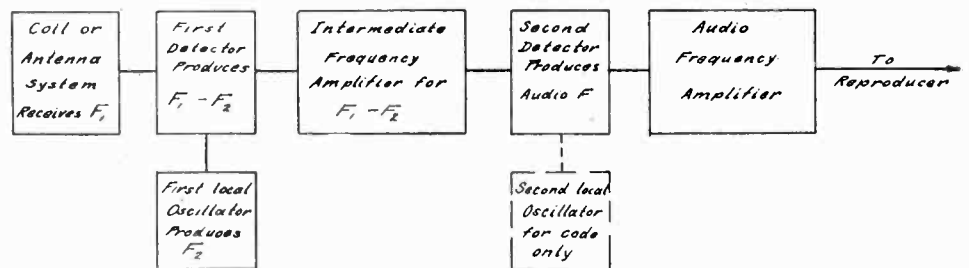
Fig. 1. Schematic Diagram for a Standard Superheterodyne
