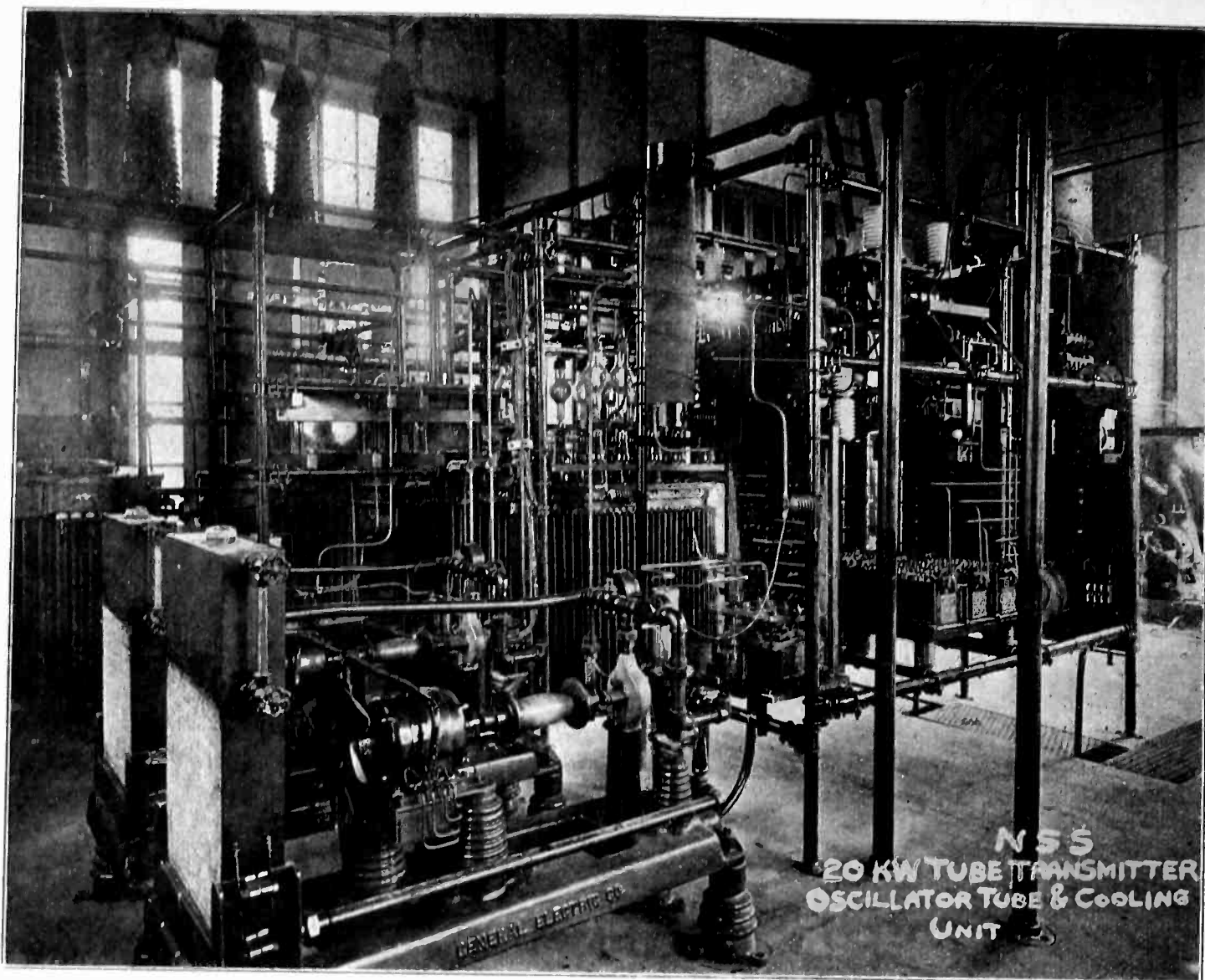
Oscillator Tube and Cooling Unit
