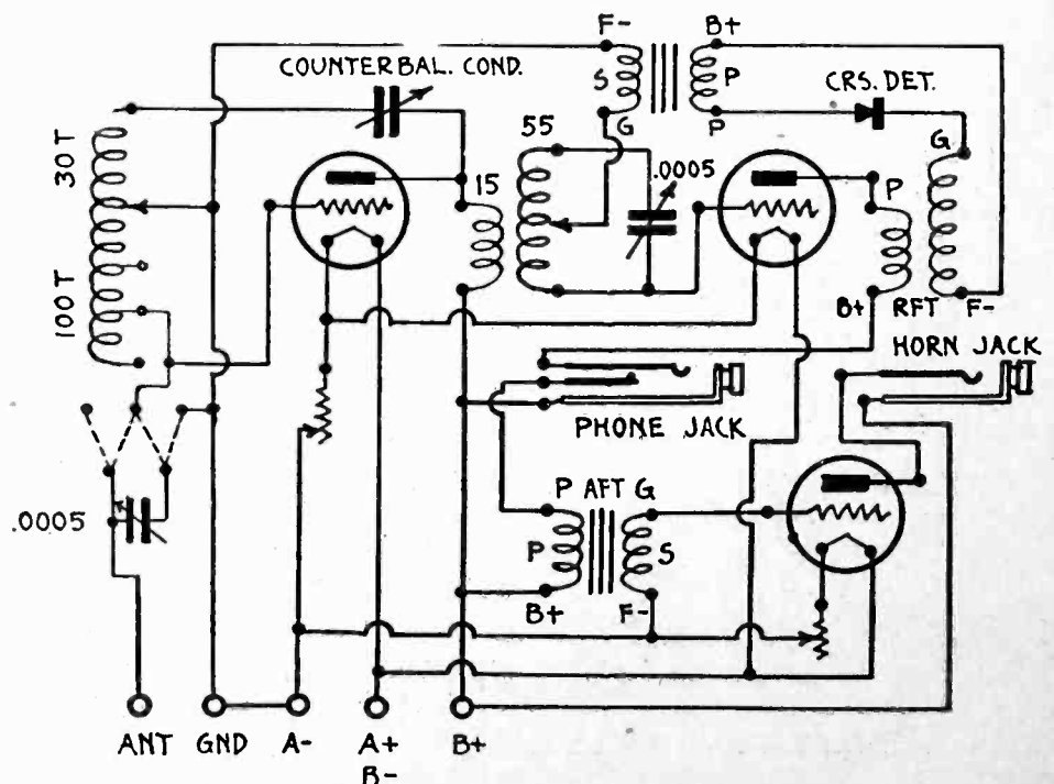
Fig. 2. Single Circuit Tuner with Two Stages of R. F.
