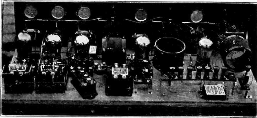
Fig. 6. Rear View of Three Control Receiver
