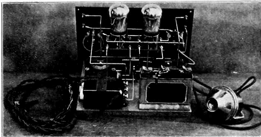
Fig. 2. Back panel view of the amplifier showing the bell ringing transformer for operating the tube filaments. The "C" battery is held to the baseboard by means of a clamp.
