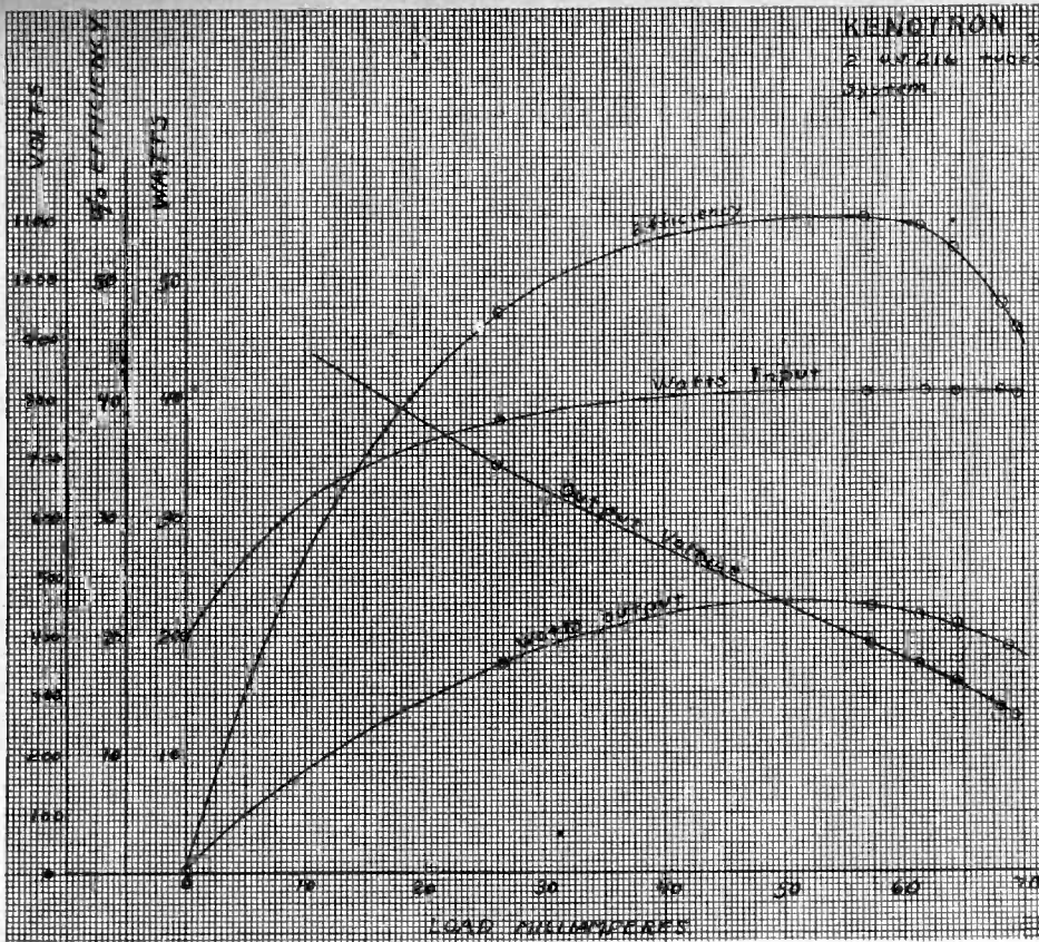
Performance Curves of Kenotron Rectifier. Center Tap System, Using Two UV-216 Tubes
