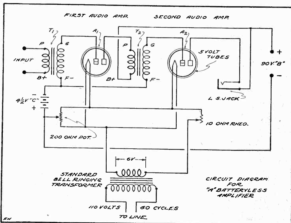
Fig. 3. Circuit diagram. Note the connection of the bell ringing transformer, potentiometer and "C" battery.
