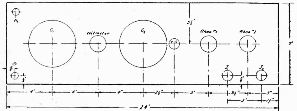
Fig. 4. Panel Layout
