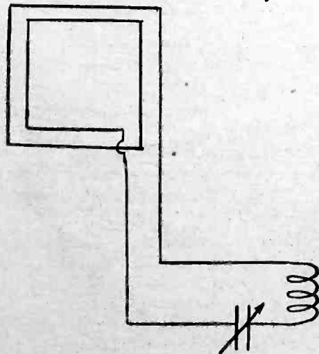
Circuit Diagram of Low-Loss Loop Receiver
