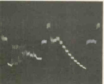
Fig. 13—In the other of the alternate frames of the TV picture, the multiburst signal is followed by the modulated staircase signal.
