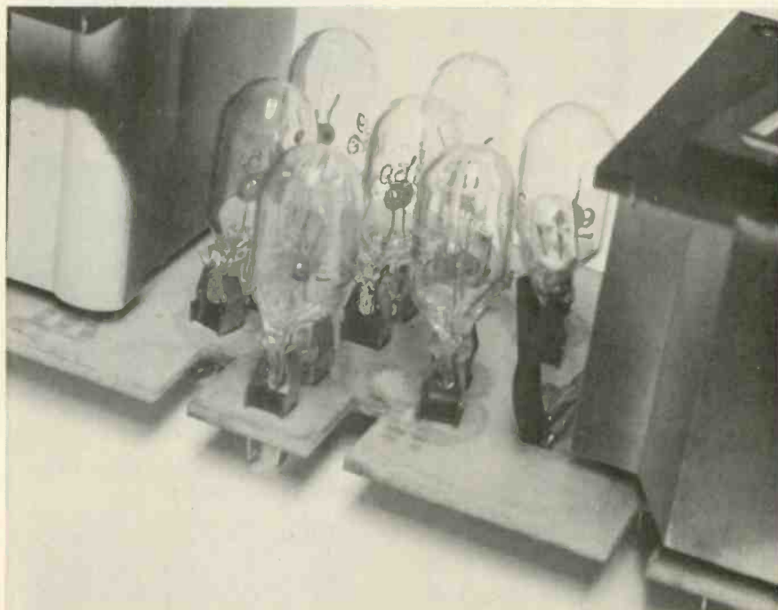
Seven lamps used in tuning indicator lamp assembly to form various segments of a numeral display, plus an additional lamp for the decimal point.
