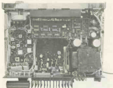
Top view of receiver with digital tuning indicator circuitry in place.
