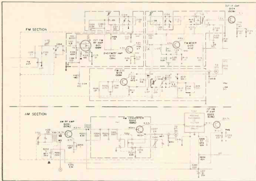
Fig. 2—Front stages of the AM and FM tuner section. Courtesy of Magnavox.
