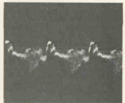
Fig. 3—Using merely the triggered-sweep scope circuitry to obtain what might normally be considered three TV horizontal-sweep traces.
