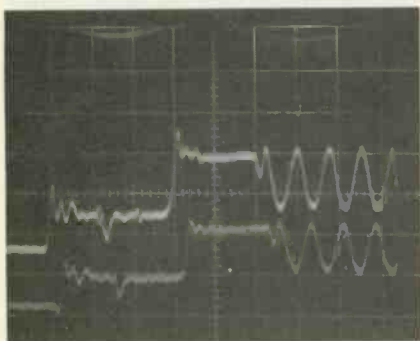
Fig. 17—By noting the apparent phase shift of the 0.5MHz signal as it passes through the color-TV set's delay coil, we are able to determine that there has been a signal delay of approximately 1\mu\text{s} .
