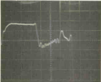
Fig. 11—The 3.58MHz color-burst signal following one of the horizontal blanking pulses can be clearly observed by increasing the scope's horizontal sweep with the "X5 GAIN" switch and using delayed-sweep circuitry.
