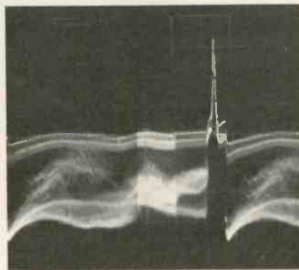
Fig. 7—The brighter portion of this waveform represents the portion of the TV vertical-sweep signal that would be expanded to cover the entire scope screen if we pressed the instrument's "B DEL'D" button.
