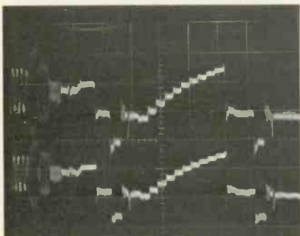
Fig. 16—The test signals before (upper trace) and after (lower trace) they pass through the color-TV set's delay coil. Note the slight phase shift due to the delaying action of the coil.
