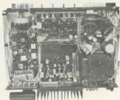
Top view of receiver with digital tuning indicator circuitry removed.
