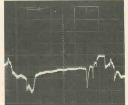
Fig. 9—The single TV horizontal-sweep signal expanded from the TV vertical-sweep signal shown in the previous photograph.
