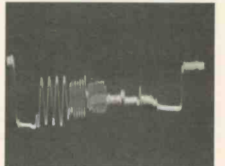
Fig. 15—The scope's delayed-sweep circuitry can also be used to obtain a stable trace of the Vertical Interval Test Signals—another aid for adjusting anything from antenna systems to video amplifiers.
