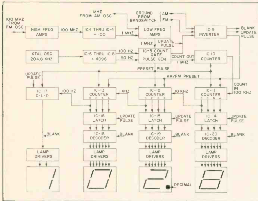
Fig. 3—Block diagram of digital tuning indicator assembly. Courtesy of Magnavox.
