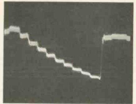
Fig. 14—By using the scope's delayed-sweep circuitry, we are able to obtain a stable trace of the 3.58MHz modulated staircase signal—a helpful service aid for checking gray scale.
