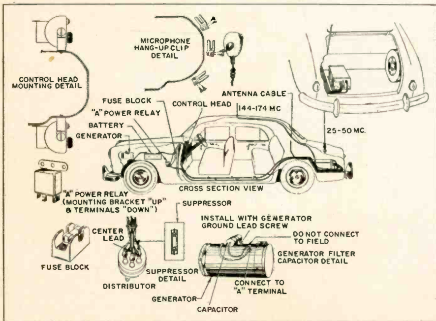
Detail for a trunk-mounted installation of a two-way mobile radio in an automobile.
