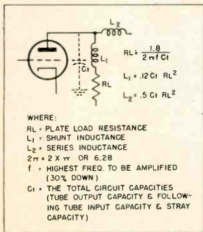
Fig. 2—Formulas for deriving values of load resistors and chokes for wideband stages.
