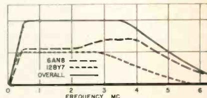
Fig. 4—Response curves for wideband stages.
