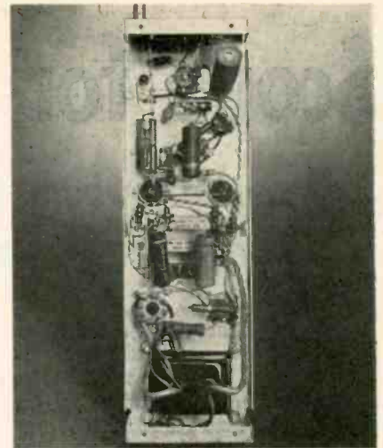
Fig. 6—Underside of the complete amplifier.
