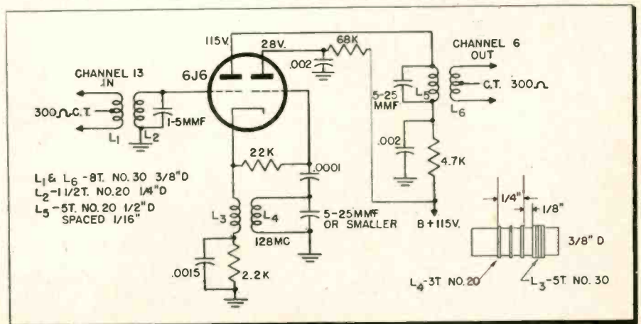
Schematic and coil detail for converter with input on Channel 13, output on Channel 6.
