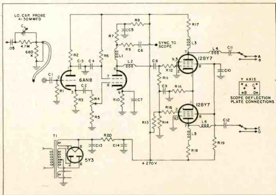
Fig. 1—Complete schematic of the auxiliary scope wideband amplifier; also LCP schematic.
