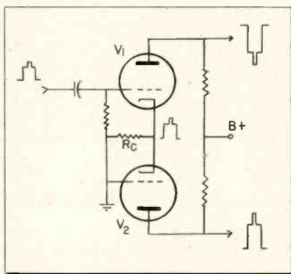
Fig. 3—Cathode-coupled paraphase circuit.
