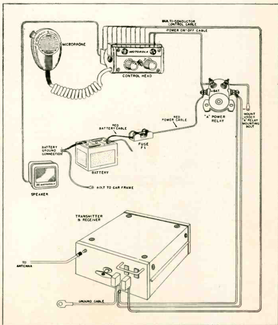
Cabling detail and connections to be made in installing a trunk-mounted mobile radio.
