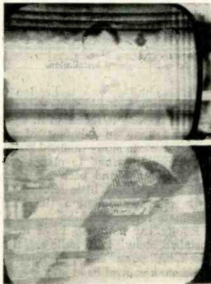
Fig. 2—These effects are produced when the neck of a crt with an open grid is tapped.
