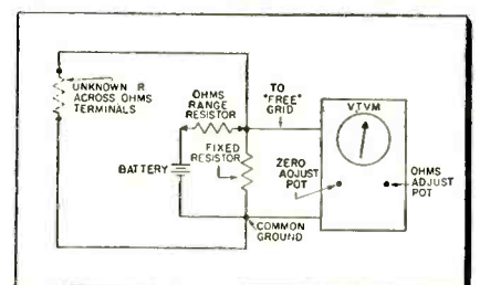
Fig. 6—Typical ohmmeter section of vtvm using battery power supply and bridge circuit.
