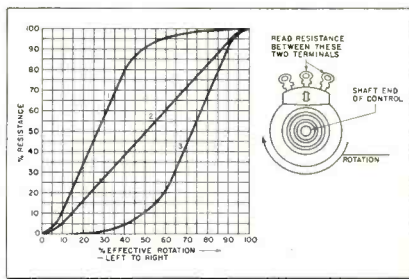
Fig. 1—Typical right- and left-hand taper curves for variable composition resistors
