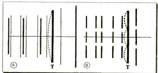
Fig. 2A—Yagi using a tripole, T, as the driven element. Low-band parasitic system is shown by heavy lines, high-band system in light outline. B—High-band operation. Low-band elements are not shown.
