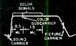
Fig. 1. RF-IF Response
