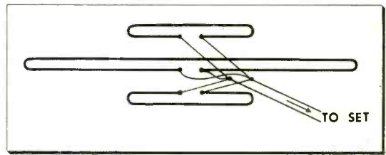
Fig. 1—Physical configuration of the basic broad-band VHF tripole.
