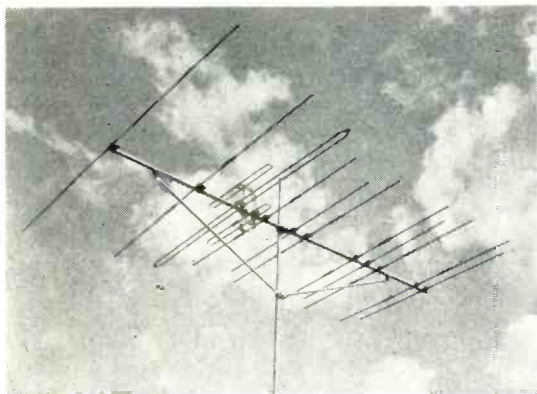
Fig. 3—Commercial example of the tripole-yagi VHF combination.
