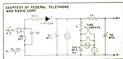
Fig. 1: Power supply of 3-way portable radio
