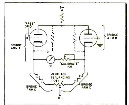
Fig. 5—Bridge with meter in cathode circuit.
