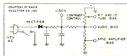
Fig. 3: An independent TV bias supply
