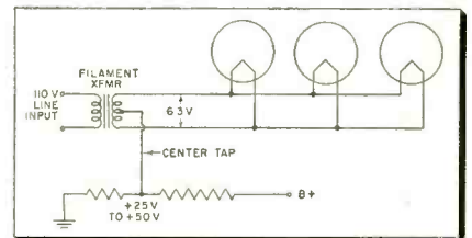
Fig. 2—Biasing the filament line to minimize cathode-to-heater emission in audio amplifier.
