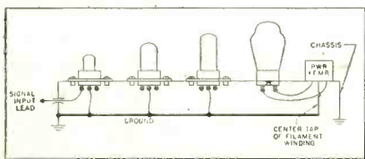
Fig. 1—Connecting filament grounds to chassis in order of tube line-up. "Hot" filament wiring is not indicated in the sketch.
