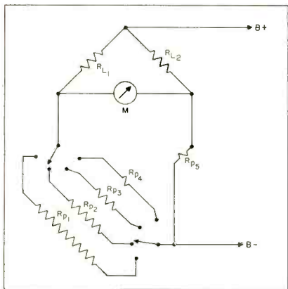
Fig. 3—Elementary bridge circuit. R_{p1} , R_{p2} , R_{p3} and R_{p4} form part of the bridge.
