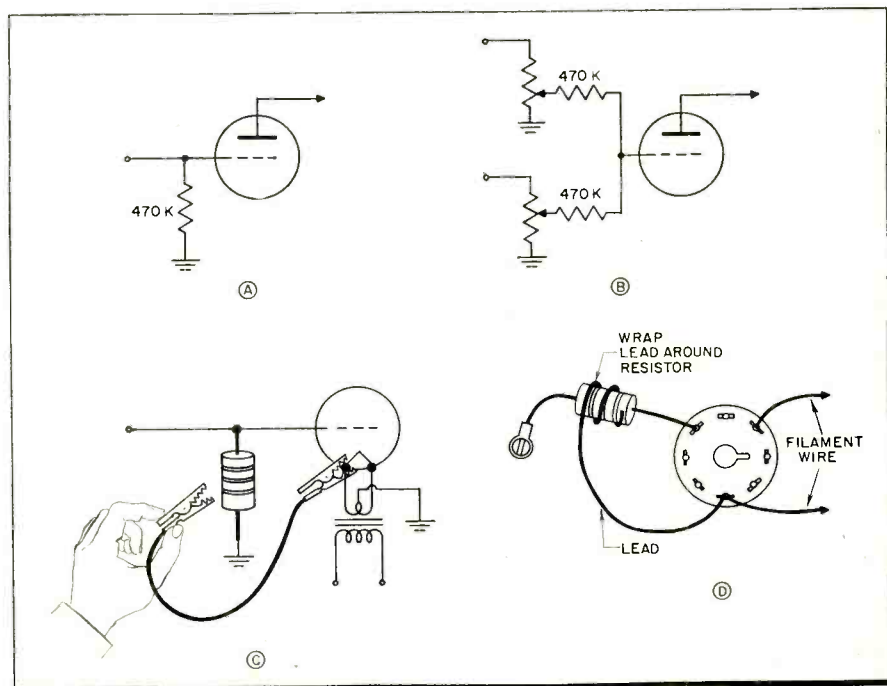
Fig. 3—Hum reduction in circuits (A) and (B) by means of a bucking voltage is illustrated in (C) and (D). Which side of the heater lead to use, other details, are discussed in the text.
