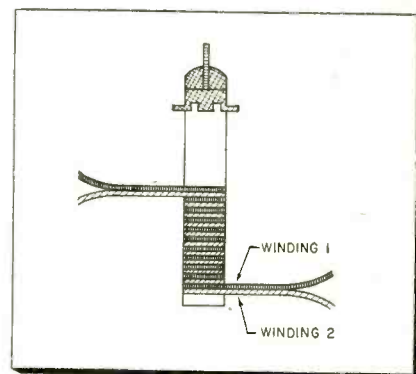
Fig. 3—Bifilar type of i-f transformer. Either winding may be used as primary or secondary. Powdered-iron slug tunes coils.
