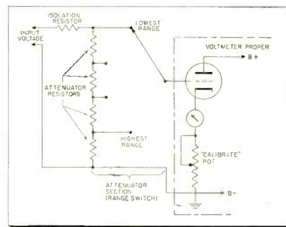
Fig. 2—Adding a range switch and a step attenuator to the vtvm will extend its range.
