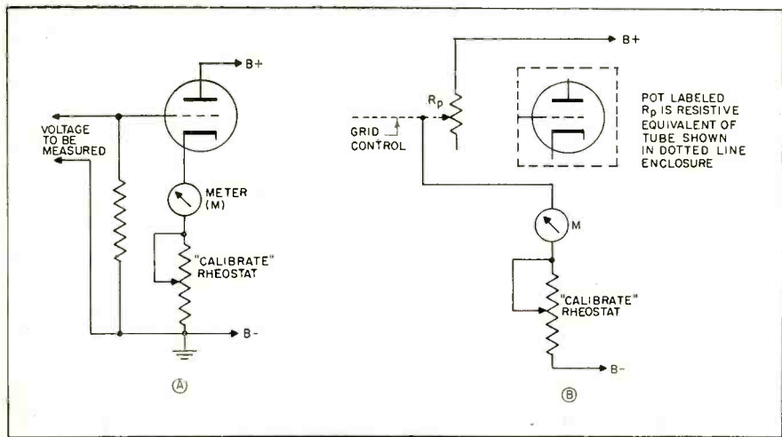
Fig. 1A—One-tube vtvm schematic. B—Equivalent circuit, tube shown as variable resistance.
