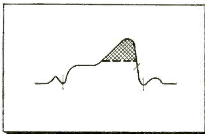
Fig. 2—Peak in response. Signals in the frequency range represented by the shaded area tend to cause spurious oscillation.
