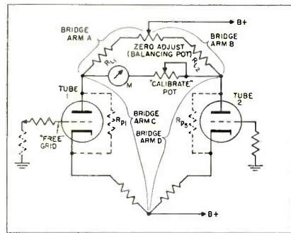
Fig. 4—Bridge circuit of Fig. 3 shown in more detail. R_{p1} and R_{p5} are tube plate resistances.
