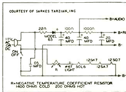
Fig. 2: Selenium use in typical ac-dc receiver
