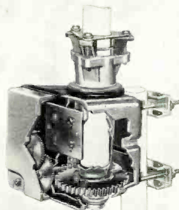
Fig. 13. Cutaway view of a rotator showing the gear train for reducing the speed of the motor to that required for proper operation, which is usually about 2 rpm.
