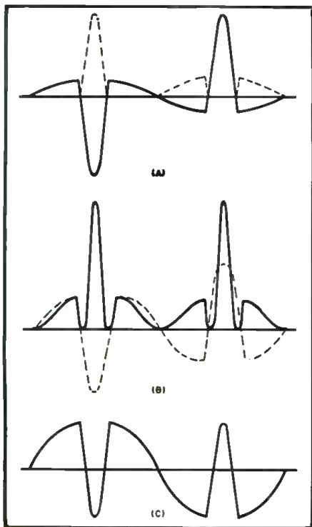
Fig. 4. Comparison of the three methods of metering for balance and harmonic estimation. (A) Using mean reading meter, solid curve shows waveform at input to meter, dotted is rectified portions of wave to give unilateral current. (B) Using r.m.s. instrument, solid curve shows the instantaneous square values, on which reading is based, dotted is the residual input wave to produce the solid curve. (C) Using a peak-to-peak reading instrument. See article.
