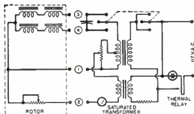
Fig. 6. The complete rotator shown here features a thermal switch for automatically turning on the rotator when the TV set is turned on. The saturated transformer minimizes line fluctuation effects.
