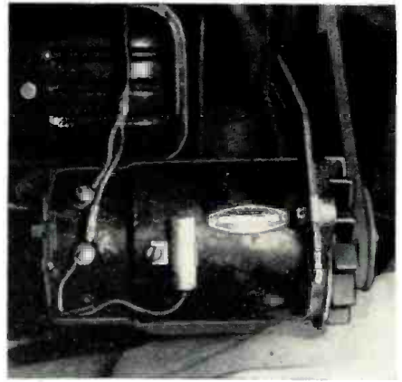
Fig. 3. Bypass capacitor on a generator. The center lead of the capacitor is connected to the armature terminal. The metal body of the capacitor must be grounded.
