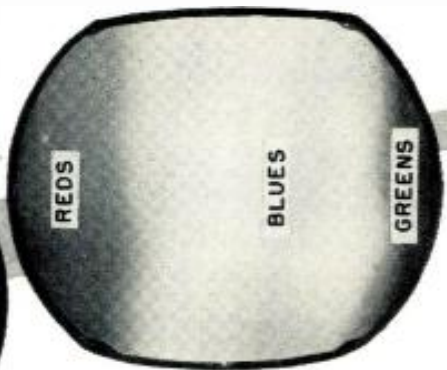
Fig. 3. Typical rainbow display on a color TV tube. The actual display, of course, is in color. Absence of a hue indicates trouble in the associated chrominance channel of the color TV set.
