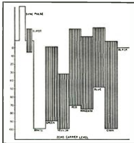
Fig. 5. Composite video signal output of one NTSC color-bar generator. The color tube display resulting from this signal has distinct vertical color bars.
