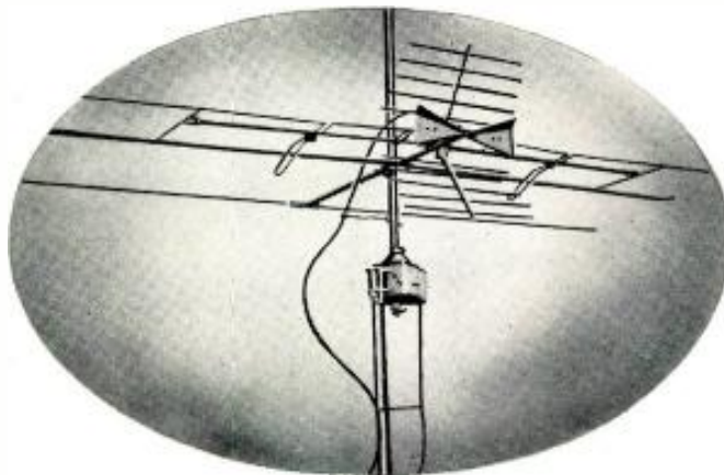
Fig. 1. The rotator shown here is of the offset type. Note that the mast supporting the rotator is not in a line with the mast holding the antenna proper. Note also how the lead-in is secured to masts.
