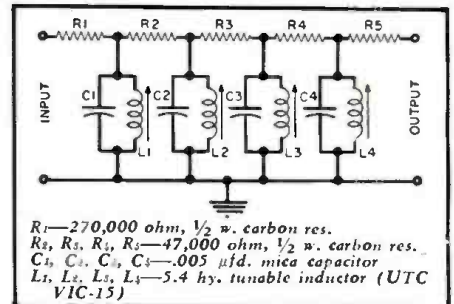
Fig. 1. Circuit of tunable bandpass filter.
