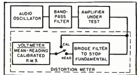
Fig. 1. Block diagram of the usual arrangement for measuring harmonic distortion. The v.t.v.m. in the distortion meter usually reads a rectified mean value, calibrated in r.m.s., assuming a sinusoidal waveform.
