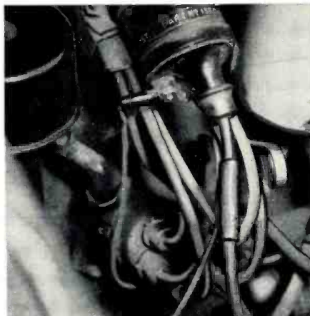
Fig. 2. A suppressor resistor is shown here connected in series with the lead from the ignition coil to the distributor.
