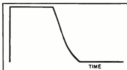
Fig. 2. Output waveform of "Injecto-cal." Note short rise time and sharp leading corner, indicating high harmonic content. This is good for the testing of response.
