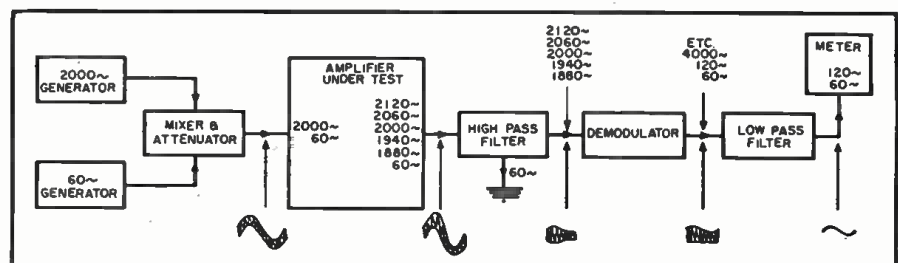
Fig. 2. The more usual method of IM measurement, showing the frequency components present at various points, assuming only first- and second-order products (wave envelopes show first-order only); high-order components will not be adequately measured by this method, for the reason explained in accompanying text material.
