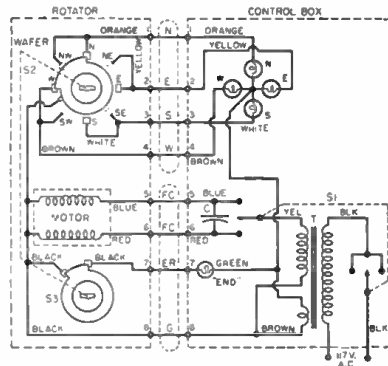
Fig. 9. This rotator uses a wafer switch ganged to the gear train of the motor. One switch section operates a pilot light which indicates the end of rotation; the other section indicates the direction.
