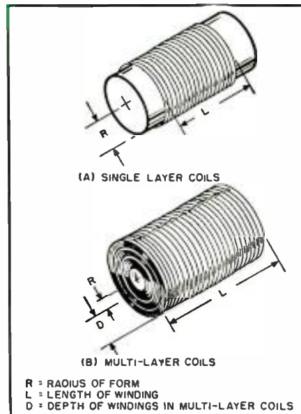
Fig. 1. Single- and multi-layer coil data.
