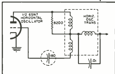
Fig. 2. Lack of horizontal sweep on a 16" RCA set was due to a defective capacitor (shown circled) in the horizontal oscillator circuit. The replacement went bad too.
