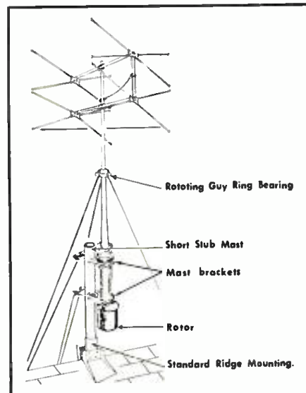
Fig. 10. Rotator and antenna installation in which the antenna mast is longer than 6 feet. Here the upper mast should be guyed using a ball-bearing guy ring.
