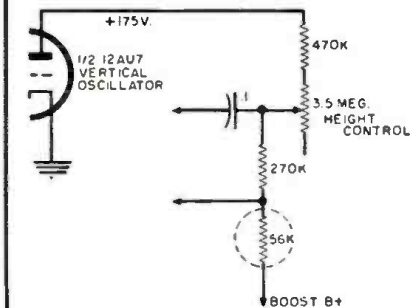
Fig. 1. The 56,000 ohm resistor shown circled in this vertical oscillator circuit of an RCA 21" receiver was bad and had to be replaced to obtain vertical stability.
