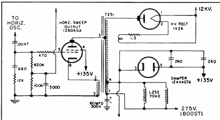
Fig. 5. The horizontal deflection coils of this G-E series "M" TV chassis are in parallel, eliminating the need for a balancing capacitor, however, more yoke current is required. Note the absence of width, linearity, and horizontal drive controls.
