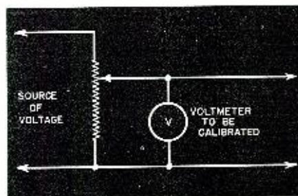
Fig. 3. Circuit for voltmeter calibration.
