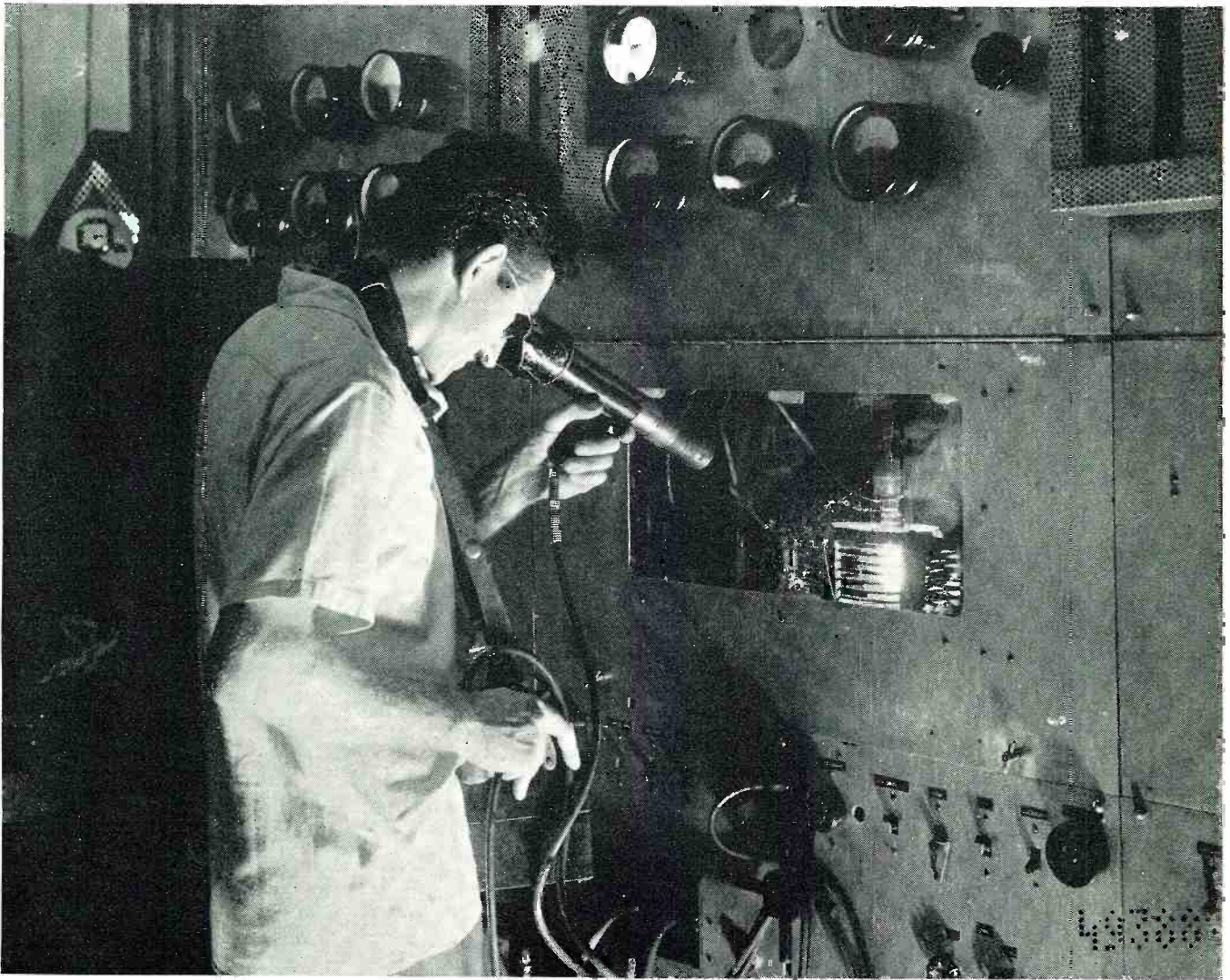
Operator is making an optical pyrometer test to obtain temperature of tube anode.
