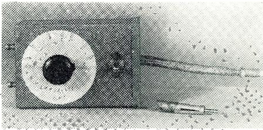
The alignment unit is built into a metal shield can measuring 5x3½x2½". Dial is cut from cardboard.
