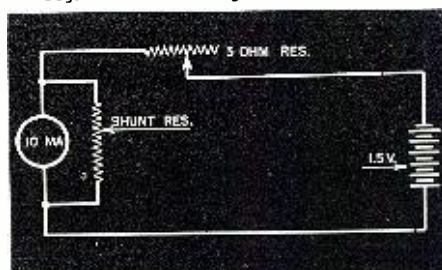
Fig. 2. Determining shunt resistance.
