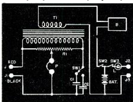
Wiring diagram of the capacity bridge.
