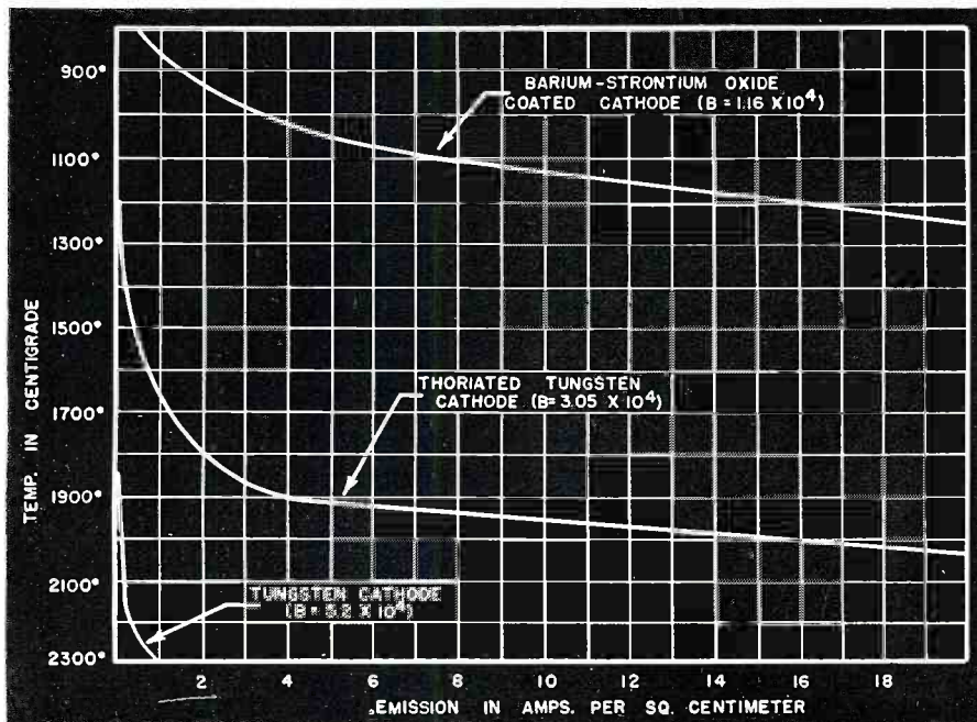
Fig. 1. Graph of Richardson's equation (See text).
