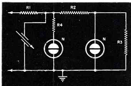
Fig. 4. Neon lamps indicate peak voltages.
