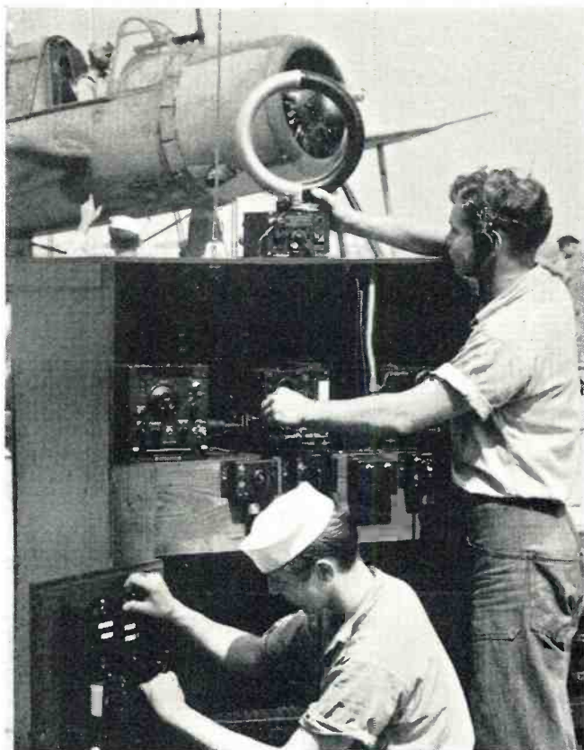
Learning the intricate parts of the direction-finder and communications sets that are used in Navy planes.
