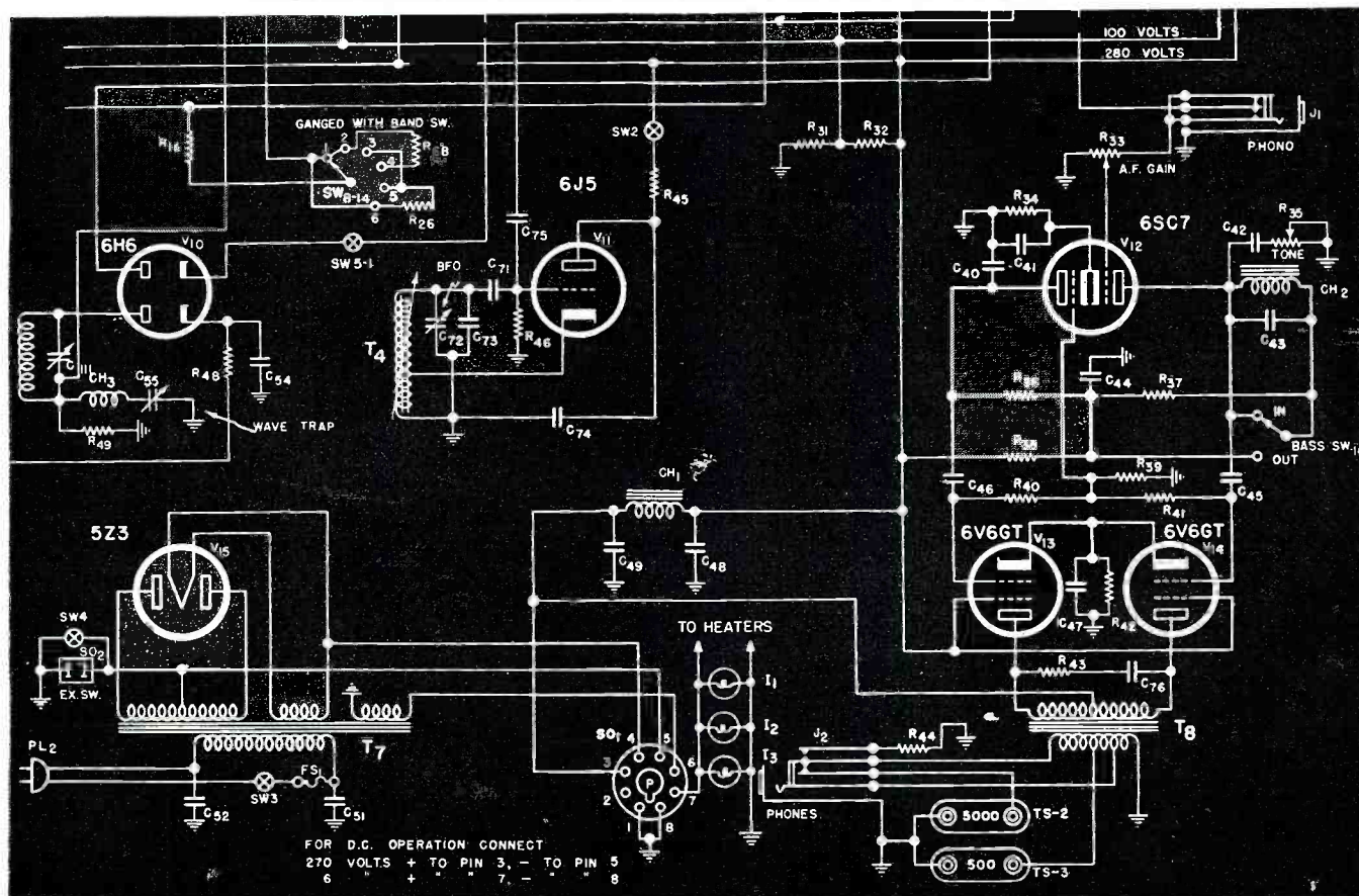
Partial schematic of SX-28 shows audio end of the set. The tonal range is fully adjustable.
