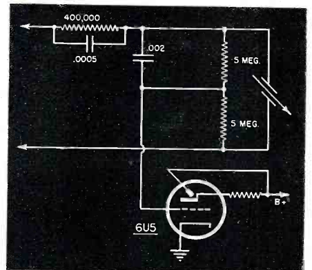
Fig. 3. Simple tuning-eye monitor.
