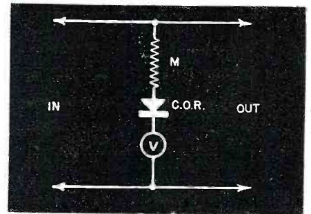
Fig. 2. Connections for db meter.
