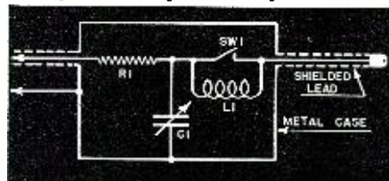
Diagram of the portable alignment unit.
