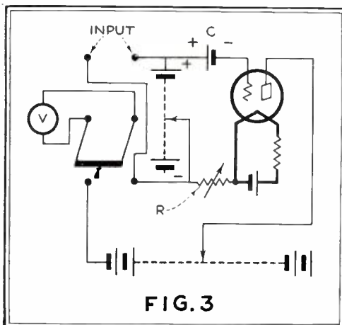
Fig. 3. A method of applying two known voltages across the input to obtain direct calibration is shown at the left
