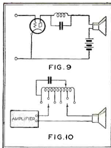
Tuned trap circuit in the output, to correct speaker deficiencies. Fig. 9 shows a single stage filter, with fixed tuning, and Fig. 10 is a variable tuning circuit
