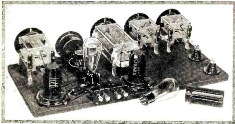
Back view of the transmitter. All the parts will fit on the baseboard easily, if this layout is followed
