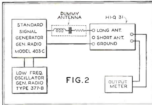
Fig. 2. Laboratory set-up for making overall measurements. The standard signal generator supplies a small known modulated r. f. voltage to the antenna system, the r. f. oscillation being modulated by a voltage from the low frequency oscillator. The power output, measured by the output meter, is maintained constant at 50 milliwatts
