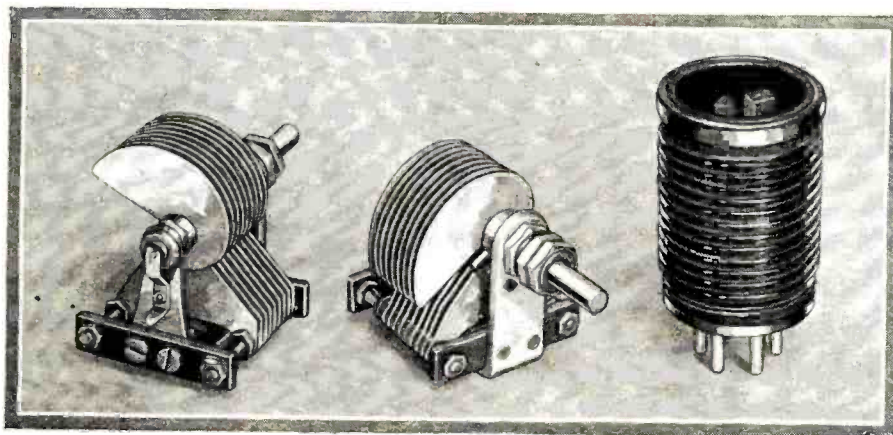
A front and rear view of condenser and the new S.-W. coil form
