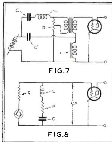
Fig. 7. Compensated input circuit, for correcting pick-up deficiencies, and the equivalent electrical circuit is shown in Fig. 8
