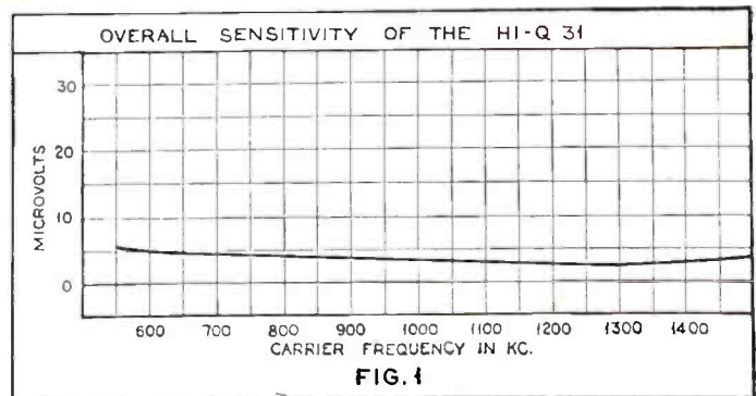
Fig. 1. Overall sensitivity characteristic. The average sensitivity is approximately one micro-volt per meter
