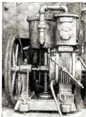
The small compressor. Future experiments will probably reduce the necessary size of the compressor materially
