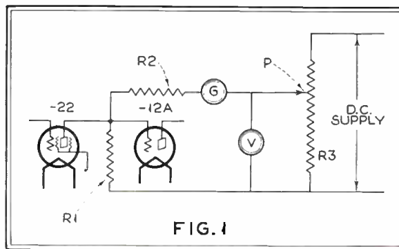
Fig. 1. A special circuit for measurements between 5 and 50 volts, when no current is to be drawn from the device being tested
