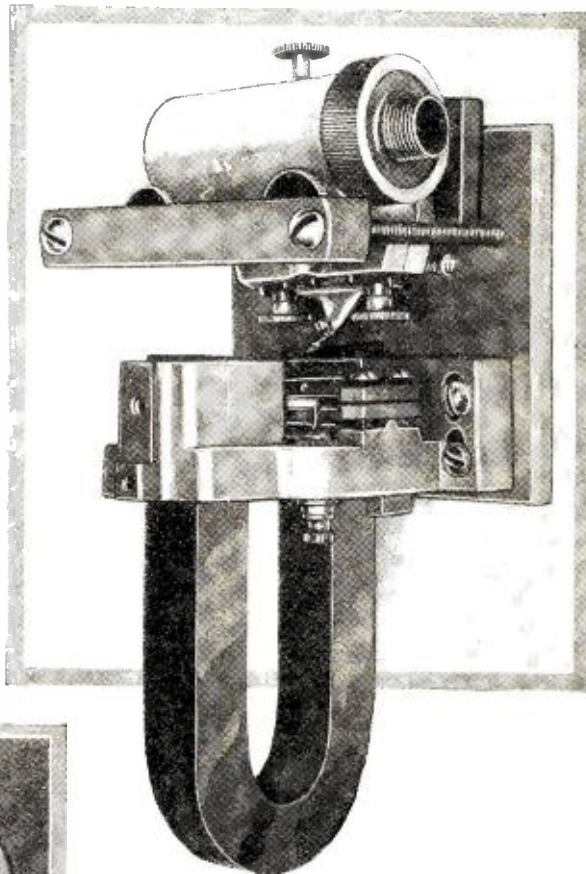
The complete sound head assembled. The motor in this instance is the familiar loud speaker unit, operating the air valve
