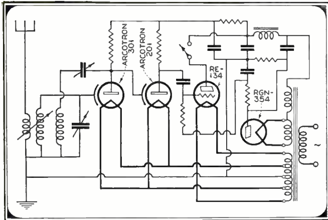
A typical German receiver circuit—the Telefunken—Hab—Aristron. This receiver employs the Arcotron tubes in the first and second sockets
