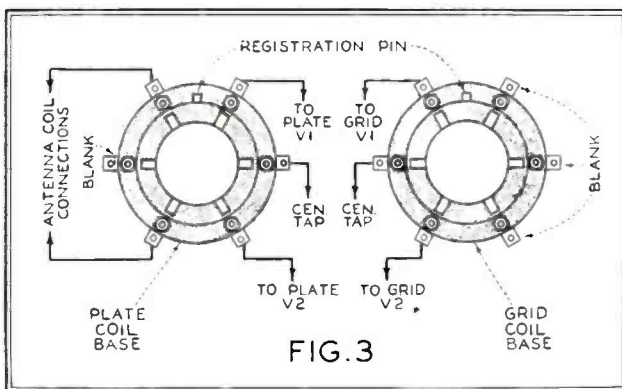
How to wire to the coil bases. This should be carefully noted, for a mistake here will prevent the transmitter from "perking"
