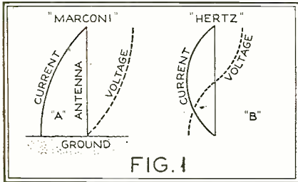
Figs. 1 to 5, inclusive, show diagrammatically the function of Marconi and Hertz antennas and also half wave, full wave, current feed and voltage feed antennas
