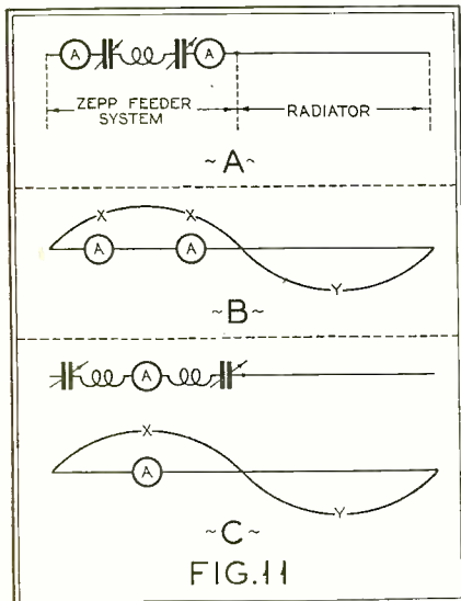
Fig. 11. "A" shows the Hertz (Zepp-fed) antenna straightened out; "B" the distribution of current in the feeders and radiator; "C" the same if it were possible to place a current meter in the electrical center of the feeder circuit
