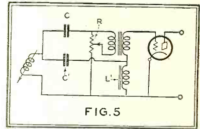
Fig. 5. Another means of high-frequency compensation for use in the pick-up circuit
