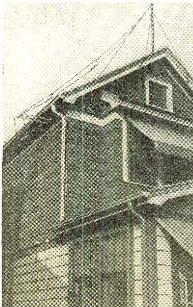
Fig. 10. In this current feed system note that the feeder is off center of the radiator portion of the antenna system. At the right is a Zepp antenna. Glass towel rods are used as spreaders
