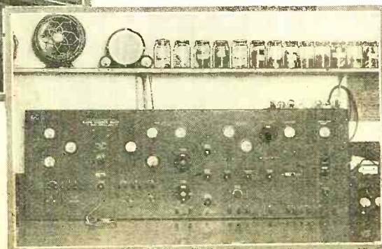
Willard W. Geiger, of Mt. Pocono, Pa., built the interesting test panel pictured above. The left hand panel contains a modulated oscillator, a vacuum tube voltmeter, a grid-dip meter and a wavemeter. Magnetic and dynamic speakers are located above middle panel. Tube sockets are at right
