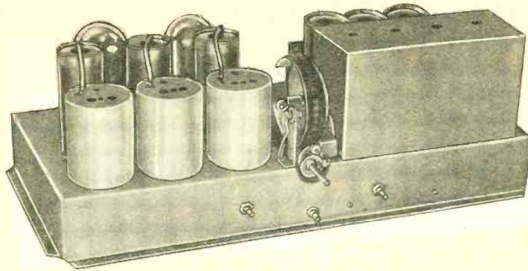
A front view of the "36" superheterodyne
