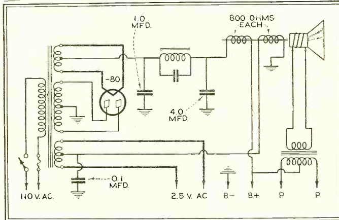
Fig. 5. The speaker windings are an enclosed part of the power supply circuit of the "36"
