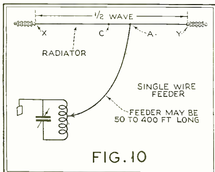
Fig. 10. In this current feed system note that the feeder is off center of the radiator portion of the antenna system. At the right is a Zepp antenna. Glass towel rods are used as spreaders
