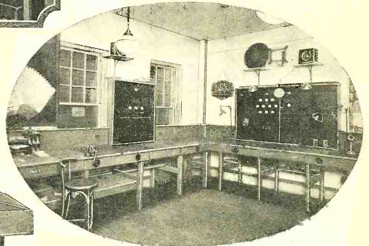
Radio Studios, Inc., New Rochelle, N. Y., submitted the photo shown above. The main test panel includes a complete set and tube tester, a high and low-resistance bridge, a 175 and 180 kc. oscillator. The small panel includes a continuity test, a milliammeter and a voltmeter connected to pin jacks. Both boards are wired with battery set voltages
