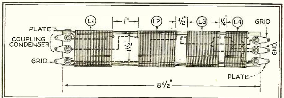
Complete coil assembly for first detector oscillator circuit. The specified spacing between coils should be carefully followed
