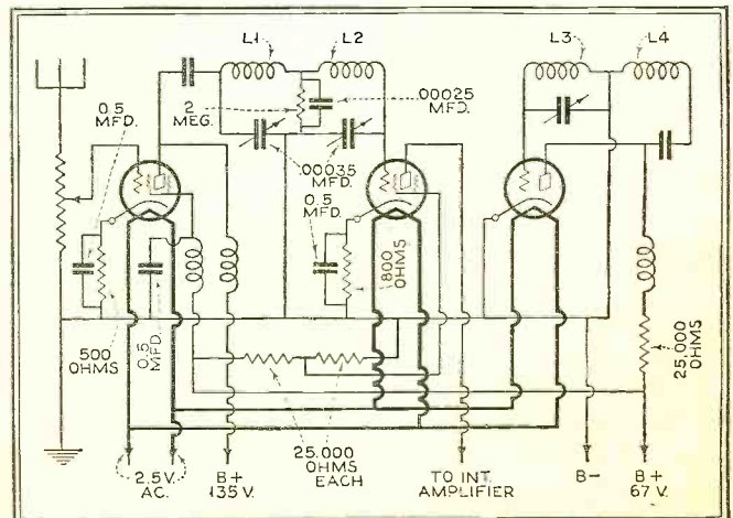
The circuit diagram of the oscillator and first detector
