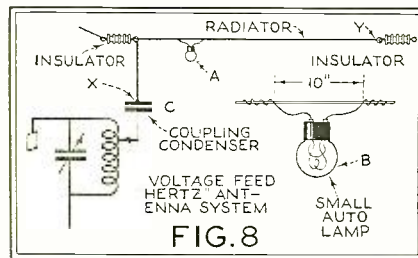
Figs. 6 to 8, inclusive, give some idea of the general construction details which enter into the erection of a suitable transmitting antenna
