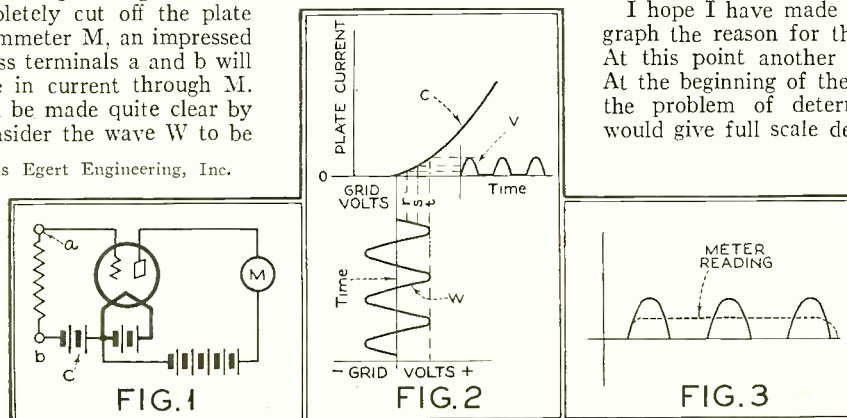
A simple tube circuit, with bucking battery to cancel out the normal plate current
