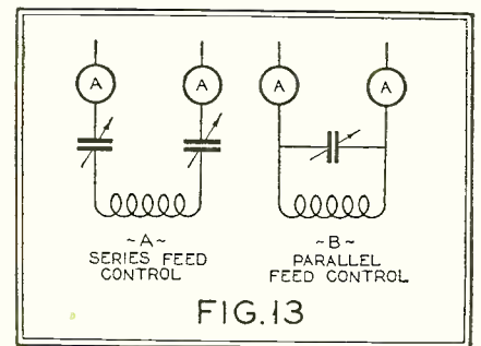
Fig. 13. Condensers arranged either in series or parallel in the feeder line provides for multiple frequency operation
