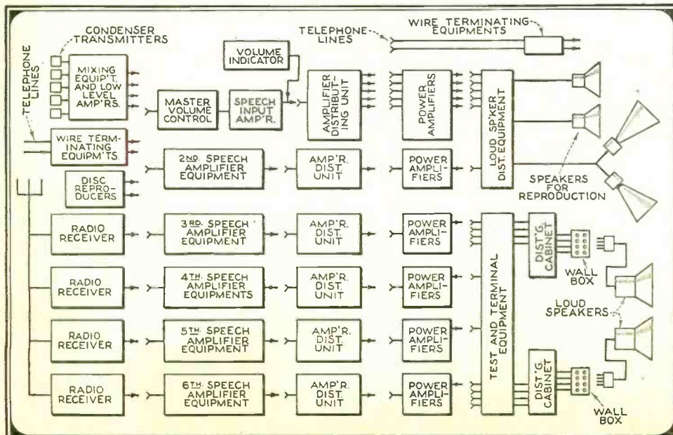
A diagrammatic presentation of the circuit arrangement employed in the speech amplifier system of the Waldorf Astoria
