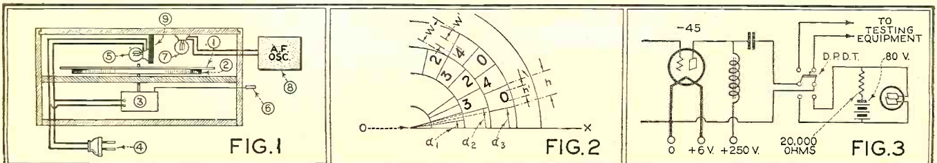
Fig. 1 shows the layout of the turntable and neon lamps. Fig. 2 shows how the radial lines are laid down on the disc, while Fig. 3 indicates the biasing circuit employed in the "flasher" neon tube circuit
