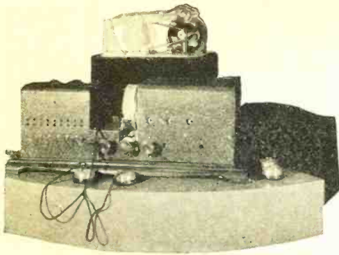
(Left) This machine jolts a vacuum tube eight hundred times a minute, but the tube still works. The tube is hooked up as a part of the circuit in the receiver below it
