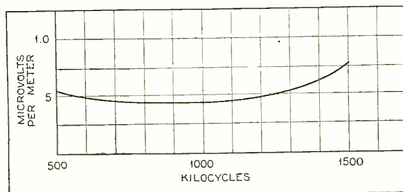
Fig. 2. The sensitivity curve for the SM-36 superheterodyne receiver shows that the maximum to minimum rate gain is less than 2 to 1. The average sensitivity is approximately 1/2 microvolt per meter
