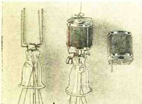
At the left, reading from left to right, are three stages of mount assembly: Four pillars sealed into glass stem, tube elements welded to four pillars, and complete assembly of tube elements
