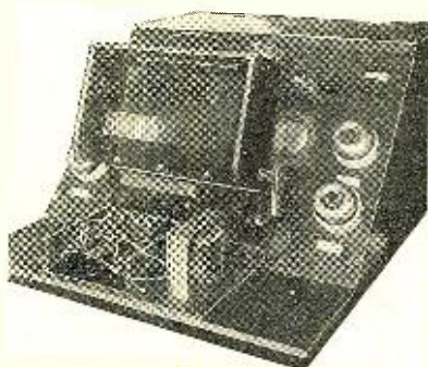
(At top) The laboratory standard oscillator by which testing units are calibrated daily. (Above) Inductance, shorted turns and "Hipot" tests on chokes and transformers
