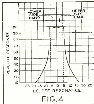
Fig. 4. Band-pass circuits, properly coupled together, eliminate side-band cutting and at the same time improve the selectivity due to the straight sides of the curve. Compare this characteristic with Fig. 3
