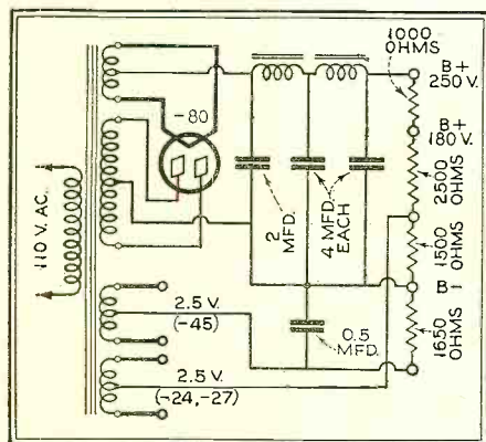
The circuit employed in the power supply unit for the "Conqueror" a.c. short-wave receiver
