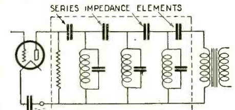
Schematic diagram of an I.F. band-pass filter, preceding the second detector of a super-heterodyne.
