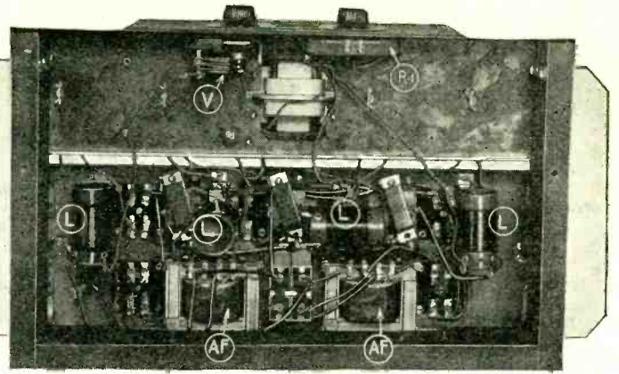
Under side of the chassis, showing the arrangement of the various R.F. and A.F. components: V, "vernier" condenser; R1, rheostat for the R.F. tubes; L, R.F. transformers; AF, A.F. transformers.
