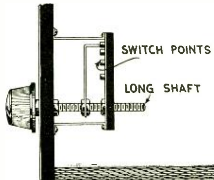
By mounting inductance taps as shown in the sketch the appearance of the panel is bettered.
