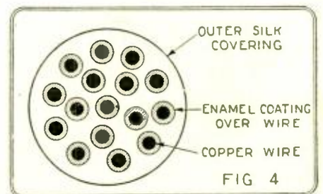
An enlarged cross-section view of Litzendraht wire. The outer silk covering holds the thin wires together, so that they may be handled as a single cable.
