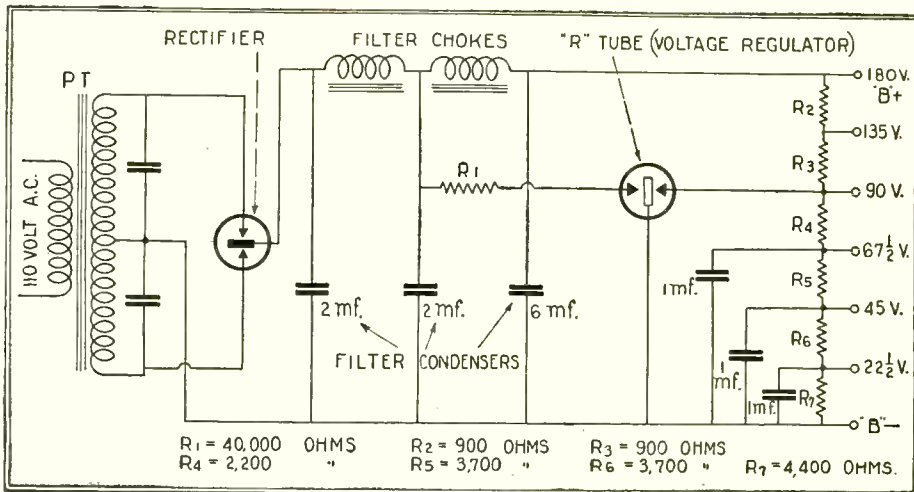
Fig. 4. The circuit diagram of a "B" power unit which uses a double-wave rectifier and a voltage regulator.
