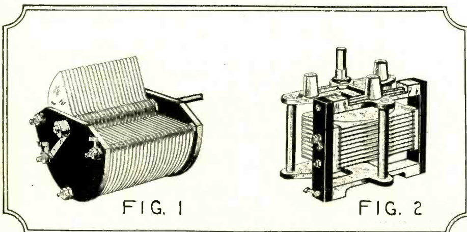
Fig. 1. An old-style variable condenser with the rotor and stator insulated from each other by large end-plates of non-conducting material.
