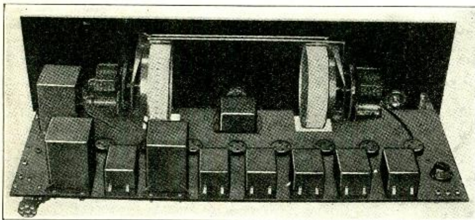
Rear view of the nine-tube superheterodyne. The various radio and audio-frequency transformers and oscillator coils are aligned evenly along the back edge of the sub-panel. The two white cylinders are the indicating scales of the condenser-control drums. Illustrations courtesy High Frequency Laboratories
