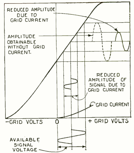
Fig. 5B. This diagram illustrates how a tube amplifies less when the grid is positive, because of the grid current.
