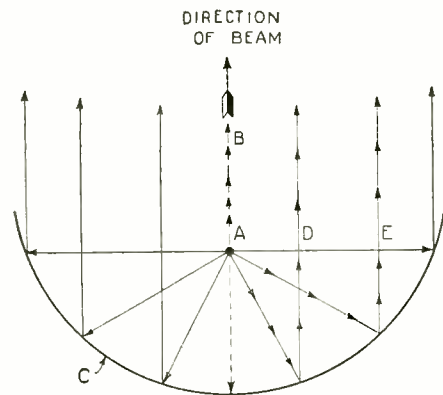
FIG 3 A is the focus of the reflector, C. The waves starting at A are reflected parallel to A-B, as indicated at D and E, thus being concentrated into a narrow beam.
