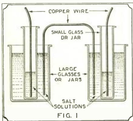
The arrangement of the jars forming the condensers, in series with each other, and in parallel with the main tuning condenser of the set.
