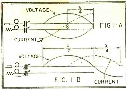
How the standing waves take their positions on Lecher wires; showing the voltage and current crests and nodes.
