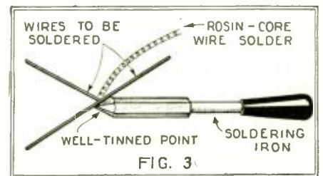
Fig. 3 shows the correct position of a soldering iron and solder, in relation to the wires being soldered.
