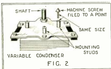
By using a machine-screw with a pointed head, the mounting holes can be easily located on a panel.
