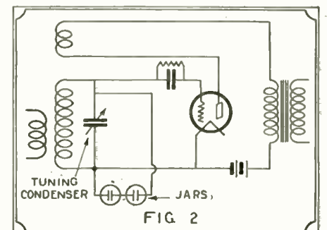
The circuit diagram, showing how the jar condensers are connected to the set. As their capacity is increased by pouring in liquid, the wavelength to which the receiver is tuned increases.
