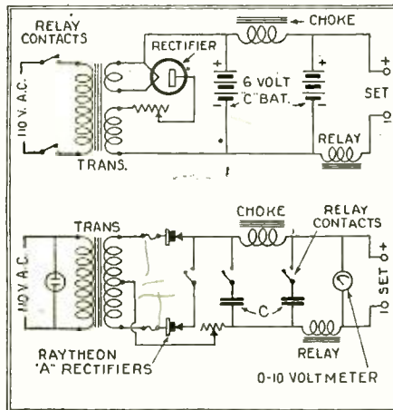
Fig. 1 (top): An early type of "A" power supply, using two batteries floating across a rectifier line. Fig. 3 (bottom) hook-up of the new "A" unit described in the accompanying article.
