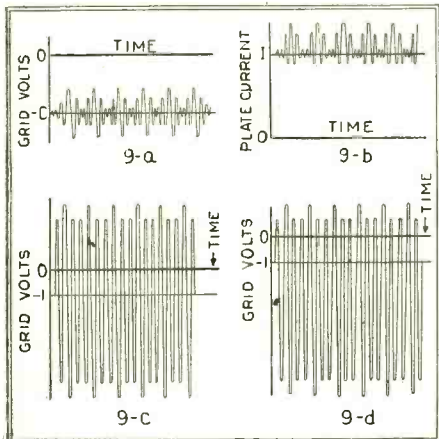
These four sets of waves illustrate the theory of the Strobodine, in its relation to the superheterodyne.
