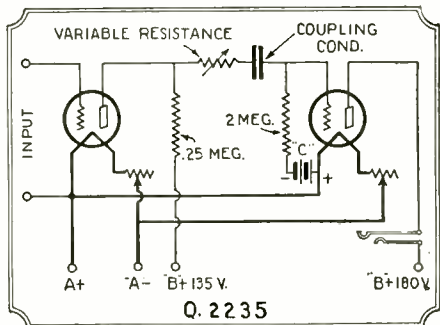
A variable resistor, of 0-500,000 ohms, in series with the coupling condenser and plate, makes a good volume control.
