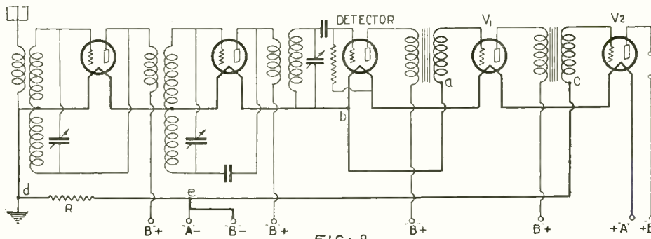
FIG. 8 When a receiver has tubes whose filaments are connected in series, negative grid voltages can be obtained easily by taking advantage of the IR drop in the filaments of the tubes, as shown above.
