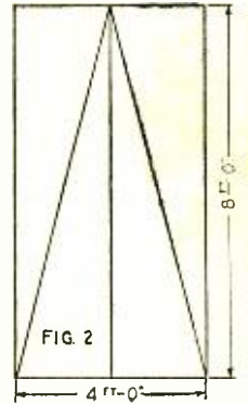
Fig. 2 shows how the wall board is cut, the four pieces necessary being taken from the same sheet. Fig. 3 illustrates the method of making the corners of the square horn airtight.
