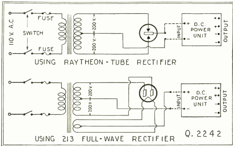
Schematic diagrams of a "B" socket-power unit, for use on 110-volt A. C., and made to utilize apparatus in a D. C. unit.
