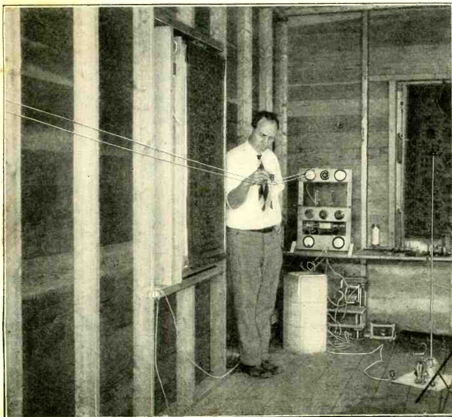
The author demonstrating the method of determining the wavelength, on which a transmitter is operating, by means of the Lecher wires and an ammeter. The transmitter and power equipment may be seen in the background.
