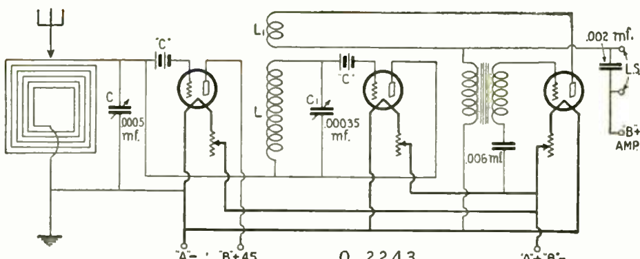
The schematic diagram of the Retrosomic three-tube receiver, with which a loop in combination with an aerial is employed.
