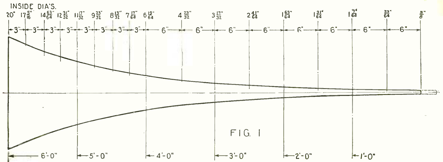
Above are shown the widths of the six-foot exponential loud-speaker horn at suitable short intervals along its length. The material necessary for making one of these horns can be obtained from a single sheet of wall board. The pattern, which is shown in Fig. 1, is prepared and laid upon the wall board; and the latter is cut along the lines indicated, allowing on one side an extra lap equal to the thickness.
