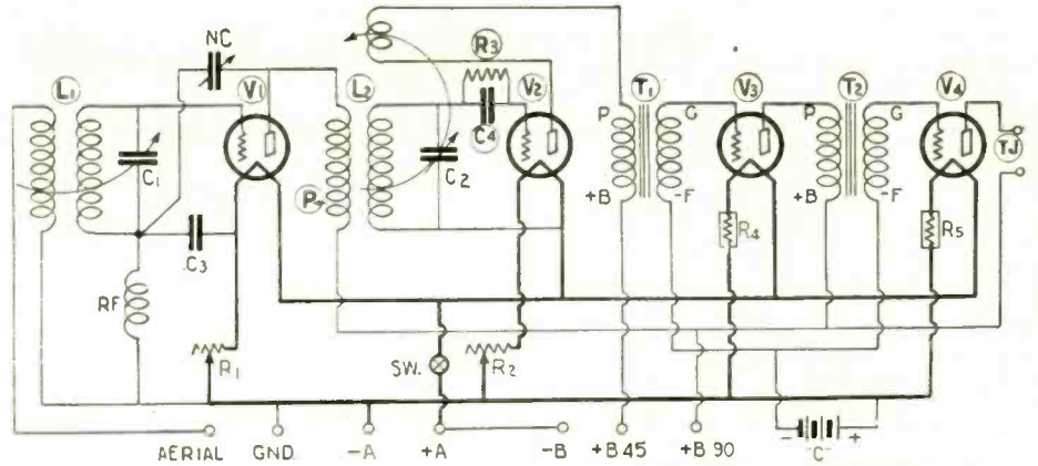
The parts in the above schematic diagram of the Knickerbocker Four are numbered, as are those in the other illustrations.
