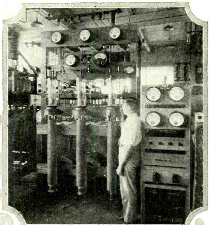
For the first time in the history of radio broadcasting a power of 100 kw. was modulated and put into the antenna, at midnight on August 4 in the transmitting laboratories of the General Electric Company at South Schenectady, N. Y. Five of the 100-kw. transmitting tubes, described in the June, 1927, issue of RADIO NEWS, are used in this powerful transmitter, which occupies less than half the space needed for the 50-kw. set. Two of these giant tubes are used in the amplifier and three are required for the modulator. The former two, with a "spare" beside them, are shown above.
