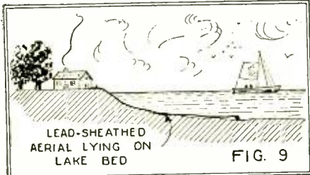
Naval tests have shown the efficiency of an aerial submerged in the water, as shown. The end, of course, is insulated.
