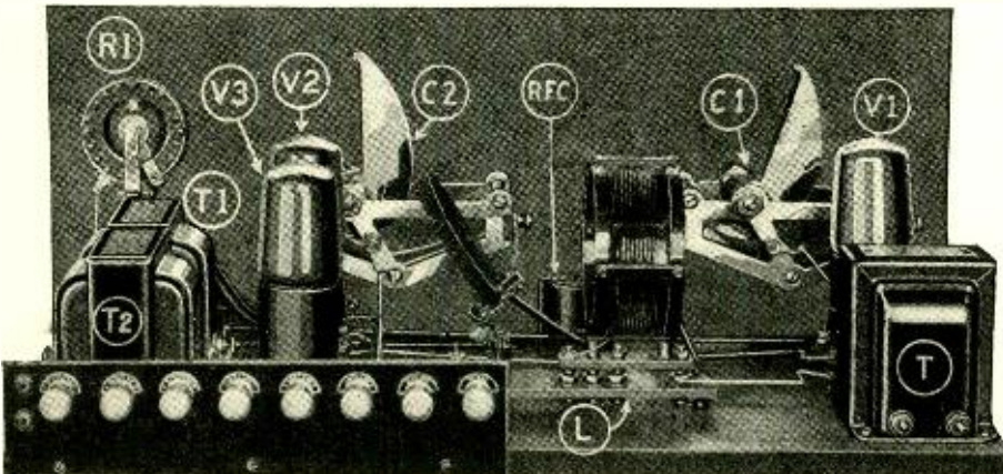
One of the plug-in inductances is here shown placed in its mounting. The various parts are marked with the same symbols as they bear in the wiring diagram.
