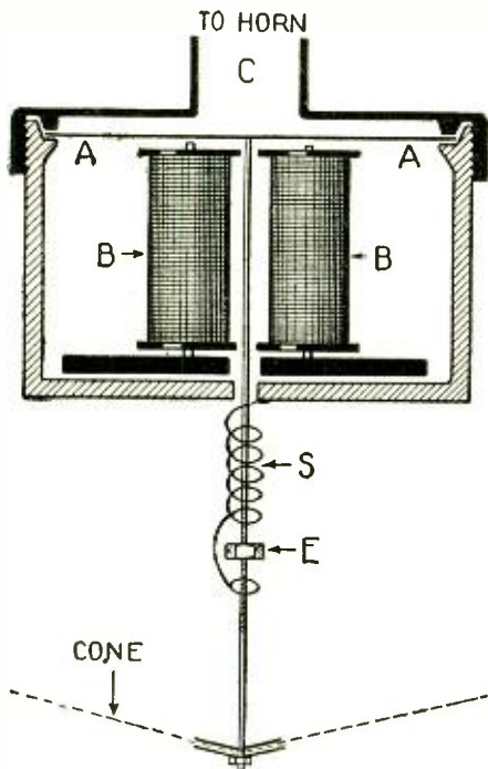
The author's ingenious plan for operating both cone and horn from one unit. The cone drive-rod must be balanced by a spring to compensate for the whole weight upon it.
