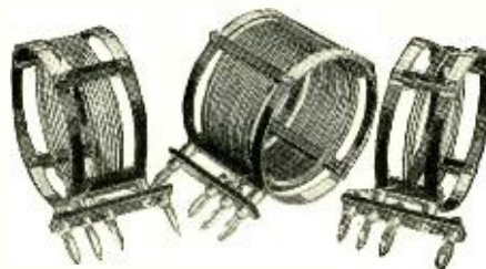
The three plug-in coils which are employed to make the receiver cover a wavelength range from 15 meters up to 130.
