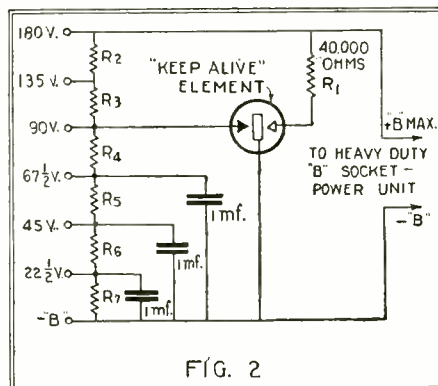
FIG. 2 Schematic diagram showing how the tube is connected in a socket-power-unit circuit. See Fig. 4 (page 346) for values of the resistors required.
