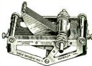
2 Karas Orthometric Extended Shaft .00037 mfd. Variable Condensers are used in the KNICKERBOCKER 4. Price, each, $6.75.
