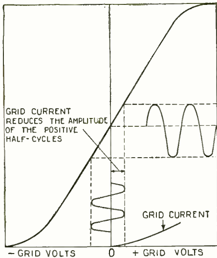
Fig. 5A. Showing how the upper halves of the cycles are smaller in amplitude than the lower halves; this is due to the grid current's damping half of the signals applied to the grid.
