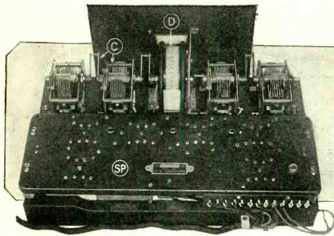
Rear view of the receiver chassis: D, scale of the drum control; C, four-gang condenser controlled by the drum; SP, the metal sub-panel on which the tubes are mounted.
