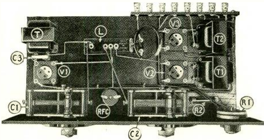
Top view of the RADIO NEWS Special Short-Wave Receiver. C1, tuning condenser; C2, regeneration control; L, plug-in coil base; T, grid choke; C3, grid condenser; R.F.C., R.F. choke; T1, T2, A.F. transformers; R1, R2, filament resistors; V1, V2, V3, tube sockets.
