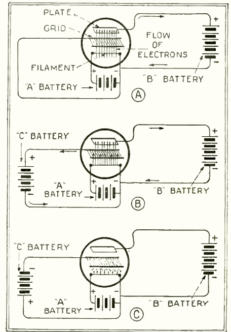
Fig. 1. At A we have the filament-plate flow of electrons in a vacuum tube. When the grid is made positive (B), more current flows between the filament and the plate; while less or even none can pass through the tube as the grid is made negative (C).
