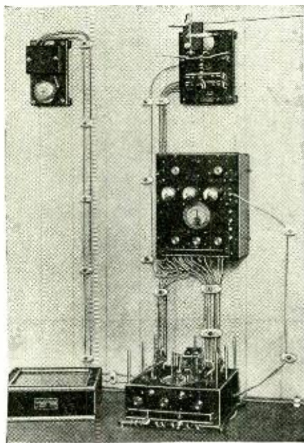
This radio receiver automatically sets off the alarm gong whenever an "SOS" on 600 meters is received, thus making it unnecessary to keep an operator listening in. This type is being installed on many British ships.
