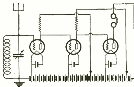
A unique system of coupling, wherein the plate of each tube and the grid of the next are at the same potential.
