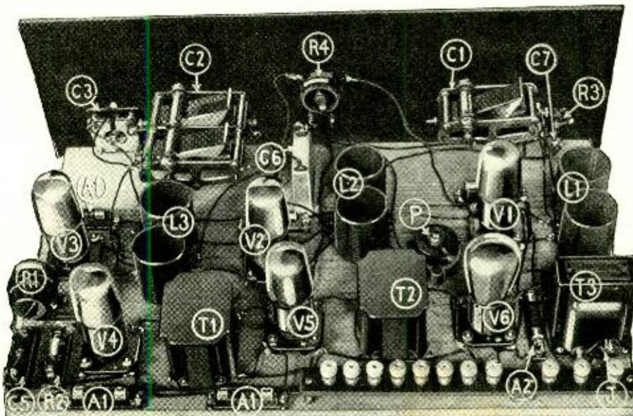
The midjet condenser C5 is out of the view in this illustration, being behind the resistor R1. That lettered C5 is really C4, as the diagram will show. The two condensers are alike. The second binding post from the right is not used, and is not shown in the working drawing.
