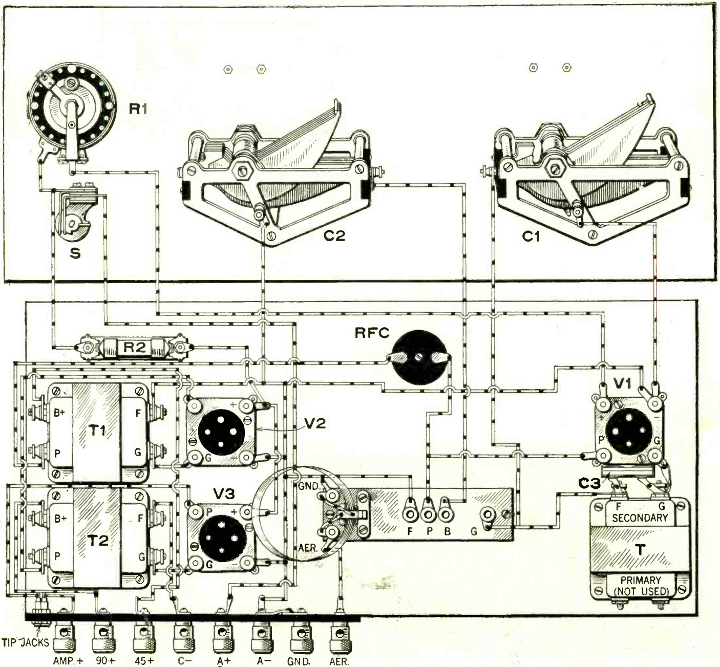
The wiring diagram shows exactly how each connection should be made. This is most important in a short-wave set; as frequencies much higher than those in the broadcast band are encountered.
