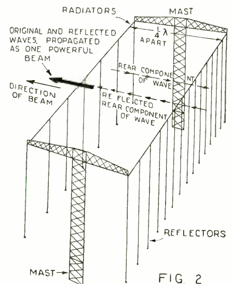
FIG 2 How the antenna system of a beam transmitter functions may be seen above.
