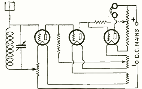
The same system using a socket-power D. C. unit. The simplicity is apparent.
