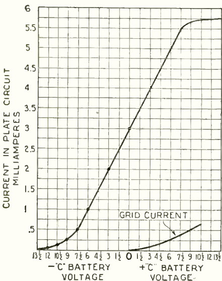
Fig. 3. A typical "characteristic curve" of a vacuum tube, made by using the hook-up in Fig. 2.
