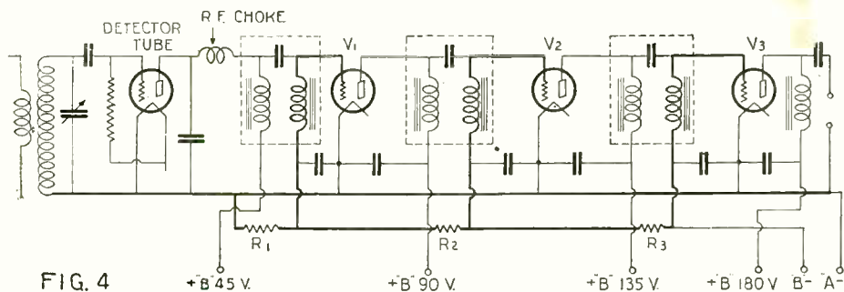
FIG. 4 When resistances, such as R1, R2 and R3, are introduced into an amplifier circuit, negative grid voltages of different values may be easily obtained.
