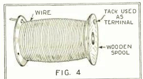
An easy method for making R. F. choke coils is to bunch-wind No. 36 wire on an ordinary spool.
