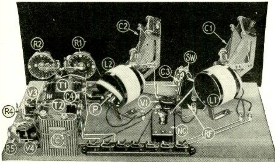
C1, C2, variable condensers; R1, R2, rheostats; L1, antenna coupler; L2, 3-circuit coil; C3, fixed condenser; C4, grid condenser; RF, R.F. choke coil; T1, T2, A.F. transformers; R4, R5, 4-ohm resistors; N.C., neutralizing condenser.
