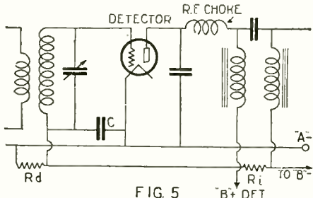
FIG. 5 In the above schematic diagram is shown a method whereby a negative grid bias can be put on the detector tube.
