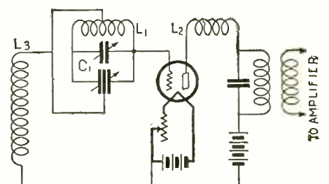
Fig. 7. The Strobodine circuit, which is the heart of the Strobodine receiver.
