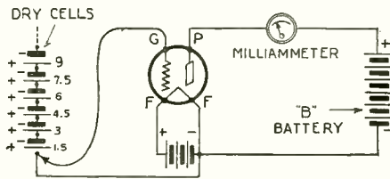
Fig. 2. The circuit that is employed for ascertaining the "characteristic curve" of a vacuum tube, such as shown in Fig. 3.
