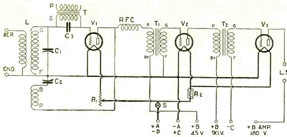
The schematic diagram of the RADIO NEWS Short-Wave Receiver. This set has a regenerative detector and two stages of transformer-coupled A.F. amplification.
