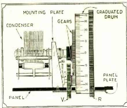
Left: How the drum control looks from the top of the panel; V, vernier-adjustment wheel; R, knurled rim of drum, permitting quick adjustment to approximate position; S, spring, holding gears tightly in mesh.
