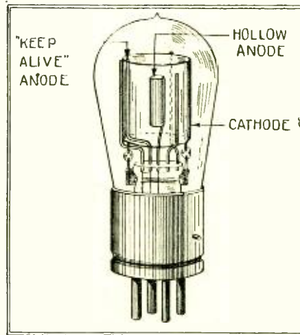
Fig. 3. A phantom view of the new tube, showing the respective positions of the three elements.
