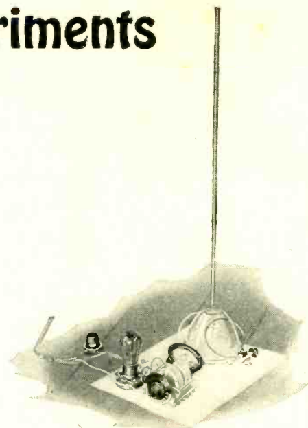
The 5-meter set, using a double condenser. (For diagram see Fig. 3.) A 5-meter wave-meter may be seen, leaning against the glass insulator.
