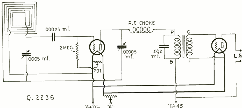
The schematic diagram of a two-tube portable receiver, which may be operated from a loop antenna, is shown above and should give satisfactory reception.
