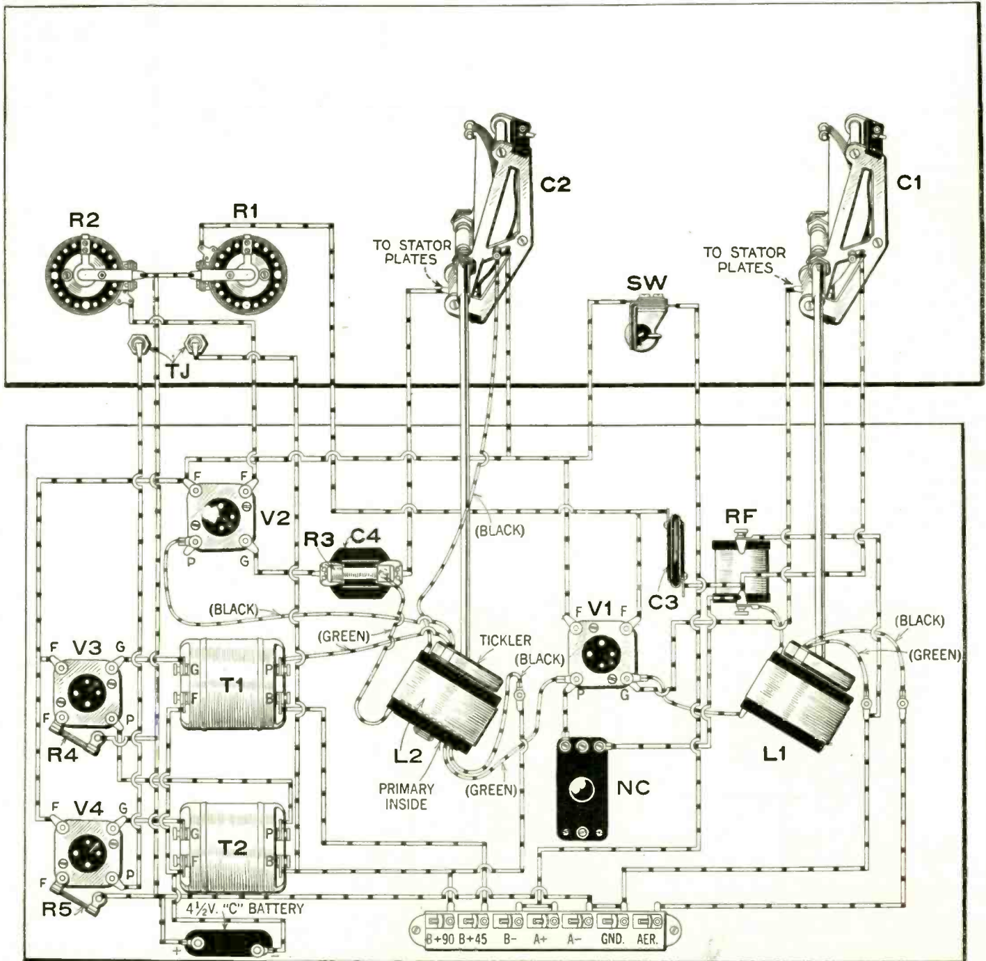
The wiring diagram of the Knickerbocker Four receiver. The diagram can be easily followed if each connection in the illustration is blacked out with a pencil after the corresponding wire has been soldered in the set. This corresponds in all details with the schematic diagram above, with which it may be compared.
