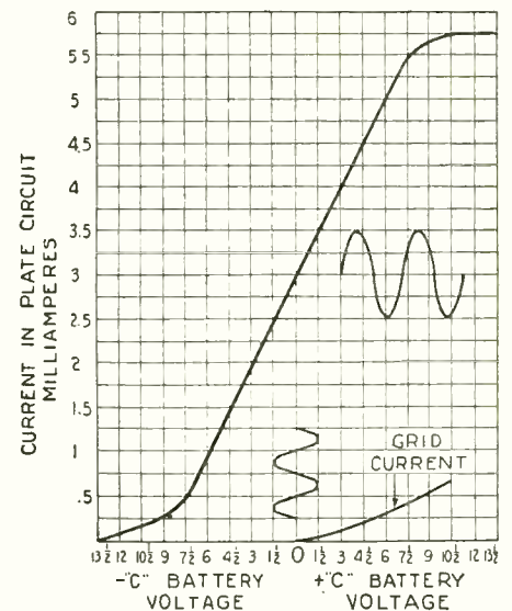
Fig. 4 shows how a signal applied to the grid of a tube varies its voltage, thereby increasing and decreasing the "B" current flowing in the tube.
