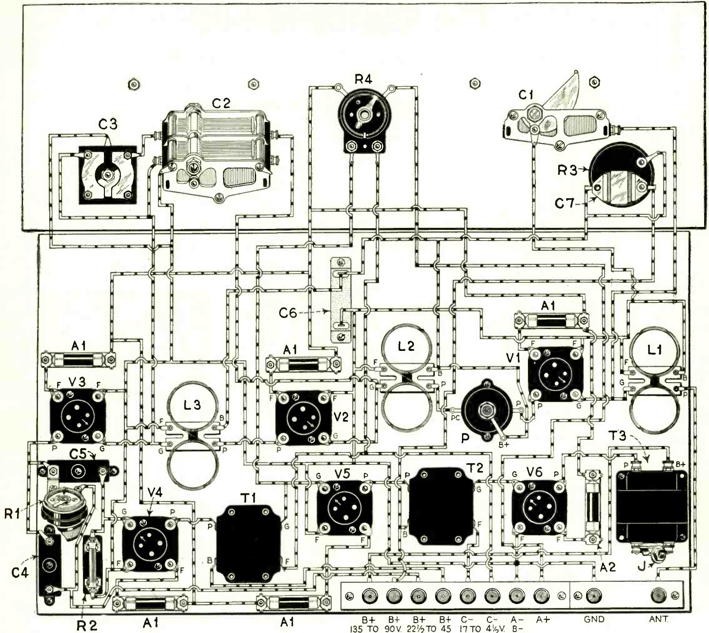
Every connection of the Qualitone Six is shown here very plainly. The terminals of the filament switch are the two lugs which protrude from the top of the resistor R4. Condenser C7 is fastened directly beneath one binding post of the resistor R3.
