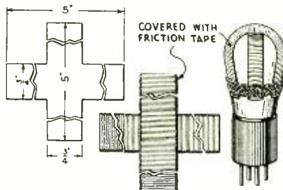
A piece of sheet lead fastened to a vacuum tube as shown will reduce microphonic noises.
