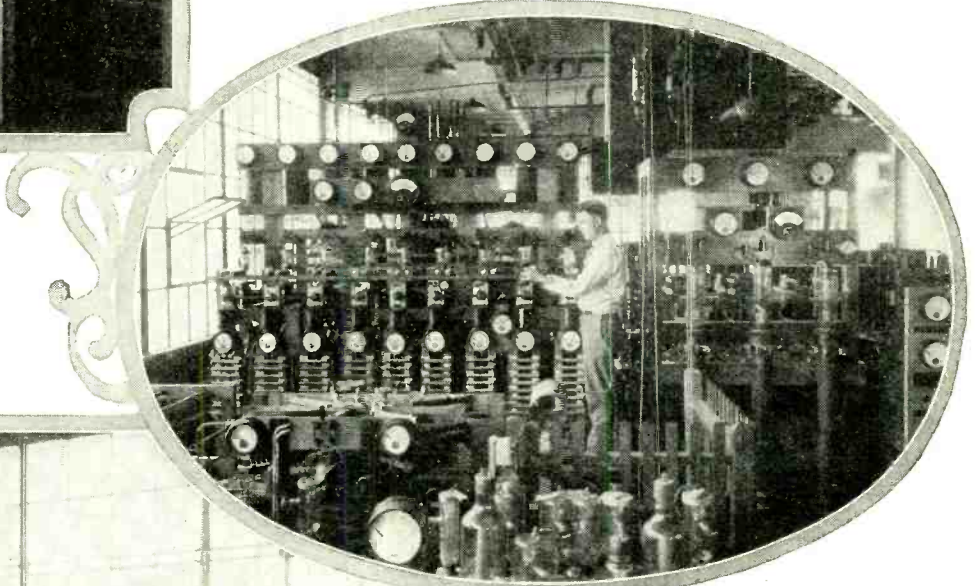
Above at the left is shown the 50-kilowatt transmitter of WGY. and at the right may be seen the new 100-kw. set. The 50-kw. set, which up to the present has been operating on 30 kw. in accordance with the ruling of the Radio Commission, has nine 20-kw. tubes, two of them "spares." A cage antenna two feet in diameter and 240 feet high, and a radial-wire counterpoise, 240 feet in diameter, are used. The 100-kw. experimental transmitter operates on exactly the same frequency, 790 kilocycles, and a quartz crystal is used to maintain this uniform. In the illustration at the left may be seen a section of the 50-kw. modulator unit and, at its right, the 100-kw. tubes used in the super-power transmitter. Because of the great amount of power employed, safety devices of all kinds are installed, so that the operators are perfectly protected at all times. Protective devices shut off the power in case a tube fails and the operator is automatically warned if the cooling water fails. Reports show that high quality was maintained, indicating remarkable control of the enormous power used.
