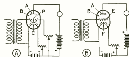
Fig. A., at the left, shows the two-filament tube; to one, the filament P, is made the usual input connection. Fig. B shows a filament having a positive and negative emitting surface.
