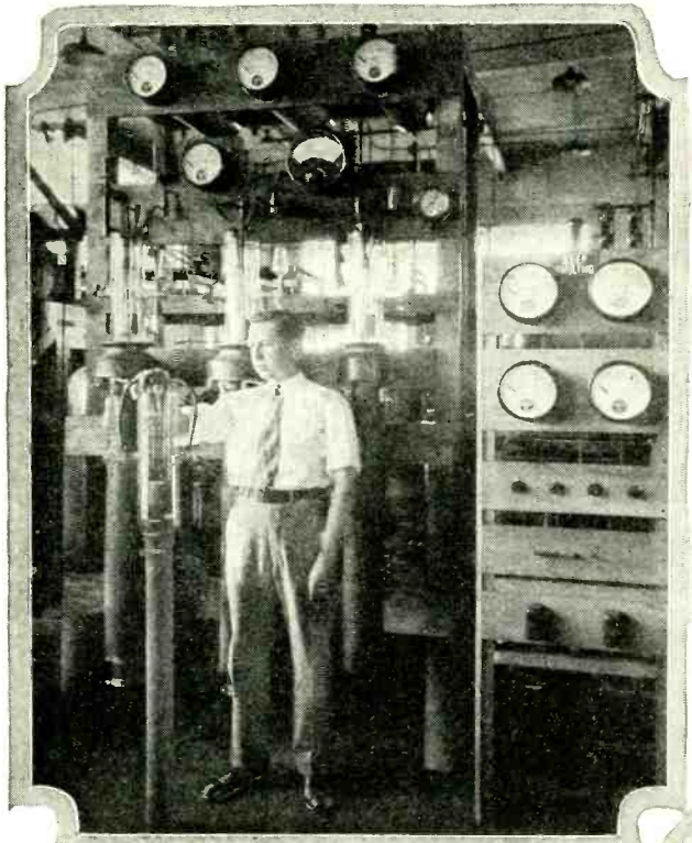
Above is shown one of the operators holding a 100 kw. transmitting tube, which has been removed from its water-cooling jacket. The anode (plate) of these tubes is of copper and approximately three feet long by 3\frac{3}{4} inches in diameter. For filament heating the tube needs 210 amperes at 33 volts, two of these tubes being normally operated in parallel. They work into a "tank" circuit, which is inductively coupled to the antenna by means of coupling coils and a transmission line.
