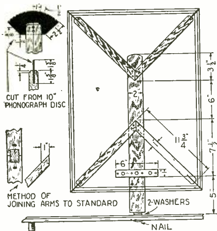
The spreaders of this loop are parts of an old phonograph record.
