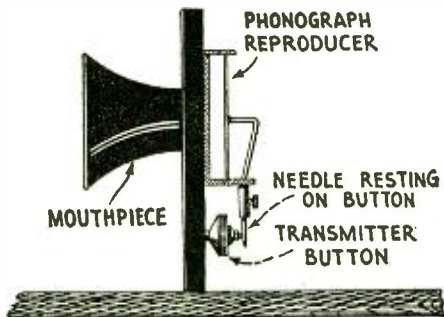
A sensitive microphone can be easily made by mounting a "Skinderviken" button as shown.
