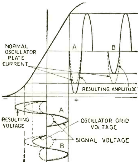
Fig. 8. The diagram shows how the received signal varies the amplitude of the oscillator current, in one way only.
