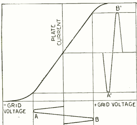
Fig. 6. Curves showing the variations of grid voltage and the corresponding plate current in a vacuum-tube oscillator.
