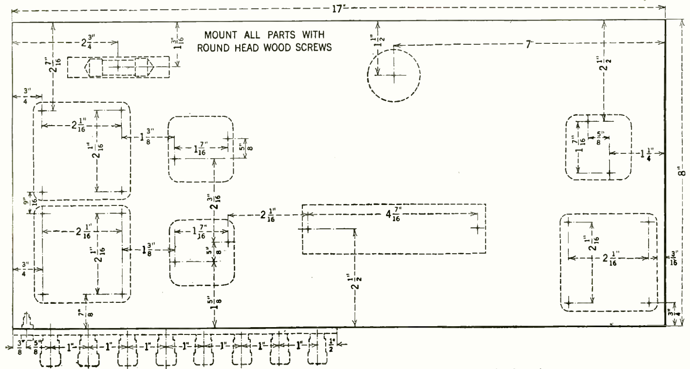
This diagram shows the location of the instruments on the baseboard, which is of wood.
