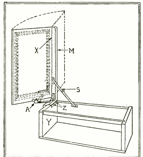
The loop which fits in the cabinet's lid may be rotated without moving the cabinet, making it ideal for portable sets.
