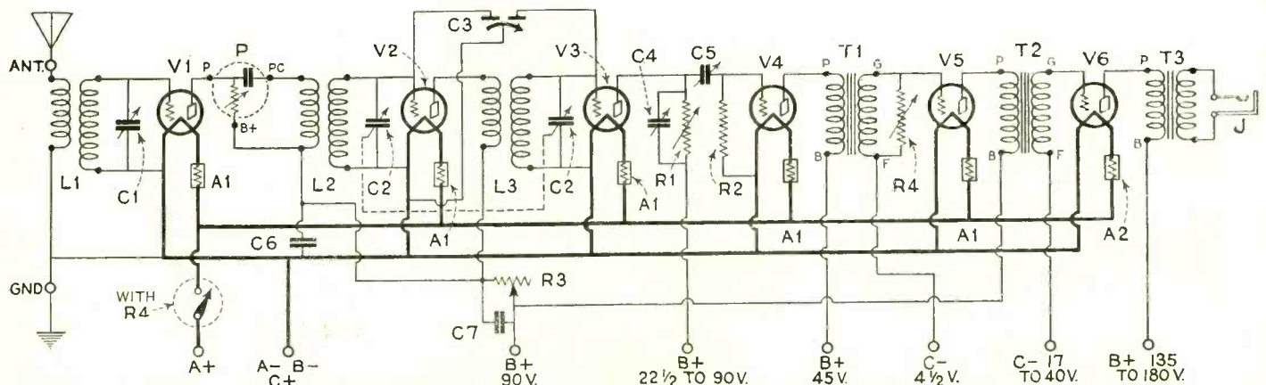
The schematic hook-up of the Qualitone Six. This corresponds exactly to the pictorial hook-up at the top of the page.
