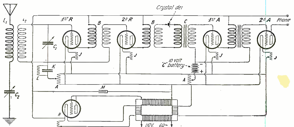
Fig. 3. Alternating current was successfully used in supplying the plates and filaments of the amplifier tubes. A crystal detector was used for rectifying the incoming signal energy.
