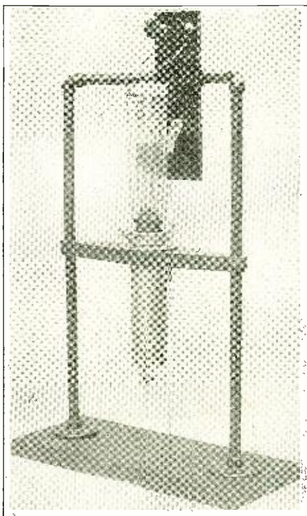
Fig. 1. Outside View of the 20-kw. Tube Which Has Already Been Manufactured in Large Quantities. It Is Known as the U. V. 207.
