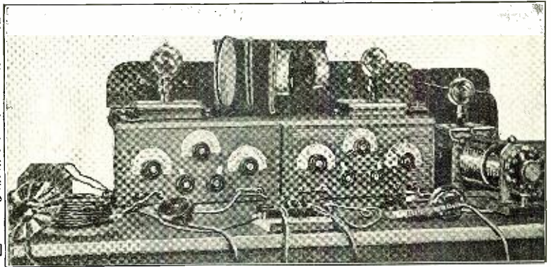
A Receiving Set Employing Both the Autodyne and Heterodyne method for Continuous Wave Reception. In this Combination, the Regenerative Effect is Retained and the Advantage of the Heterodyne Incorporated.
