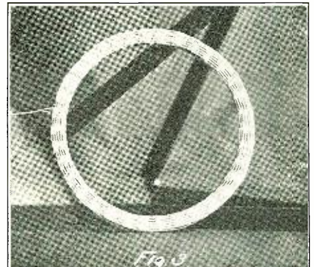
The Completed Coil After Removing the Nails.
