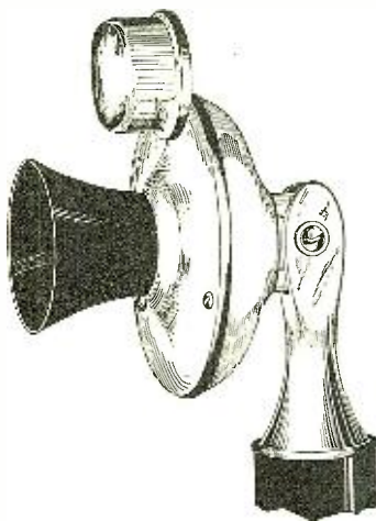
By Mounting the Buzzer on the Microphone, Its Vibrations Will Effect the Telephone Line Currents.
