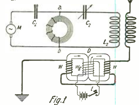
The circuit used in conjunction with the high frequency alternator.
