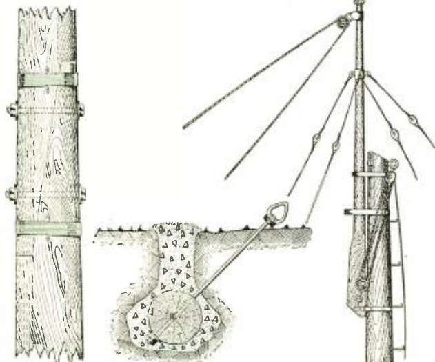
The Mast Guys are Attached to Deadman Anchors Embedded in Cement.
