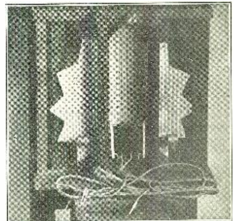
Rear View of the Loudspeaker. An Iron Armature is Fastened to the Lower part of the Round Board.
