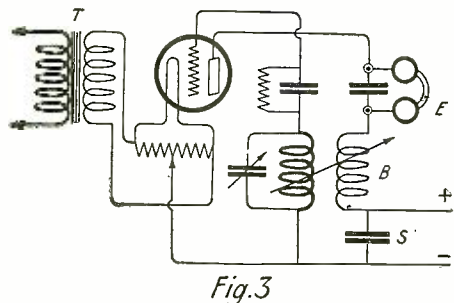
Fig. 3 This Circuit Incorporates the Potentiometer Method of Decreasing the Hum, Together with a Filter System in the Grid Circuit.
