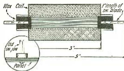
A Choke Coil Amplifier Made from Ford Coil Secondaries.
