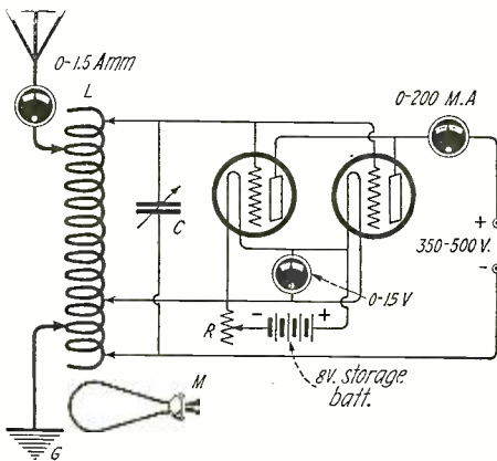
Fig. 2. The circuit of the 10 watt radio telephone transmitter is shown above. Absorption modulation is used.
