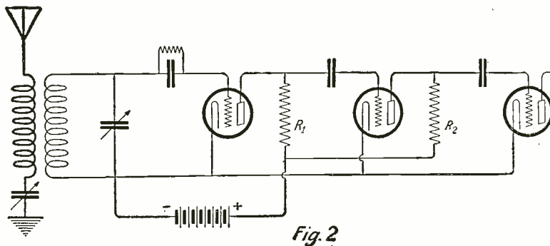
Fig. 1 Illustrates a Resistance-Coupled Circuit, While in Fig. 2 the Same Type Is Shown Applied to a Cascade Amplifier
