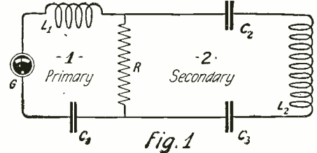
Fig. 1 Illustrates a Resistance-Coupled Circuit, While in Fig. 2 the Same Type Is Shown Applied to a Cascade Amplifier
