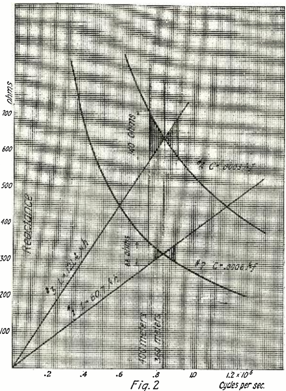
Curves Designating the Reactance of a Circuit in Relation to Various Frequencies. Shaded Portions Denote the Effective (total) Reactance.
