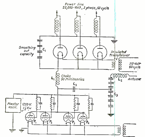
Fig. 3. The Circuit Used in the Recent Tests. The Power Is Supplied from a Three-Phase 60-Cycle, 22,000-Volt Line.
