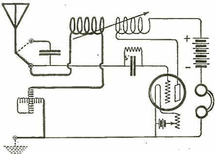
Q. 581. Circuit of the Aeriola Sr. Where a Large Aerial Is Used It Is Connected to the Upper Binding Post as Shown by Dotted Line.
