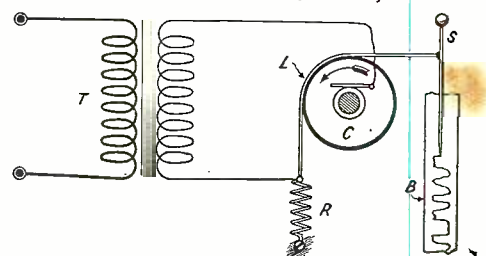
Using an Electro-Static Telephone as a Recorder.
