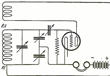
A Circuit Employing Tickler Feed Back and Capacitive Coupling.
