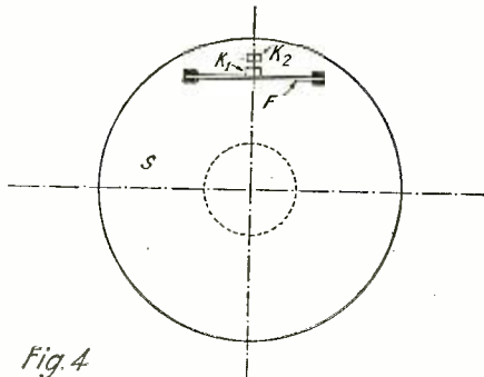
Diagram of the Automatic Speed Regulator Mounted on the Flywheel of the Alternator.
