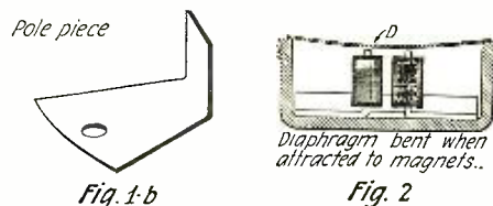
Design of the Soft Iron Pole Piece. Fig. 2 Designates the Influence on the Diaphragm When a Current Traverses the Magnet Coils.
