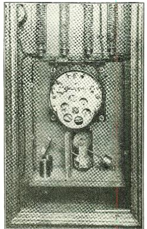
This mercury interrupter is closed one minute before the time signals are sent, and closes all the control circuits.
