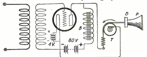
Hook-up of Electro-Static Telephone Used as a Loud Speaker in Conjunction with an Amplifier.
