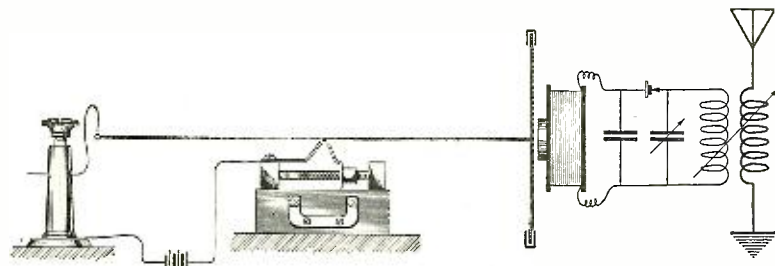
An interesting Type of Mechanical Relay Adaptable to the Recording of Received Signals. The Movement of the Diaphragm is Mechanically Magnified by a Steel Wire Which Completes a Local Circuit.
