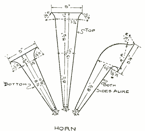
Accurate Mechanical Details are Here Given for the Construction of the Loud Speaker.
