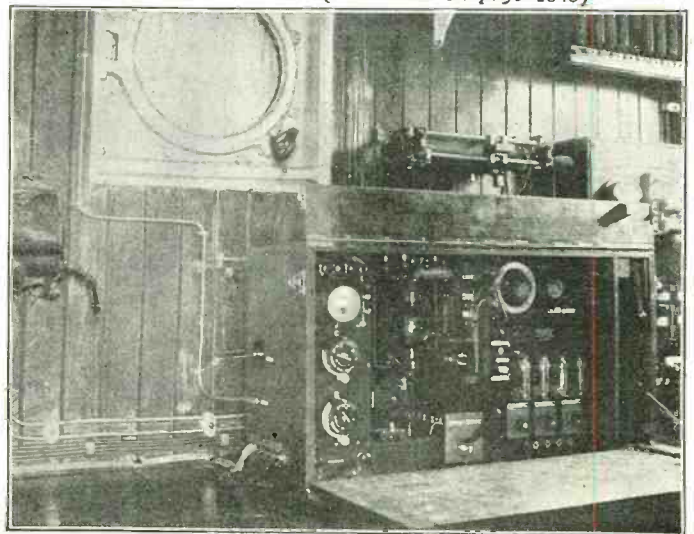
The Lightship Installation.
