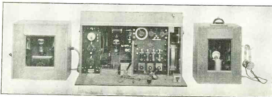
Left: Wireless Bell Call Transmitter. Center: 100-Watt Portable Telephone-telegraph Station. Right: Wireless Bell Call Receiver.
