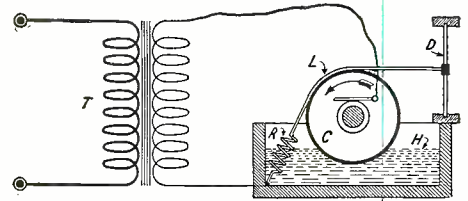
Details of the Electro-Static Telephone Having a Layer of Oil as the Dielectric.
