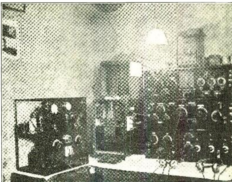
A Station Particularly Neat in Appearance, and Showing Evidence of Precise Workmanship. On the Extreme Left is a 10-Watt Tube Transmitter, Using Either Phone, I. C. W. or C. W.
