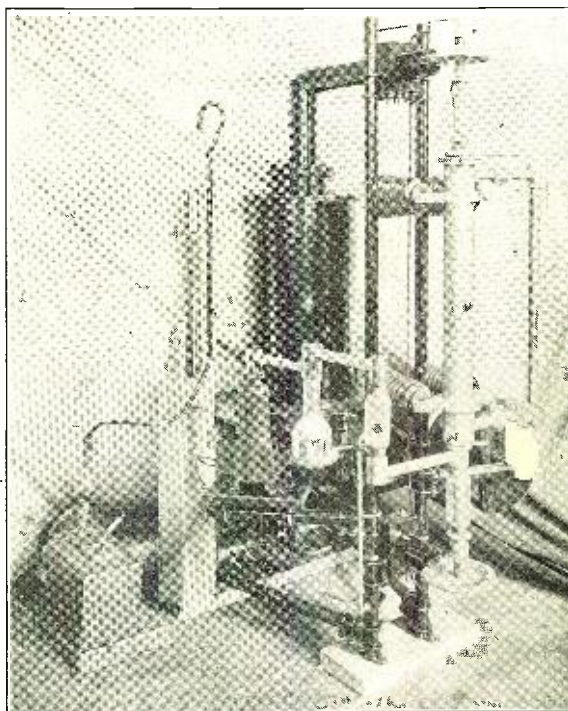
The Space Taken Up by This 1,000-kw. Tube Is Very Small Compared to That Required by a High-Frequency Alternator of the Same Capacity.
