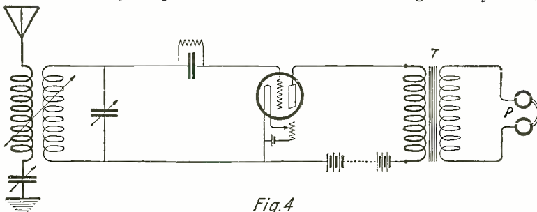
A Vacuum Tube Receiving Circuit Incorporating a Step-Down Transformer in Conjunction with a Pair of Low Resistance Phones as Described in this Article.
