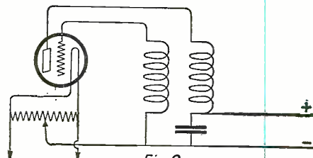
Fig. 2 This Circuit was Found Practical in Using A.C. Filament Lighting. The A.C. Hum is Decreased to a Considerable Degree.
