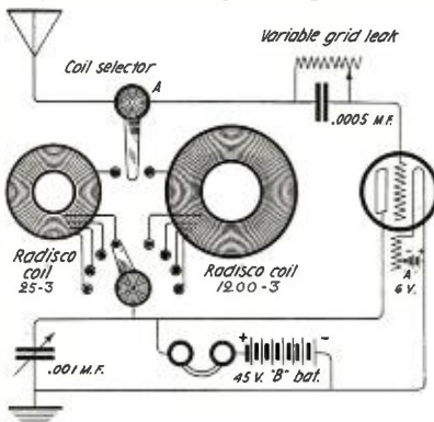
Complete Hook-up of the Light and Efficient Portable Receiver for Vacationists.
