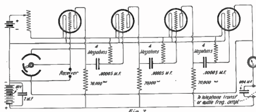
This Four-Step Resistance Amplifier May Be Used Alone or With a Two- or Three-Step Audio Frequency One Hooked Up in Place of the Fones.
