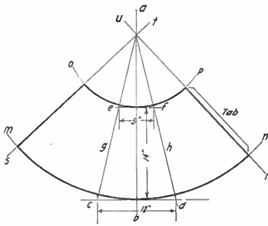
With This Sketch It is Very Simple to Make Cones of Any Desired Dimension Without Wasting Pounds of Paper.
