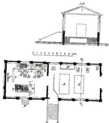
FIG. 1.—GROUND PLAN AND ELEVATION OF ROME RADIO STATION. A 250 kw. Set. I Antenna Inductance. B 200 kw. Set. J Arc Switchboard. C Auxiliary 110 Volt Set. K Motor for Rotating Cathodes. D Shunt Capacity across Arc. L Panel Board Carrying Contacts of Keys. E Keys. M Starting Arc-Resistance. F Ground Condenser. N Operating Table Carrying Keys. G Antenna Switchboard. O Blowers for Keys. H Close Galle. P Arc Starting Resistance. I Illuminating Gas Aspirator. Q Resistance of Arc Shunt, Circuit. J Motor-generator Switchboard. S Fouling Arcs.
