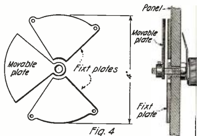
Diagram of the Reaction Condenser. The Distance Between the Movable and the Fixt Plates is to Be Found by Experiment.
