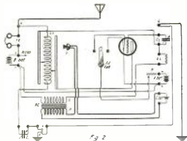
Diagram of Connections for the Simple Radio-telephone Circuit Using Only One Tube for Transmitting and Receiving.
