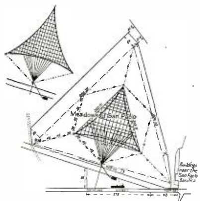
Bird's Eye View of the Triangular Antenna at Rome Radio Station.
