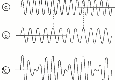
Fig. 2. This Diagram Shows Clearly How Beats Are Produced in the Auto or Heterodyne Reception.
