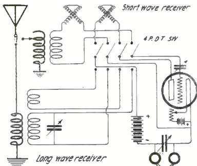
Here is How to Use the Same V. T. Detector With a Short Wave Regenerative or a Honeycomb Coil Set. A Telephone Switch Does the Trick.
