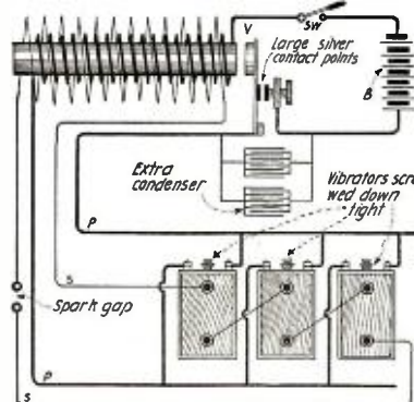
Bugs! Why Not Use Your Old Ford Coils This Way and Obtain More Juice?
