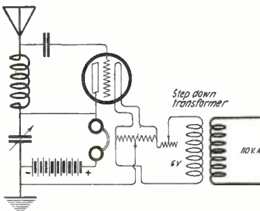
With a Set Connected as Shown, the Filament of the V. T. May Be Supplied With A.C. as Well as in Any Other Receiving Circuit.
