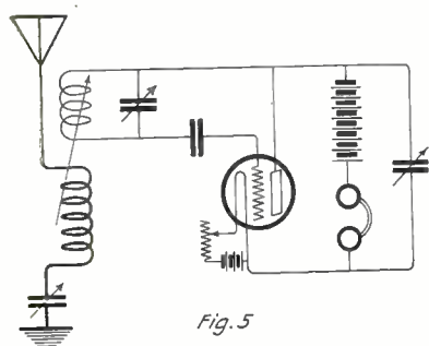
This Ultraudion Circuit Uses Capacity Instead of Inductive Coupling Between the Plate and Filament.
