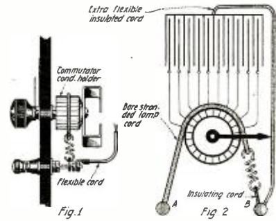
With an Old Motor Commutator You Can Make a Fine Variable, Boys. Look Here and See How Simple It Is.
