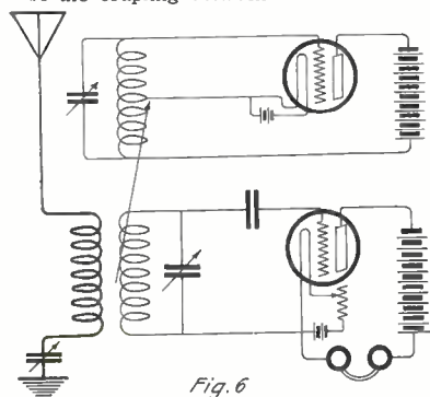
How Beats are Produced by the Use of a Separate Heterodyne Which Acts as a Small Transmitter Closely Coupled to the Receiver.
