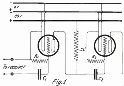
This Diagram Shows the Typical Connections of a Resistance Amplifier.
