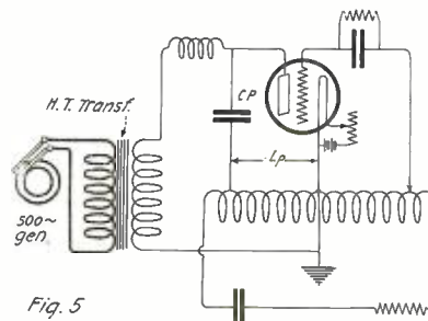
Fig. 5 Hook-up of a C.W. Transmitter Supplied With 500 Cycles A.C. as Plate Current.
