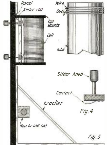
Side View of the Panel Showing How the Inductance is Fixed and Details of the Slider and Winding. Note the String Placed Between Each Turn of Wire.
