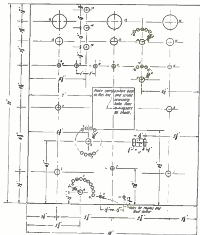
Layout of the Panel. In This Sketch All Necessary Dimensions Are Given for the Benefit of the Amateur Who May Build a Similar Receiver.
