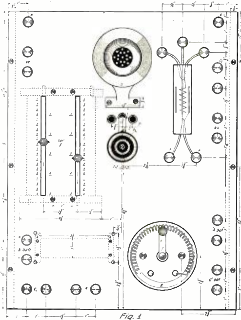
Fig. 1 Dimensions and General Layout of the Panel on Which All the Elements of the Radiophone are Placed.
