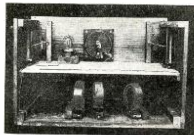
Inside View of a Receiving Set in Which the Primary and Secondary Condensers Are of the Type Described in This Article. They May Be Seen on Each Side of the Upper Shelf.
