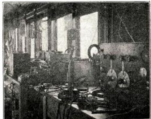
Inside View of the Coach Used as a First Station, Showing the Microphone and Receiving Set Used for the Tests.
