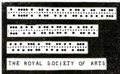
Fig. 7. Tape Perforated by the Creed Perforator Shown in the Photograph and the Same Sentence as Printed in Roman Type by the Automatic Typewriter.
