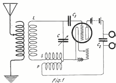
The Typical Armstrong Feed Back Circuit, Better Known Among the Amateurs as the Regenerative Circuit.
