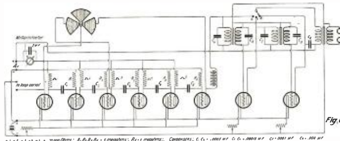
This Eight-Step Radio Audio Frequency Amplifier is the Most Sensitive Actually Used, and Gives Wonderful Results With Only a Small Loop Aerial.
