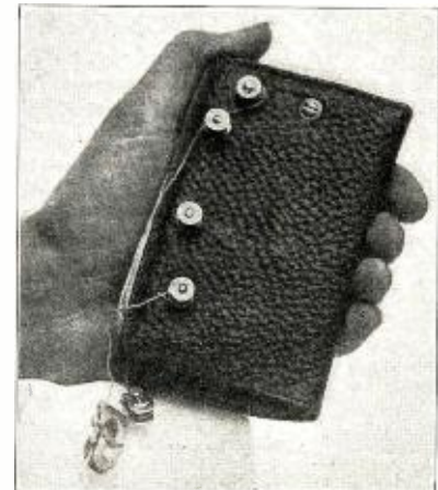
This Shows the Size of the Set When Folded. Two of the Binding Posts are for Aerial and Ground, the Two Others for the Fones.
