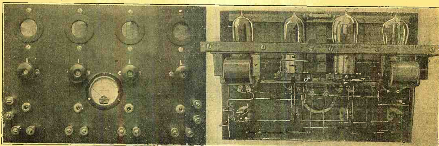
Here is Proof of the Pudding, illustrated for the Benefit of Those Who May Doubt the Fact That Any Boy, Armed with the Proper Tools and Knowledge Gained from Contemporary Radio Magazines Cannot Duplicate the Above Example of Workmanship. To the Left is Seen the Front View of the Panel Which Has Sufficient Appliances to Operate a Detector and Three Stages of Audio Frequency Amplification. To the Right We Have the Rear View of the Instrument Which Shows How the Various Parts Were Mounted. The Center Amplifying Transformer Is at Right Angles to the Two Outside Ones. The Wiring is Well Spaced Which, in Addition to the Rest of the Set-up, Helps Make the Set a Very Business-like One. Let Us See More Samples of Amateur Workmanship.
