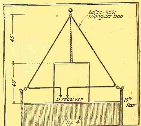
Fig. 4 Schematic Sketch of One Type of Loop Antenna Tried Out by the Navy Dept. at the "Times" Radio.
