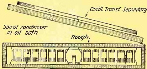
Build a Trough and Get Yourself Four Hard Rubber Combs, as Well as Some Copper Strips, Then Go to It.
