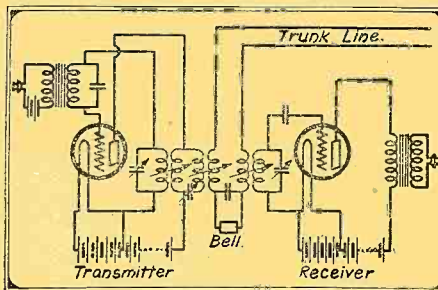
Fig. 1. Schematic Wiring Diagram of the System as Applied to Multiple Telephony.
