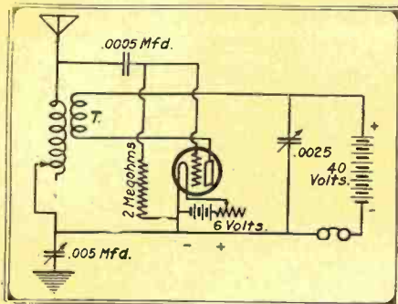
A Simple Damp-Undamp Circuit Employing One Single Inductance In Addition to a Tickler Coil.
