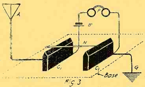
Simple Form of Auto-Coherer Made by Placing a Needle Upon the Top of Two Small Carbon Blocks.
