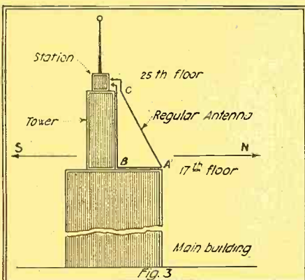
An Unusual Triangular Loop Where Two Sides of the Antenna Were Formed by the Steel Structure of the Building.
