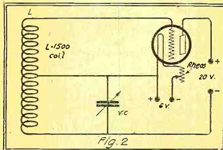
Fig. 2 Simple Heterodyne Circuit Used to Provide Necessary "Beat" Notes in Connection with the Receiver Shown in Fig. 1.
