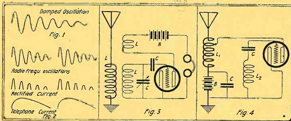
Figs. 1 and 2 illustrate the performance of a damped oscillation in a detector circuit. Fig. 3 shows a simple inductive feed back circuit, while Fig. 4 is that of a conductive coupling, which furnishes greater power in the antenna circuit.
