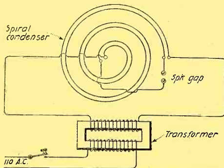
Here is the Circuit Diagram of the Inductodenser. Nice Little Jigger. It Combines Capacity and Inductance.
