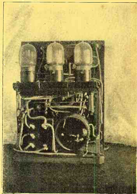
Rear View of the Stearns Radiophone Set, Showing the Three Oscillator Tubes. No Modulator Tube is Employed Here.
