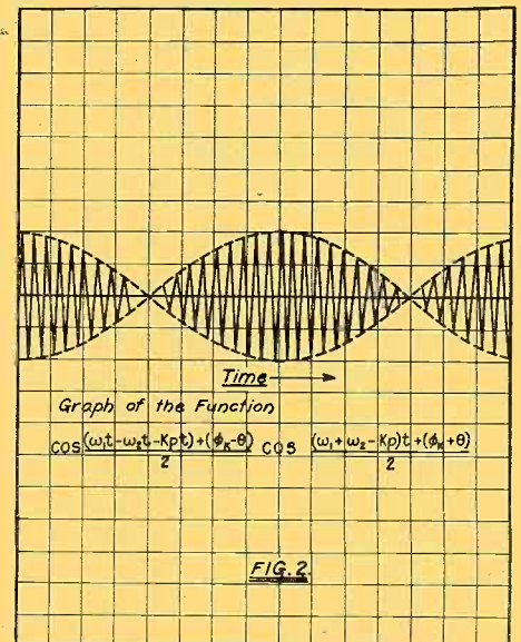
Fig. 2—The Waveform and Trigonometric Product of a Certain Radio Frequency Voltage in Short Wave Reception.
