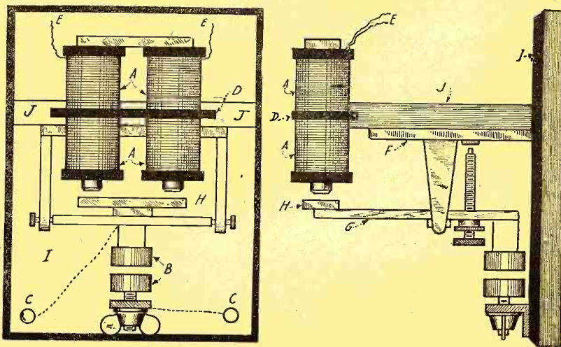
General Layout and Construction Details of a Magnetic Relay Key Designed for Radio Transmission Work Which Mr. Wuth Has Used to Advantage.
