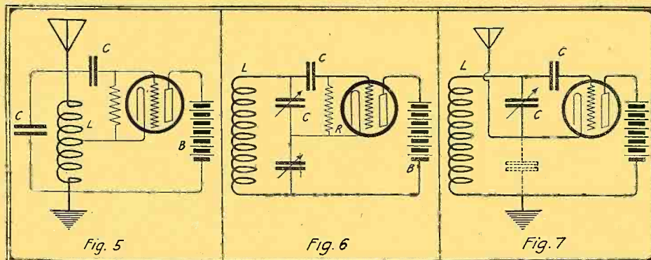
In Fig. 5 is shown another method of feed back. Fig. 6 is the common capacity feed back, while Fig. 7 is similar to Fig. 6, but with antenna in circuit.
