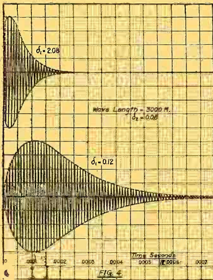
Fig. 4—The Upper Graph (a) Approximates a Static Disturbance of High Decrement While the Lower Graph (b) is That Produced in a Receiving Circuit By a Given Spark Transmitter of Low Decrement.
