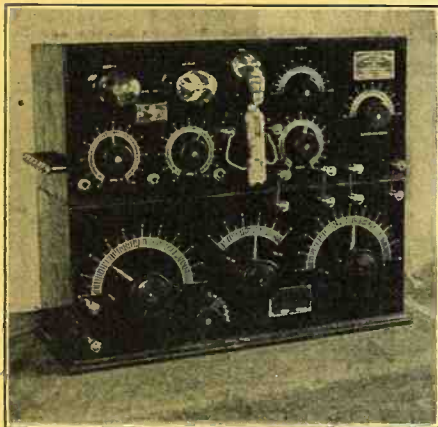
C. R. L. Paragon Short Wave Reg. Receiver
