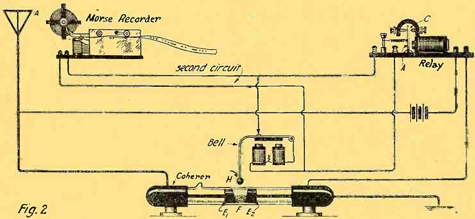
This is the way the Marconi Coherer is made to intercept radio waves in such a manner that the waves cause a sensitive relay to respond and in turn operate the Morse Ink Recorder. An additional battery must of course be placed in series with the second circuit.
