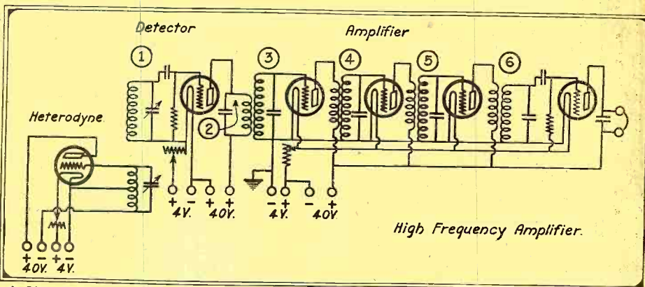
A Circuit Diagram of the Connections Employed in the Armstrong High Frequency Amplifier System.
