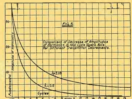
Fig. 5—In This Instance It is Seen That the Amplitudes in the Highly Dampnt Signal Fall Off Less Rapidly Than the Lightly Dampnt Signal.
