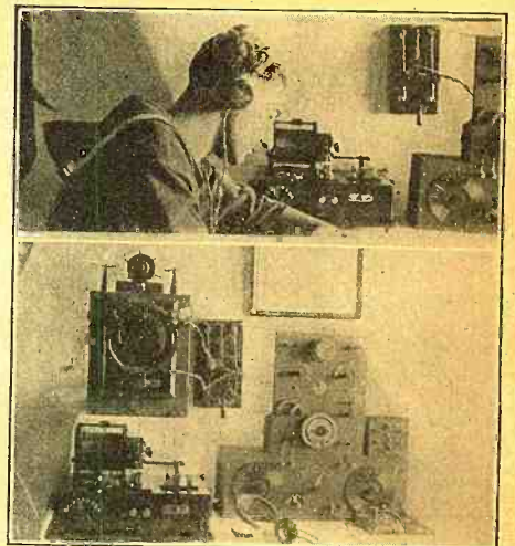
Three Cheers for the Navy. Mr. Kohnitz is Still in the Service and is Going Strong. Transmitter and Receiver Layout of Real Merit.
