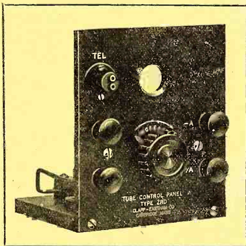
Tube Control Detector Panel Z. R. D., $12.00
