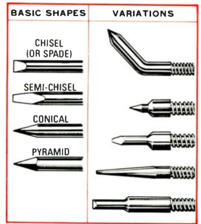
FIG. 2—SOLDERING-IRON TIPS are available in a wide variety of sizes and shapes. They come as complete tips, interchangeable elements, or tips for interchangeable elements.
