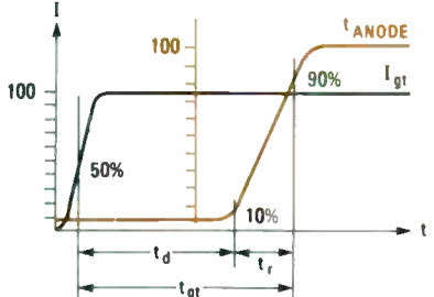
FIG. 7—AN SCR's TURN-ON time is composed of delay time t_d and rise time t_r .
