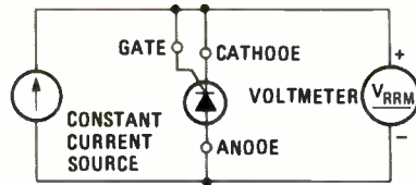
FIG. 4— V_{RRM} IS MEASURED using a constant-current source.
