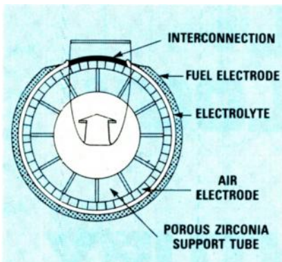
FIG. 6—STATE-OF-THE-ART FUEL CELL. Developed by Westinghouse, this cell has produced power outputs as high as 32 watts. For higher outputs, cells can be bundled in a variety of configurations.
