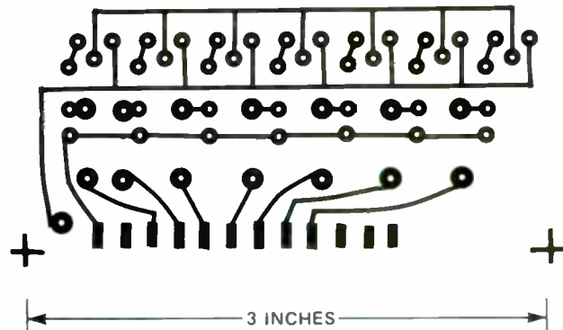
COMPONENT-SIDE DIRECT-ETCH FOIL PATTERN for the C64 Armatron controller. Don't forget to install the jumper!
