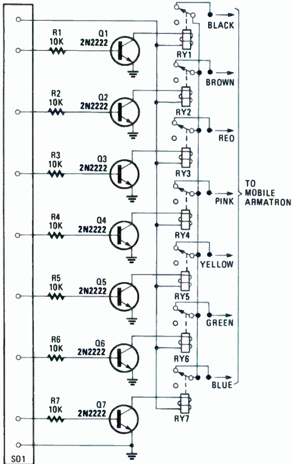
FIG. 1—YOU CAN ADD COMPUTER CONTROL to a Radio-Shack Mobile Armatron with this simple interface. It replaces the robot arm's control module.
