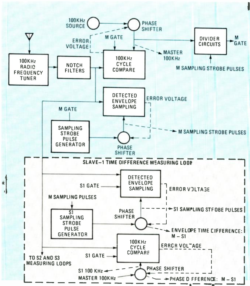
FIG. 5—A KEY TO THE ACCURACY of Loran is the receiver's ability to track its local oscillator to that of the master station through a 100-kHz Cycle Compare circuit—actually a conventional phase-locked loop.
