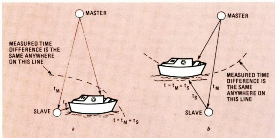
FIG. 2—LOCATION IS DETERMINED by the time difference between signals received from a master and those from its associated slave station(s).
