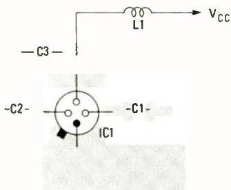
FIG. 5—THIS IS THE COMPONENT LAYOUT for the basic amplifier. All components are on the soldering side of the board.
