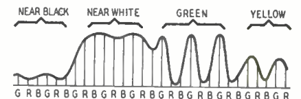
Fig. 4—Signal after passing through 4-mc filter. This is applied to modulator.
