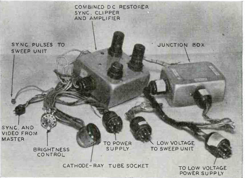
Fig. 3—This maze of cables and plugs connects the various units together. Be sure to label everything unmistakably to avoid that nervous breakdown later on.
