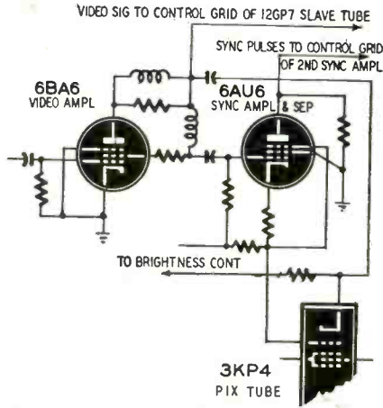
Fig. 4—A portion of the Pilot receiver.
