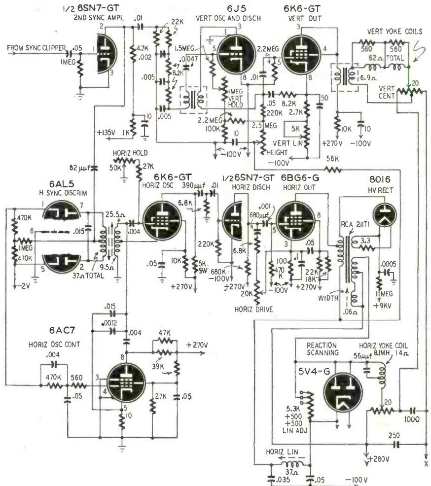
Fig. 2—Vertical oscillator and output stages, horizontal a.f.c., oscillator, and output stages shown above were all on a single chassis, and in working order.
