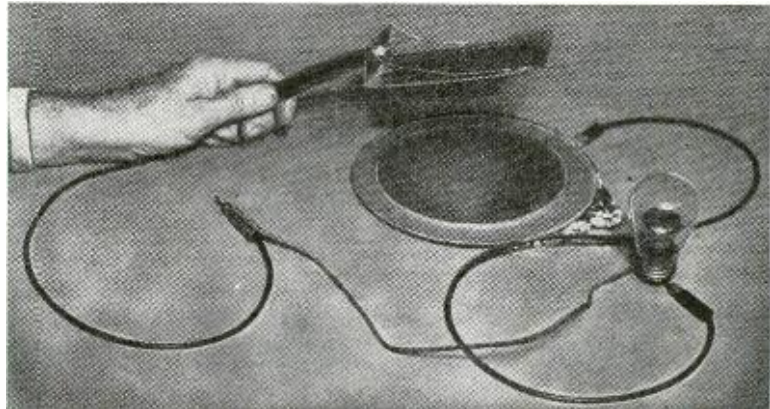
Fig. 4—Electret provides output enough to flash 2-watt neon lamp.
