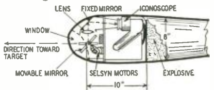
Fig. 2—Arrangement of components.
