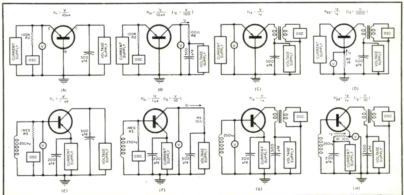
Fig. 4. Equivalent circuits for h measurements for p-n-p transistors. The upper row shows the grounded base connection, while the lower row shows the corresponding grounded emitter connection.
