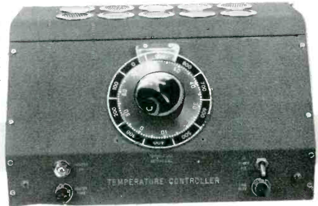
An over-all view of a production model of the temperature controller, showing the Helipot ten-turn dial, pilot light, power switch, and the two fuses.
