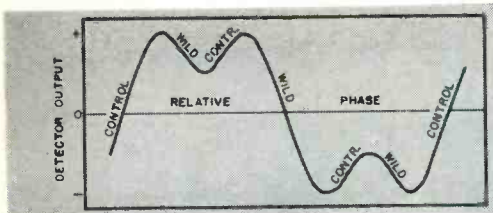
Fig. 8. Phase detector output for complicated ratios can have several maxima and minima, and control slopes as shown.
