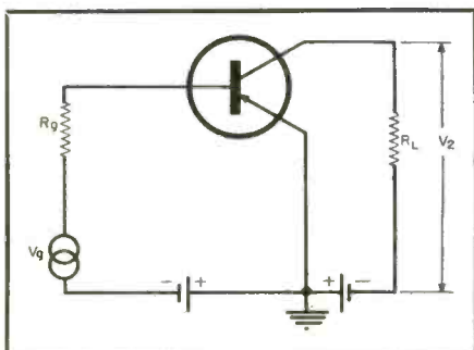
Fig. 7. Grounded emitter amplifier.
