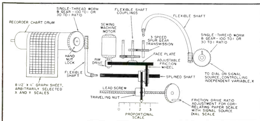
Fig. 4. Mechanical schematic diagram of the Y-function plotter.
