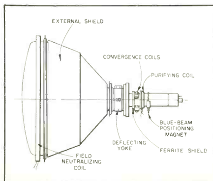
Fig. 4. Layout of external components.
