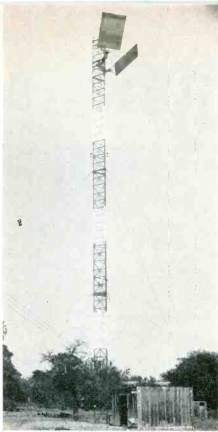
A 6000-mc. microwave repeater station using passive reflectors on tower.
