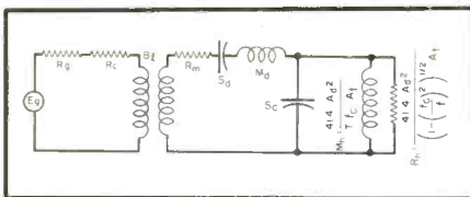
Fig. 1. General equivalent circuit of a horn-loaded loudspeaker.
