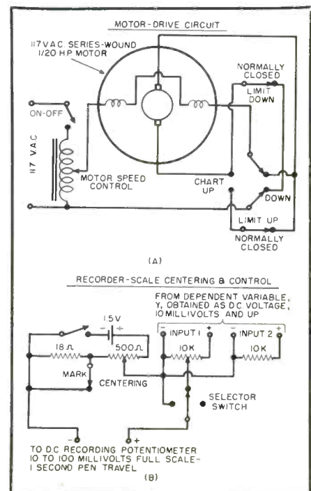
Fig. 5. (A) Motor drive circuit and (B) recorder-scale centering and control.
