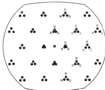
Fig. 7. Ideal error pattern. Dynamic convergence controls are adjusted to form equal size triangles over entire screen area. Static convergence adjustments serve to superimpose dots of all triangles.
