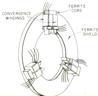
Fig. 3. Convergence assembly for "205."
