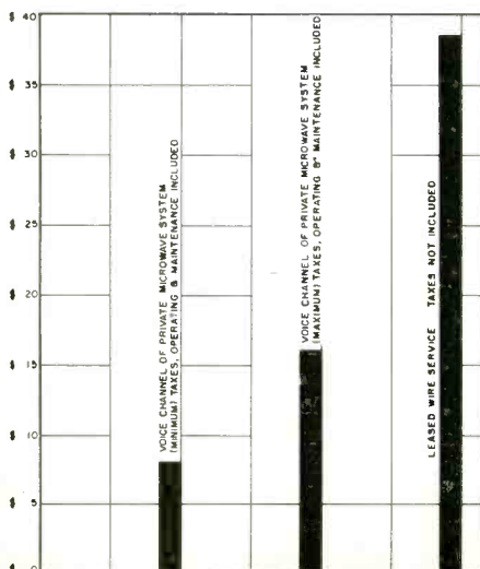
Relative per-channel-mile cost of a single voice channel of a 24-channel 300-mile microwave system compared with estimated cost of leased wire service.
