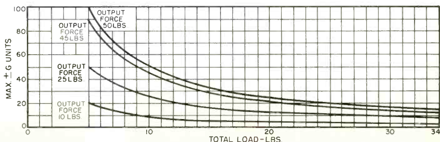
Fig. 1. Force output necessary to produce a specific g with a specific loading.
