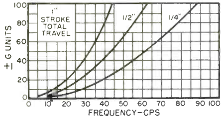
Fig. 3. Frequency vs. g units for various lengths of stroke travel.
