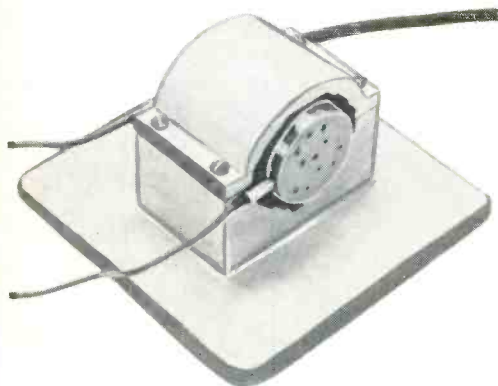
A piezoelectric shaketable vibrator.
