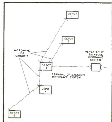
Possible method of distributing microwave-derived channels in a large city when leased wire lines are not available.
