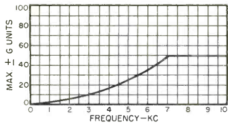
Fig. 2. Characteristics of Glennite Model AT-10 piezoelectric shaker.
