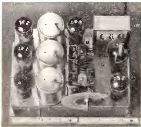
The chassis of the Falck Model 77 is unusually sturdy, and completely shielded, with all wiring insulated, and the transformer well ventilated and cooled.
