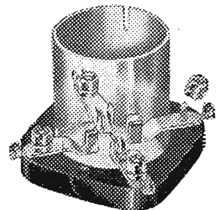
The revolutionary design of the C-H Low Loss Socket created a sensation everywhere. Thin ORANGE Bakelite shell. Base of heatproof Thermopax — terminals cannot loosen under heat of soldering iron. One piece contact springs integral with soldering lugs. Contacts grip both sides of each tube prong and are SILVER plated to prevent corrosion losses. Preferred by careful builders at 90c—now 60c because of huge production savings.
