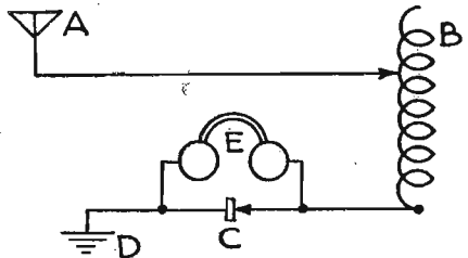
A represents the antenna, B is a coil of wire permitting the antenna to be tuned, C is a detector (one-way street), D is the ground, and E the head phones.
