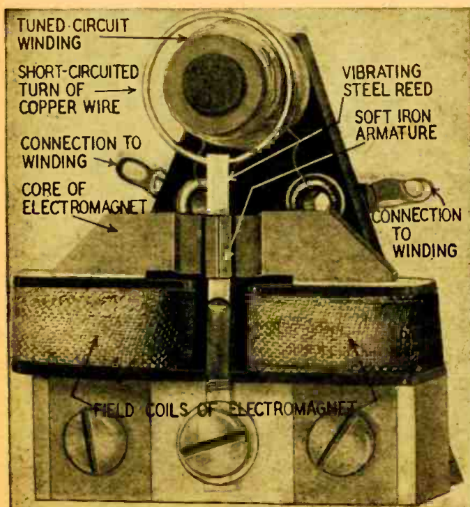
The heart of the instrument is this mechanical frequency modulator.
