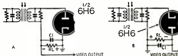
Fig. 6—Detector adjustments to insure positive picture polarity.
