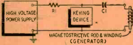
Fig. 2—Another transducer-excitation system.
