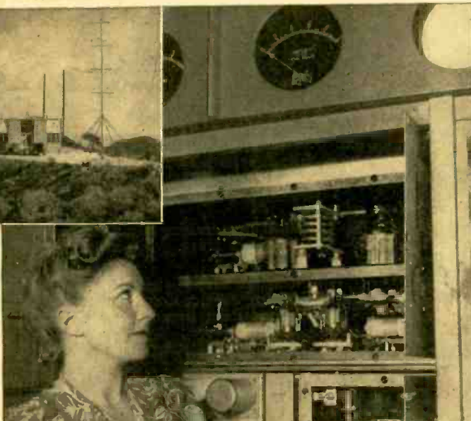
Above—View of FM station K45LA, erected atop Mt. Lee in Hollywood. Right—Virginia Sfmms takes a peep at the internal structure of the W. E. Frequency Modulation Transmitter operated by the Don Lee Broadcasting System in Hollywood.
