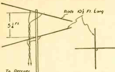
Simple FM Receiving Aerial
