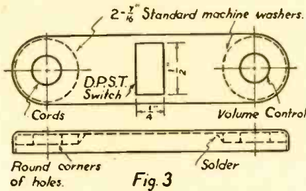
Bottom end of tin File thru Drill for V.C. - Sw. and cords. See Fig 3
