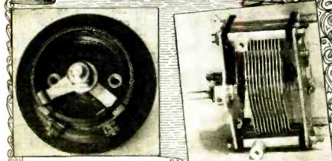
Early Filament Rheostat, 1922-25 G.S.
