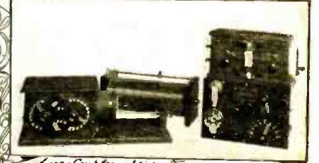
Loose Coupler, Slide Tuner and Audio Control Boxes, from 1915-1919 M.C.M.S.
