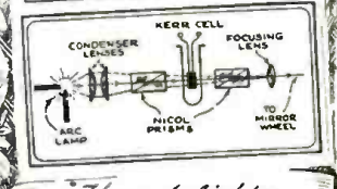
Kerr (light-modulating) cell, and system showing its application, about 1931.
