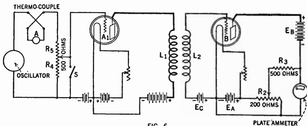
FIG. 6 METHOD OF MEASUREMENT OF TRANSFORMER-COUPLED AMPLIFIER
