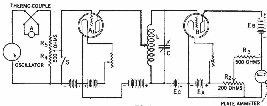
FIG. 4 METHOD OF MEASUREMENT OF TUNED AMPLIFIER
