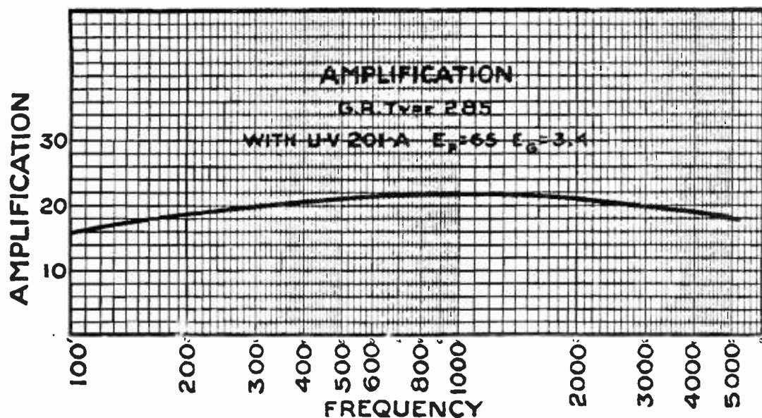
Amplification Curve of the Type 285 Audio Transformer
