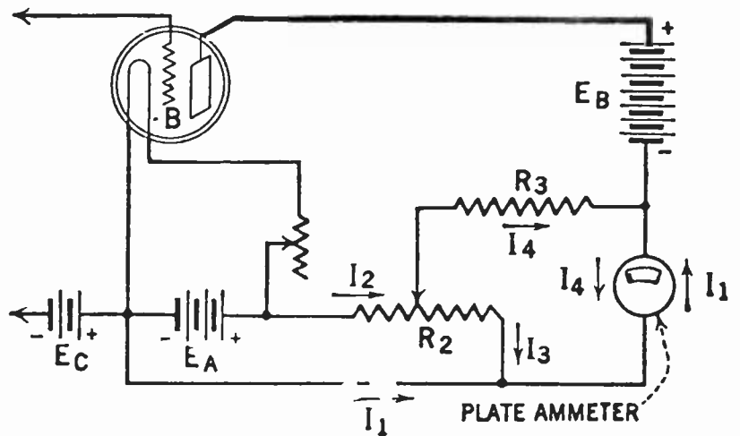
FIG. 5 DETAILS OF BALANCING ARRANGEMENT
