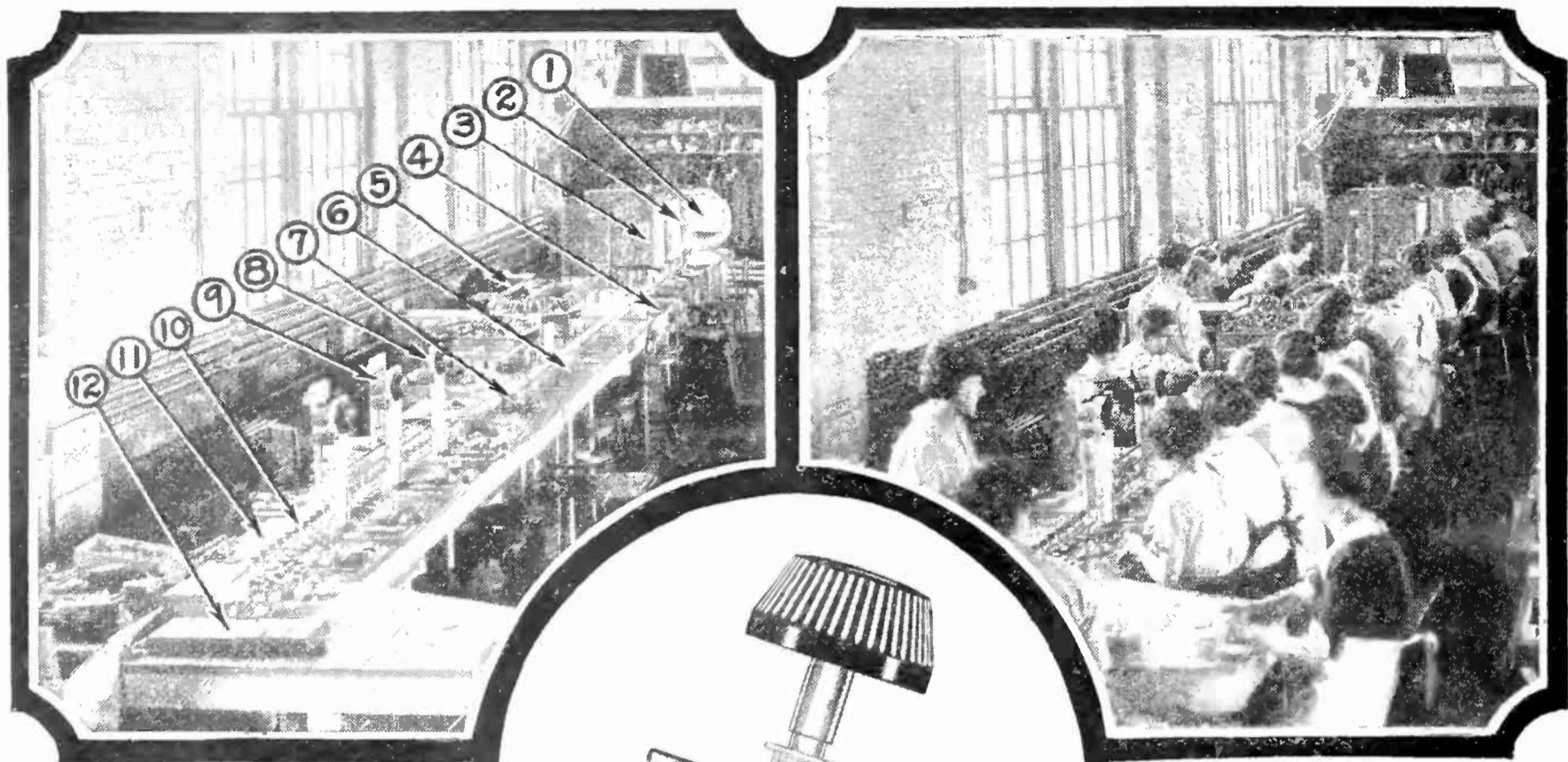
View of one production line, showing operators assembling Bradleystats and packing them in cartons for shipment. All parts are fabricated in other departments. The electric furnaces are in a separate building.
