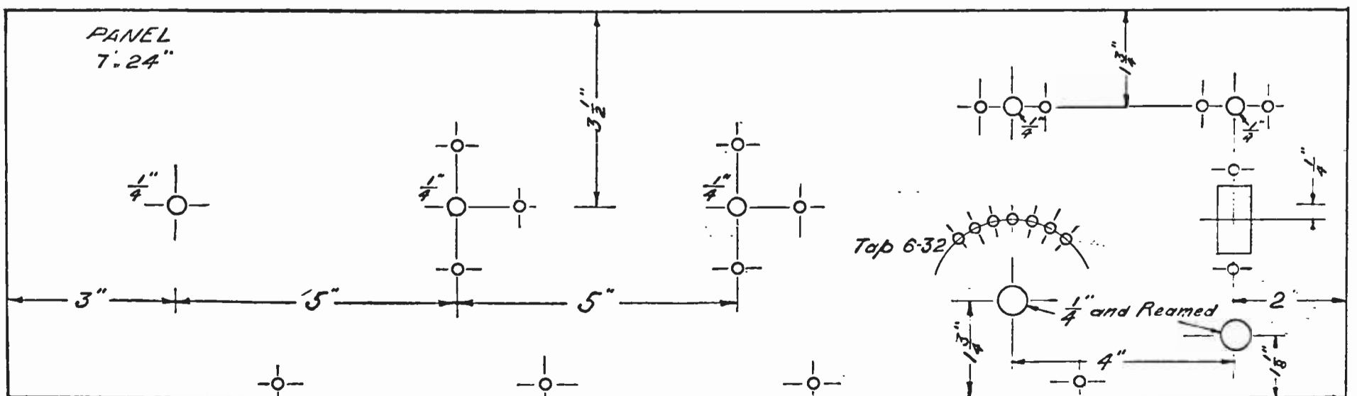
FIG. 3 The panel layout
