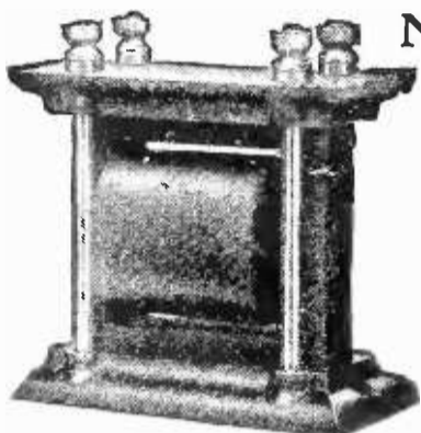
No. 95 Variocoupler
