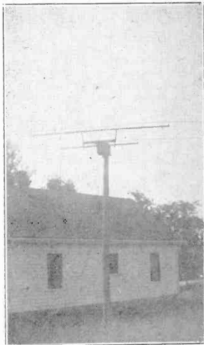
D—The W1CBV antenna, a two-element rotary beam, entirely home-made except the elements and the motor that turns it.
