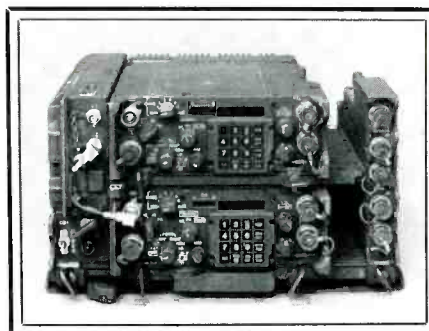
Manpack configuration of ITT's SINGGARS radio.
