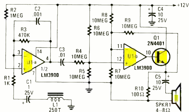
Fig. 5. This telephone amplifier is great for the hearing impaired, or anyone in a noisy environment. It also lets the whole family listen in on a conversation.
