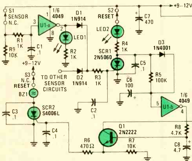
Fig. 1. Two SCR's, a transistor, a 4049 hex inverter, and a few support components, all combine to form a closed-loop detection circuit with a delay feature that allows you to enter a protected area and deactivate the circuit before the sounder goes off.
