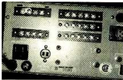
Professional systems have provisions for 25-volt and 70-volt constant-voltage speaker lines. The set of screw terminals in the upper left corner of this amplifier are the constant-voltage outputs.
