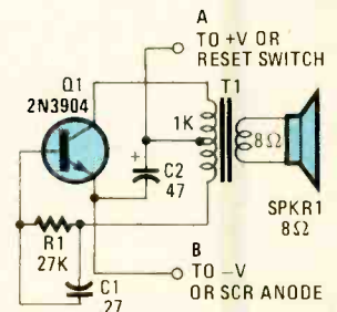
Fig. 3. The Low-Level Sounder produces low-level noise that's loud enough to be heard, but not loud enough to warn off an intruder in another location.
