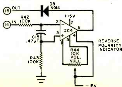
Fig. E. Reverse-polarity indicator.
