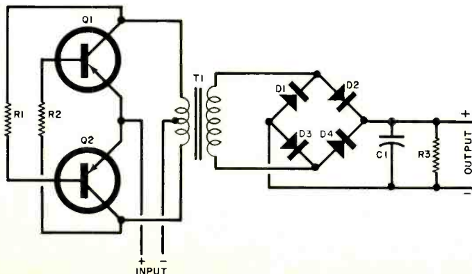
Fig. 2. Practical dc/dc converter featuring "push-pull" transistors.
