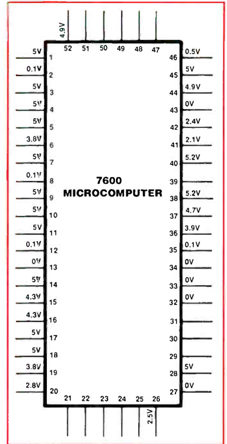
Figure 1. Pinout diagram for the microprocessor in the Philips' A8 (and Y6) chassis.
