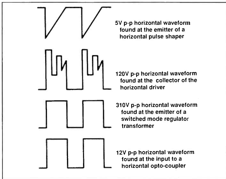
Figure 11. Shown here are samples of typical waveforms found in the horizontal circuit of a scan-derived television power supply.
