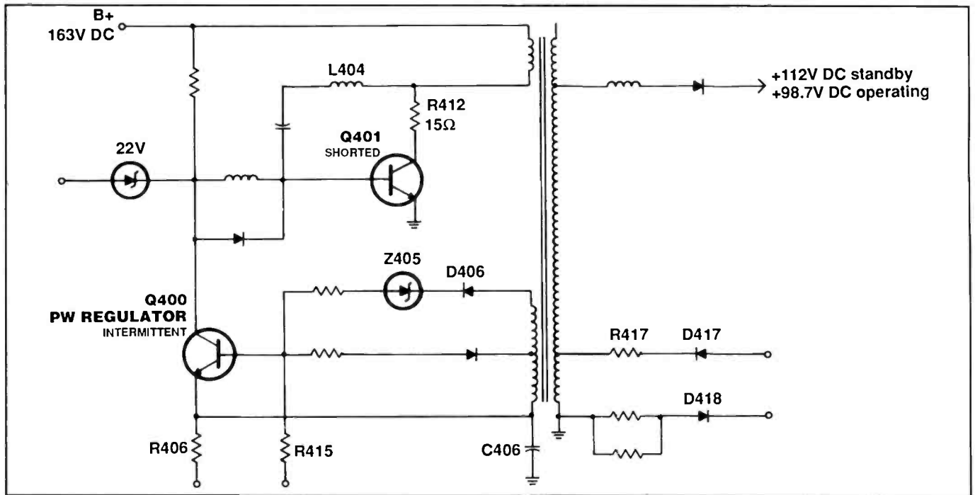
Figure 12. This is the schematic diagram of the switched-mode power supply of a Sylvania Model RAJ147 television set.
