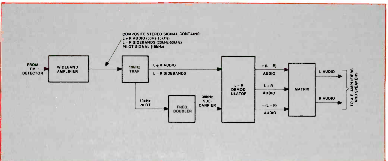
Figure 6. Block diagram of one type of stereo doubler.
