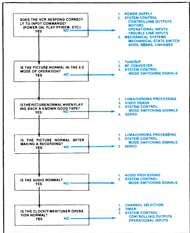
Figure 2. A logical troubleshooting approach will help isolate a problem to a specific area of the VCR. ES&T
