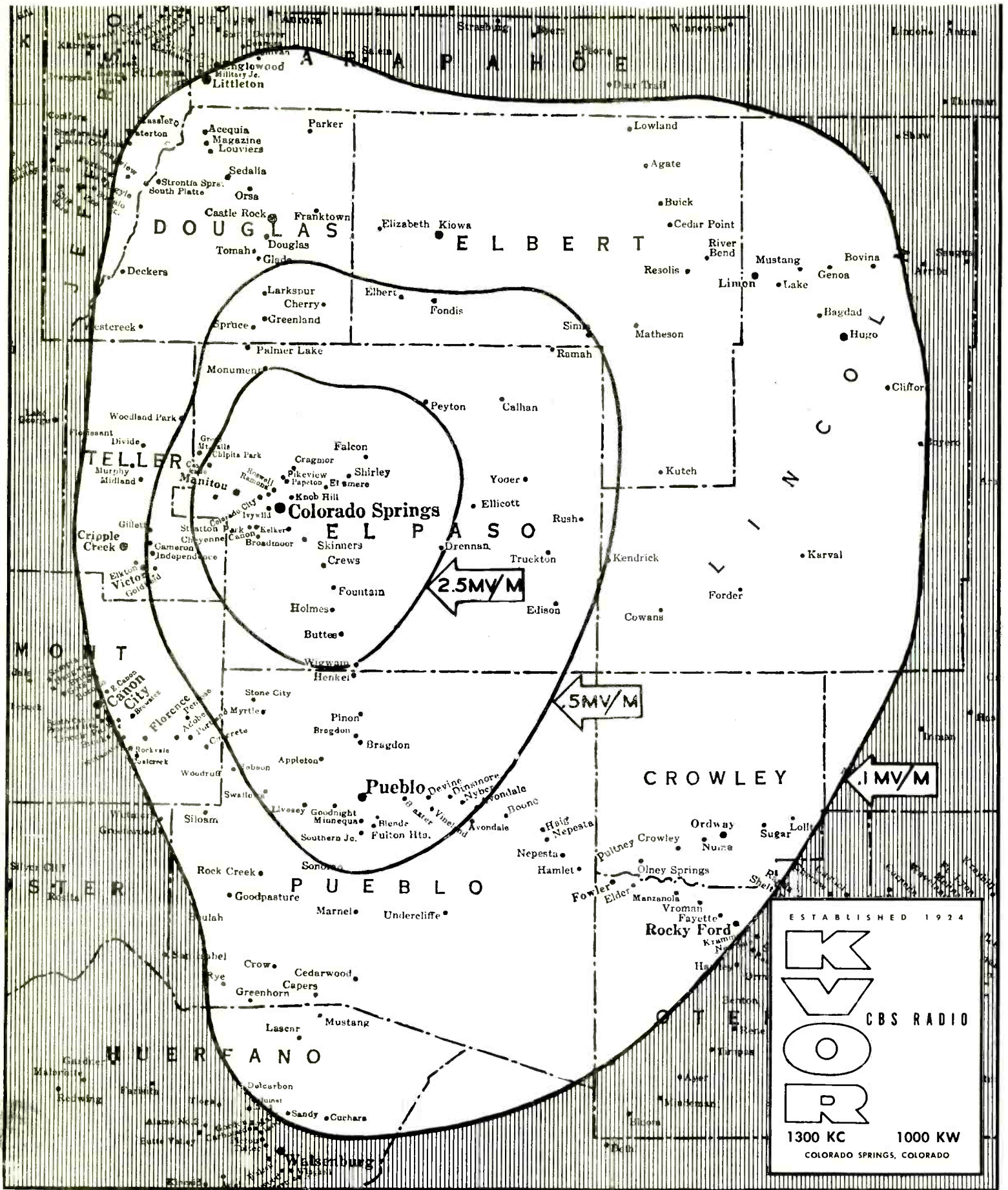
KVOR Dept. of Engineering - Coverage Contour Map
