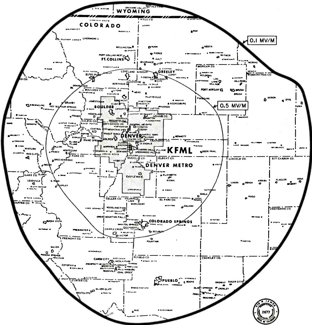
COMPUTED COVERAGE CONTOURS
