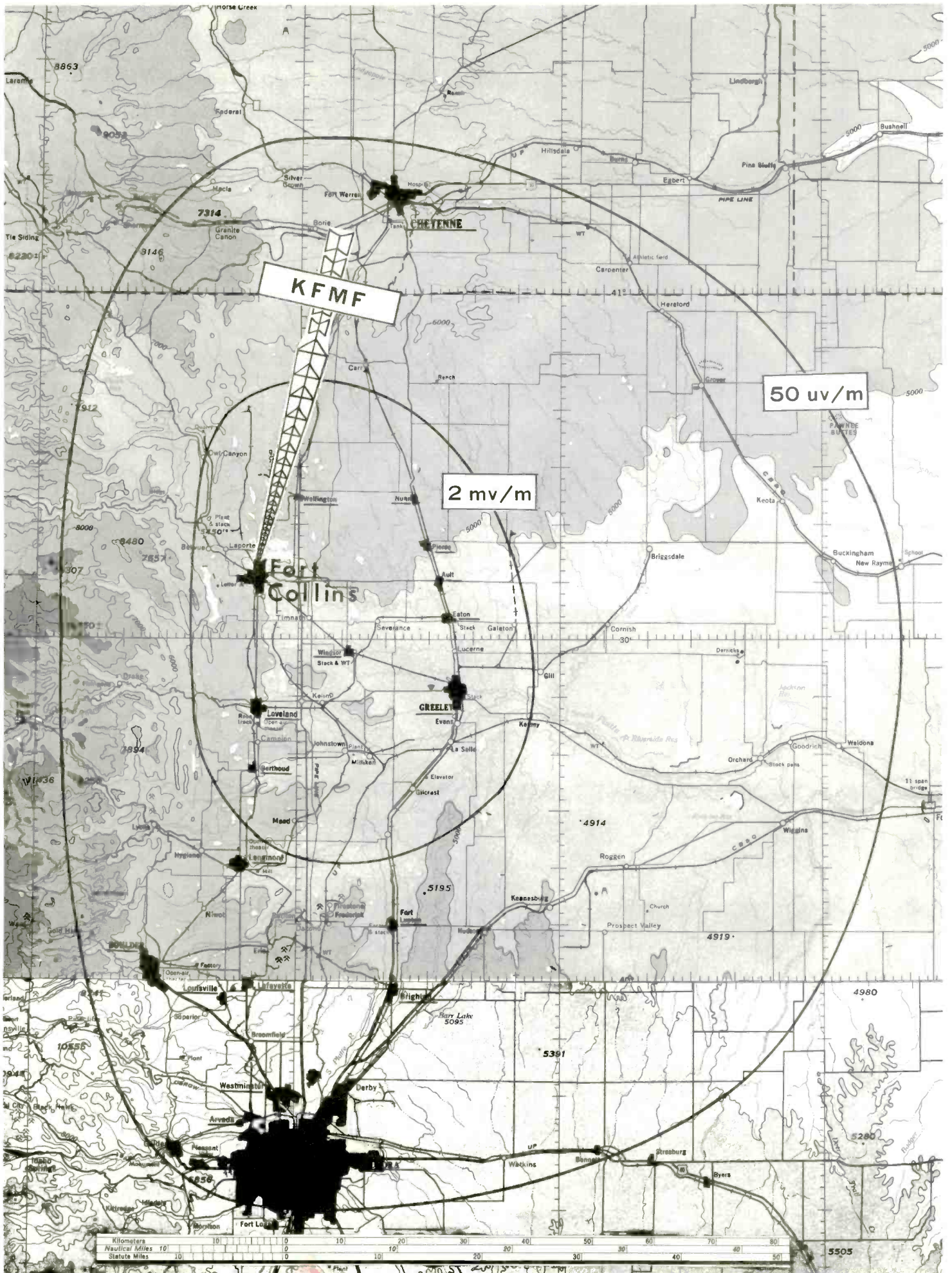
KFMF Coverage Area
