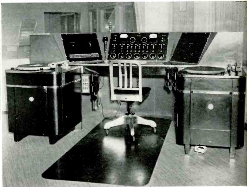
Seated at this control turret the operator has a clear view of both studios and of three racks of speech input equipment.
