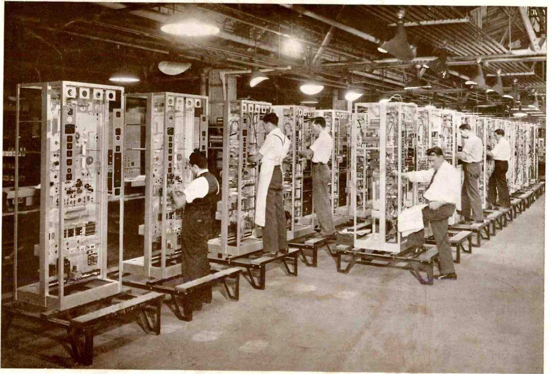
Soon to be in service—twenty seven 405A-1 250 Watt Western Electric transmitters reach final assembly at the Specialty Products Shop, Kearny, N. J. This transmitter was described in Pick-Ups , August, 1940.
