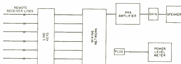
Block schematic of the remote receiver system.
