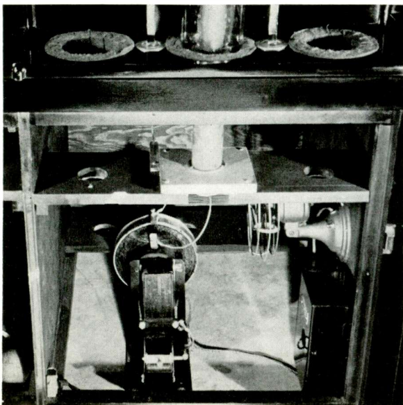
Below: The transformer compartment of the conditioner. Right: Operator closes the shorting bar across filament and grid.
