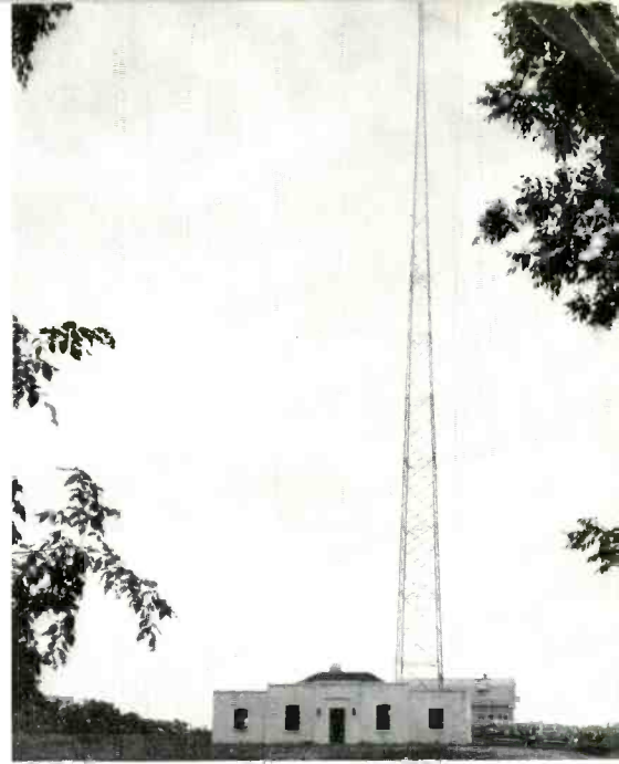
WKAR's 300-foot Blaw Knox shunt fed radiator.
