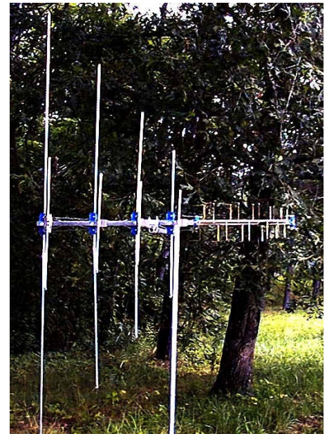
Grove Scanner Beam Antenna II could be the best performing inexpensive VHF antenna on the market. (Courtesy: Grove Enterprises)
