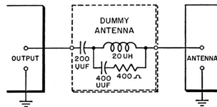
Fig. 1. Specifications for dummy antenna as originally recommended by the Radio Manufacturers' Association.
