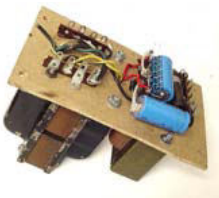
The power supply board is now almost ready to mount over the dynamotor well.
