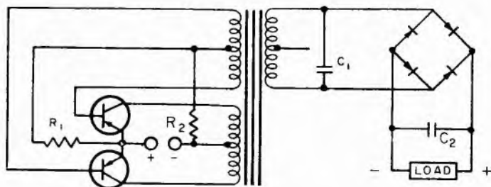
TYPICAL CIRCUIT
