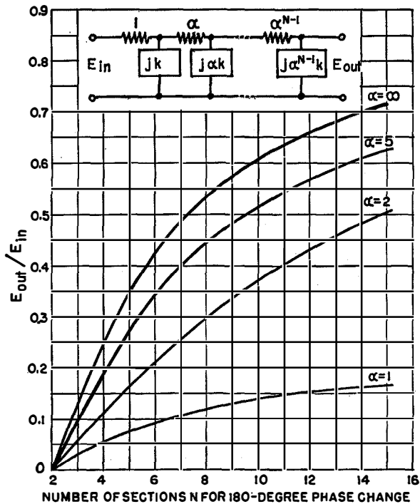
Figure 1—Attenuation characteristic as a function of the number of meshes required for a 180-degree phase change.
