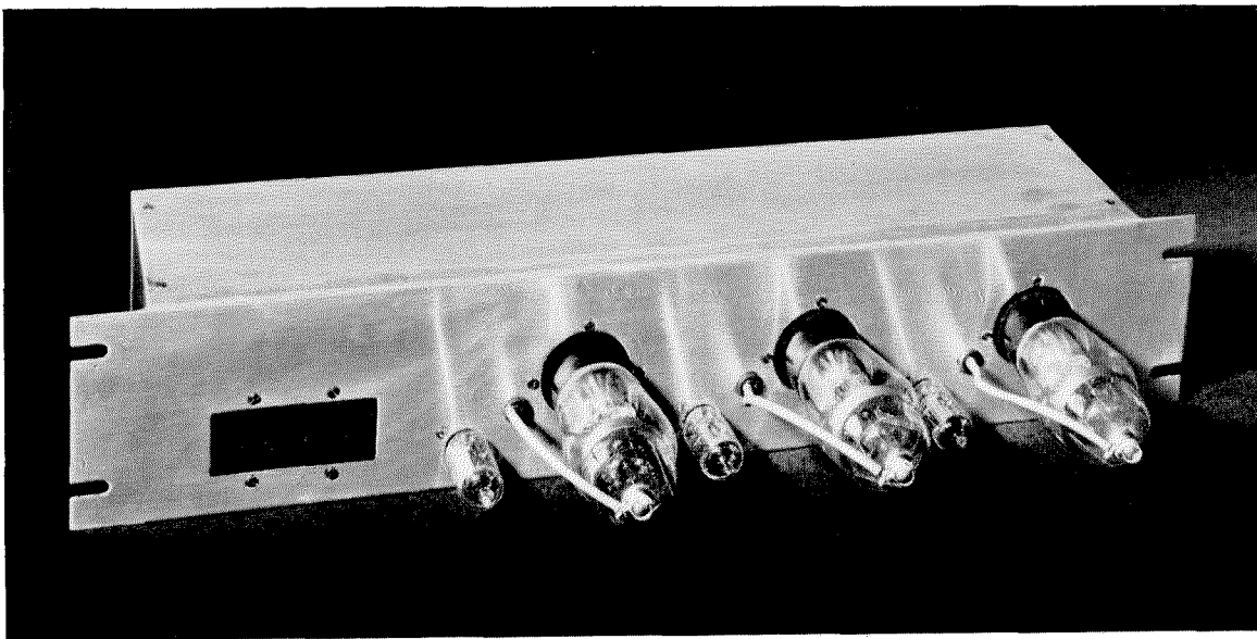
Figure 10—These three multicathode tubes and their associated trigger tubes will count to 1000.
