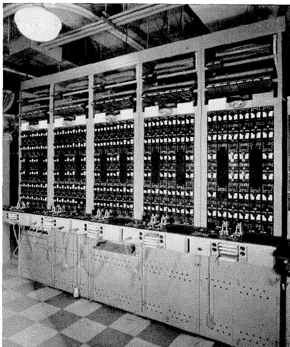
Voice-frequency carrier telegraph installation in a modern Western Union Telegraph Company office. Each vertical rack of carrier equipment (left) mounts 8 channels. The test board is at the right.
