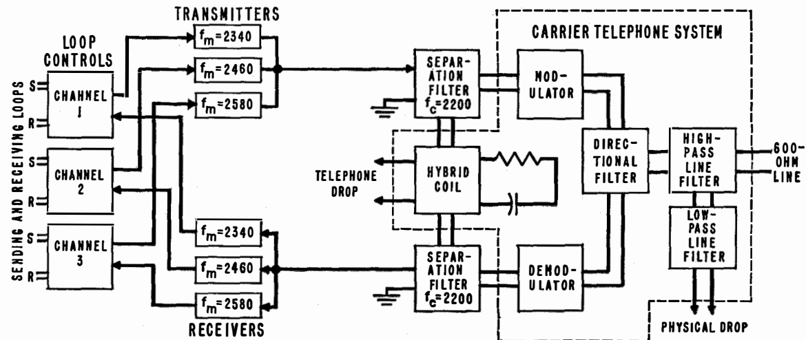
Figure 11—Speech-plus-3-duplex carrier telephone system applied to a carrier telephone system. The crossover frequency f_c of the separation filters is 2200 cycles.
