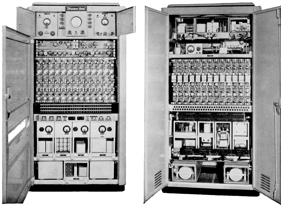
Transmitter and receiver cabinets of an ultra-high-frequency time-division-multiplex radio link supplying 24 telephone channels. This equipment may be set up to give over 500 teleprinter circuits.
