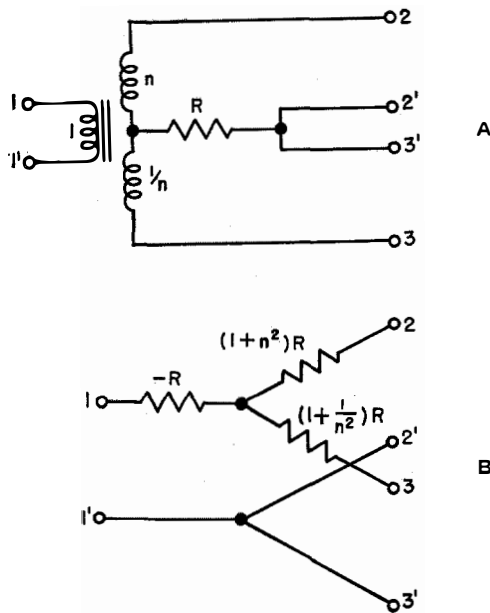
Figure 5—A—Hybrid coil. B—Equivalent circuit of A.
