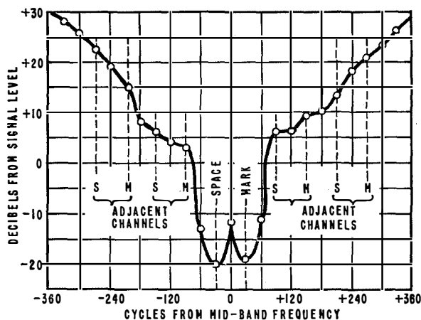
Figure 7—Curve showing level of single-frequency interference producing 4-percent distortion in a telegraph circuit at 75 words per minute.
