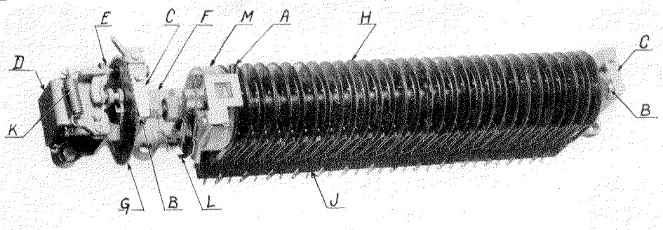
Figure 18—7101 Type Sequence Switch.
