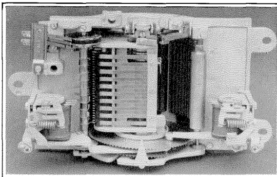
Figure 13—7120 Type Selector.
