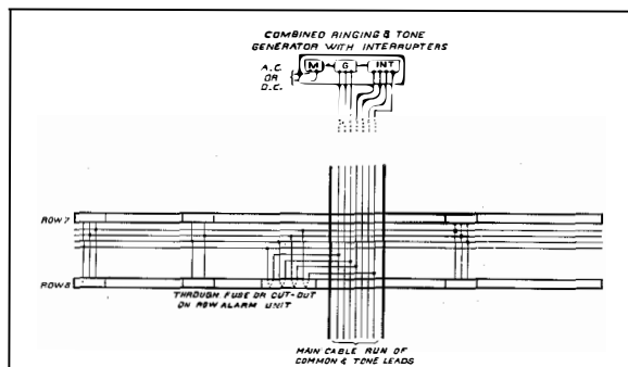
Figure 29—Schematic of Common Tone and Ringing Leads.
