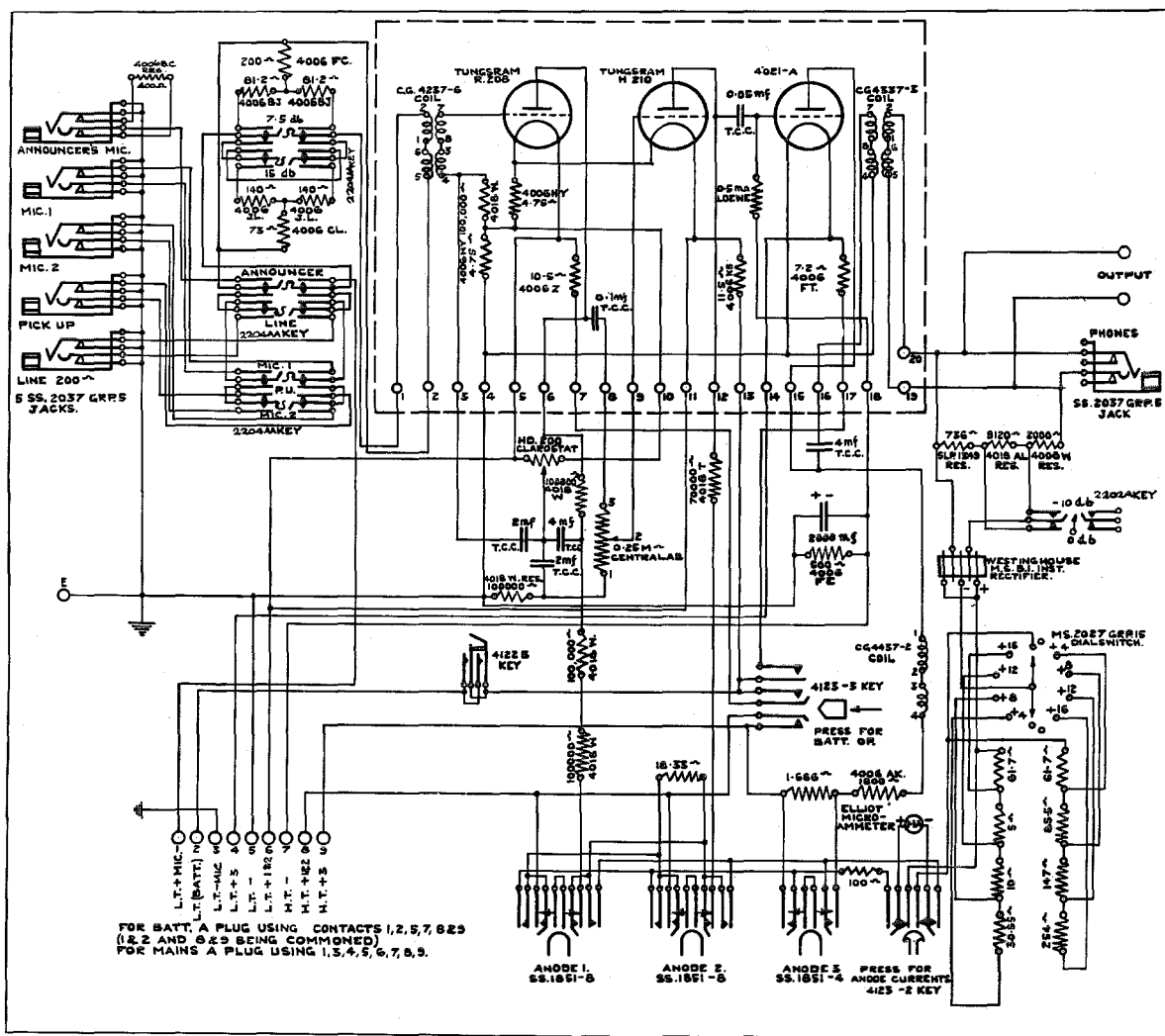
Figure 8A—Schematic of Outside Broadcast Amplifier M.S. 3029.
