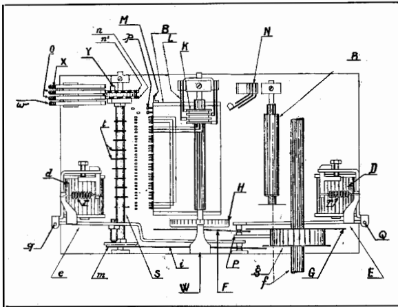
Figure 17—Diagram of New Type Selector.
