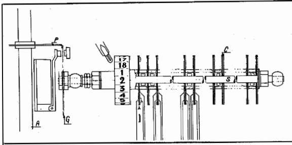
Figure 20—Schematic of Sequence Switch.
