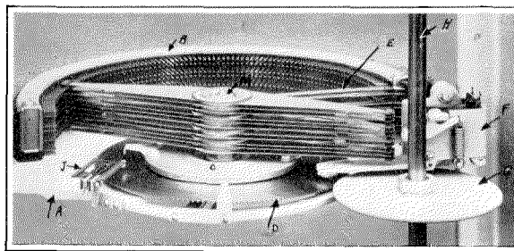
Figure 2—7200 Type Line Finder.
