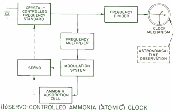
Fig. 12—Servo-controlled ammonia-absorption-cell oscillator systems.
