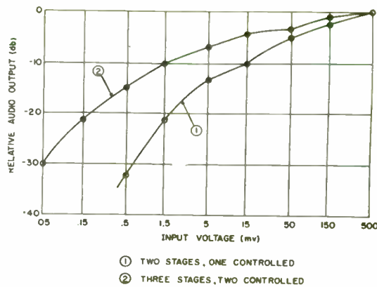
Fig. 18—AGC characteristics of IF amplifiers.
