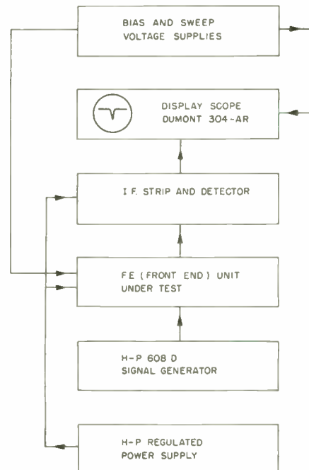
Fig. 1—Block diagram of wide-range dielectric tuned panoramic receiver.
