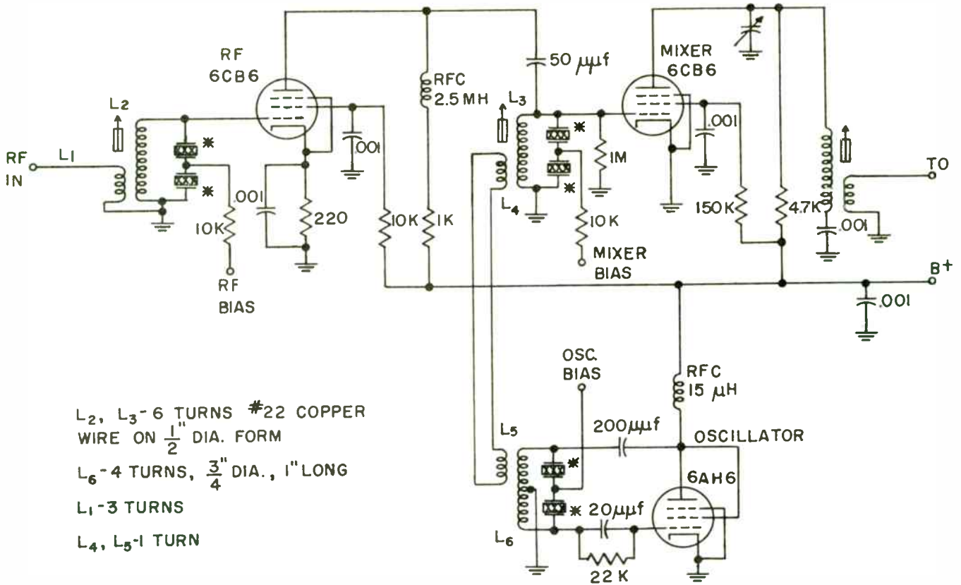
Fig. 7—Schematic of receiver front-end unit.
