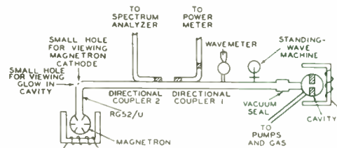
Fig. 9—Test setup used at high power levels and for gas-break-down tests.
