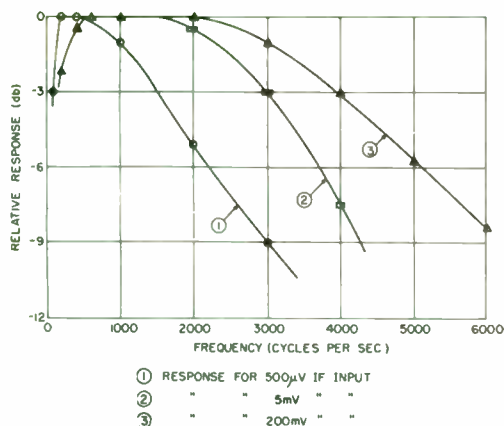
Fig. 22—Audio response of controlled IF amplifier-detector.
