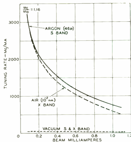
Fig. 15—Tuning rate as a function of beam current for spiral-beam tuning in gas atmospheres.
