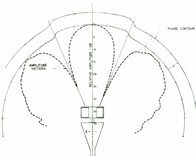
Fig. 4—Phase and amplitude plot of horn with septum.
