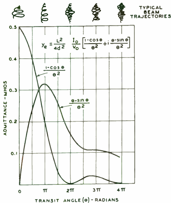
Fig. 2—Electronic admittance as a function of transit angle, \theta .
