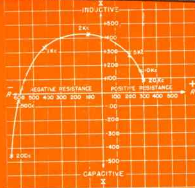
Plot of Impedance Z_1 of Feedback Circuit . . .
