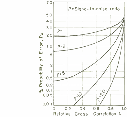
Fig. 3—Ambiguity of signals of unknown phase.
