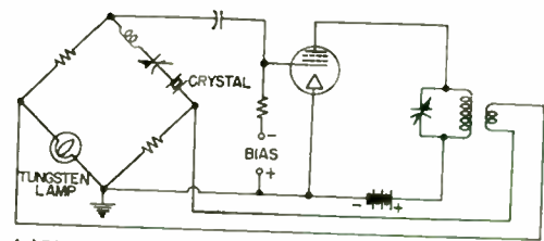
(a) BRIDGE STABILIZED OSCILLATOR (MEACHAM)
