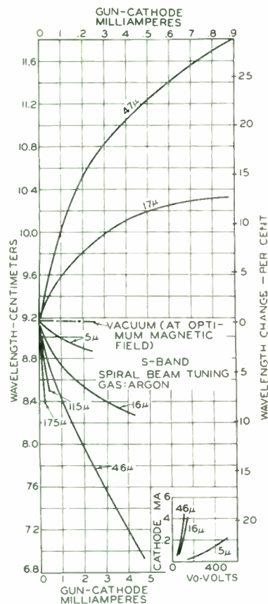
Fig. 14—Frequency as a function of gun-cathode current for a spiral-beam S-band cavity filled with argon at various pressures for two fixed values of magnetic field.
