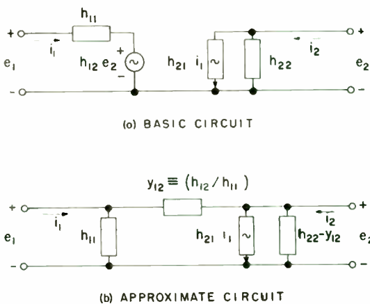
Fig. 6—Equivalent circuits for representation of a network by small-signal series-parallel h parameters; (a) Basic two-generator circuit, (b) Approximate one-generator circuit.
