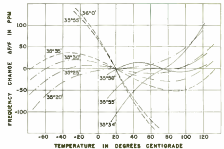
Fig. 1—Frequency-temperature characteristics of AT-cut crystals with different ZZ' angles fabricated from natural and aluminum-doped synthetic quartz. The solid curves are the characteristics for aluminum-doped crystals; the dashed curves for natural quartz having same ZZ' angles; and dot-dashed curves for natural quartz having similar frequency-temperature characteristics.
