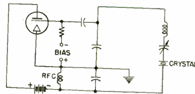
(b) GOURIET-CLAPP OSCILLATOR
