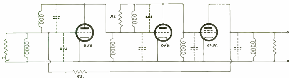
Fig. 2—Experimental amplifier showing ac connections only.
