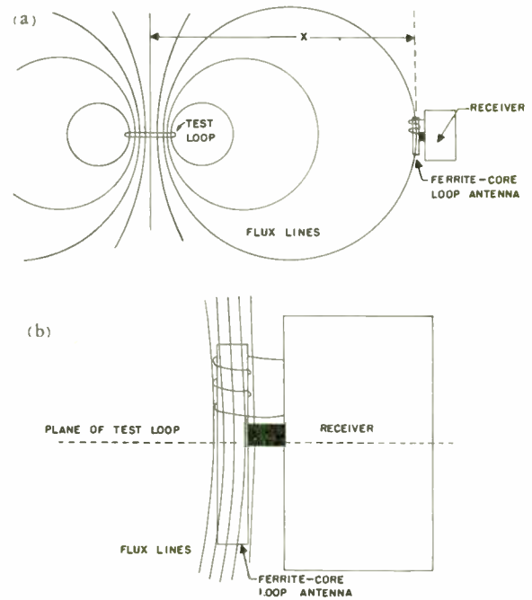
Fig. 2—Field configuration suitable for ferrite core loop antennas.
