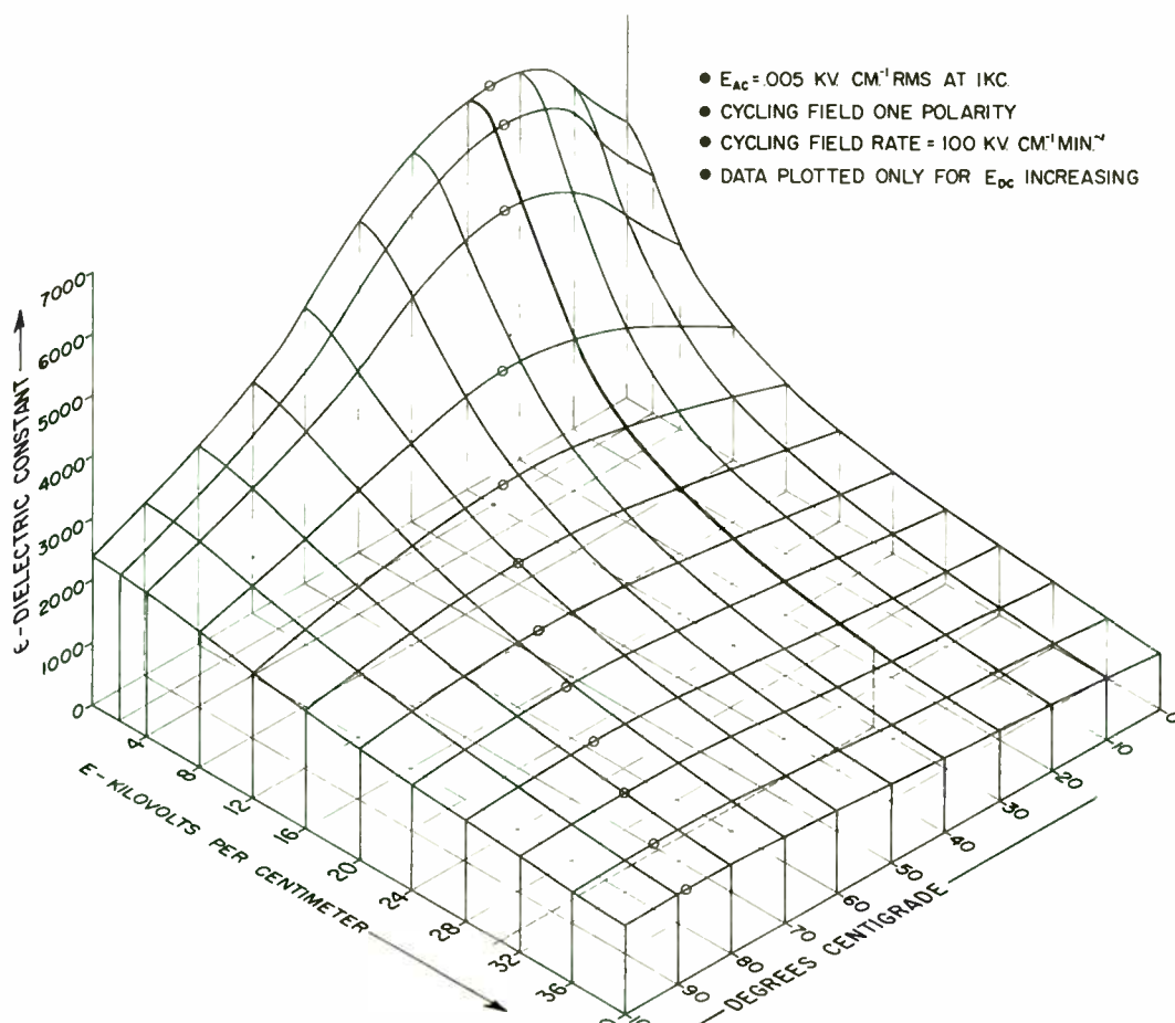
Fig. 2— \epsilon - T - E surface for aerovox Hi-Q 41.
