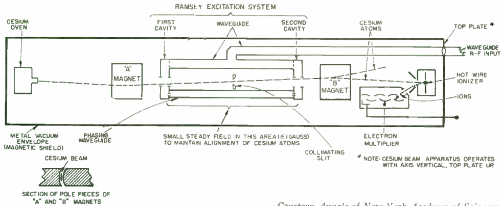
Fig. 17—Cesium atomic-beam frequency-standard apparatus.
