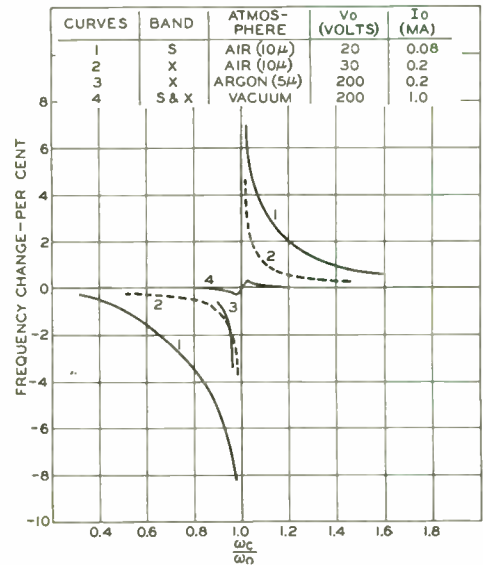
Fig. 13—Frequency change as a function of magnetic-field density for spiral-beam tuning in gas atmospheres, and comparison to results with vacuum.
