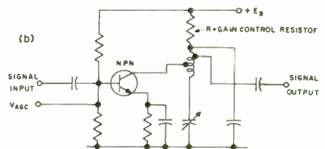
Fig. 15—Indirect V_c -control of tuned amplifier with AGC voltage applied to base.
