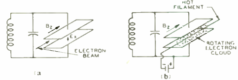
Fig. 1—(a) Schematic representation of resonant cavity using spiral-beam tuning. (b) Schematic representation of resonant cavity using space-charge tuning.
