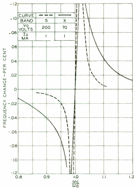
Fig. 11—Frequency change as a function of magnetic-field parameter for spiral-beam tuning in vacuum.
