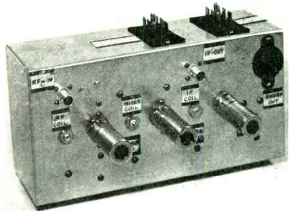
Fig. 5—Exterior view of a front-end unit.
