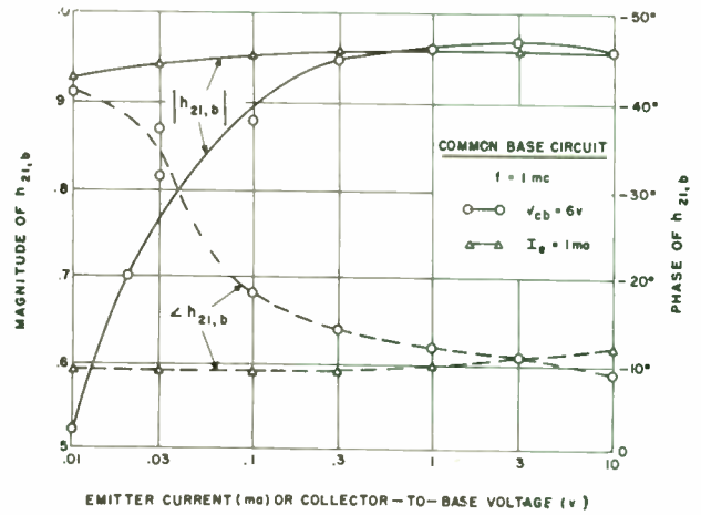
Fig. 6— h_{21,b} as function of emitter current and collector-to-base voltage.
