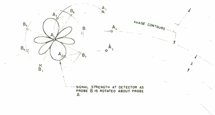
Fig. 3—Diagram illustrating the procedure of plotting phase contours.
