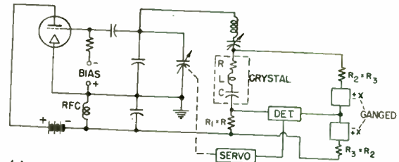
(c) SERVO-CONTROLLED (LEA)
