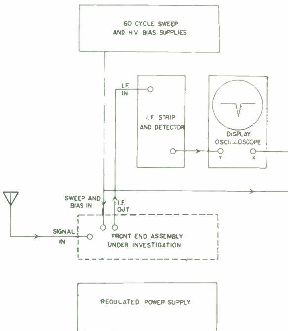
Fig. 4—Block diagram of receiver.
