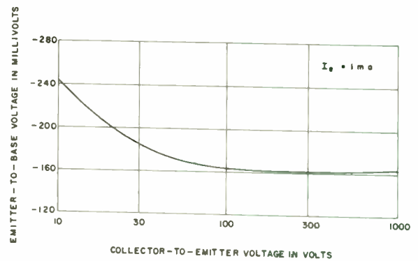
Fig. 7—Emitter-to-base versus collector-to-emitter voltage at constant emitter current.
