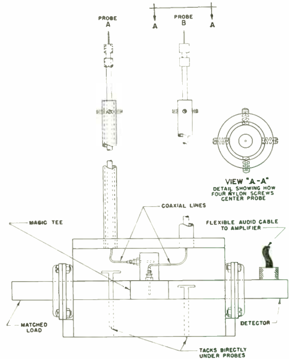
Fig. 2—Sketch of phase contour plotter.
