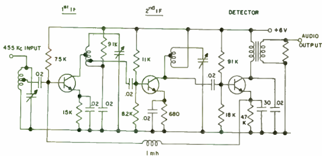
Fig. 17—Two stage IF amplifier followed by detector with V_c type AGC.
