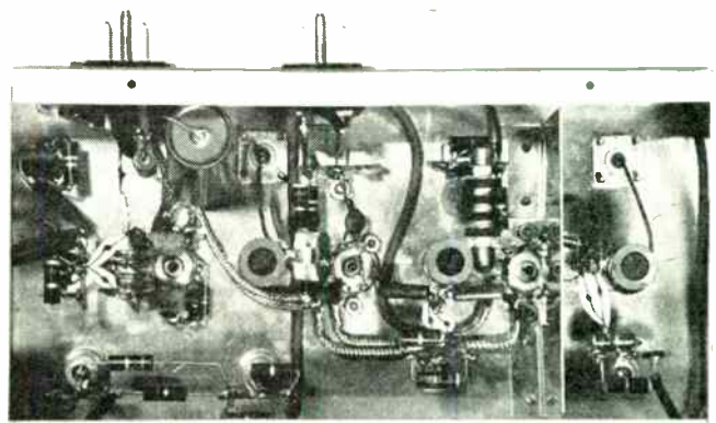
Fig. 6—Interior view of a front-end unit.
