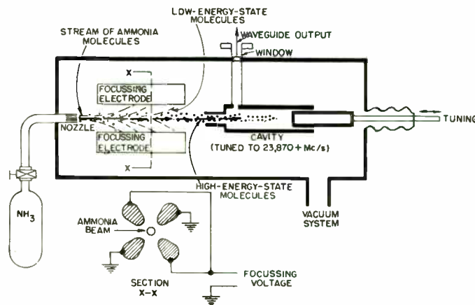
Fig. 16—Ammonia oscillator (Townes).
