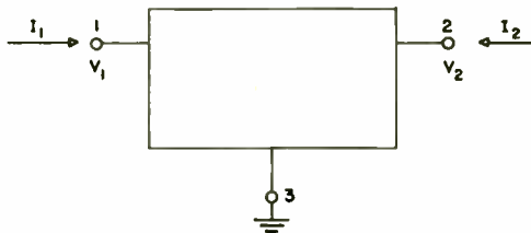
Fig. 1—The general 3-terminal element.
