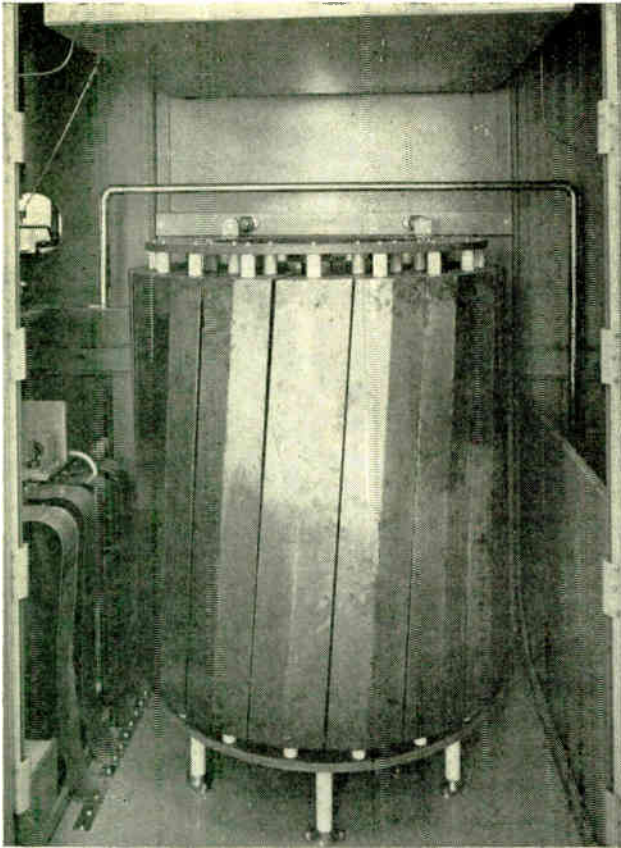
Fig. 11—Output tank inductor is high-current toroid.
