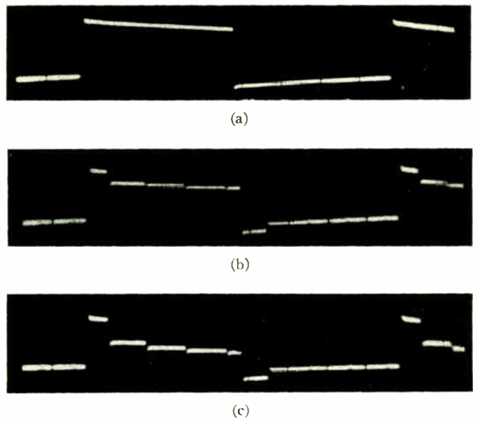
Fig. 11—Flux in the z direction for different values of the sensing current I_y : a. I_y = 70\text{mA} , b. I_y = 750\text{mA} , c. I_y = 1.5\text{A} .
