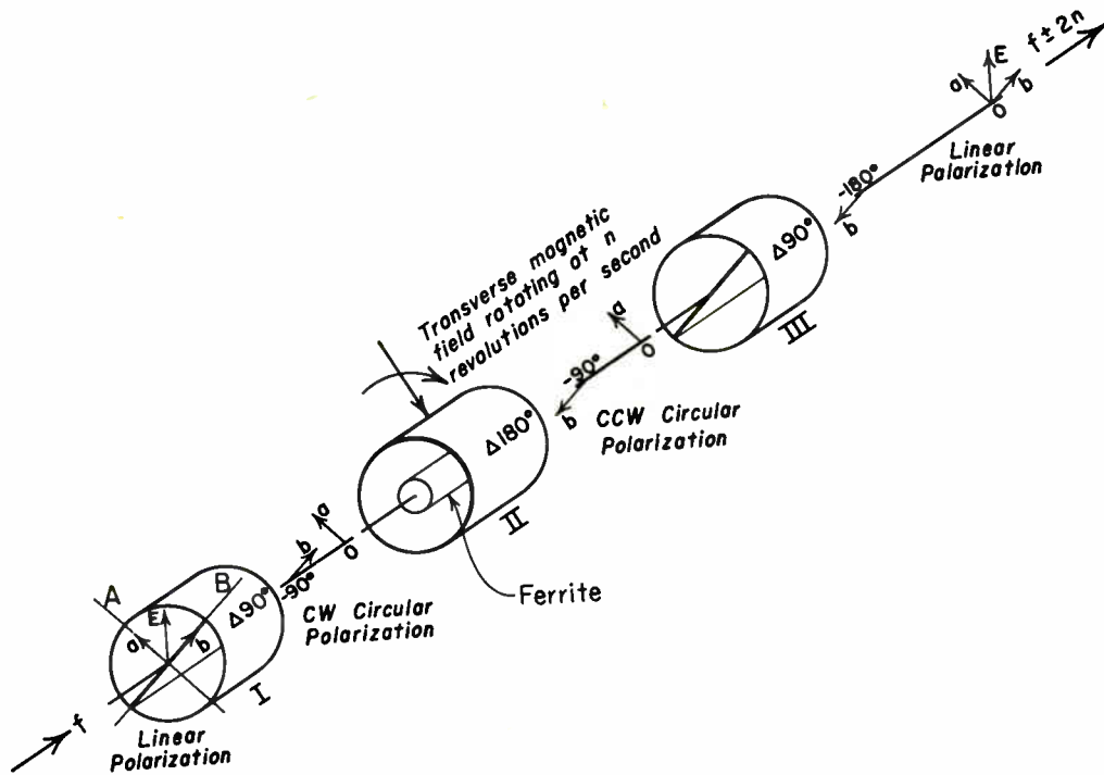
Fig. 1—Microwave single-sideband modulator.
