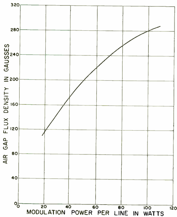
Fig. 7—SSM magnet characteristic.
