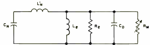
Fig. 3—Equivalent circuit of pulser.
