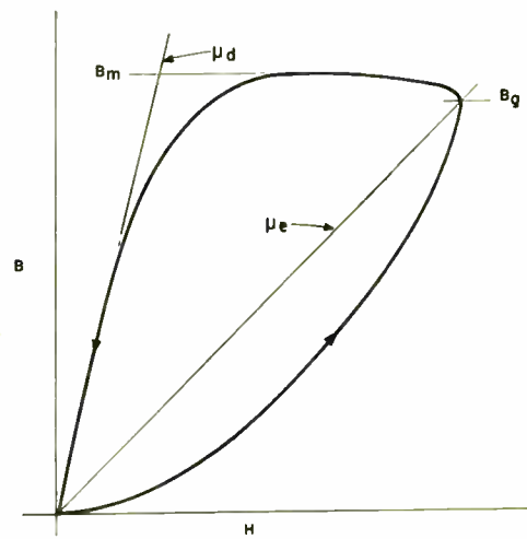
Fig. 4—Pulse permeability.
