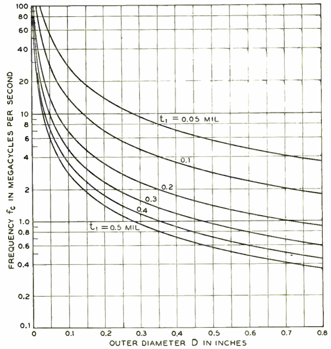
Fig. 6—Characteristic frequency f_c as a function of cable diameter and conductor thickness.
