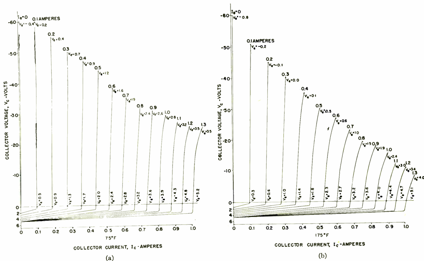
Fig. 5—Transistor characteristics for ambient temperatures of (a) 75 degrees F. and (b) 175 degrees F. with the mounting base connected to an "infinite" heat sink.
