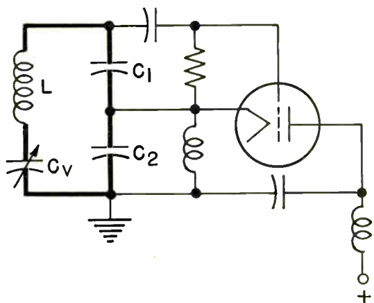
Fig. 1—Gouriet-Clapp.
