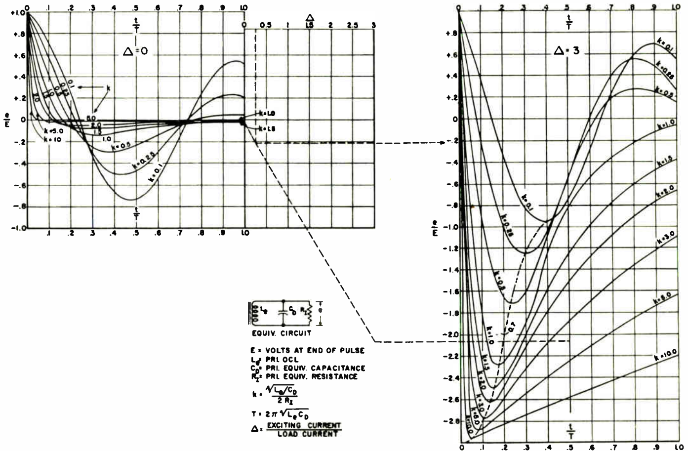
Fig. 7—Interpolation chart for finding backswing amplitude.
