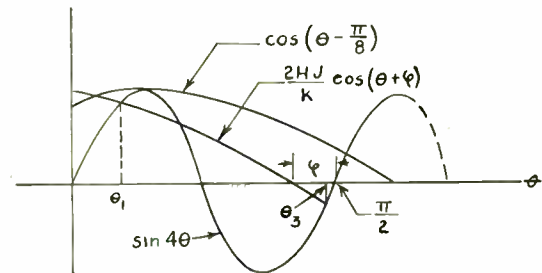
Fig. 7—Graphical solution of (19); upper curve for \phi = -(\pi/8) and H = K/2j .
