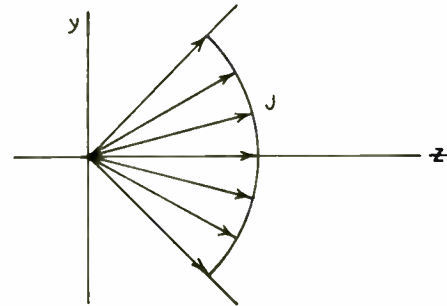
Fig. 5—Distribution of domains of a material magnetized in the z direction.
