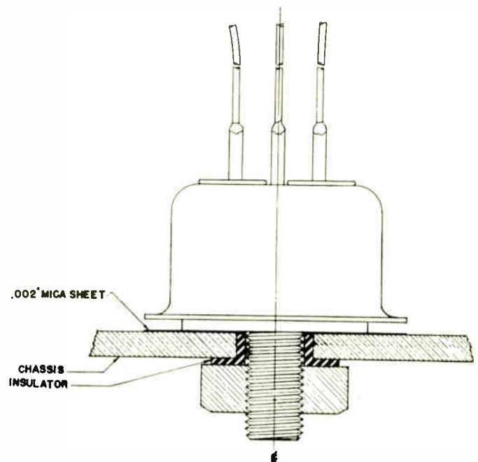
Fig. 3—A simple way of mounting transistor on chassis for effective heat transfer. A mica sheet, 2 mils thick, and a positioning ring insulate, electrically, transistor from chassis. Effective heat transfer is possible through the mica sheet to chassis.
