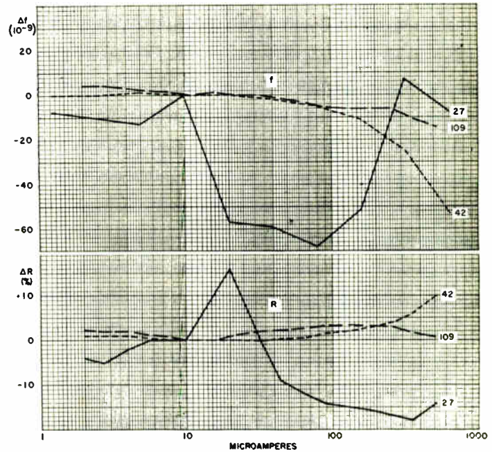
Fig. 5—Frequency and resistance variation versus crystal current for three GT crystal units.
