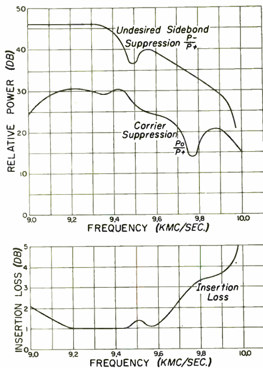
Fig. 11—Frequency characteristic of SSM (reflection type).
