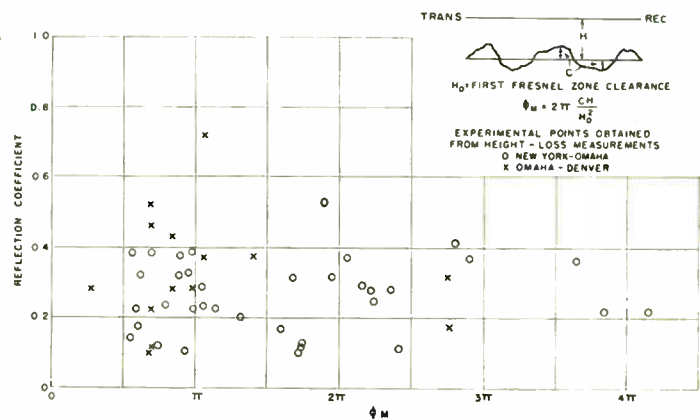
Fig. 3—Reflection coefficients of irregular terrain, 4,000 mc.
