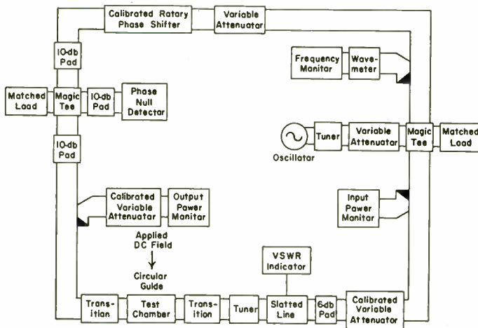
Fig. 2—Block diagram of the experimental setup.
