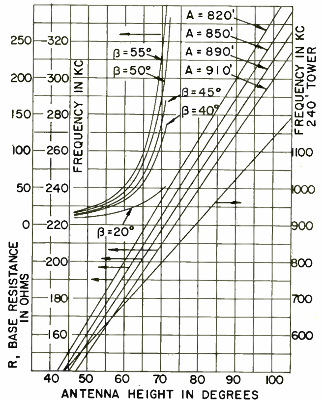
Fig. 18—Base resistance for various values of top-loading angle \beta for 8 umbrella cables.
