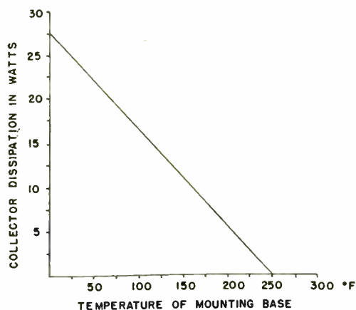
Fig. 4—The maximum collector heat dissipation of the transistor as a function of the base temperature of the transistor shell.
