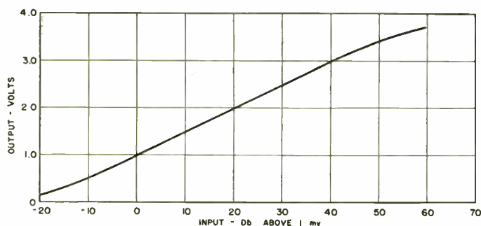
Fig. 6—Amplitude response of narrow-band logarithmic receiver.
