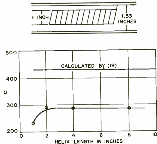
Fig. 4—Experimental and calculated values of Q versus helix length. In the experimental helix, Nd = 1/3 and there were 116 turns with one end connected to the outer conductor.
