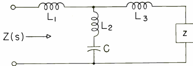
Fig. 1—A Brune cycle with an ideal transformer. Case L_1 > 0
