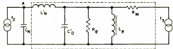
Fig. 9—Equivalent network for close false echoes.
