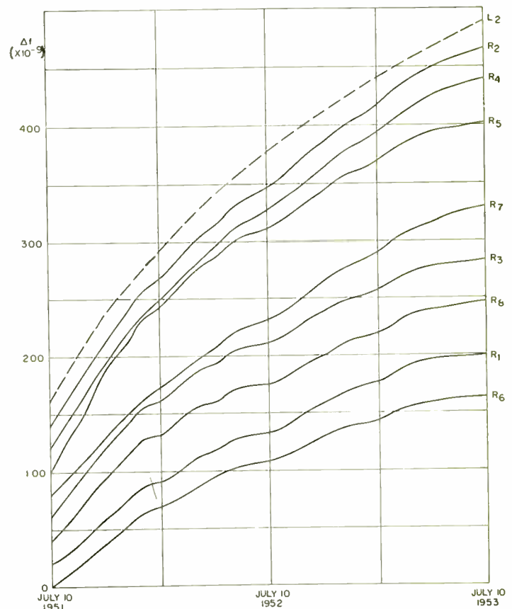
Fig. 6—Frequency drift based on absolute values for eight resonator crystals and computed logarithmic drift for one unit (dashed curve). \Delta f , expressed in parts in 10^9 , indicates change from the fundamental frequency.
