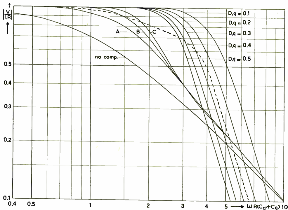
Fig. 2—Gain-frequency characteristics of the constant gain compensation of the various networks. The dotted line gives the gain-frequency characteristic of the 1 per cent tolerance compensation of network D, q=0.5 .
