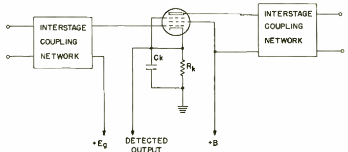
Fig. 2—The basic nonamplified back-biased stage of the logarithmic receiver.
