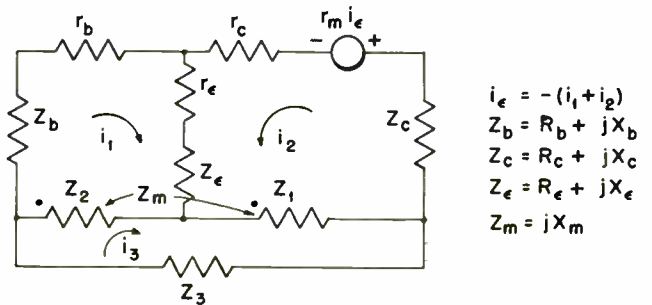
Fig. 2—Generalized equivalent circuit for the Hartley and Colpitts transistor oscillators.
