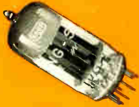
6AU7 (Prototype—12AU7) Heater Volts 3.15* Heater Current 0.6 A
