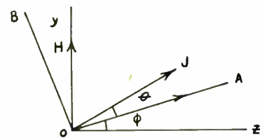
Fig. 6—Rotation of the domain J by an angle \theta , upon application of a field in the y direction; OA, OB crystal axes.
