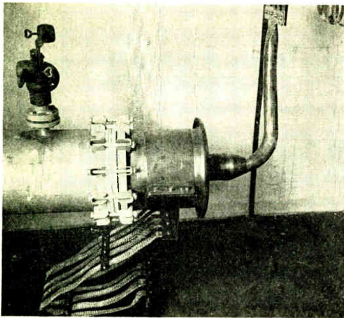
Fig. 16—Concentric-line termination in tuning-house.
