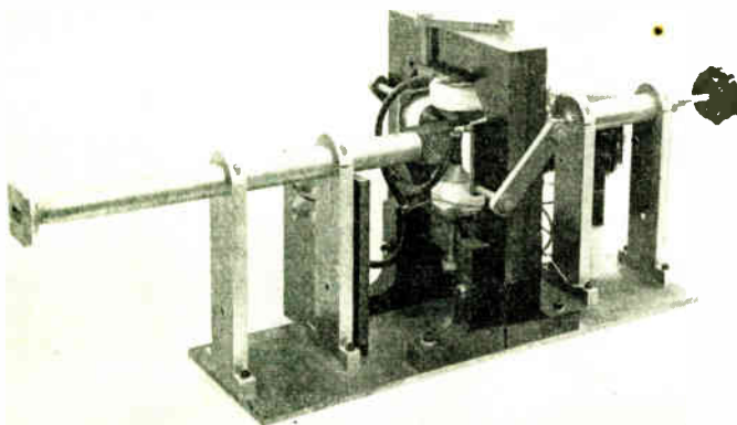
Fig. 8—Microwave single-sideband modulator (reflection type).
