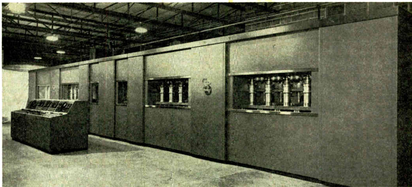
Fig. 5—Front view of million-watt transmitter and control console.
