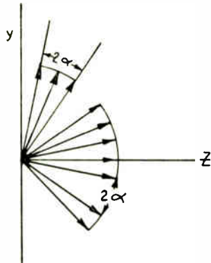
Fig. 8—Distribution of domains after H , satisfying the inequality (20), is removed.
