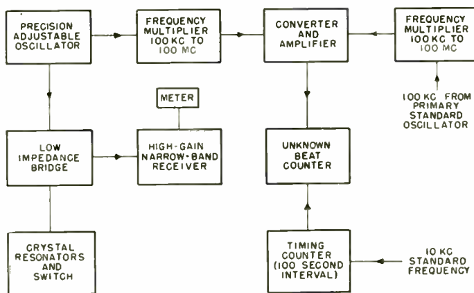
Fig. 2—Block diagram of resonator measuring equipment.
