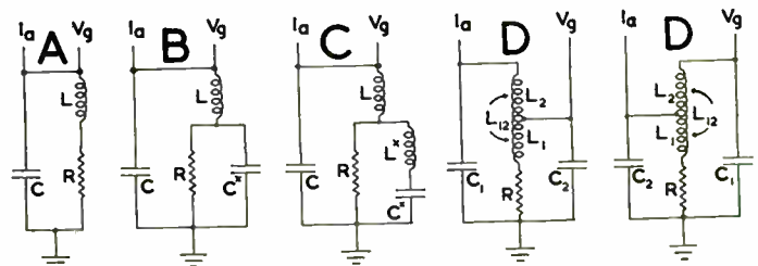
Fig. 1—Investigated networks.
