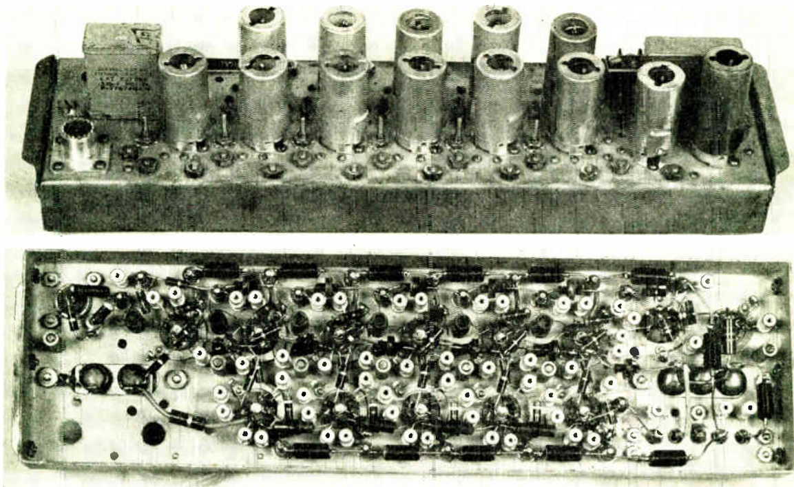
Fig. 4—Narrow-band logarithmic receiver.
