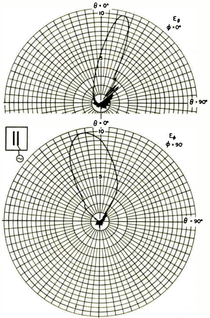
Fig. 5—Measured patterns of the tapered-depth slot radiating in the presence of an adjacent parasitic slot (one wavelength spacing).
