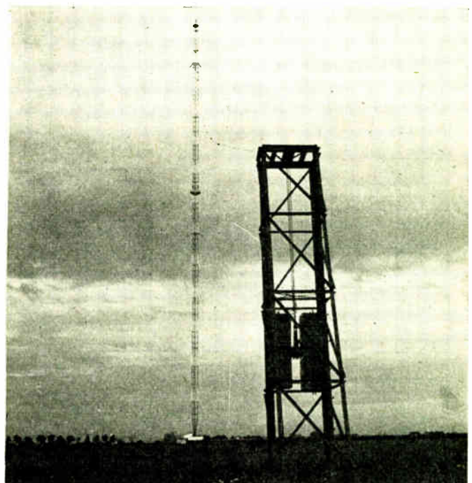
Fig. 25—Counterweight "A" frame to support top-loading cable.
