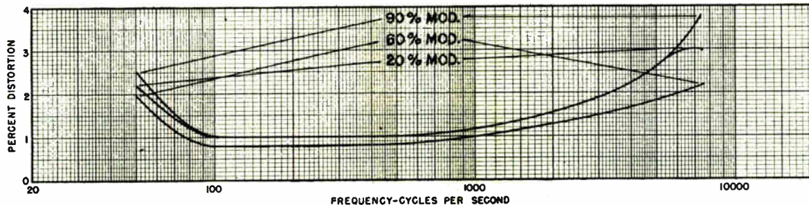
AUDIO FREQUENCY HARMONIC DISTORTION
