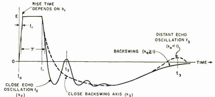
Fig. 6—Oscillations on pulse backswing.
