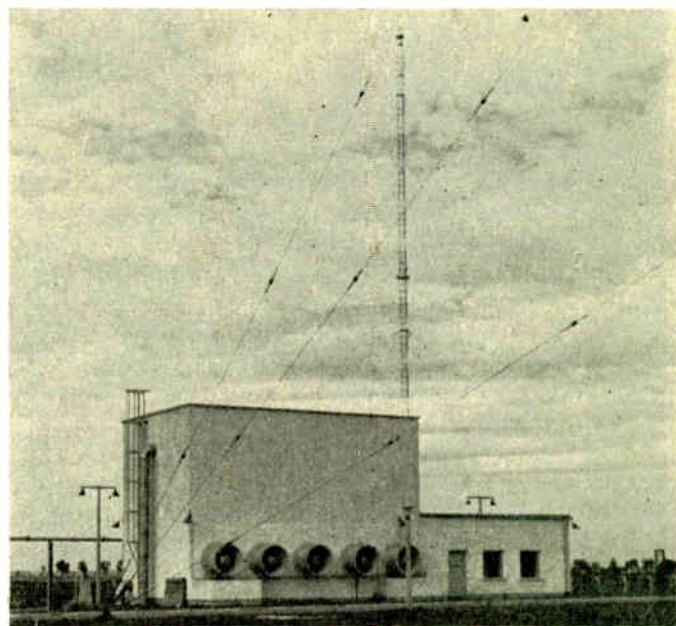
Fig. 4—Cooling tower capable of dissipating 20 million BTU per hour of heat from the transmitter and diesel engines.
