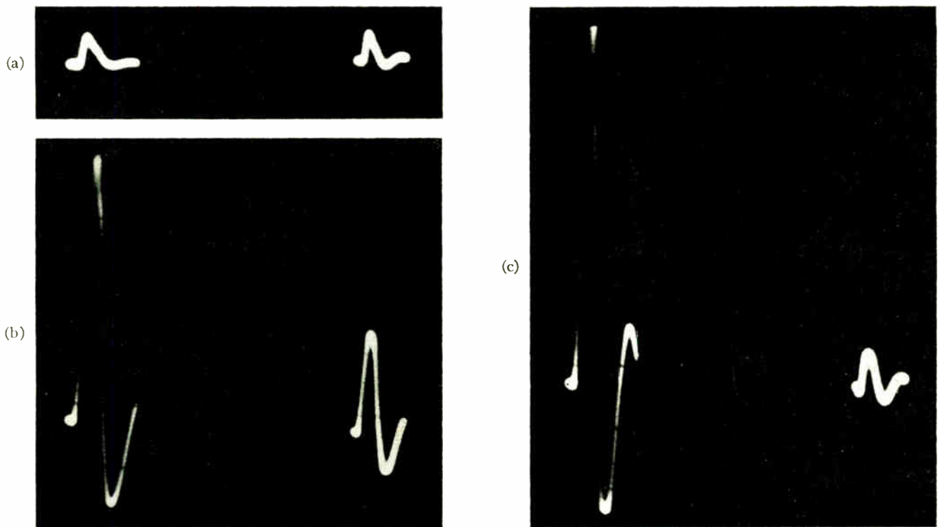
Fig. 12—Output voltage e(t) for different values of the sensing current I_y : a. I_y = 280\text{mA} , b. I_y = 570\text{mA} , c. I_y = 850\text{mA} . curves to the left: for first application of I_y . Curves to the right: for second application of I_y .
