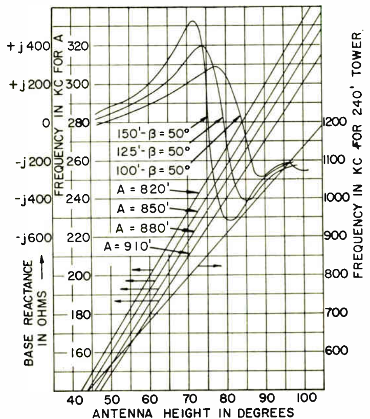
Fig. 22—Base reactance for various lengths of 12 top-loading cables in terms of antenna height.
