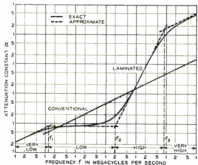
Fig. 2—Schematic plots of the attenuation constants of a laminated cable and a conventional air-filled coaxial cable of comparable size. Shading indicates the region in which the laminated cable has lower attenuation than the conventional cable.
