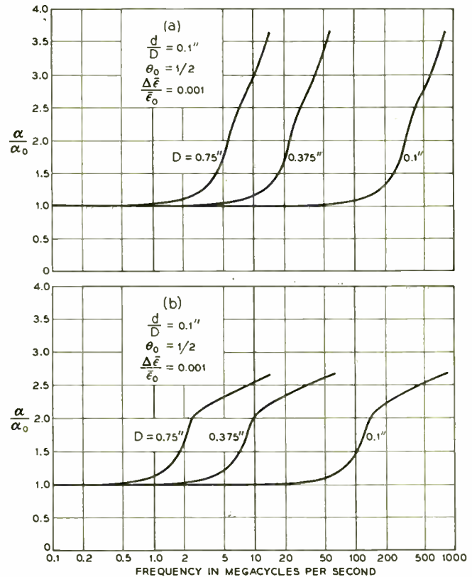
Fig. 10—Normalized attenuation of nonuniform Clogston cables of various diameters with 0.1 per cent total variation in \bar{\epsilon} : (a) linear variation, and (b) step-function variation.
