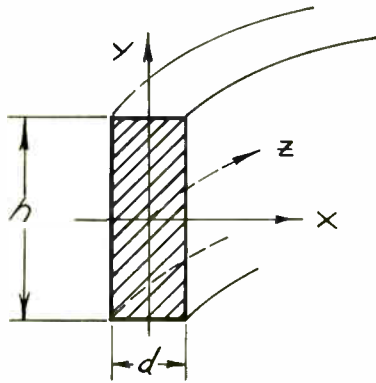
Fig. 1—Cross section of the magnetic material.
