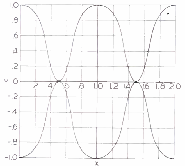
Fig. 4—Outline of cosine phase-converter mask.
