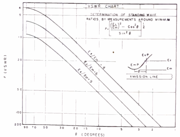
Fig. 2—Voltage-standing-wave-ratio chart.
