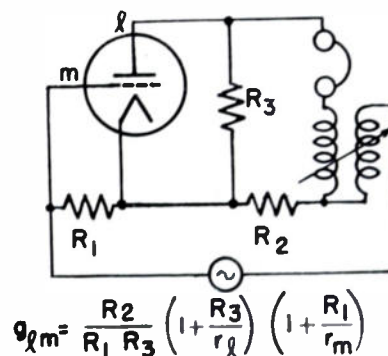
Fig. 49—Basic resistance-balance circuit for measuring transconductance.
