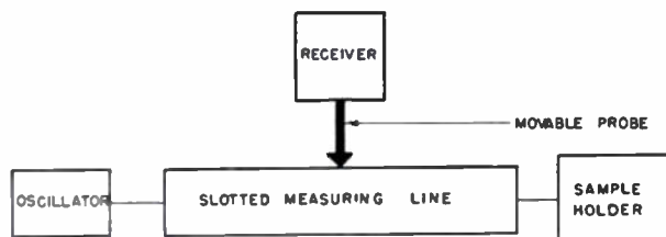
Fig. 3—Block diagram of measuring equipment.
