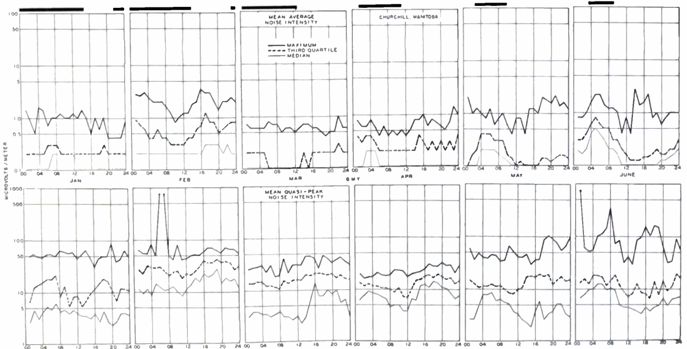
Fig. 5—Hourly mean average and mean quasi-peak noise intensity (January through June, 1947), Churchill, Manitoba.
