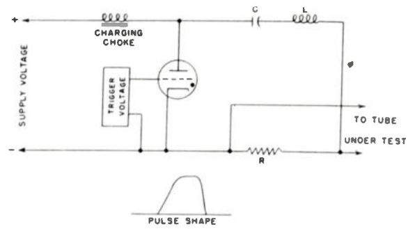
Fig. 20—Basic circuit arrangement for gas-tube LC pulse generator.
