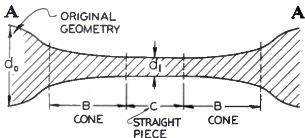
Fig. 5—Axial view of drawn-down geometry (scale distorted).
