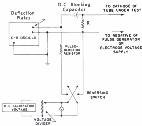
Fig. 24—Cathode-ray-oscillograph current indicator.
