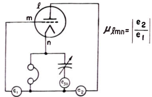
Fig. 55—Basic voltage-ratio circuit for measuring \mu factor.
