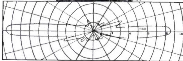
VERTICAL RADIATION PATTERN OF TYPE 3000 ANTENNA
