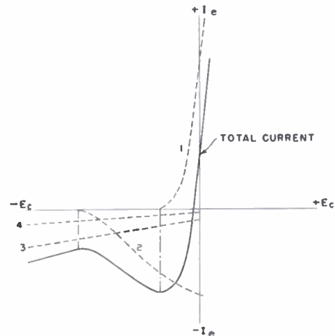
Fig. 27—Total grid current and its components. Curve 1—Electrons from the cathode that reach the grid by virtue of contact potentials and initial velocities. Curve 2—Ionization current. Curve 3—Leakage current. Curve 4—Electron emission from the control grid.
