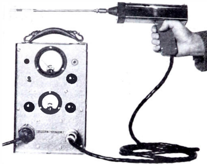
Fig. 8—The head and control unit of a leak detector.
