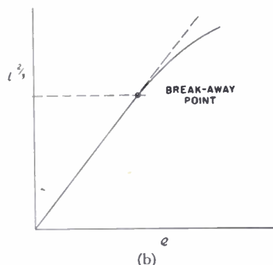
Fig. 10—Determination of emission break-away point.
