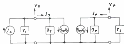
Fig. 36—Low-frequency equivalent circuit of a triode.
