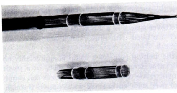
Fig. 6—Tungsten-quartz cage-grid combination, real diameter, 1.2 mm.
