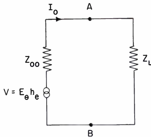
Fig. 12—Equivalent circuit of receiving antenna. Z_L = load impedance Z_{00} = R_{00} + jX_{00} (self-impedance of antenna) E_0 = incident electric field h_e = effective height of antenna.
