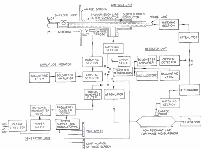
Fig. 2—Block diagram of measuring setup.
