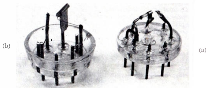
Fig. 3—Experimental fieldistor models, mounted on standard octal tube bases. (a) Spacer-type fieldistor. (b) Line-contact type, wax sealed.
