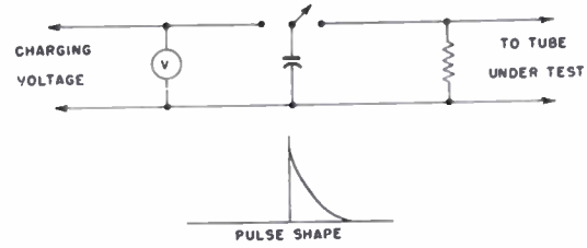
Fig. 18—Basic circuit arrangement for capacitor-discharge pulse generator.
