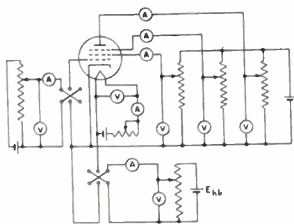
Fig. 13—Circuit arrangement for measuring static characteristics.
