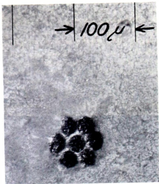
Fig. 11—7-electrode configuration, top view ( 25\mu wires).
