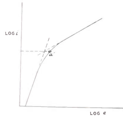
Fig. 7—Determination of flection-point emission current, slope-intersection method.
