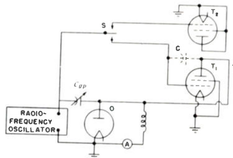
Fig. 46—Circuit arrangement for measuring interelectrode capacitance by Substitution Method B.
