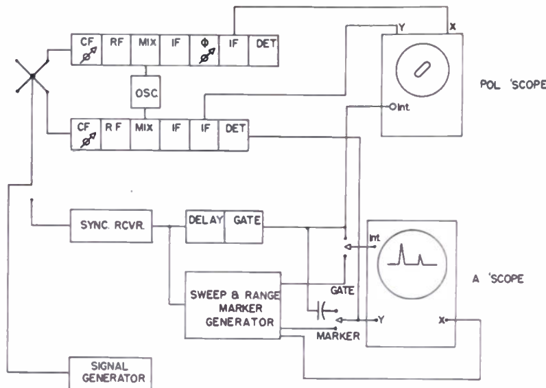
Fig. 1—Block diagram of polarimeter.
