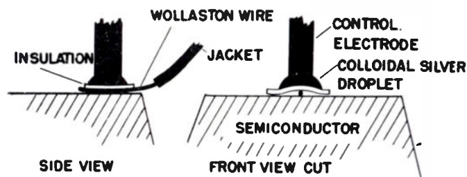
Fig. 2—Line-contact fieldistor arrangement.
