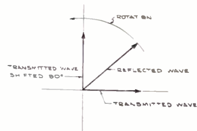
Fig. 7—Vector relationships in the sense detector.
