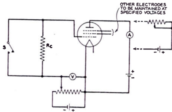
Fig. 29—Circuit arrangement for measuring small control-grid currents.
