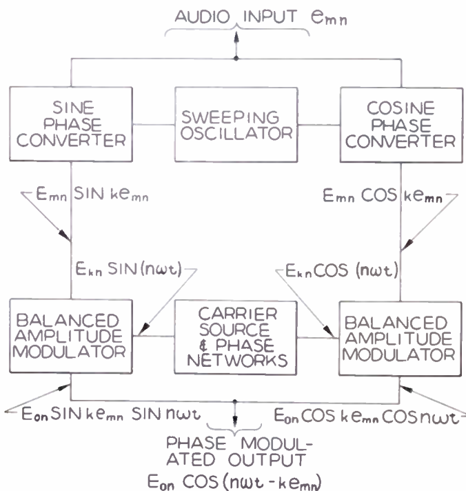
Fig. 3—Block diagram of product phase-modulation system.
