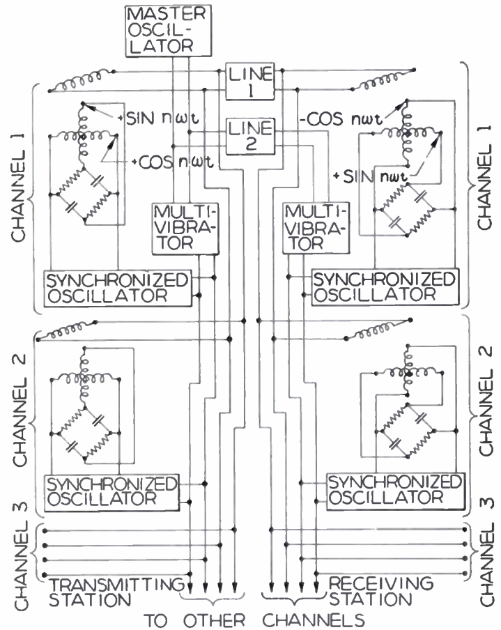
Fig. 1—Block diagram of multichannel synchro system.
