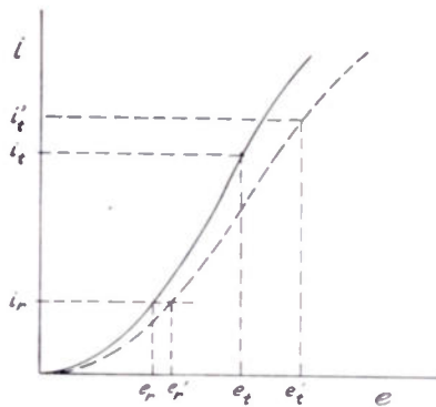
Fig. 11—Comparison of the emission currents of electron tubes.
