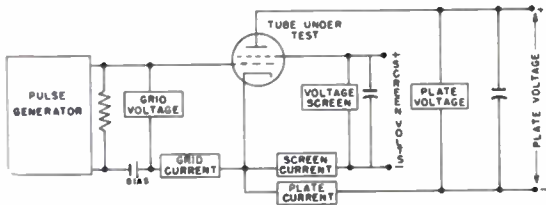
Fig. 16—Circuit arrangement for pulse measurement of tube characteristics, single-generator method.
