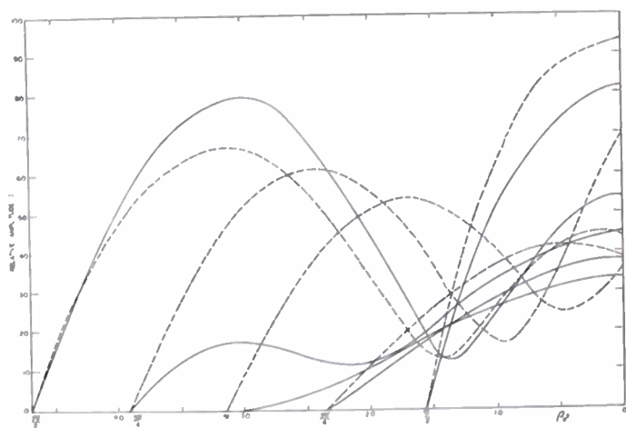
Fig. 14—Current distribution on receiving antenna. — Z_L = 0 - - - Z_L = X_{00}^* with E_{incident} = \text{constant} .
