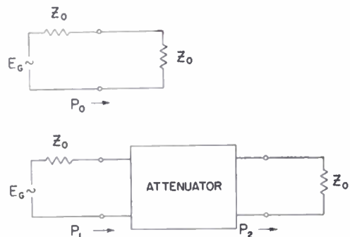
Fig. 1—Insertion loss in a matched system. A_T = 10 \log_{10} (P/P_2) .
