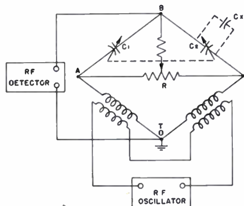
Fig. 43—Circuit arrangement for radio-frequency bridge for measuring interelectrode capacitances.
