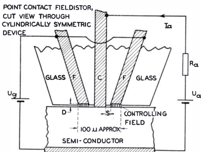
Fig. 1—Schematic diagram of point-contact-type fieldistor.
