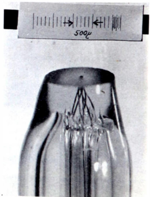
Fig. 10—7-electrode microspacer.
