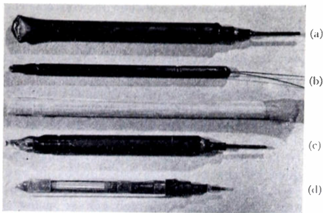
Fig. 15—Subminiature tubes, with match for comparison.
