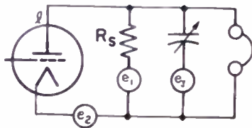
Fig. 53—Basic voltage-ratio circuit for measuring electrode resistance.
