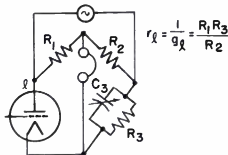
Fig. 48—Basic bridge circuit for measuring electrode resistance.
