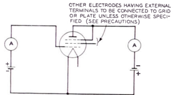
Fig. 30—Circuit arrangement for measuring gas current, ionization-gauge method.
