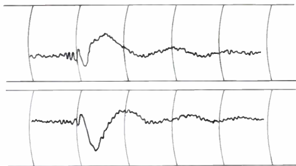
Fig. 8—Doppler beats demonstrating technique of determining sign of shift.
