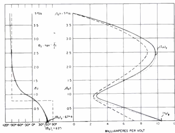
Fig. 9—Comparison of measured and theoretical current distribution, h = 5/8\lambda . ——— Second order (approximate); - - - - first order \Omega = 10 ; ····· experimental \Omega = 11.94 .
