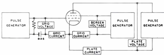
Fig. 17—Circuit arrangement for pulse measurement of tube characteristics, multiple-generator method.
