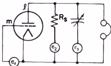
Fig. 53—Basic voltage-ratio circuit for measuring electrode resistance.
