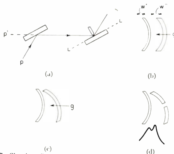
Fig. 7—Showing effect of stop pin and tilt of work crystal for double-crystal goniometer. (a) No-tilt, stop-pin centers work crystal. (b) Part of radiation cone of width W'' about to be swept by acceptance cone for case (a). (c) How a tilted acceptance cone would sweep the radiation cone to produce a broadened peak. (d) A gap in the acceptance cone produces a double peak on passing through the radiation cone.
