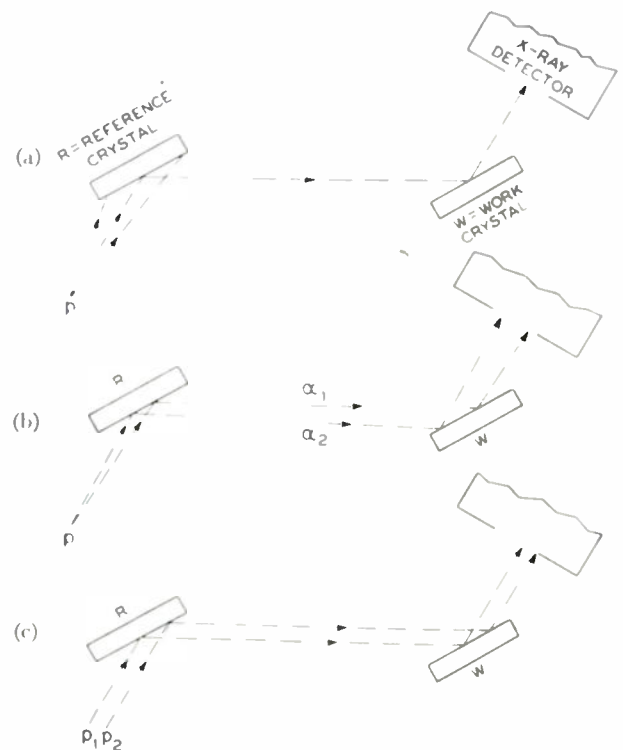
Fig. 3—X-ray reflections in double-crystal goniometer.
