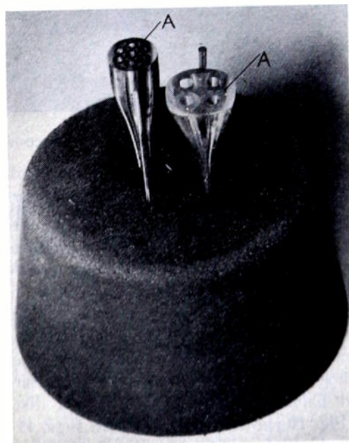
Fig. 7—Pyrex spacers with antimony (A) codrawn electrodes.
