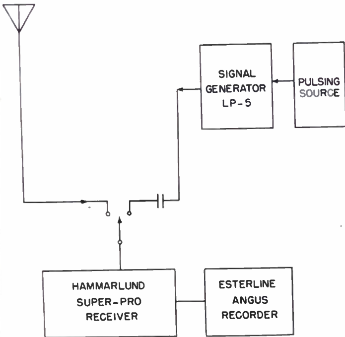
Fig. 3—Block diagram of arrangement of equipment.
