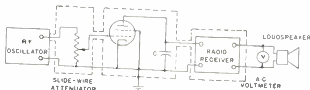
Fig. 47—Circuit arrangement for measuring interelectrode capacitance by Substitution Method C.
