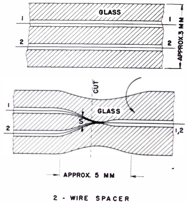
Fig. 9—Manufacturing of extremely small radial distances.
