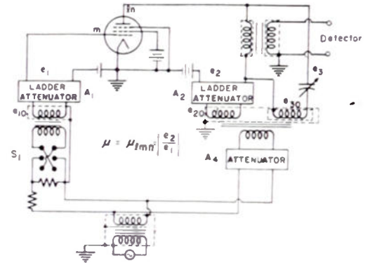
Fig. 56—Detailed voltage-ratio circuit for measuring \mu factor.
