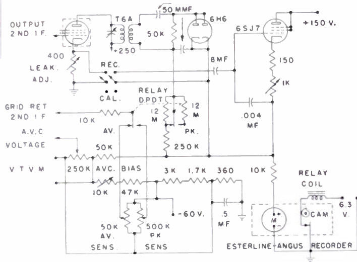
Fig. 2—Receiver circuit diagram.
