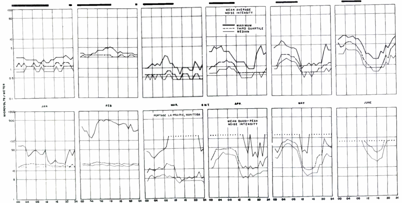
Fig. 9—Hourly mean average and mean quasi-peak noise intensity (January through June, 1947), Portage la Prairie, Manitoba.
