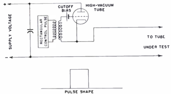
Fig. 19—Basic circuit arrangement for high-vacuum-tube pulse generator.
