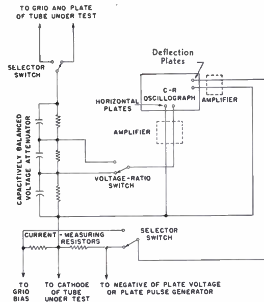
Fig. 25—Cathode-ray-oscillograph voltage and current indicator.
