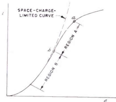
Fig. 6—Typical diode characteristic.
