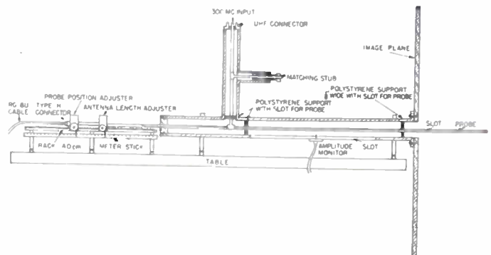
Fig. 1—Schematic diagram of measuring line.
