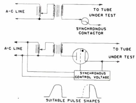
Fig. 22—Basic circuit arrangement for sine-wave-type pulse generator.
