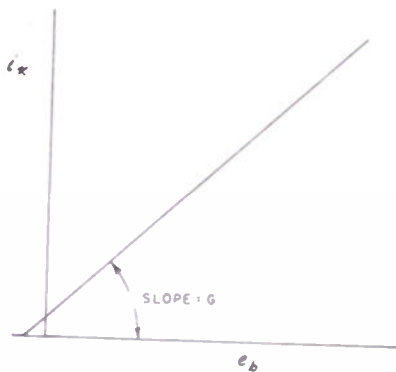
Fig. 14 Determination of the perveance of an electron tube from a 3/2 plot.
