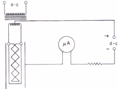
Fig. 6—Elementary circuit of the leak detector.
