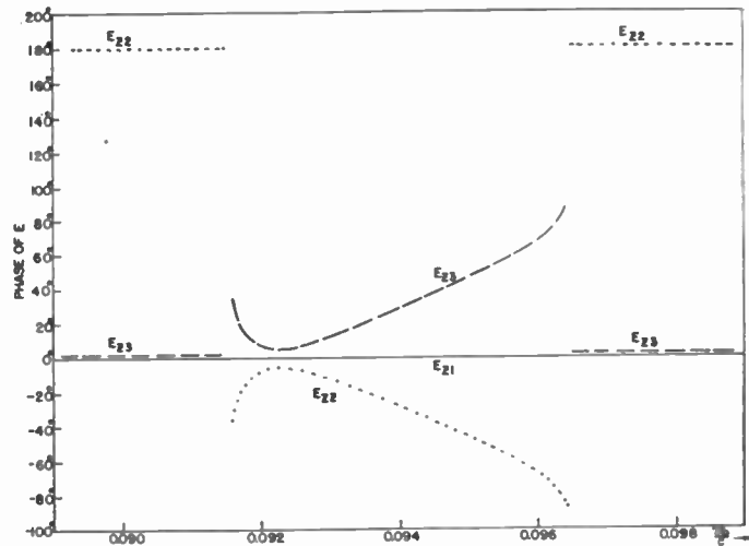
Fig. 10—Initial relative phases of the three component axial electric fields as functions of the average electron velocity ( v_0 ). I=10^{-3} amp.
