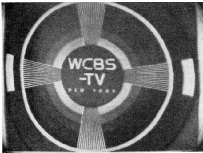
Fig. 9—Test shot to determine the limiting resolution broadcast by station WCBS-TV. The chart has a maximum horizontal resolution of 350 lines, somewhat greater than could be resolved by the 4-Mc. band of the receiver. Detuning was introduced to bring the upper transmitter sideband well within the receiver pass band, thus permitting full 350-line resolution (lower wedge). This indicates that transmitter sidebands extend to about 4.2 Mc. Detuning removed the low frequencies and reversed the tonal values of the image, as in a photographic negative.
