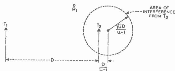
T_1 AND T_2 ARE LAND-STATION TRANSMITTERS R_1 IS A MOBILE RECEIVER INTERFERENCE AREA IS THAT IN WHICH \frac{\text{FIELD (VOLTAGE) FROM } T_2}{\text{FIELD FROM } T_1} IS GREATER THAN A SPECIFIED VALUE OF u , WHERE u IS THE ADVERSE RATIO WHICH R_1 CAN TOLERATE WITHOUT INTERFERENCE.
