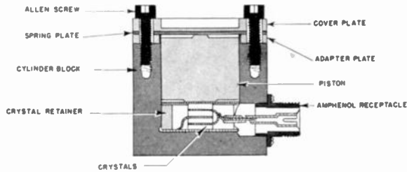
Fig. 6—Cross section of a piezoelectric accelerometer.
