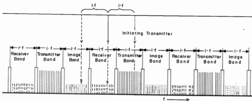
Fig. 2—A possible method of frequency allocation.
