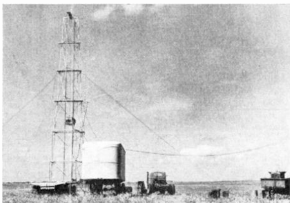
Fig. 6—Transmitting equipment.
