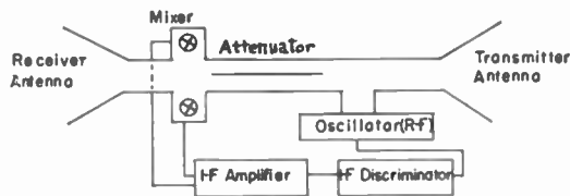
Fig. 3—A relay booster station.
