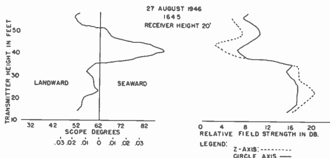
Fig. 10—Typical angle and field-strength curves.
