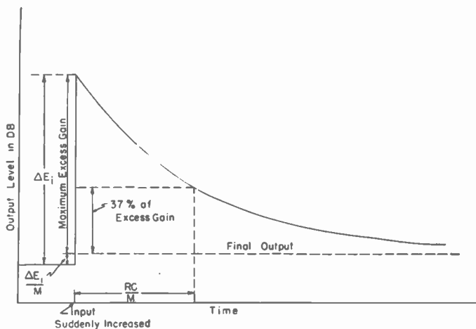
Fig. 4—Output level of an a.v.c. amplifier as a function of time, following a small sudden increase of input level.
