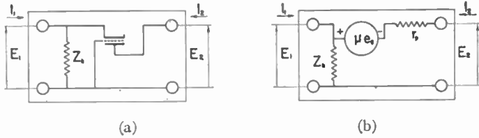
Fig. 4—Grounded-grid connection as a four-terminal network.
