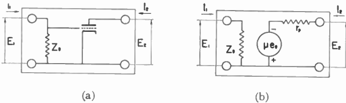
Fig. 2—Grounded-cathode connection as a four-terminal network.
