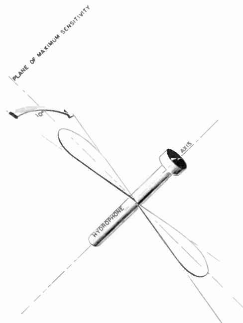
Fig. 8—Field pattern of the directional hydrophone.
