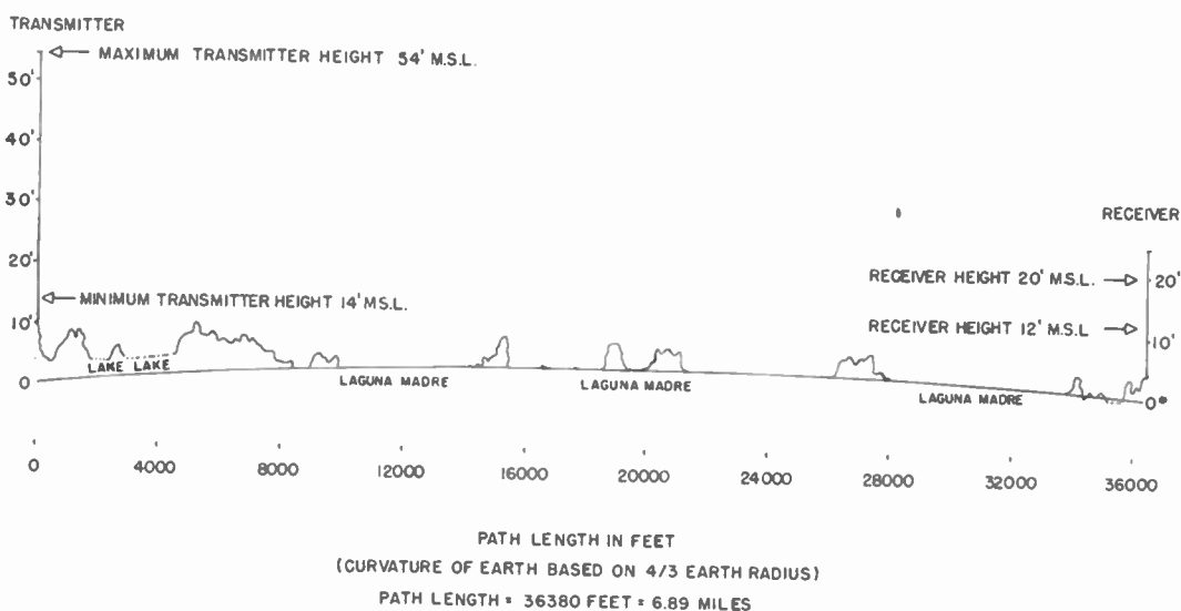
Fig. 3—Profile of path.
