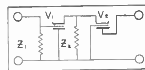
Fig. 6—Cathode-coupled triode amplifier represented as a four-terminal network.
