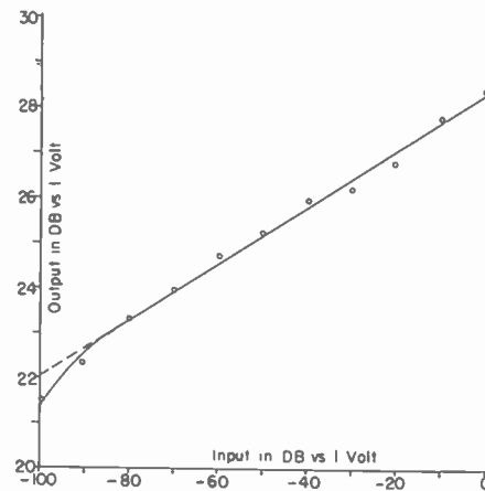
Fig. 6—Equilibrium output-input characteristic for the a.v.c. amplifier which furnished the data for Figs. 2 and 3.
