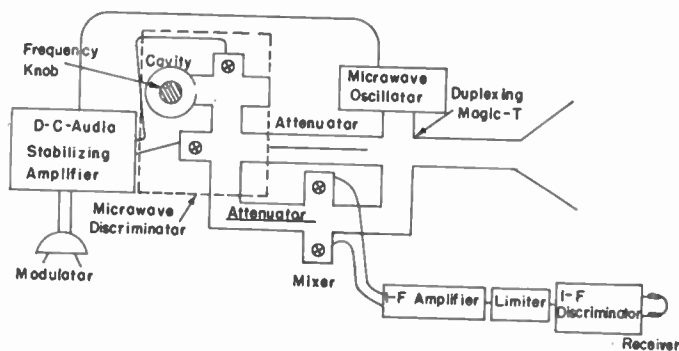
Fig. 1—Block diagram of the duplex communication station.
