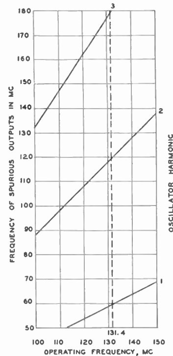
Fig. 7—Spurious output frequencies for the receiver of Fig. 6.
