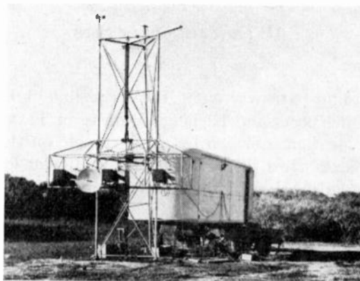
Fig. 5—Receiving tower with horns at 8-foot level.
