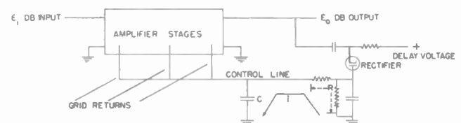
Fig. 1—Simplified a.v.c. circuit for analysis.
