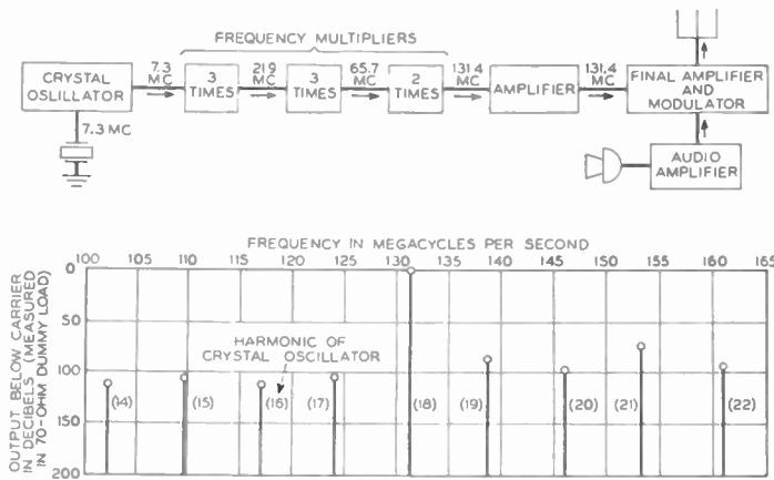
Fig. 4—Block schematic and spurious outputs of a 131.4-Mc. radio transmitter.
