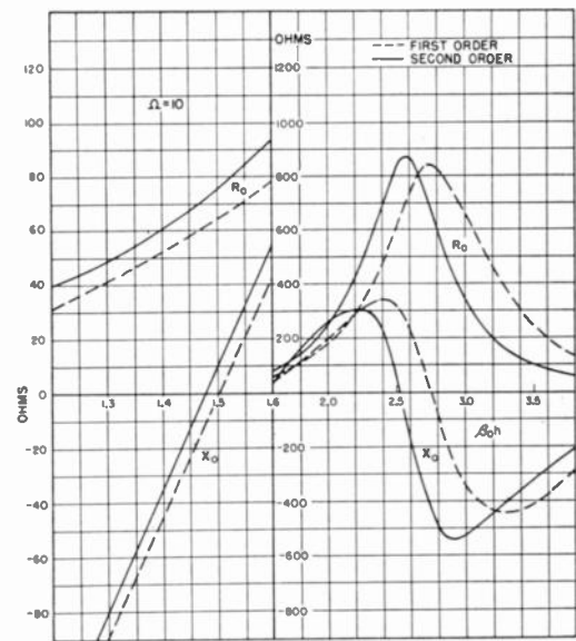
Fig. 8—First- and second-order impedances of an isolated center-driven antenna of half-length h and ratio a for \Omega = 2\pi 2h/a = 10 .
