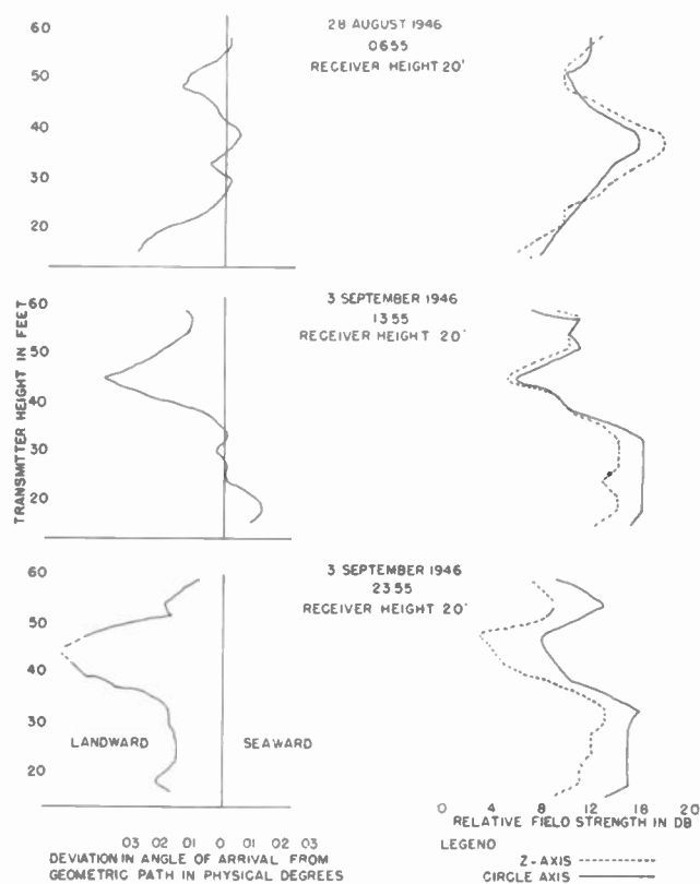
Fig. 7—Typical angle and field-strength curves. Group I.
