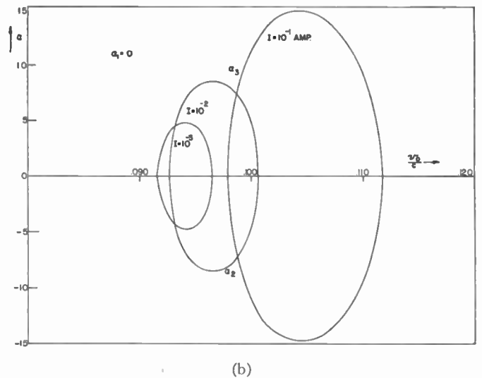
Fig. 8—Attenuation and phase constants of the three component waves as functions of the average electron velocity ( v_0 ) for beam currents I=10^{-3} , I=10^{-2} , I=10^{-1} amp. (a) Phase constants, (b) attenuation constants.
