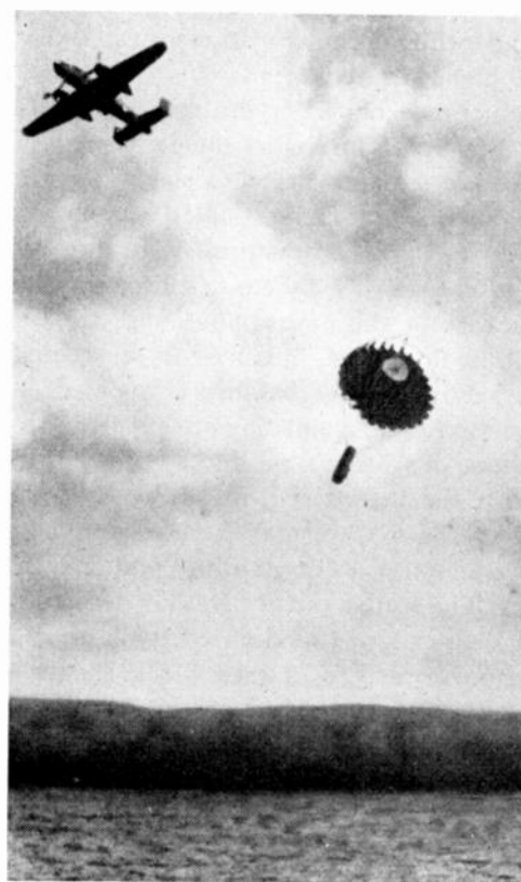
Fig. 5—Influence mine being laid by aircraft.
