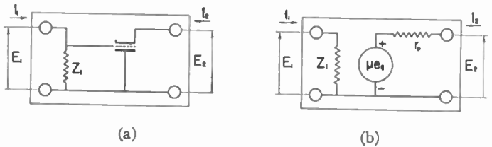
Fig. 3—Grounded-plate connection as a four-terminal network.
