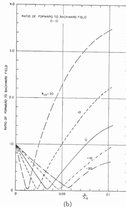
Fig. 5 (a)—Ratio of forward to backward field as obtained from Fig. 2 (a). (b)—Ratio of forward to backward field as obtained from Fig. 2 (b).
