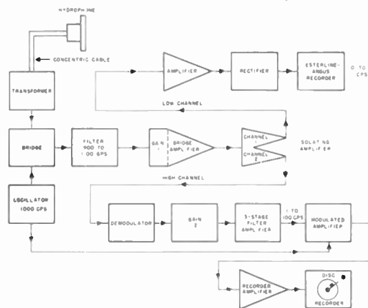
Fig. 2—Block diagram of the low-frequency system.
