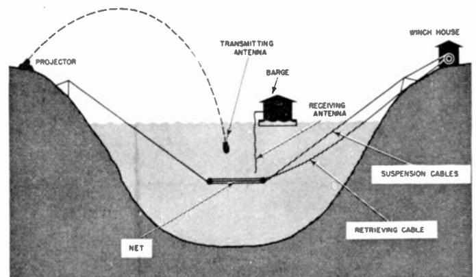
Fig. 3—Arrangement for testing depth charges.
