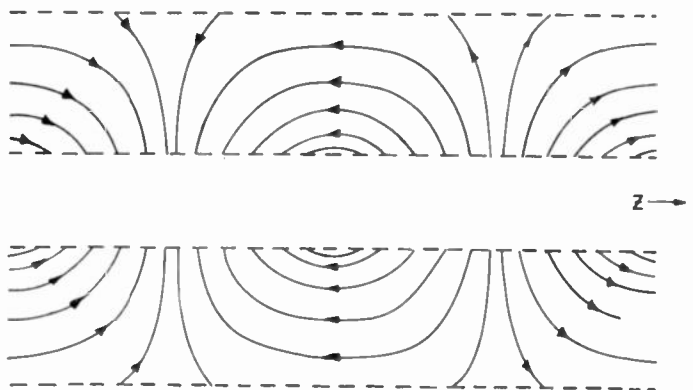
Fig. 3—Instantaneous configuration of the electric field associated with the K_0(pr) function (longitudinal section).
