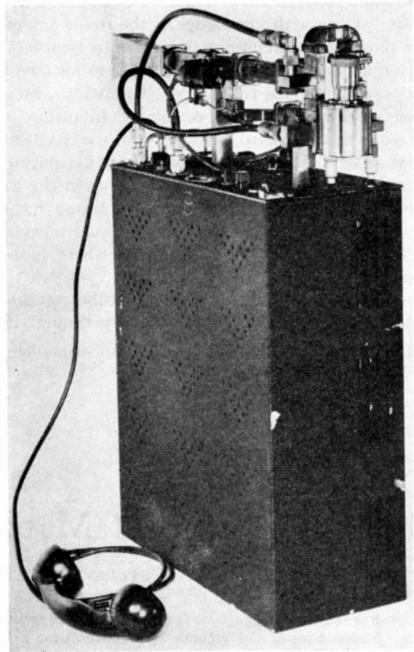
Fig. 5—A duplex communication set for the 3-centimeter band.
