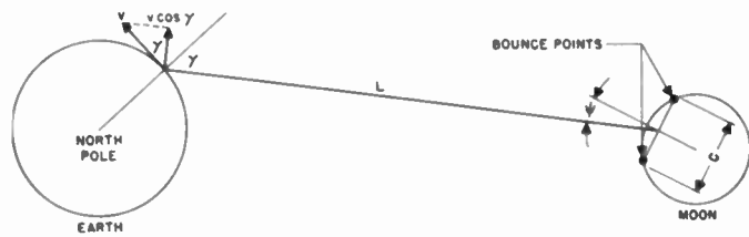
Fig. 14—Multipath transmission.
