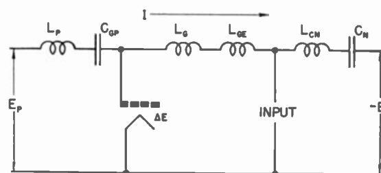
Fig. 19—Equivalent triode neutralizing circuit.
