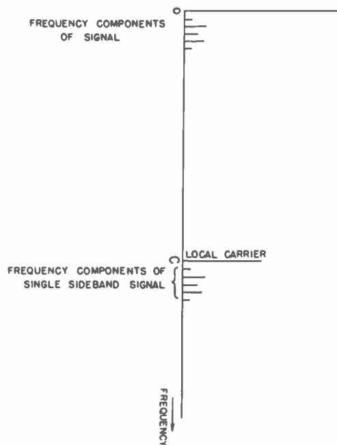
Fig. 3—Single-sideband transmission as a displacement of the information components in the frequency spectrum. (This figure shows only one set, either the a or the b components. The other set would be displaced in the same manner.)
