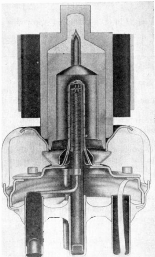
Fig. 15—Cross-sectional view of the 4X500A tetrode.
