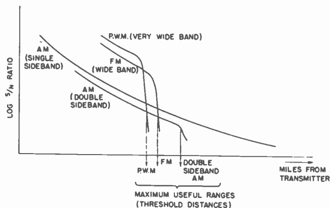
Fig. 6—Threshold versus range for a given average power, using various types of modulation.
