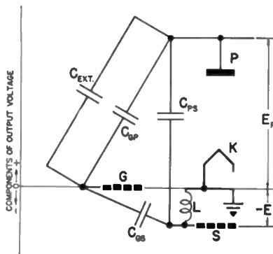
Fig. 7—Components of output voltage of a tetrode when neutralized by added external grid-to-plate capacitance.
