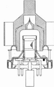
Fig. 16—Cross-sectional drawing of the 4X150A tetrode.
