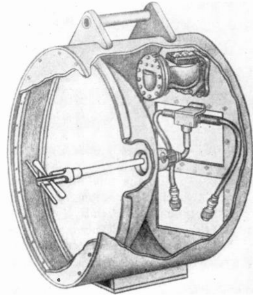
Fig. 2—Cutaway view of the antenna assembly.
