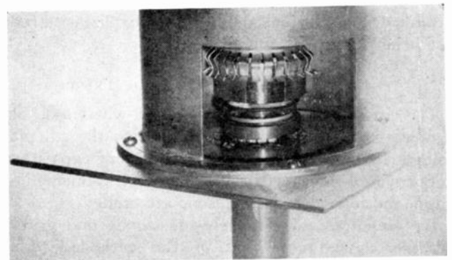
Fig. 17—Typical u.h.f. installation of a 4X150A tetrode.
