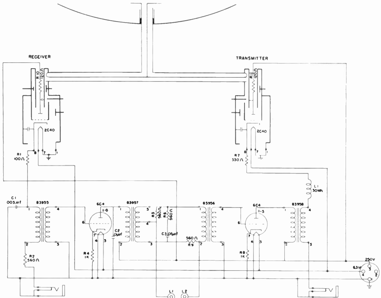
Fig. 7—Circuit diagram of Radio Set AN/PRC-3.
