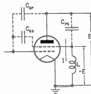
Fig. 4—More complete concept of the feedback circuit in tetrodes.
