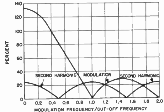
Fig. 10—Per cent modulation and per cent second harmonic for a square-law detector using amplitude modulation and narrow beam.
