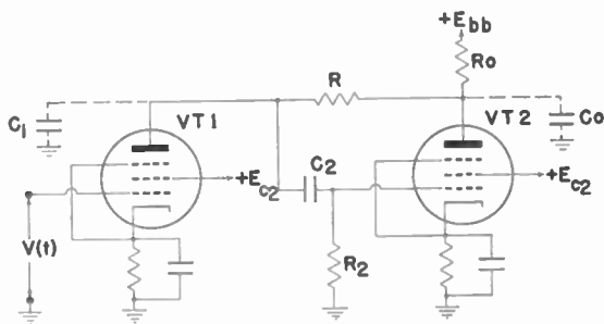
Fig. 1—Two-stage feedback amplifier showing shunt capacitances.
