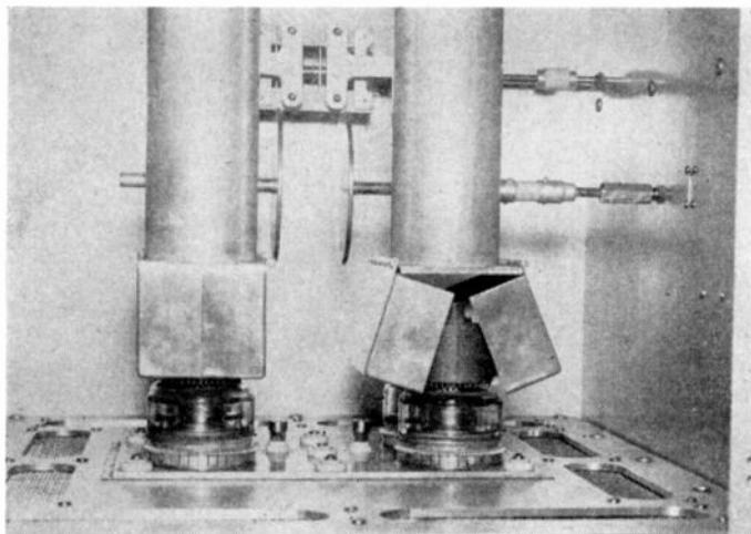
Fig. 18—Typical v.h.f. installation of a 4X500A tetrode.
