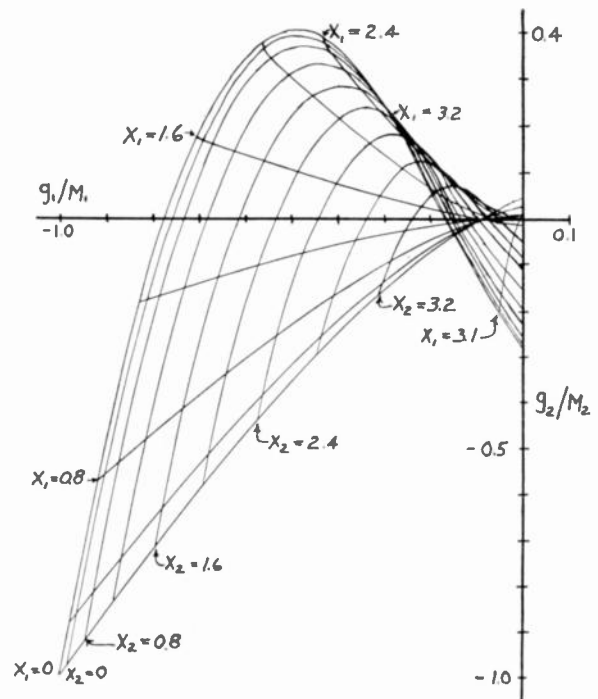
Fig. 1—Electronic conductance contours for constant-amplitude oscillations on modes N_1 = 2\frac{3}{4} and N_2 = 4\frac{3}{4} .
