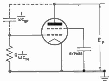
Fig. 3—Oversimplified concept of feedback in tetrodes.
