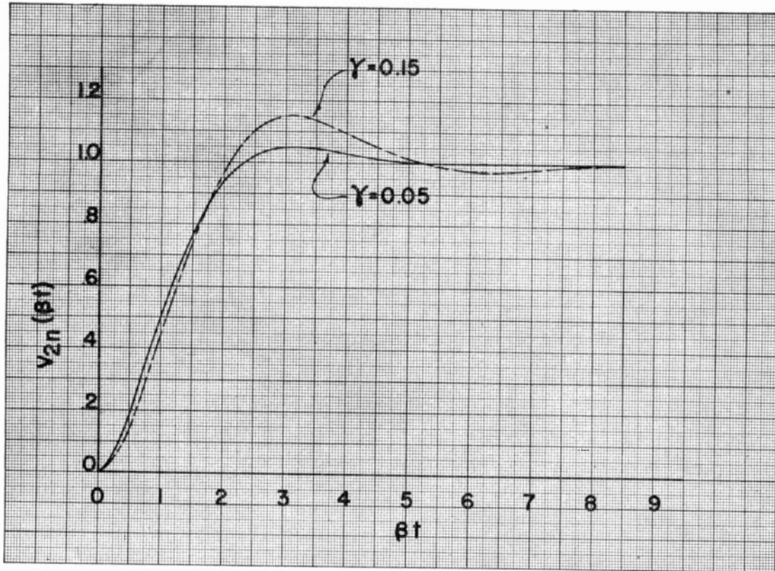
Fig. 3—Representative transient-response curves for feedback doublet.
