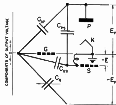
Fig. 9—Components of output voltage of a tetrode when neutralized by added conventional cross neutralization.
