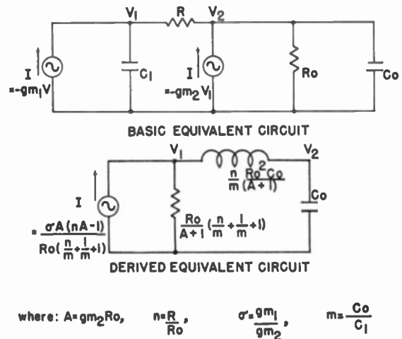
Fig. 9—Basic and derived equivalent circuits for a two-stage voltage-feedback video amplifier.
