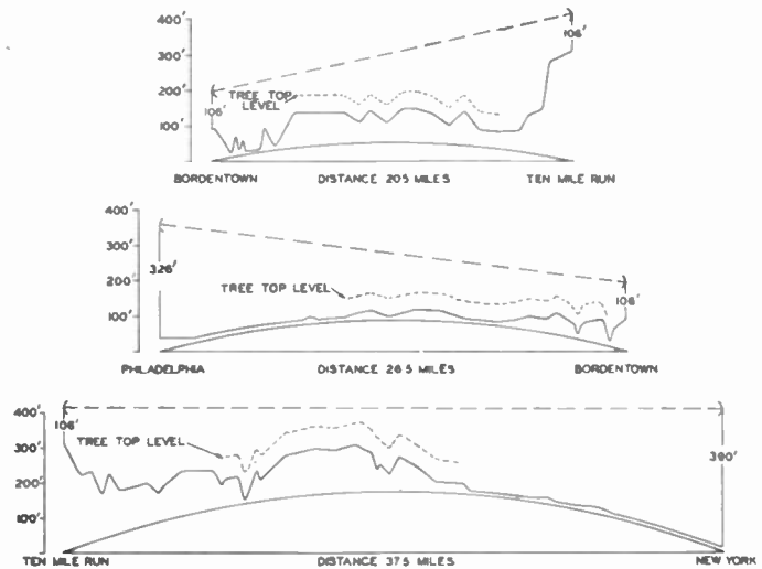
Fig. 1—Profile maps of the experimental propagation paths.
