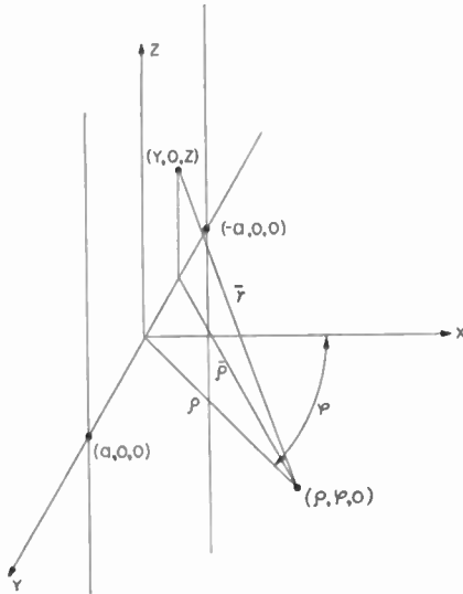
Fig. 3—Infinite-strip antenna.
