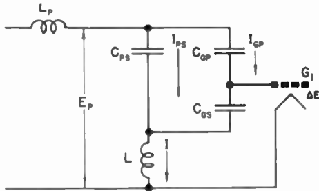
Fig. 20—Equivalent tetrode neutralizing circuit.
