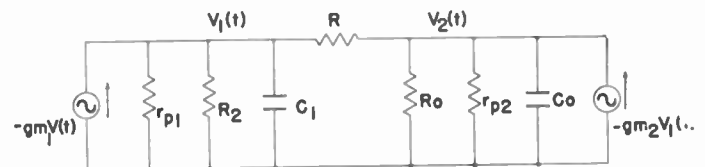
Fig. 2—High-frequency equivalent circuit of amplifier shown in Fig. 1.
