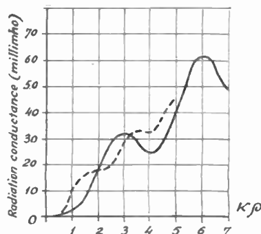
Fig. 7—Total radiation conductance as function of 2\pi\rho/\lambda . The dotted curve shows the radiation conductance of a sphere, calculated by Stratton and Chu.
