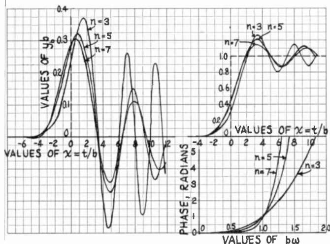
Fig. 4—Impulse and step transient responses, and phase-response characteristics of all-pass networks whose phase distortion is \Delta B = (bw)^n radians.
