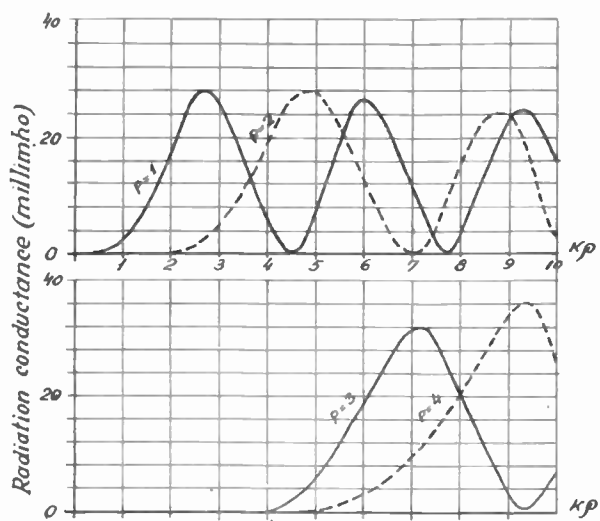
Fig. 5—Radiation conductance of first four wave modes as functions of 2\pi\rho/\lambda .
