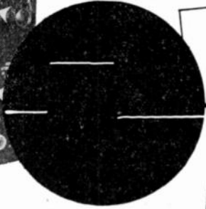
Oscillogram of 1 micro-second pulse passed through video amplifier of Type 256-D Oscilloscope.
