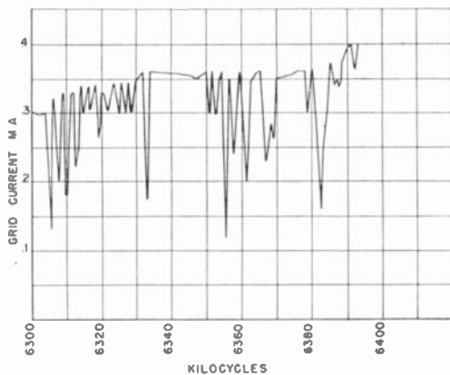
Fig. 3—Activity-versus-frequency characteristic of plated crystal (BT-cut) without damping.
