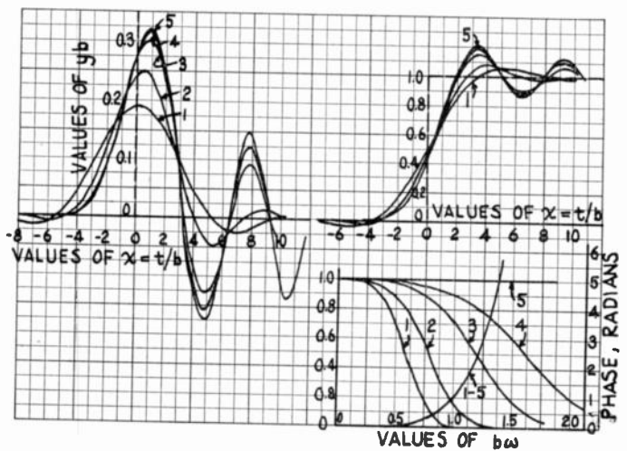
Fig. 8—Impulse and step transient responses, phase- and amplitude-response characteristics of combined networks whose phase distortion is (b\omega)^5 radians, and attenuation distortion is (a\omega)^4 nepiers.
