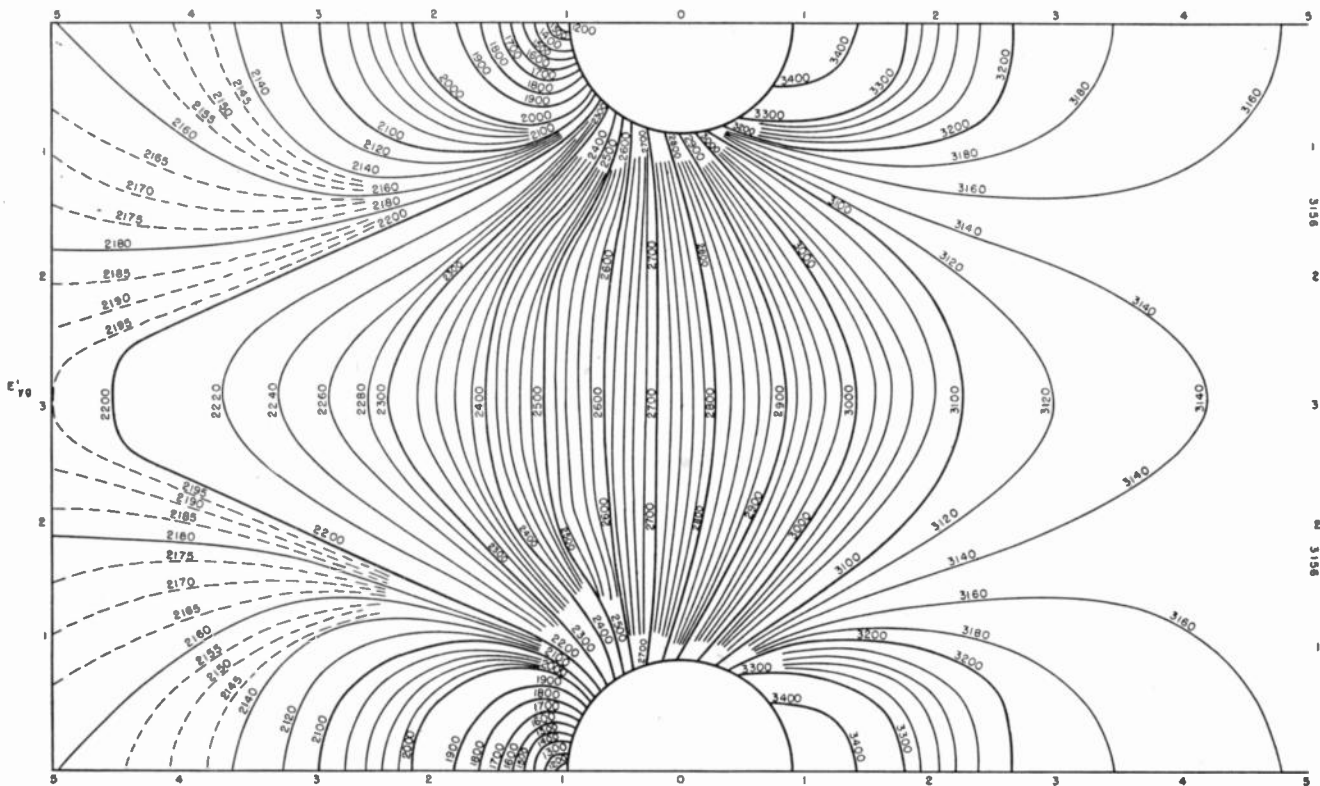
Fig. 3—Contours of constant E_{0y}' for the 2C39 tube.
