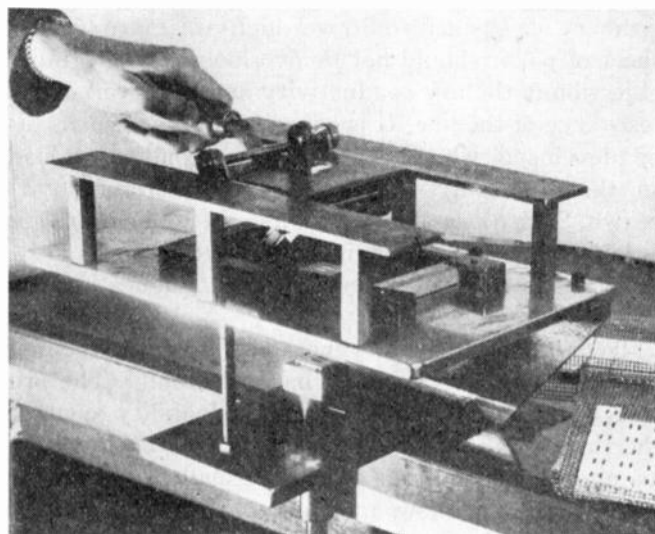
Fig. 17—Pressure-controlled painted-resistor applicator.
