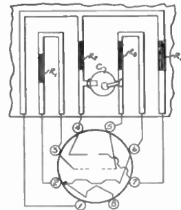
Fig. 38—Circuit diagram and developed stencil for the two-stage amplifier of Fig. 37.
