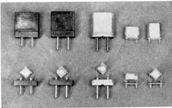
Fig. 9—Various types of high-frequency plated crystal units.
