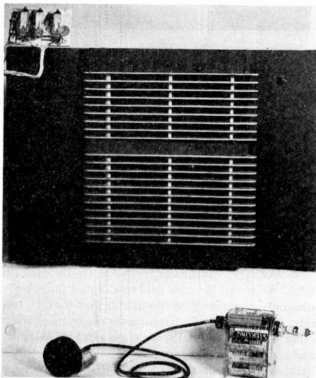
Fig. 42—Subminiature printed transmitter and receiver. The 2 \times 3 -inch printed receiver (top) has sufficient power to operate the standard 10-inch console speaker. The transmitter assembly (below) consists of a power pack with the tube transmitter and microphone cable plugged into opposite sides.
