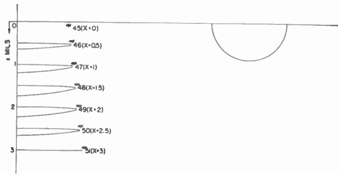
Fig. 9—Electron trajectories for \alpha = 1.8 radians.
