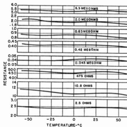
Fig. 28—Resistance versus temperature characteristics of printed resistors.
