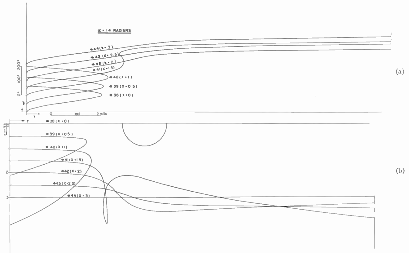
Fig. 7—(a) Time vs. distance plots for \alpha=1.4 radians. (b) Electron trajectories for \alpha=1.4 radians.
