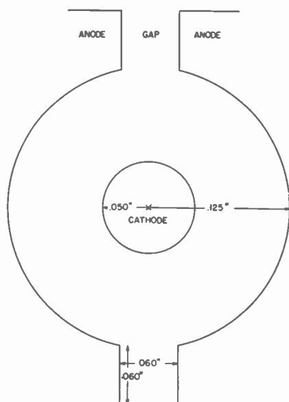
Fig. 1—Split-anode-magnetron configuration.
