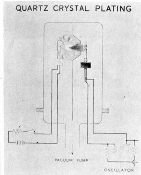
Fig. 7—Evaporator schematic.
