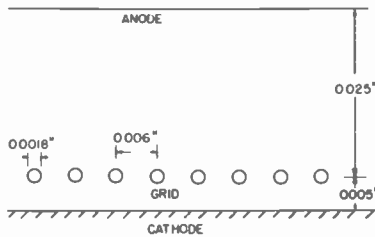
Fig. 1—Cross section showing configuration of the 2C39 tube.
