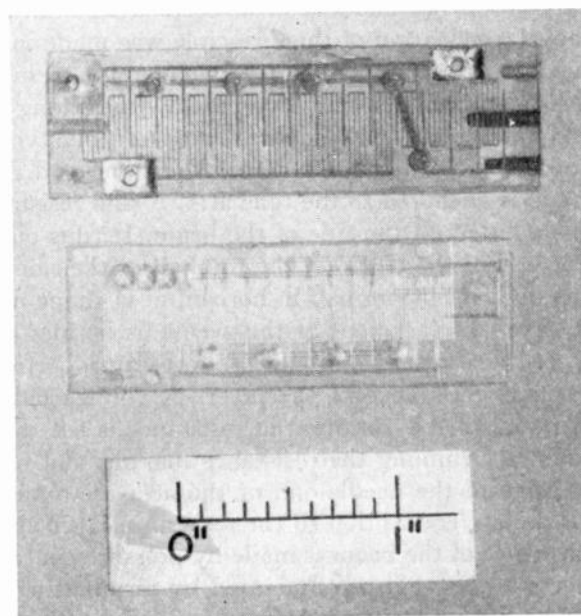
Fig. 51—Radiosonde commutator made by printed-circuit techniques.
