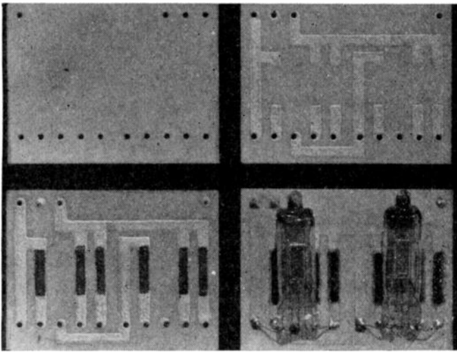
Fig. 13—Four stages in printing an electronic circuit by the stenciled-screen process: top left, blank steatite plate; top right, conductor pattern of silver paint applied through the silk screen; lower left, six resistors added with carbon paint, using a second stencil; lower right, subminiature tubes soldered in place.
