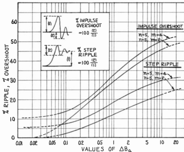
Fig. 10—Impulse overshoot and step peak-to-peak ripple versus the phase distortion at amplitude cutoff \Delta B_a , for values of n=5 , and m=2, 4 .
