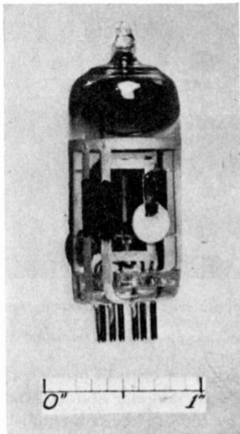
Fig. 37—A two-stage amplifier painted on the glass envelope of a twin-triode miniature vacuum tube (type 6J6) using the stenciled-screen process.
