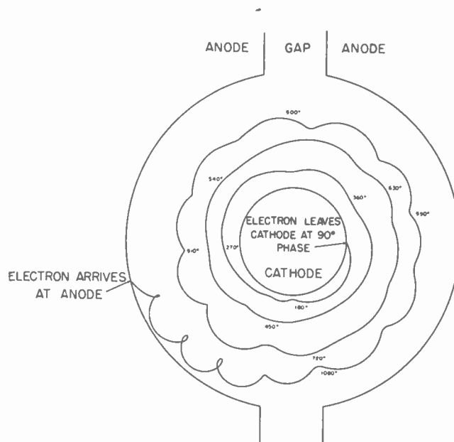
Fig. 2—Typical electron trajectory in split-anode magnetron. Magnetic field = 1500 gauss; d.c. voltage = 1750; a.c. r.m.s. voltage = 400; and frequency = 360 Mc.
