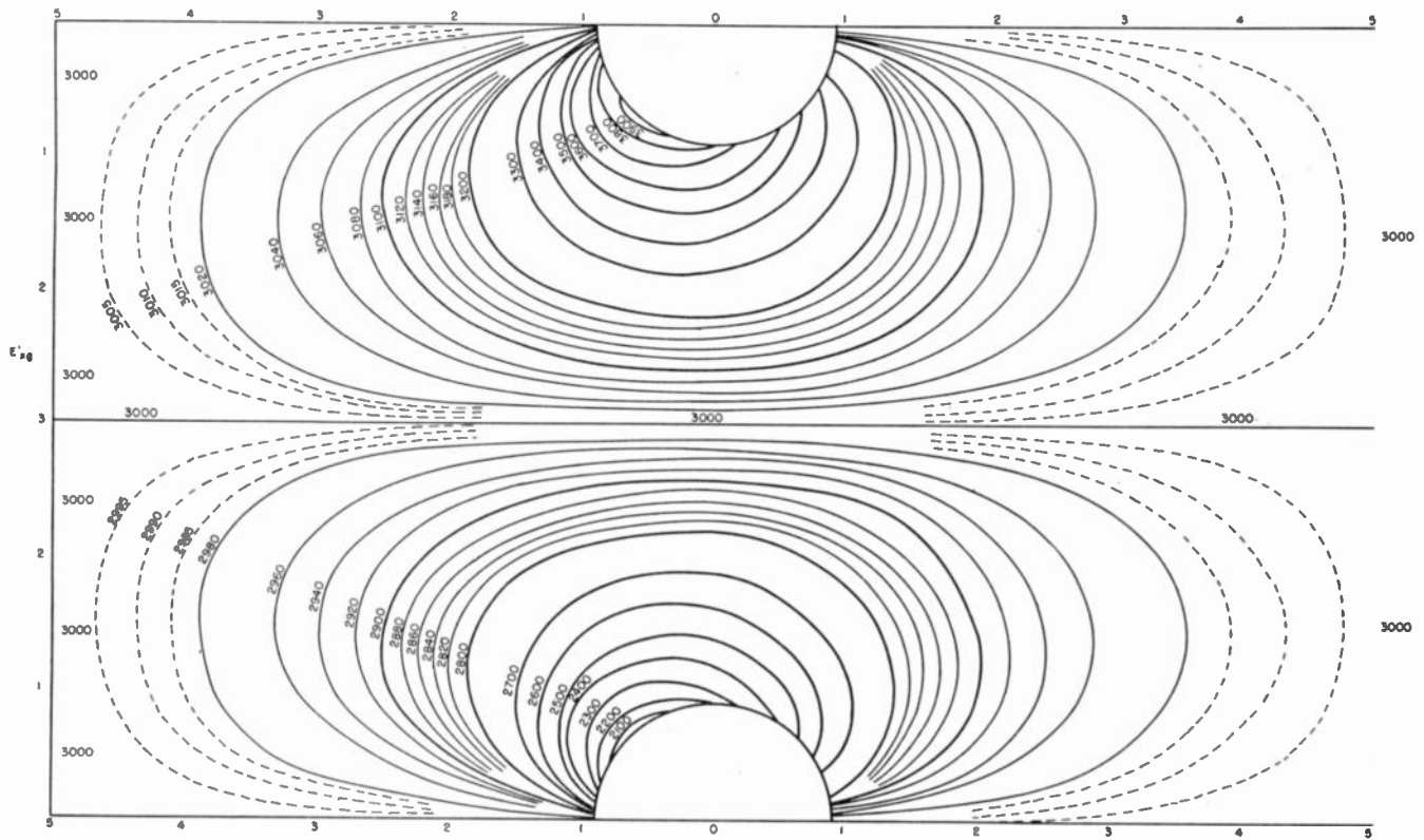
Fig. 2—Contours of constant E_{0z}' for the 2C39 tube.
