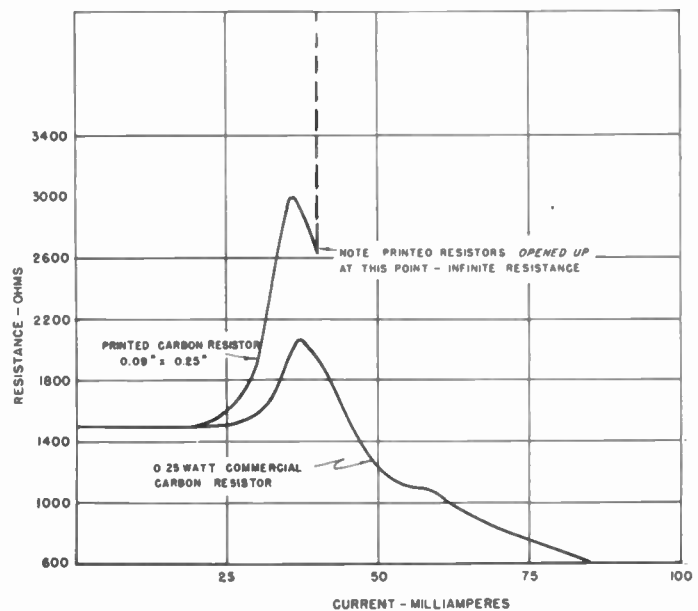
Fig. 26—Comparison of the current-carrying capacity of an average carbon resistor with a 0.25-watt commercial carbon resistor. Both are nominally 1500 ohms.
