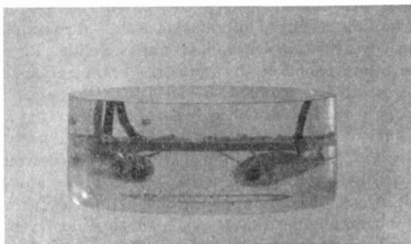
Fig. 50—Two-stage amplifier printed on a ceramic plate and encased in NBS Casting Resin.
