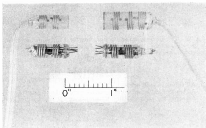
Fig. 46—Examples of inductors applied to glass tube envelopes with ruling pen and lathe.
