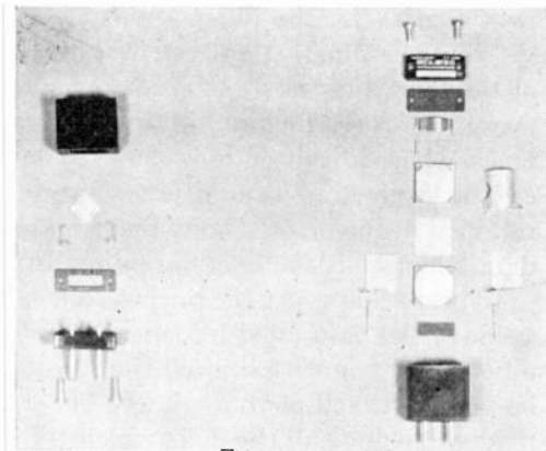
Fig. 1.—Assembly details of plated- and clamped-type quartz crystal units.
