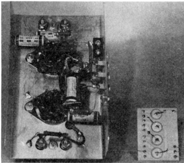
Fig. 3—View of bottom sides of printed and conventional units of Fig. 2.
