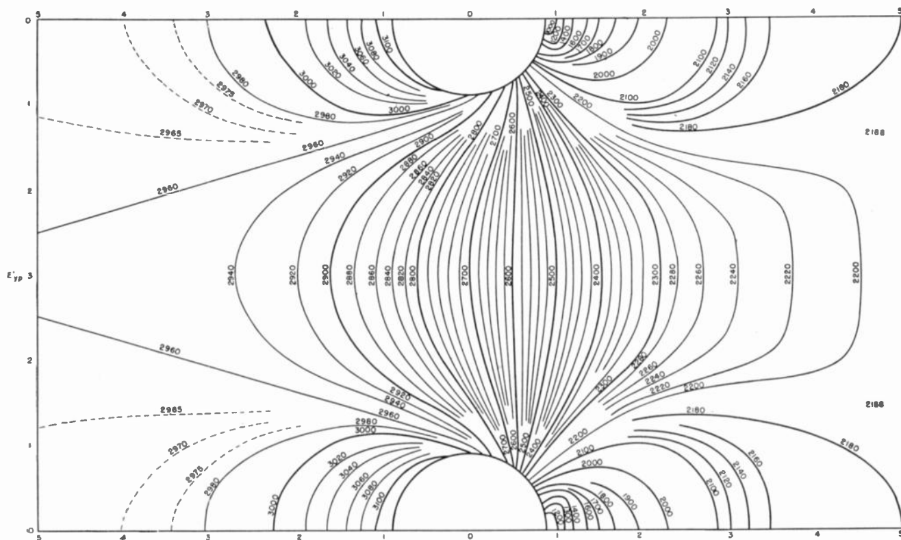
Fig. 5—Contours of constant E_{py}' for the 2C39 tube.
