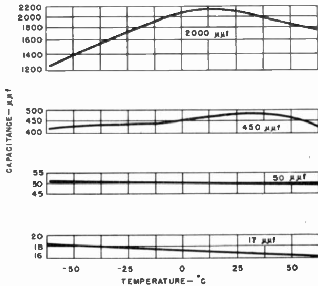
Fig. 29—Capacitance versus temperature characteristics of ceramic-disk capacitors.
