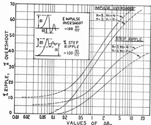
Fig. 9—Impulse overshoot and step peak-to-peak ripple versus the phase distortion at amplitude cutoff \Delta B_a , for values of n=3 , and m=2, 4 .
