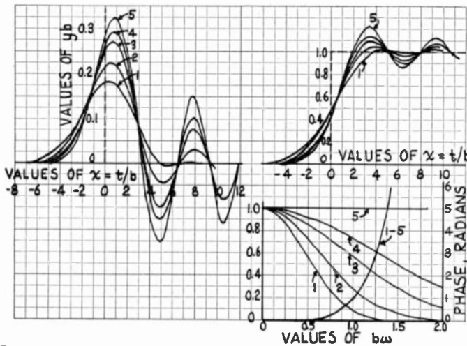
Fig. 6—Impulse and step transient responses, phase- and amplitude-response characteristics of combined networks whose phase distortion is (b\omega)^5 radians, and attenuation distortion is (a\omega)^2 nepiers.
