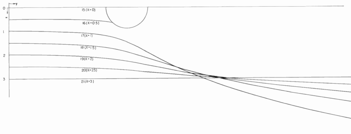
Fig. 6—Electron trajectories for \alpha=0.4 radians.
