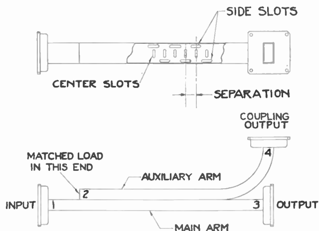
Fig. 1—Basic directional coupler.
