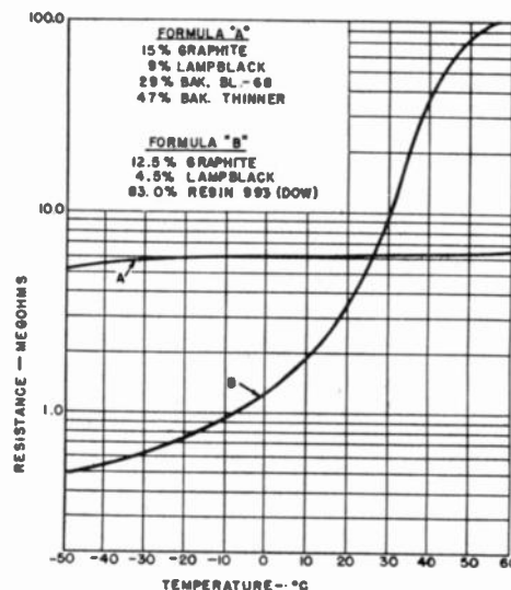
Fig. 27—Effect of composition on the resistance versus temperature characteristics of printed resistors.
