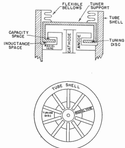
Fig. 5—By properly shaping the anode vanes, motion of a single tuning disk varies both inductance and capacitance.
