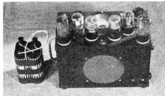
Fig. 11—Demonstration duplicator.
