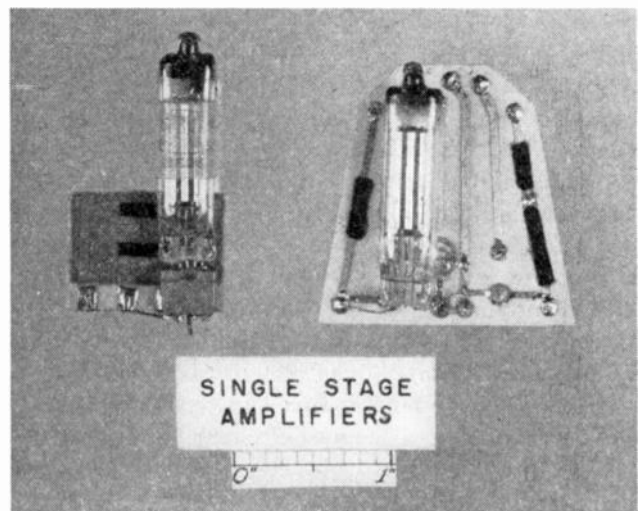
Fig. 6—Single-stage amplifiers printed on steatite plates by the stenciled-screen process.
