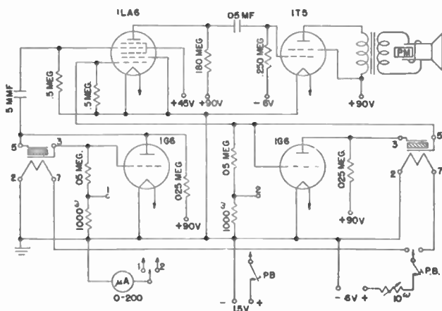
Fig. 10—Circuit of demonstration duplicator.
