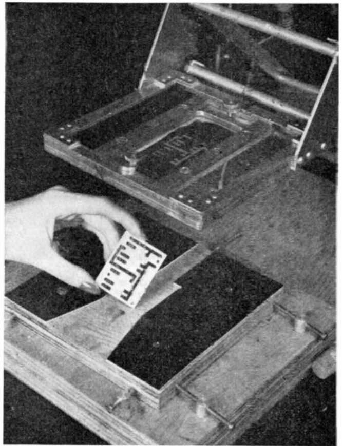
Fig. 11—A retractable stencil holder for applying paint to an insulated plate. The holder moves forward and down over a plate held in the platen. The plate shown has just been removed from the platen.
