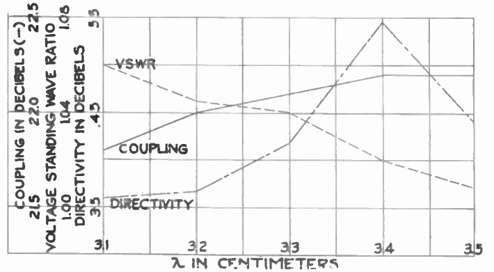
Fig. 6—Performance data of directional coupler. 20 pairs of slots \frac{3}{16} \times \frac{1}{16} inch \times 0.221 separation.
