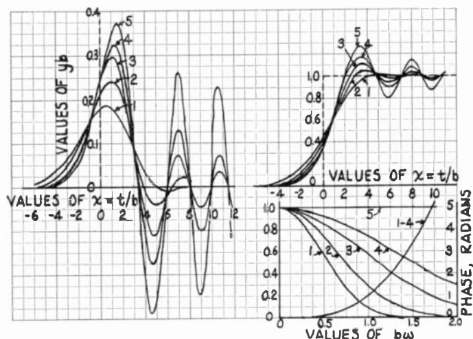
Fig. 5—Impulse and step transient responses, phase- and amplitude-response characteristics of combined networks whose phase distortion is (bw)^3 radians, and attenuation distortion is (a\omega)^2 nepers.
