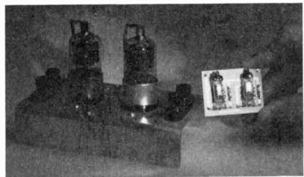
Fig. 2—Comparison of a two-stage voltage amplifier printed on a ceramic plate (right), with an equivalent amplifier constructed according to present-day radio practice (left).
