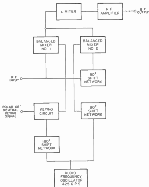
Fig. 6—Frequency-shift keying by raising and lowering the r.f. signal by an audio frequency.
