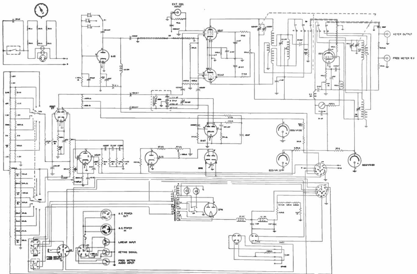
Fig. 11—Schematic diagram of reactance-type frequency-shift transmitter keyer.
