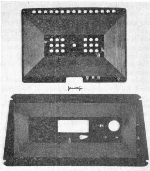
Fig. 22—Loop antennas stamped from single pieces of sheet copper onto insulated bases.
