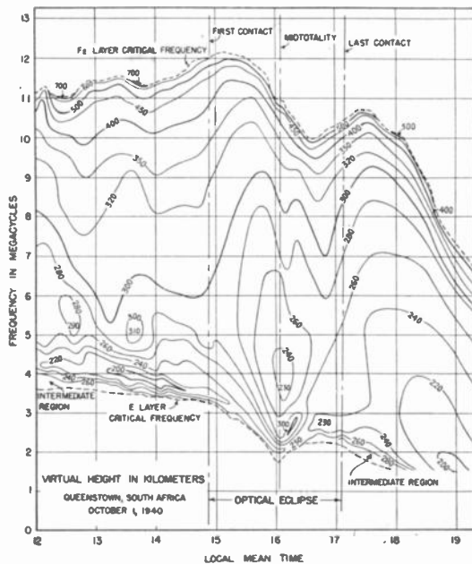
Fig. 8—Contours of constant virtual height of reflection of the ordinary ray from the F region on the afternoon of the eclipse.
