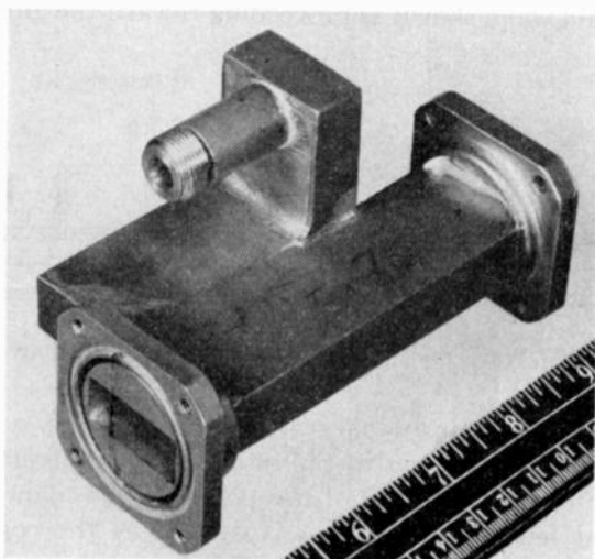
Fig. 43—Wave-guide directional coupler.
