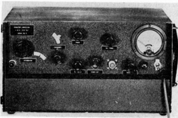
Fig. 38—Frequency-modulation test set.
