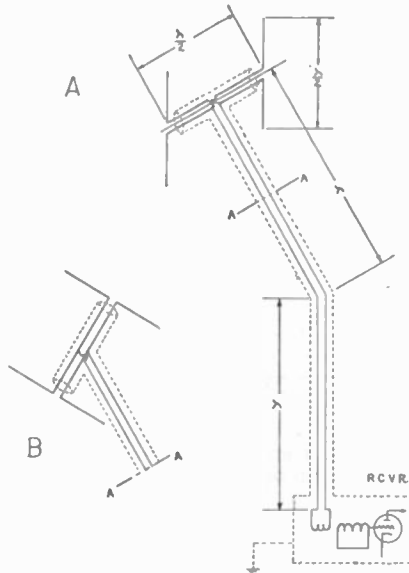
Fig. 2—A: General layout of the Adcock antenna system. B: General layout of the H antenna.
