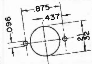
MOUNTING LAYOUT
