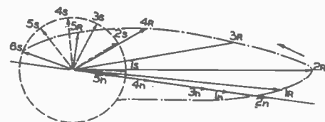
Fig. 3—Vector diagram showing how noise pulse causes momentary change of resultant phase, resulting in a click.
