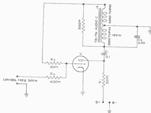
Fig. 1—Basic circuit of frequency-controlled oscillator.
