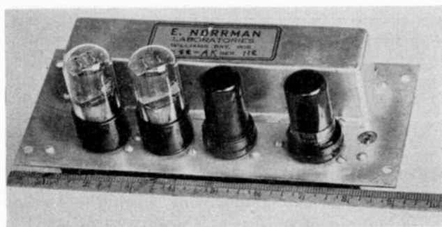
Fig. 6—Top view of four-stage frequency divider.
