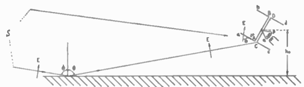
Fig. 4—Sketch showing the reception of both the direct component and the reflected component of the radiation emitted from a distant source S (to the left of the figure) by an H-antenna system at a height h_0 above ground.
