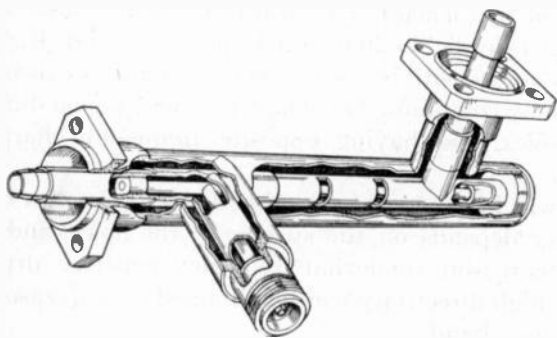
Fig. 44—Coaxial directional-coupler schematic diagram.
