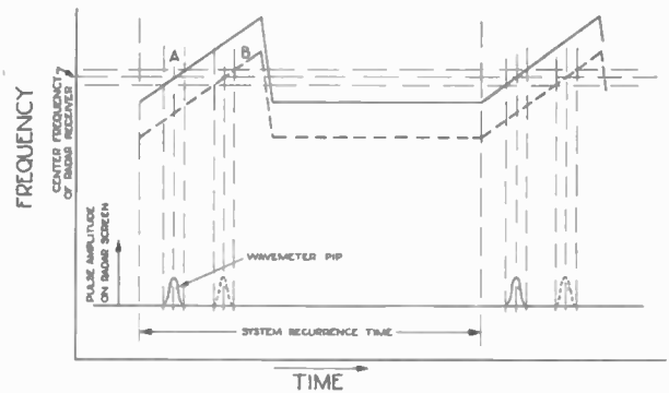
Fig. 35—Operational diagram of the frequency-modulation test set.
