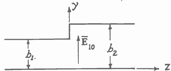
Fig. 8—Capacitive change of cross section.
