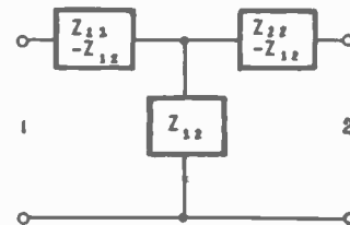
Fig. 2—T network.
