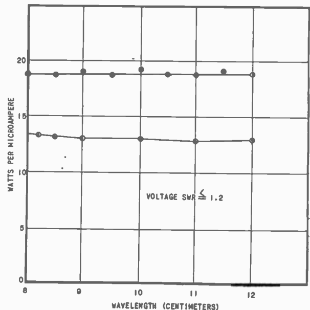
Fig. 8—Calibration curves for two representative thermocouples.
