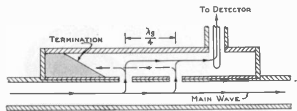
Fig. 42—Wave-guide directional-coupler schematic diagram.
