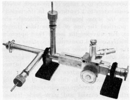
Fig. 1—Coaxial slotted section.
