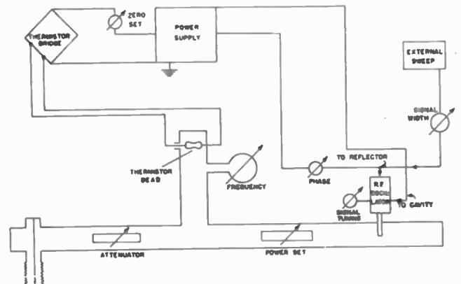
Fig. 36—Block diagram of the frequency-modulation test set.
