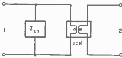
Fig. 3—Approximate equivalent circuit.
