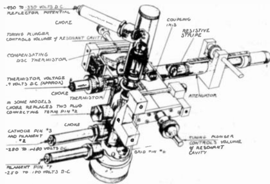
Fig. 33—Cavity for velocity-modulation tube showing tube in place.
