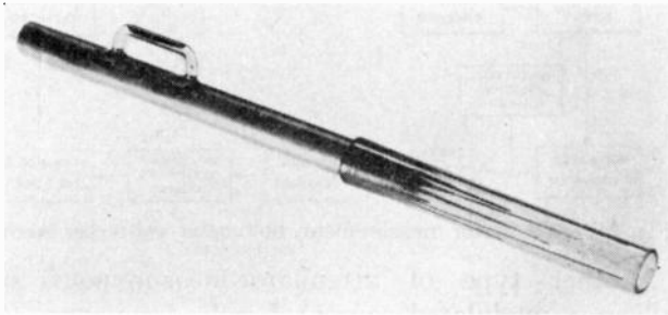
Fig. 19—Slider for coaxial variable attenuator showing tapered matching section.
