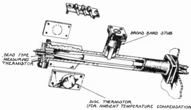
Fig. 13—Broad-band coaxial thermistor mount with taper to type-N connector.
