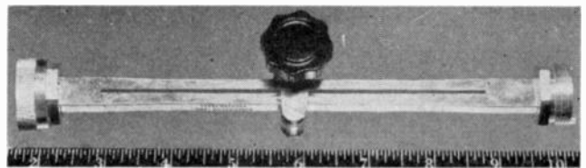
Fig. 3—Wave-guide squeeze section.
