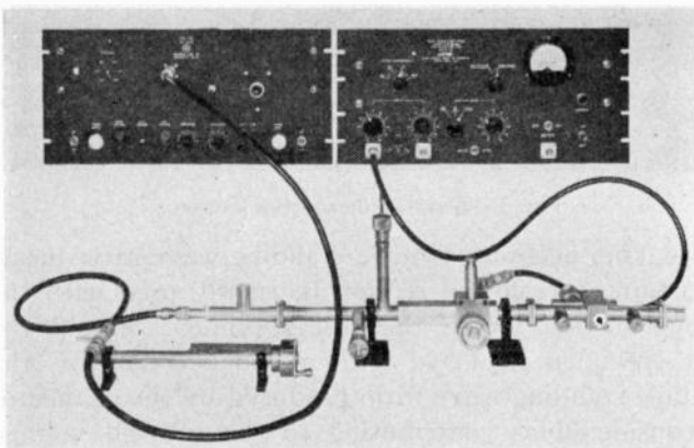
Fig. 4—Coaxial standing-wave setup.
