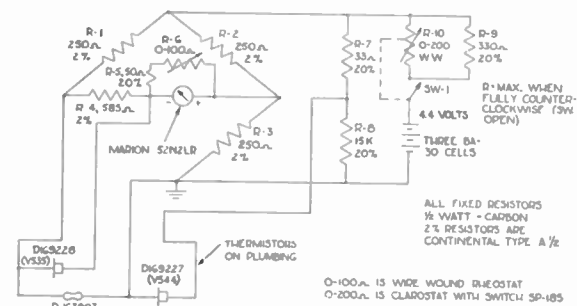
Fig. 16—Two-milliwatt thermistor bridge, temperature compensated.
