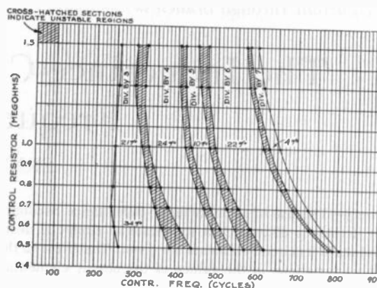
Fig. 3—Characteristic curves for even divisions.
