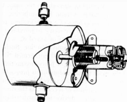
Fig. 45—Resonant-cavity echo box.
