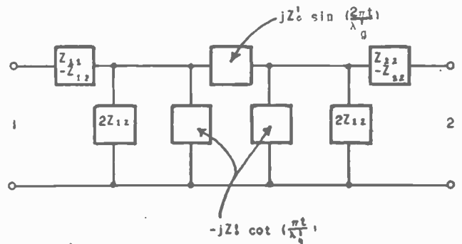
Fig. 4—Equivalent circuit for thick obstacle.
