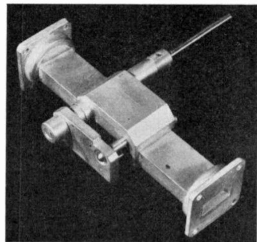
Fig. 21—Metalized-glass-type wave-guide attenuator.
