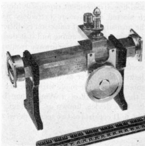
Fig. 2—Wave-guide slotted section.
