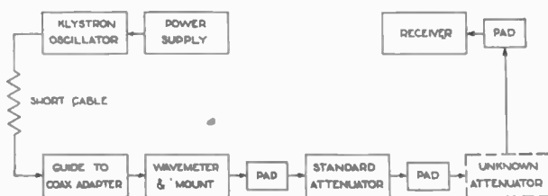
Fig. 23—Block diagram of the attenuator comparator.
