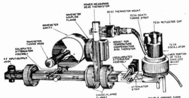
Fig. 37—Frequency-modulation test set; radio-frequency plumbing layout.
