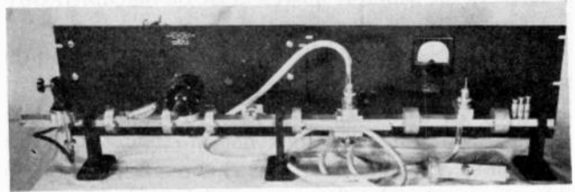
Fig. 5—Wave-guide standing-wave setup.
