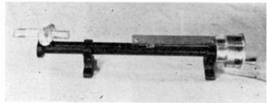
Fig. 27—Short-circuited coaxial-line wavemeter.
