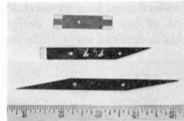
Fig. 20—Metalized plates for wave-guide attenuators: top, tongue-type matching sections; center, unilaterally matched with taper; bottom, bilaterally matched with tapers.
