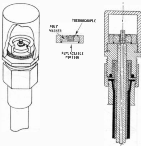
Fig. 6—Thermocouple construction.
