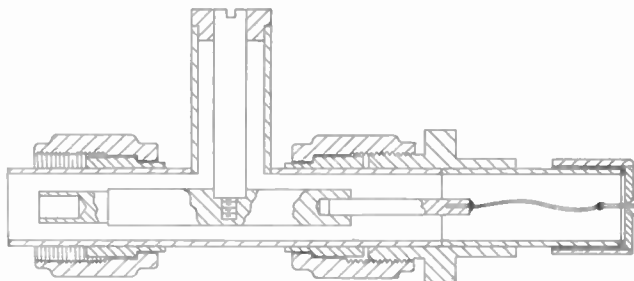
Fig. 14—Cross section of \frac{1}{4} -inch metalized-glass coaxial bolometer mount.
