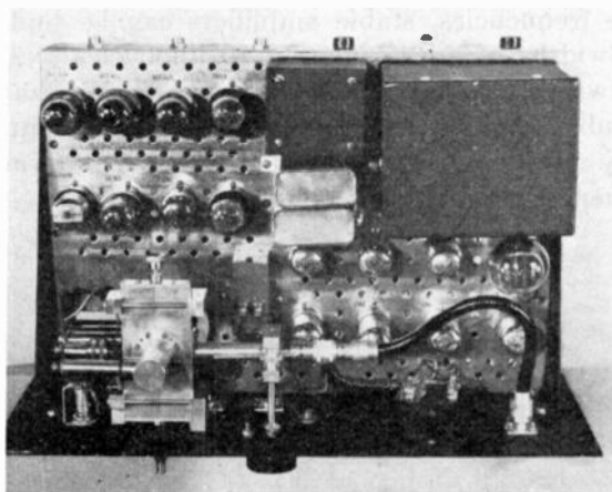
Fig. 34—Signal generator for use in the 3000-megacycle region of the spectrum.
