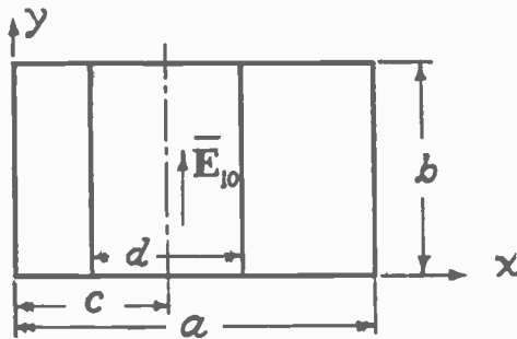
Fig. 6—Inductive window.
