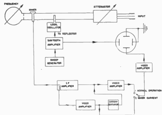
Fig. 39—Block diagram of the spectrum analyzer.
