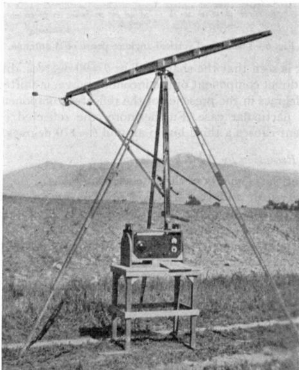
Fig. 3—Complete assembly of the direction finder.
