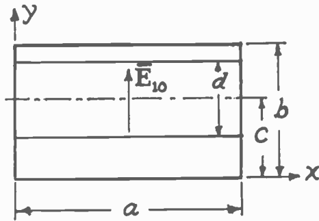
Fig. 7—Capacitive window.
