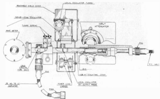
Fig. 40—Spectrum analyzer for use in the 10,000-megacycle region.
