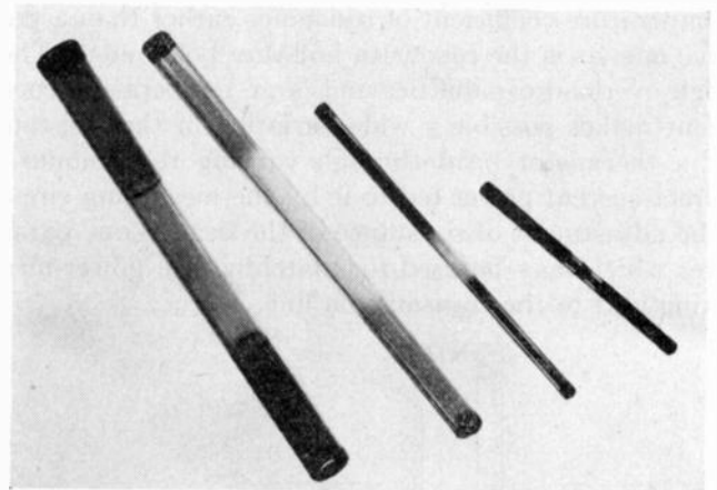
FIG. 18—Coaxial attenuator inserts. Metalized-glass type with matching sections.
