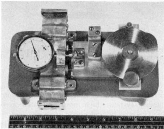
Fig. 22—Standard wave-guide attenuator, metalized-glass type.
