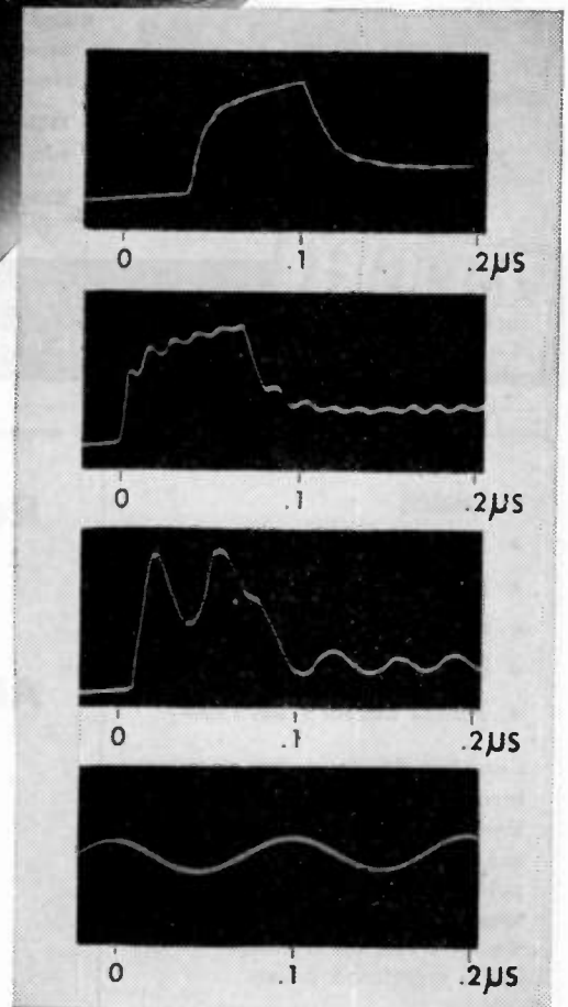
Typical high-speed single-transient recordings with 5RP at 18,000 volts accelerating potential. (Courtesy of Prof. M. Newman, Institute of Technology, University of Minnesota.)
