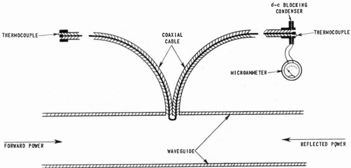
Fig. 3—Direct-current circuit arrangement.
