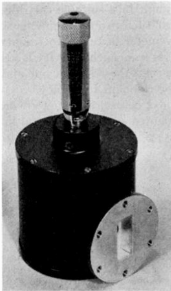
Fig. 28—Cavity-type wavemeter for 10,000-megacycle use.
