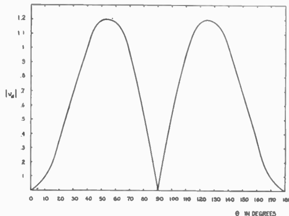
Fig. 5—Direct component of the signal received by H antenna as a function of \theta calculated theoretically.
