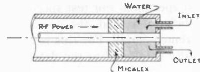
Fig. 11—Coaxial water load.
