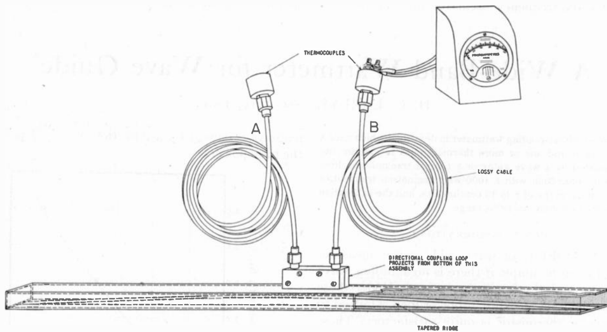
Fig. 2—Wattmeter assembly.
