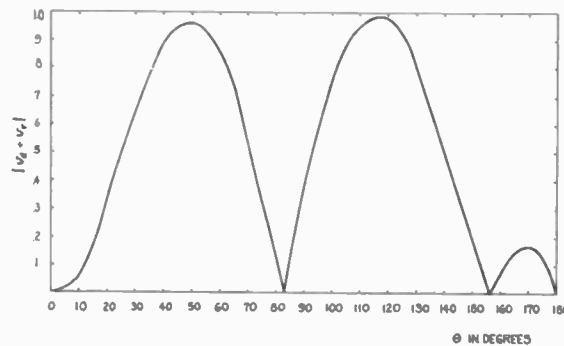
Fig. 6—Theoretical vertical-angle response of H antenna.
