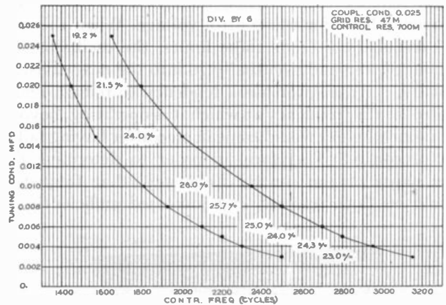
Fig. 5—Frequency versus tuning capacitance. Turns in plate circuit = 2200; turns in grid circuit = 630.
