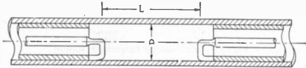
Fig. 17—Wave-guide beyond-cutoff attenuator. Attenuation for \Delta l = D , (DB/Dia.):
