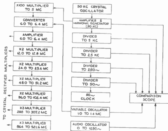
Fig. 25—Crystal frequency standard for microwave application.
