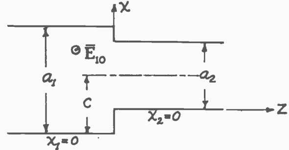
Fig. 9—Inductive change of cross section.
