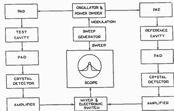
Fig. 30—Block diagram of the cavity comparator.
