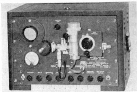
Fig. 41—Spectrum analyzer for 10,000 megacycles.
