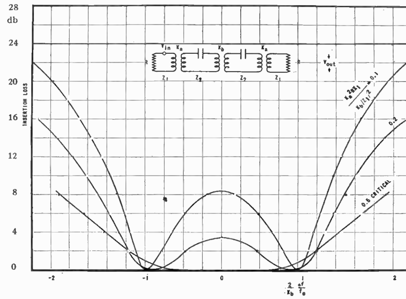
Fig. 3—Universal insertion-loss versus frequency characteristics of a double-resonant-circuit band-pass filter.
