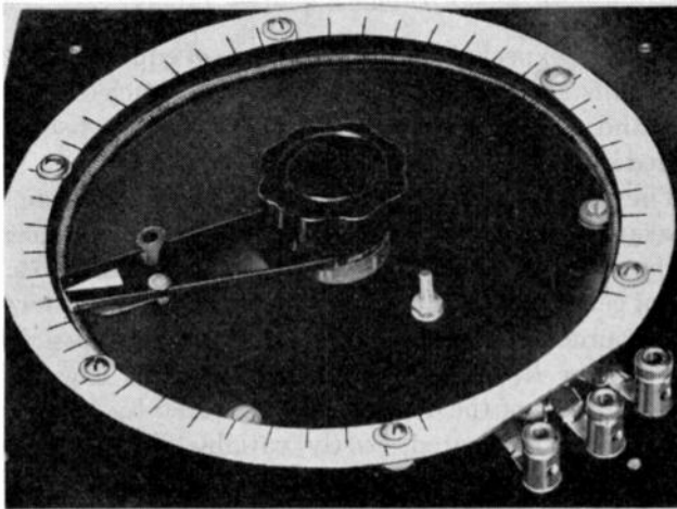
Fig. 12—Variable delay line.
