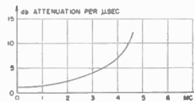
Fig. 19C—Attenuation.
