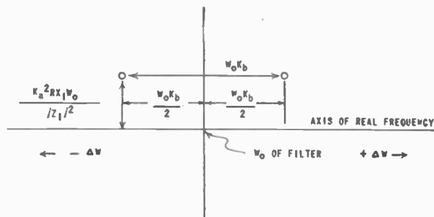
Fig. 7—Location of the roots of the impedance determinant for the double-resonant-circuit filter in the complex-frequency plane.
