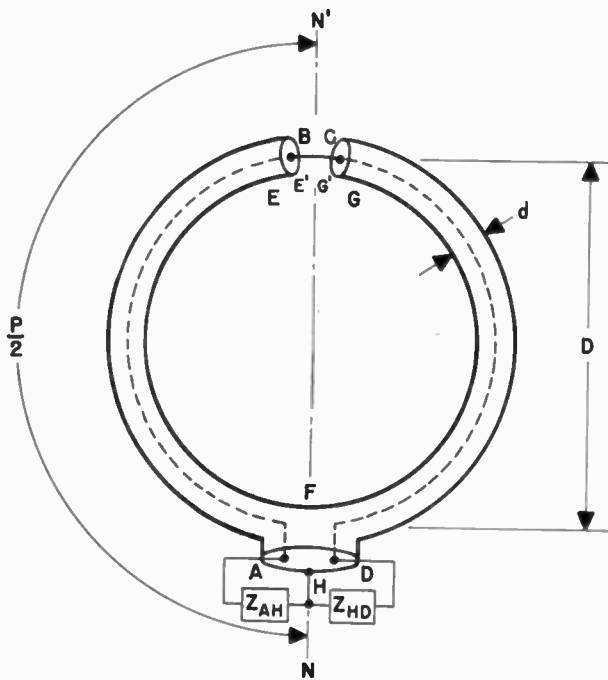
Fig. 1—Single-turn balanced shielded loop antenna.
