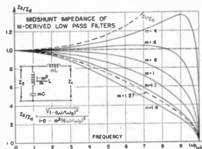
Fig. 27—Impedance characteristics of m -derived low-pass filters.
