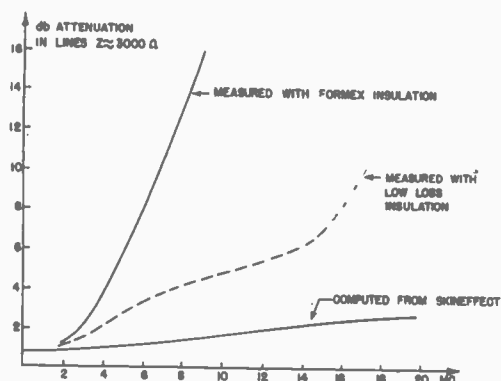
Fig. 15—Attenuation in delay lines with Formex, and with low-loss wire insulation.
