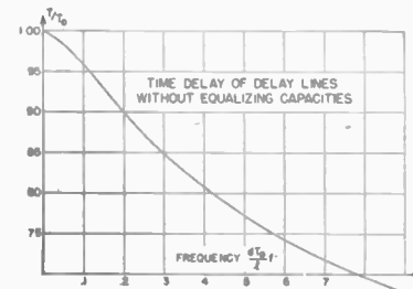
Fig. 5—Decrease of time delay in delay lines with higher frequencies.
