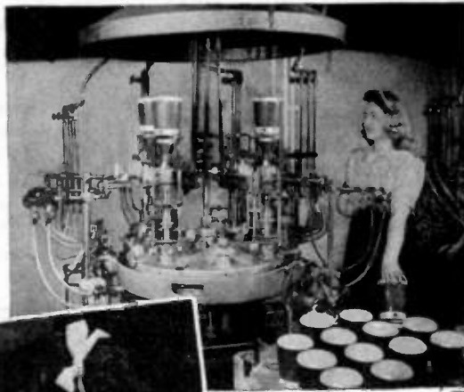
Sealing the gun and stem assembly within the bulb
