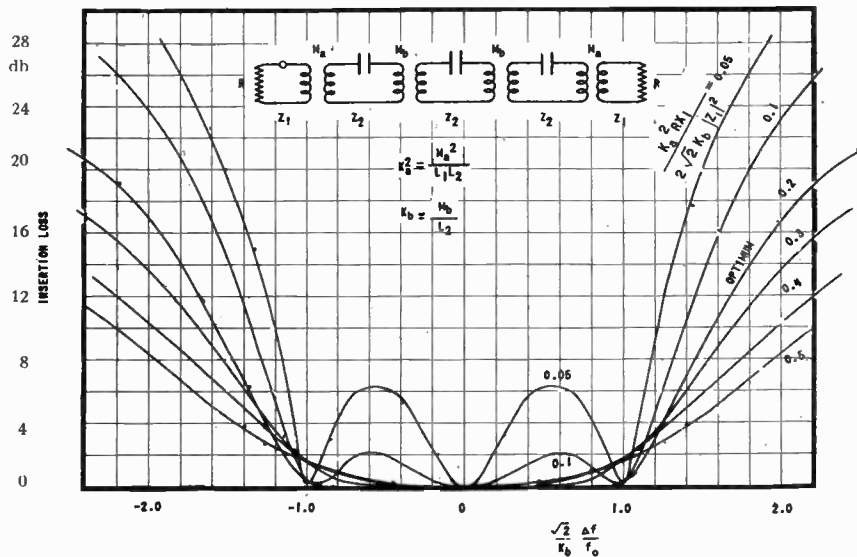
Fig. 4—Universal insertion-loss versus frequency characteristics of a triple-resonant-circuit band-pass filter.
