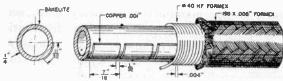
Fig. 20A—Patch-equalized delay line with grounded-braid cover, impedance 1000 ohms.
