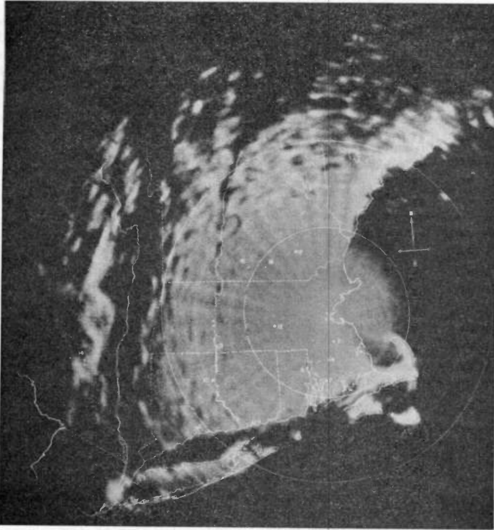
Fig. 1—Superimposed map on airborne-scope photograph. Parts or all of nine states are visible. Note general contour and coastline, which closely follow inapping contours. Aircraft at 20,000 feet.
