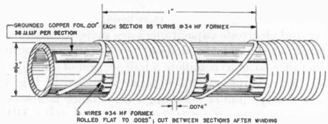
Fig. 21A—Equalized, section-wound delay line, impedance 1000 ohms.
