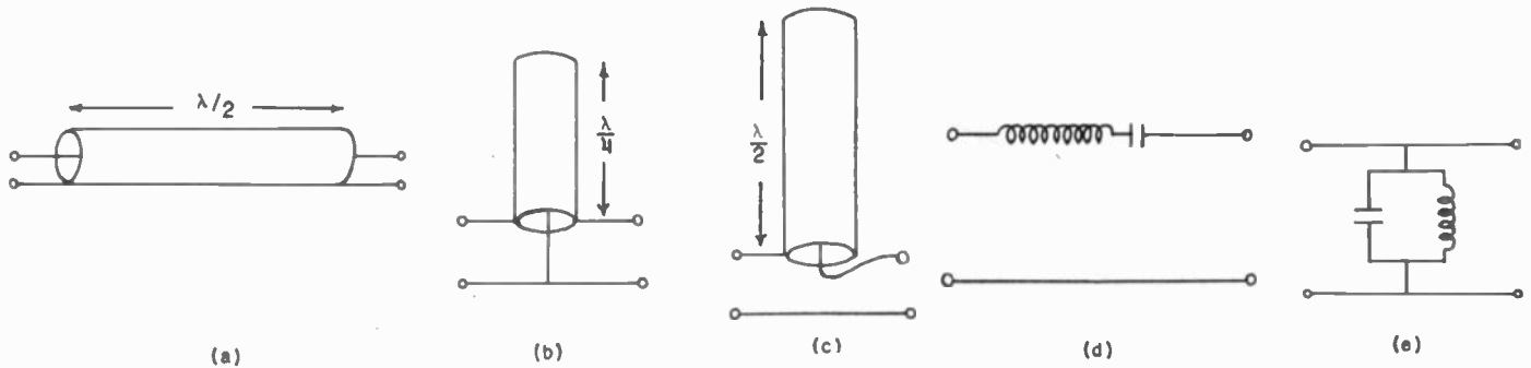
Fig. 2—Typical resonator elements.
