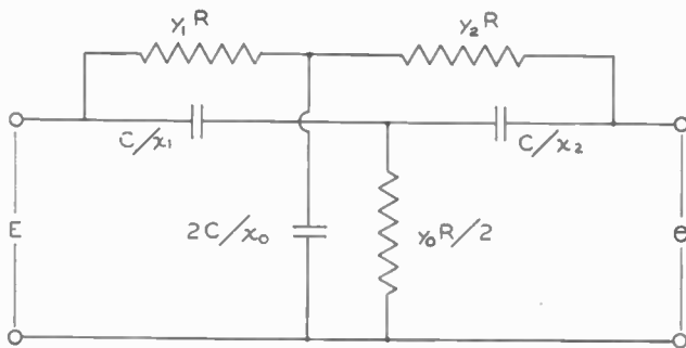
Fig. 1—Resistance-capacitance filter circuit.
