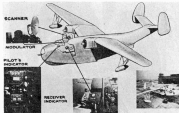
Fig. 9—AN/APS-2 radar in Mariner (PBM-3).
