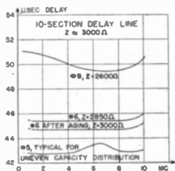
Fig. 22B—Delay.
