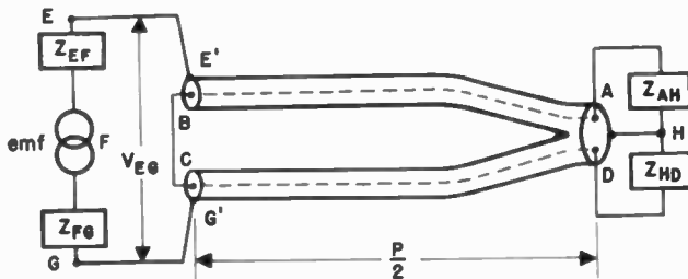
Fig. 3—Modified equivalent circuit showing coaxial lines.
