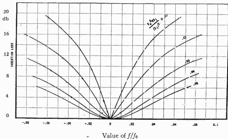
Fig. 2—Universal insertion-loss versus frequency characteristics of a single-resonant-circuit band-pass filter.
