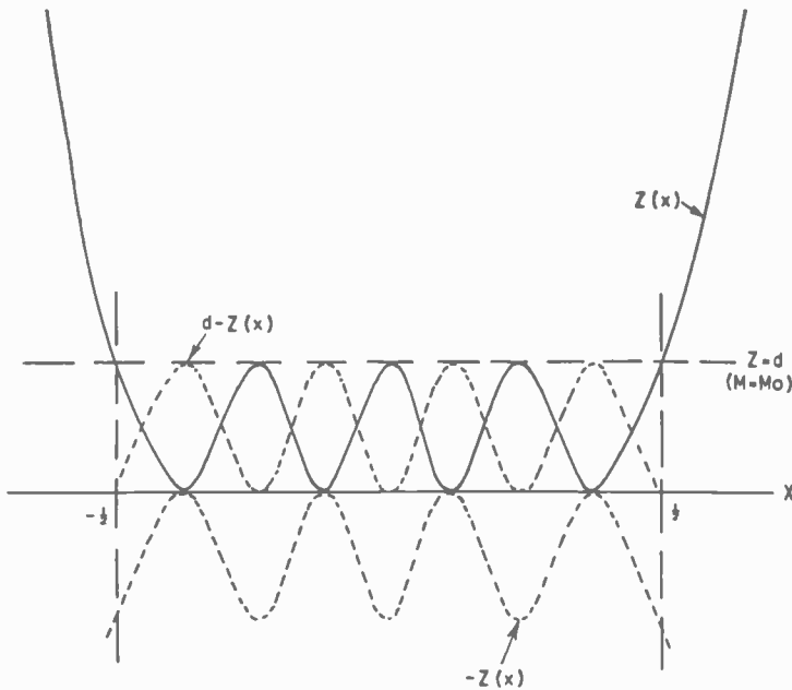
Fig. 6—Optimum Z(x) and bounds for p(x) .
