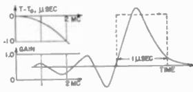
C Phase distortion only.
