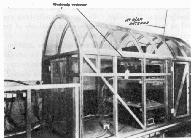
Fig. 56—BTM-1 systems test, looking aft.
