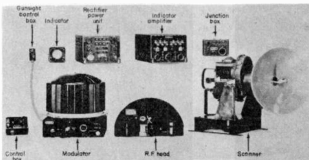
Fig. 43—AN/APS-6 intercept radar system assembly.
