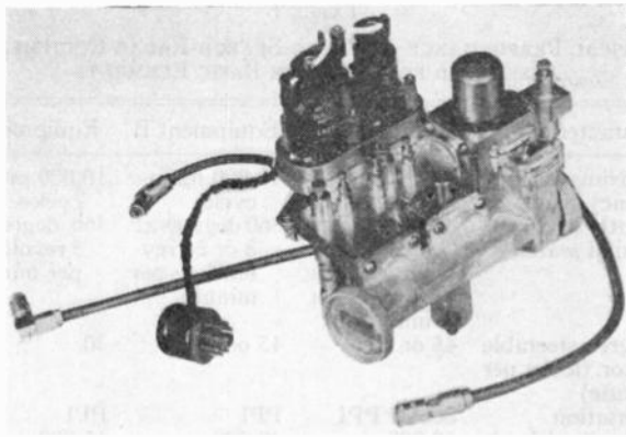
Fig. 27—Mixer assembly, showing radar and beacon local oscillators, cavities, T-R and R-T assemblies, and associated plumbing.
