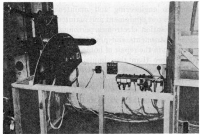
Fig. 55—BTM-1 systems test, looking forward.
