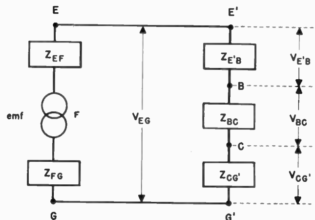
Fig. 2—Equivalent circuit of shield and gap impedances.
