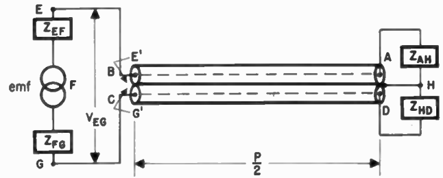
Fig. 4—Simplification of transmission-line connections.
