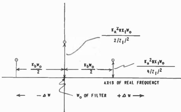
Fig. 9—Location of the roots of the impedance determinant for the triple-resonant-circuit filter in the complex-impedance plane.
