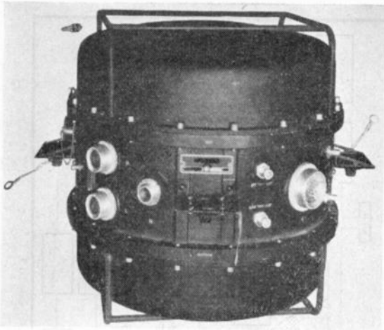
Fig. 22—Modulator-power supply of modern aircraft search radar.
