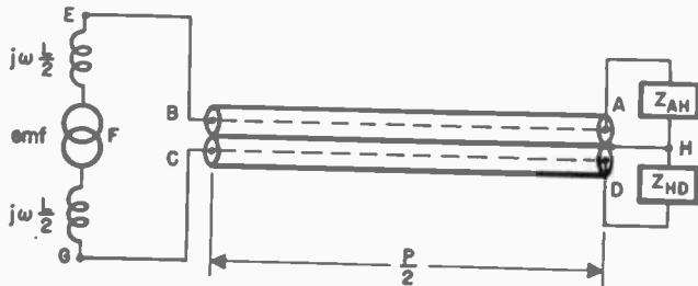
Fig. 5—Low-frequency condition corresponding to Fig. 4.
