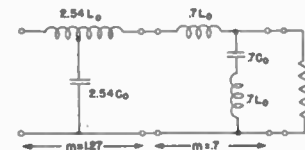
Fig. 26—Terminating half section, m =0.7, for delay network.
