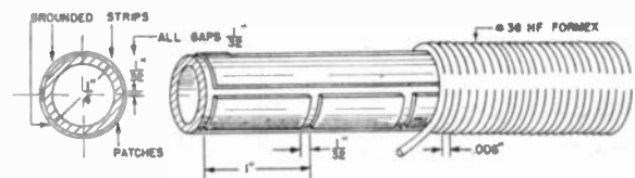
Fig. 19A—Patch-equalized delay line with 400 ohms impedance.
