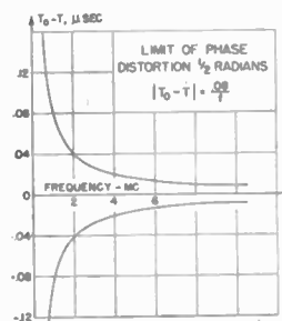
Fig. 2—Limits of delay distortion for \frac{1}{2} -radian phase distortion.
