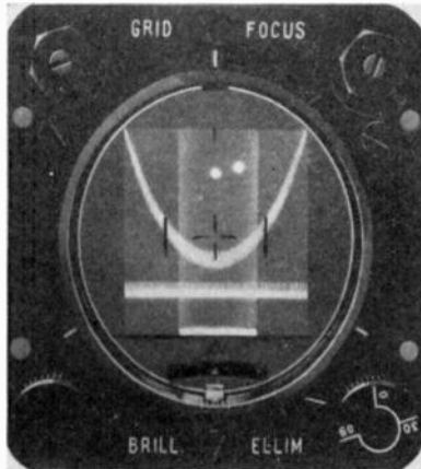
(a)—Intercept double-dot display. Target at 0-degree azimuth, 15-degree elevation, 2\frac{1}{2} -mile range.
