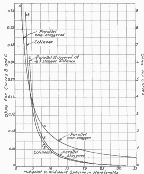
Fig. 6—Mutual impedance of half-wave dipoles in various orientations by simplified method.
