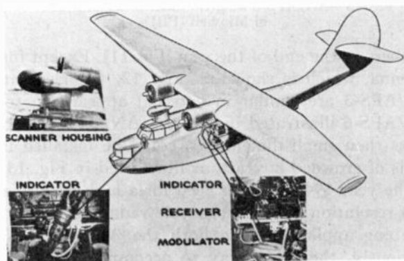
Fig. 11—AN/APS-3 radar in Catalina (PBY-5).
