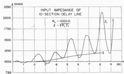
Fig. 21D—Impedance.
