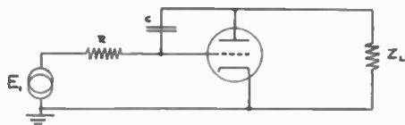
Fig. 3—Integrating amplifier.
