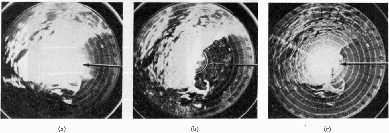
Fig. 35—Comparison of anticlutter circuits applied to normal radar-receiver operation. 100-mile sweep; altitude 10,000 feet. (a) Receiver normal—no anticlutter circuits. (b) Sensitivity time control applied to radar receiver. (c) Combination of all anticlutter circuits, STC, IAVC, FTC, and detector balanced bias applied to radar receiver.
