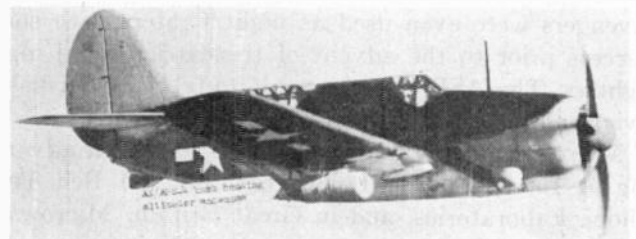
Fig. 15—AN/APS-4 radar in Helldiver (SB2C-4) showing wing-bomb-type installation. (Note also AN/APN-1 altimeter antennas.)
