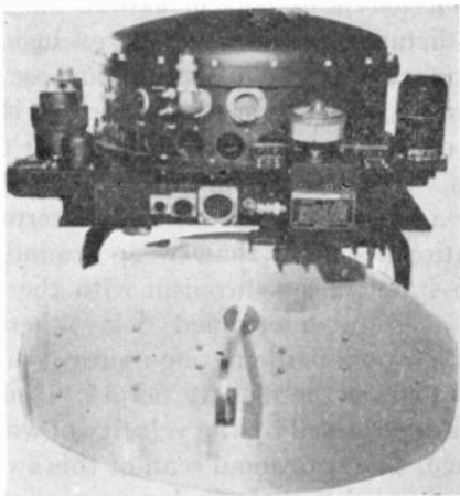
Fig. 28—All-around-looking antenna assembly of modern aircraft search radar with transmitter-receiver and pressurizing pump mounted in place.
