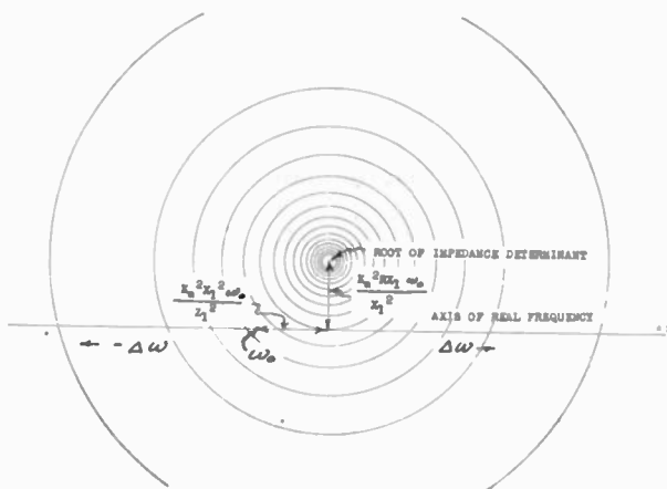
Fig. 5—Location of the root of the impedance determinant for the single-resonant-circuit filter together with contours of constant insertion loss in the complex-frequency plane.
