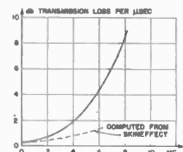
Fig. 21C—Attenuation.
