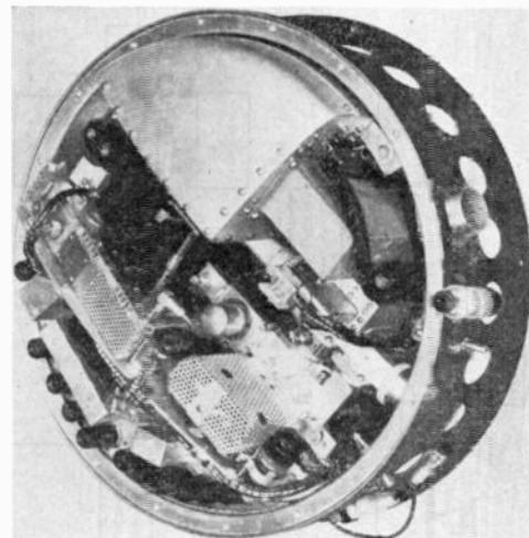
Fig. 26—Interior top view of transmitter-receiver.
