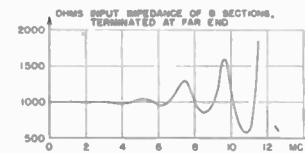
Fig. 25D—Impedance.
