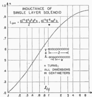
Fig. 3—Inductance of single-layer solenoid as function of l/d .
