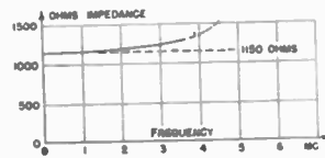
Fig. 20D—Impedance.
