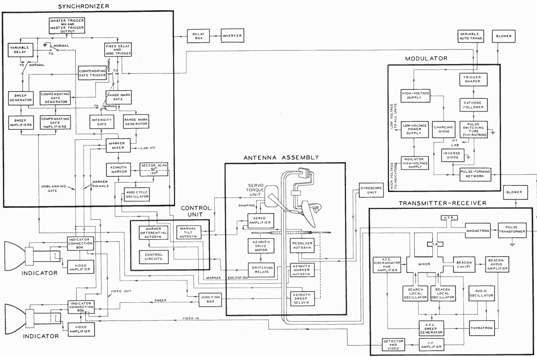
Fig. 20—Functions of primary elements of search radar shown in Fig. 19.
