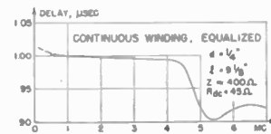
Fig. 19B—Delay.
