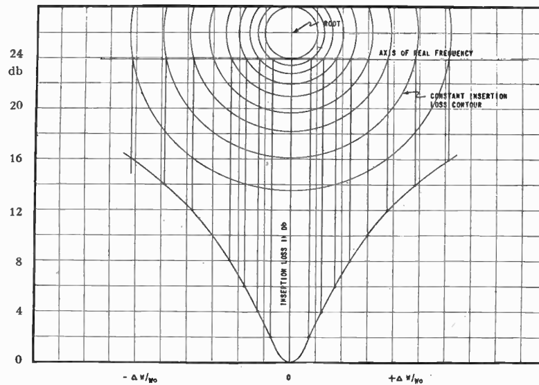
Fig. 6—Method of constructing the insertion-loss versus frequency characteristics from the contours of constant insertion loss of Fig. 5 for the case of the single-resonant-circuit filter.
