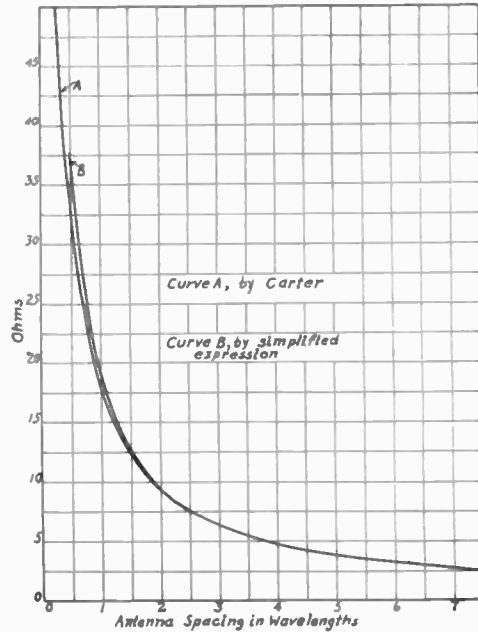
Fig. 5—Mutual impedance of nonstaggered parallel half-wave dipoles. Absolute values by Carter versus those by simplified method.
