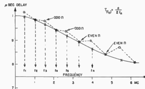
Fig. 11—Plot of time-delay characteristics from observed data.
