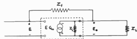
Fig. 2—Equivalent circuit for determination of A .
