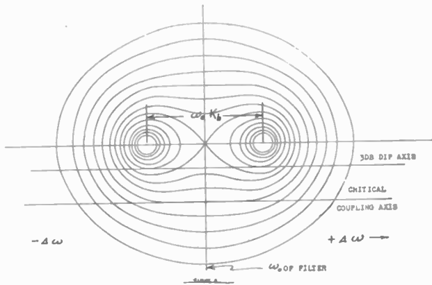
Fig. 8—Contours of constant insertion loss in the complex-impedance plane for the case of the double-resonant-circuit filter.
