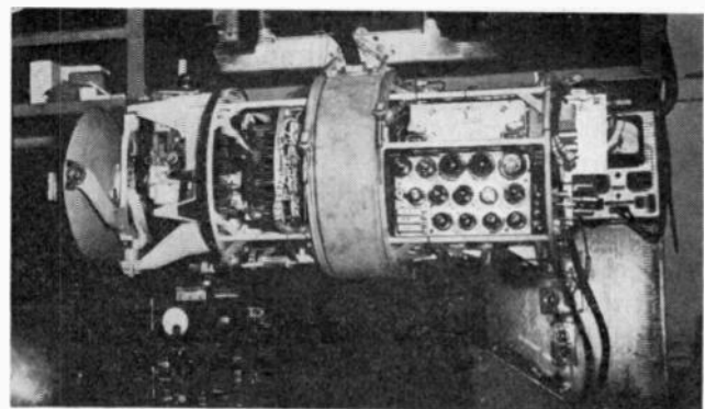
Fig. 16—AN/APS-4 radar, bomb housing removed, and associated test equipment.
