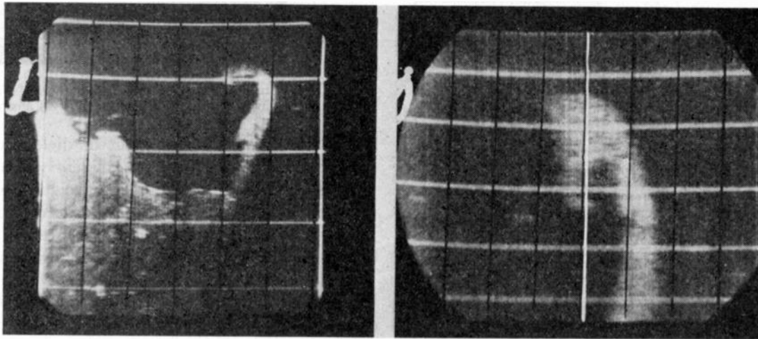
Fig. 37—Cape Cod on Type-B scan at long and short ranges illustrating distortion inherent at short range.
