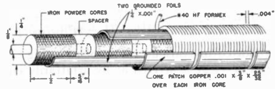
Fig. 23A—Equalized delay line with iron-powder cores.
