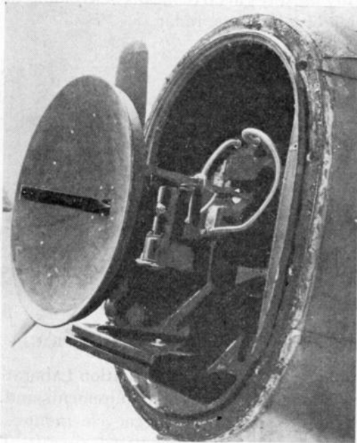
Fig. 12—AN/APS-3 radar antenna installation in Ventura (PV-1).
