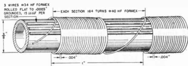
Fig. 22A—Section-wound delay line, impedance 3000 ohms.
