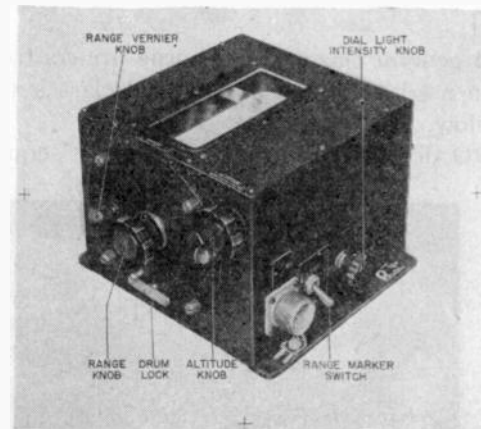
Fig. 51—H+B-type bombing computer used with AN/APS-15 radar.
