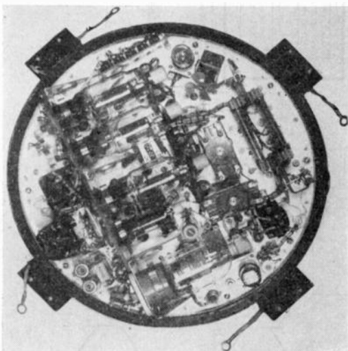
Fig. 23—Interior view of modulator.
