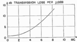
Fig. 22C—Attenuation.
