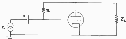
Fig. 4—Differentiating amplifier.
