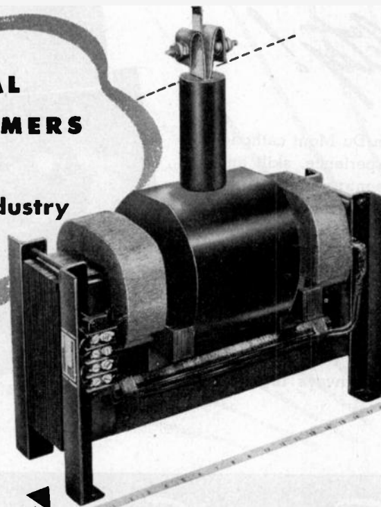
"Electro" Filament Transformer—Plastic Insulated, Dry Type, for External Anode 50 K.W. tube. 25 volts, 415 Amps. Short circuit, 750 Amps. 25 K.V. D.C. Wkg. Overall dimensions: 19 1/2" long x 8 1/4" wide x 18" high.
