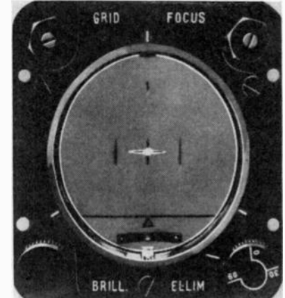
(c)—Intercept gunsight display. Target bore-sighted, range 400 yards.
