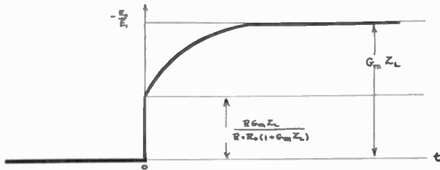
Fig. 6—Sweep-circuit output-voltage wave form.
