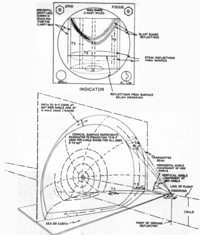
Fig. 44—Intercept spiral scan and display of resultant information.
