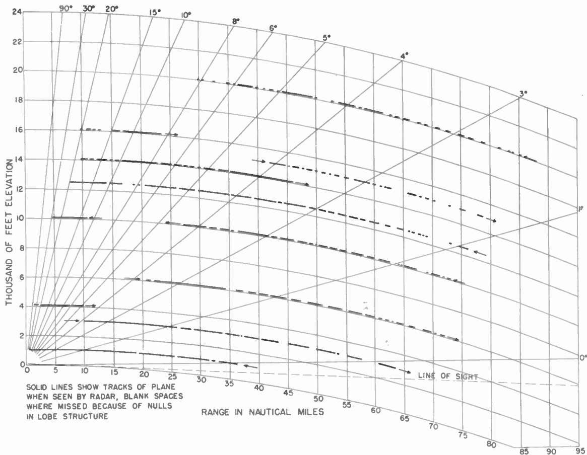
Fig. 7—Coverage on TBM plane over water.
