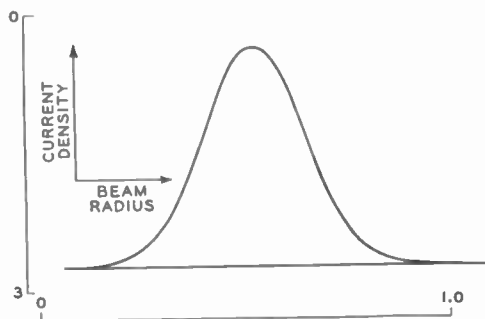
Fig. 5—Current-density distribution obtained by "slit-scanning" experiments.
