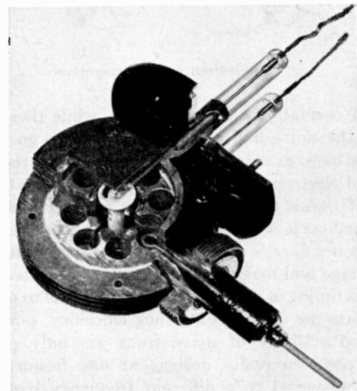
Fig. 22—Cutaway view of magnetron.
