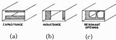
Fig. 36—Wave-guide matching diaphragms.
