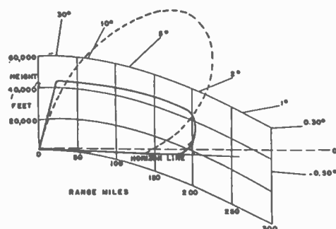
Fig. 63—Cosecant-squared beam.
