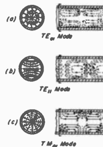
Fig. 31—Modes in circular wave guide.
