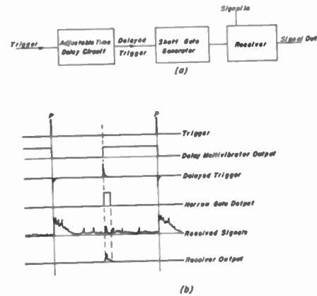
Fig. 51—"Short-gated" receiver.
