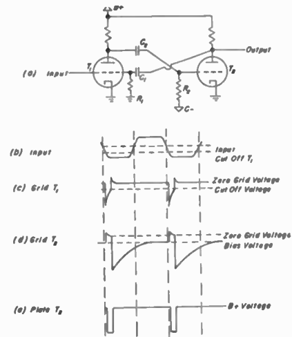
Fig. 11—Multivibrator and wave forms.
