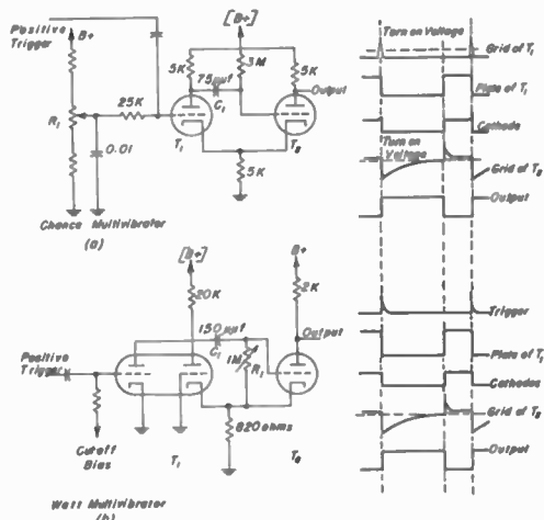
Fig. 67—Cathode-coupled multivibrators.
