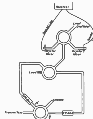
Fig. 47—Full-wave balanced mixer.
