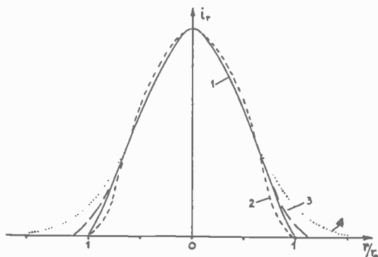
Fig. 7—Radial-current distribution in electron beam. Curve 1: At cathode (calculated). Curve 2: at position of final lens (measured). Curve 3: Same as 1, but corresponding to “slit scanning.” Curve 4: Gaussian distribution.
