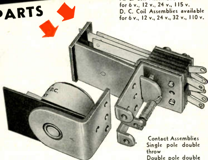
Series 200 Relay
