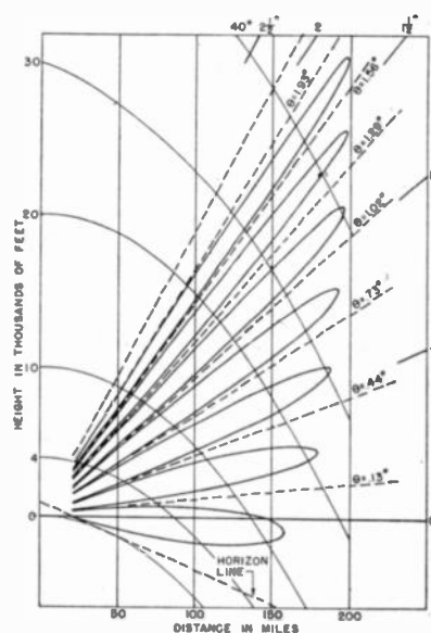
(b) Antenna height = 1000 feet.
