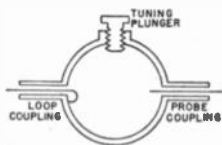
Fig. 17—Resonant cavity.
