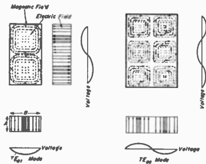
Fig. 30—Modes in rectangular wave guide.
