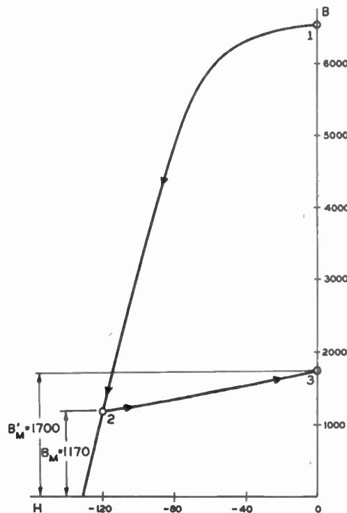
Fig. 7—Increase in magnetization of 1000-cycle signal upon removal of demagnetizing field.
