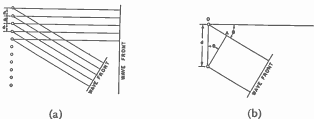
Fig. 54—Diffraction antenna.
