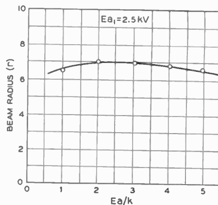
Fig. 4—Experimental plot of the variation of r with E_a/k .
