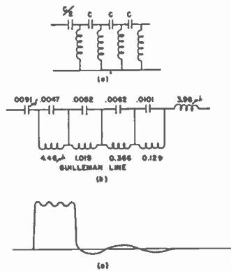
Fig. 15—Pulse-forming network. (a) Artificial line (b) Pulse network (c) Pulse output
