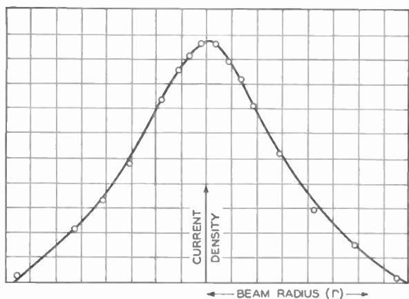
Fig. 6—Experimental plot of current distribution obtained by "hole-scanning" method.
