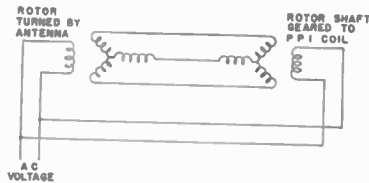
Fig. 75—Selsyn drive.
