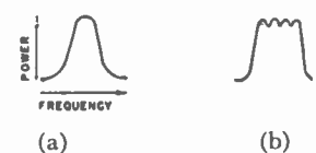
Fig. 28—Frequency response. (a) Single circuit (b) Coupled circuits
