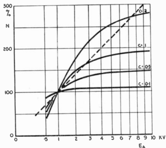
Fig. 2.—Definition (reciprocal spot size) as function of final anode voltage E_a in the presence of spherical aberration for constant primary spot size d_0 , as predicted by new theory. Dashed line represents square-root law as predicted by "crossover" theory.
