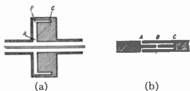
Fig. 27—Choke joint.
