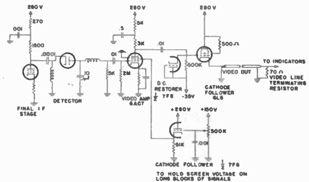
Fig. 49—Detector and video amplifier.
