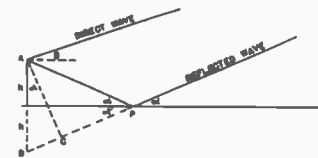
Fig 4—Reflection of radar beam.
