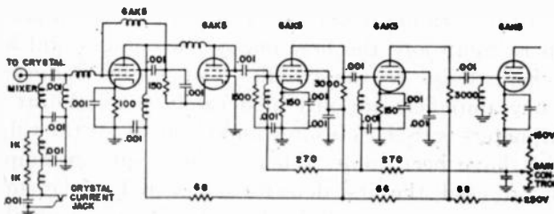
Fig. 48—Receiver input.
