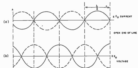
Fig. 24—Standing waves.
