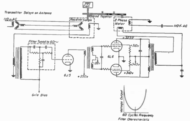
Fig. 76—Alternating-current servo system.
