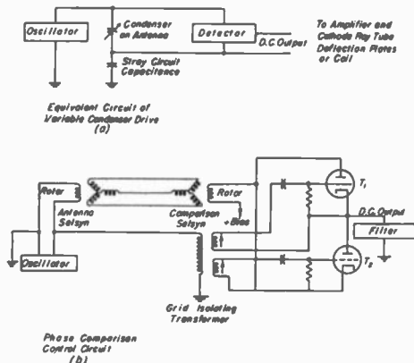
Fig. 72—B-scan azimuth sweep-control circuits.
