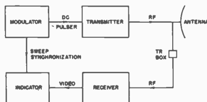
Fig. 9—Block diagram of basic radar set.
