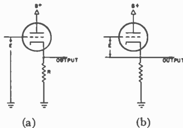
Fig. 13—(a) Cathode follower. (b) Bootstrap amplifier.
