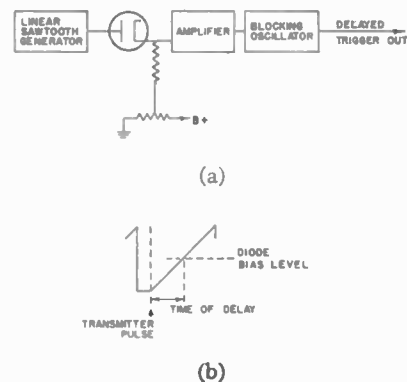
Fig. 68—Saw-tooth delay circuit.
