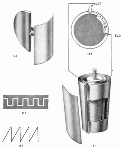
Fig. 61—Foster scanner.
