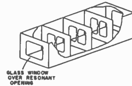
Fig. 37—Wave-guide broadband transmit-receive box.
