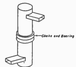
Fig. 32—Rotating wave-guide joint.
