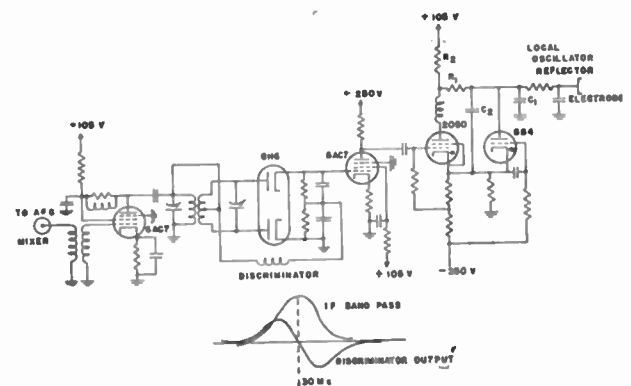
Fig. 52—Automatic frequency control.
