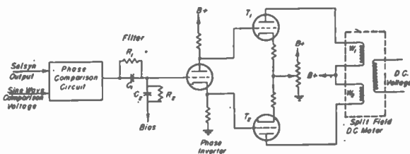
Fig. 77—Direct-current servomotor drive.
