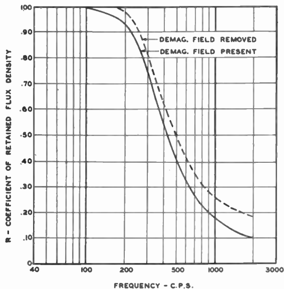
Fig. 8—Coefficient of retained flux density — k for 0.004-inch wire at 2\frac{1}{2} feet per second.
