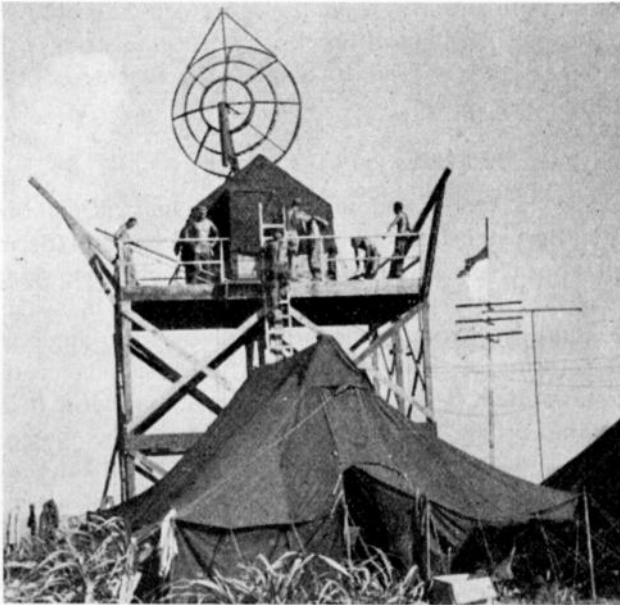
Fig. 78—AN/TPS-3 set placed on tower to clear surrounding obstacles.
