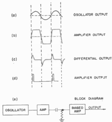
Fig. 10—Square-wave generation from sine wave.
