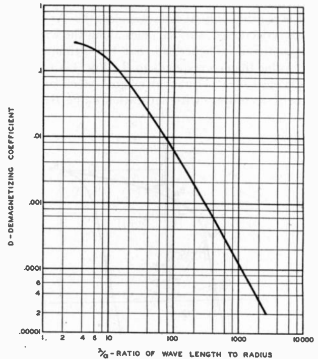
Fig. 5—Demagnetizing coefficients for sinusoidally magnetized wire.
