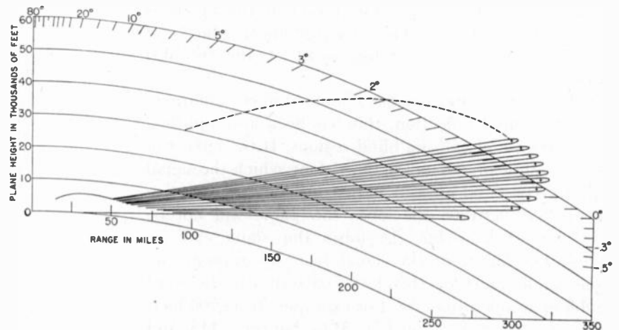
Fig. 6—Vertical coverage diagram for 3000 megacycles. Antenna height, 100 feet.
