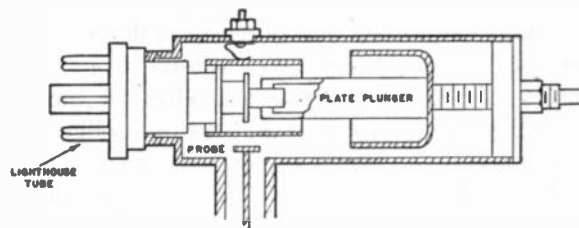
Fig. 18—Lighthouse tube in re-entrant cavity.
