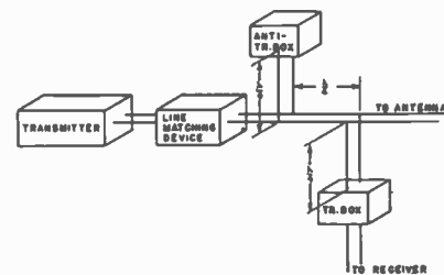
(a) Block diagram
