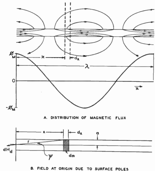
Fig. 4—Demagnetizing effect of surface poles.
