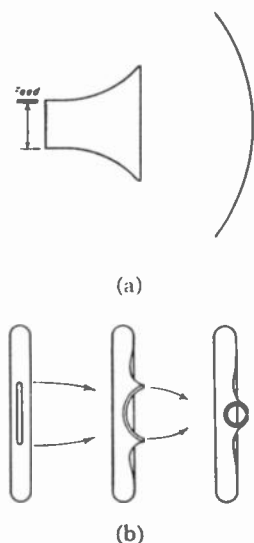
Fig. 60—Robinson feed.
