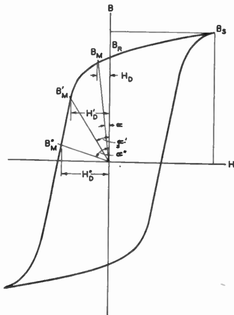
Fig. 3—Magnetization retained by a wire.
