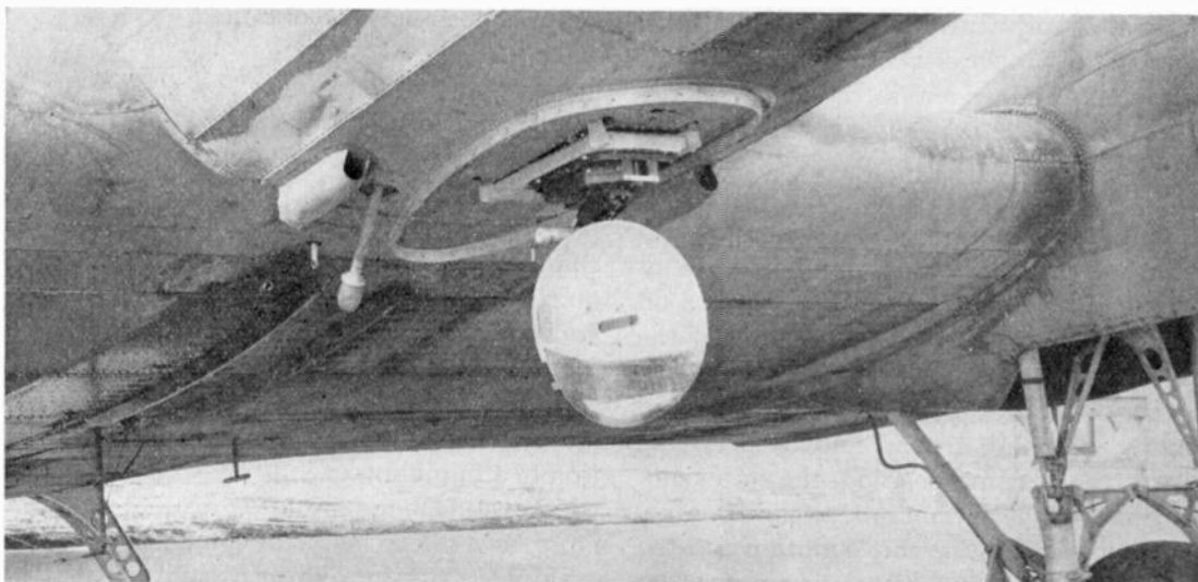
Fig. 82—AN/APS-10 antenna on C-47, antenna housing removed.
