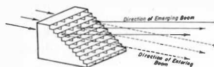
Fig. 59—Wave-guide prism.
