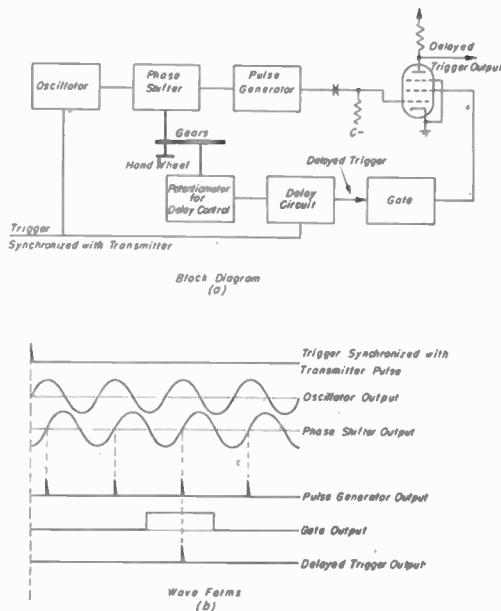
Fig. 70—Accurate range delay circuit.
