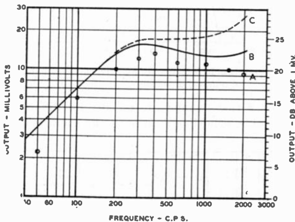
Fig. 9—Calculated and measured output versus frequency for a magnetic record.
