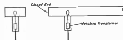
Fig. 33—Probe transition section.
