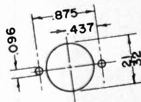
MOUNTING LAYOUT
