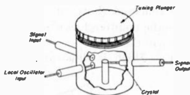
Fig. 43—Tuned mixer.
