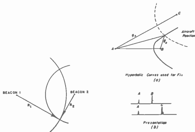
Fig. 84—Range triangulation. Fig. 85—"Gee" system for navigation.
