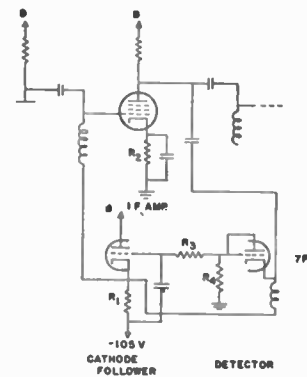
Fig. 50—Back-bias circuit.
