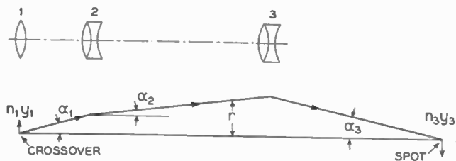
Fig. 3—Application of Helmholtz-Lagrange law.
