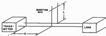
Fig. 25—Transmission line with T junction.
