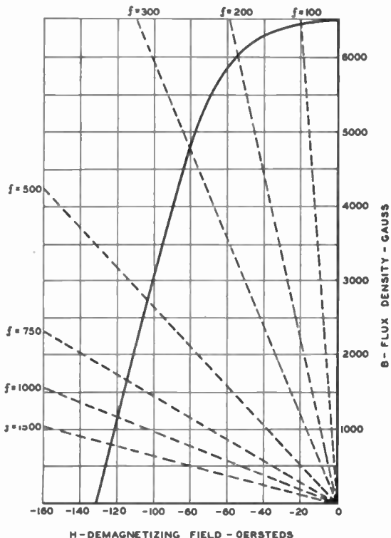
Fig. 6—Graphical solution for B_M at various frequencies. Wire diameter = 0.004 inch. Wire velocity = 2\frac{1}{2} feet per second.
