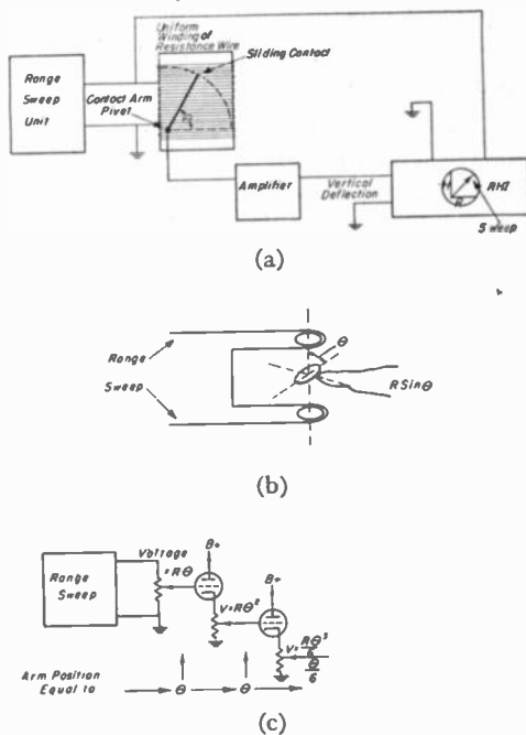
Fig. 73—Range-height-indicator sweep circuits.
