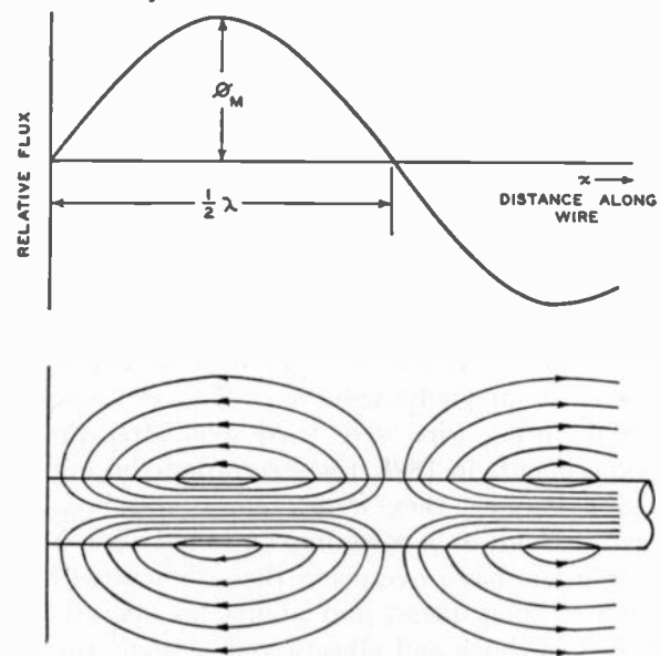
Fig. 2—Sinusoidal flux distribution.
