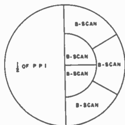
Fig. 79—Possible scope coverage.
