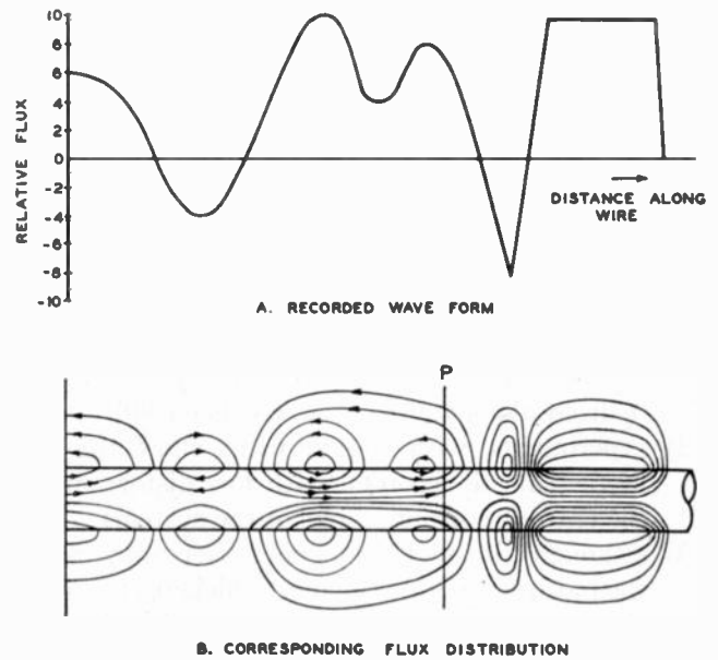
Fig. 1—Flux distribution around a wire record.
