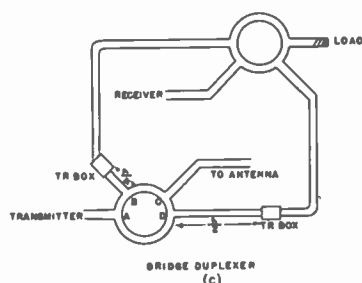
Fig. 40—"Rat-race" bridge duplexer.
