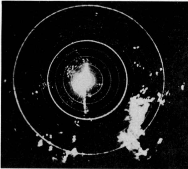
Fig. 8—Echoes from dense clouds on 10-centimeter radar.
