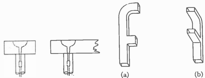
Fig. 35—T's and bends in wave guide. (a) H -plane bend and T. (b) E -plane bend and T.
