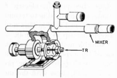
Fig. 38—Tuned transmit-receive box.
