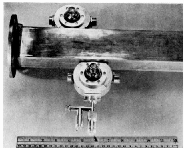
(b) 10-centimeter duplexer. Fig. 39—Duplexing system.
